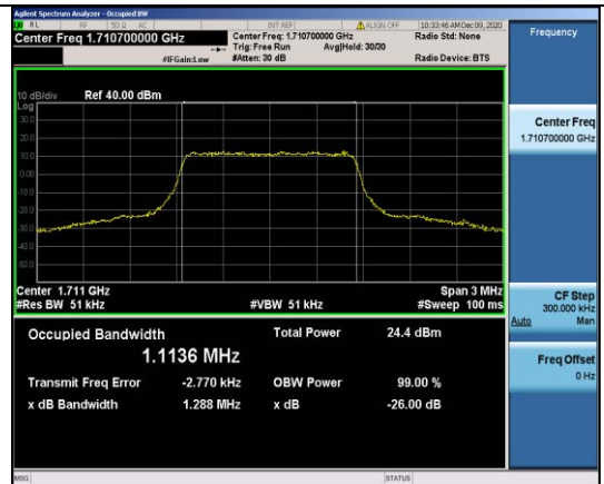
Band4-1.4MHz-QPSK-19957-6RB#0-1.1136
