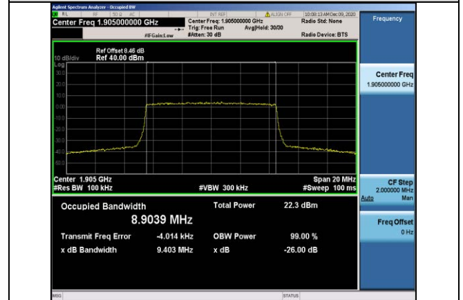
Band2-10MHz-QPSK-19150-50RB#0-8.9039
