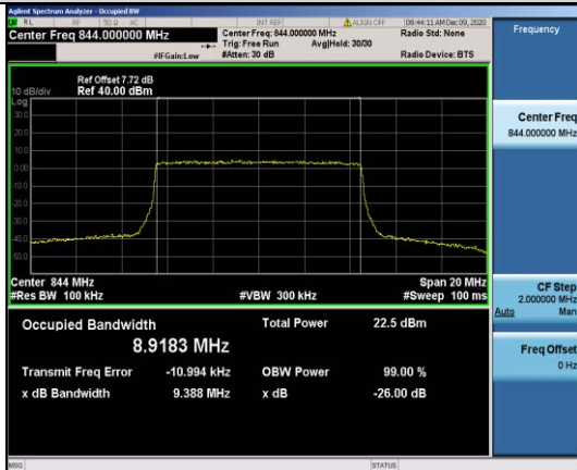
Band5-10MHz-16QAM-20600-50RB#0-8.9183
