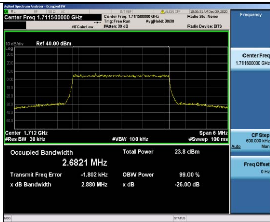
Band4-3MHz-16QAM-19965-15RB#0-2.6821
