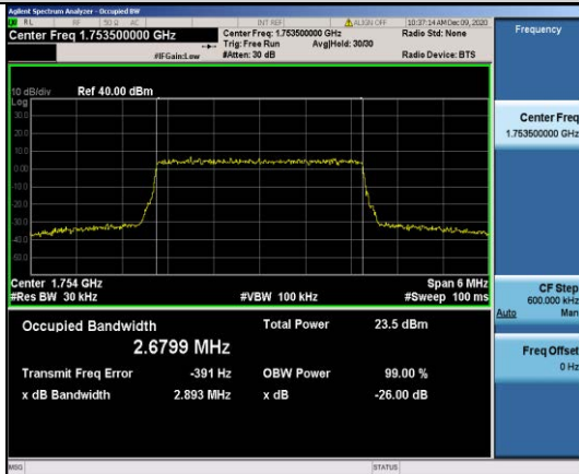
Band4-3MHz-16QAM-20385-15RB#0-2.6799
