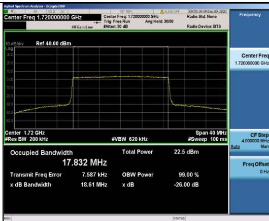
Band4-20MHz-16QAM-20050-100RB#0-17.832
