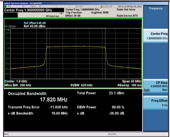
Band2-20MHz-QPSK-19100-100RB#0-17.820
