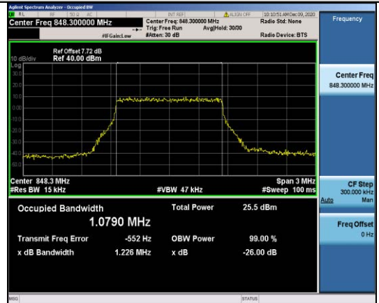
Band5-1.4MHz-QPSK-20643-6RB#0-1.0790
