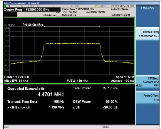
Band4-5MHz-QPSK-20375-25RB#0-4.4701
