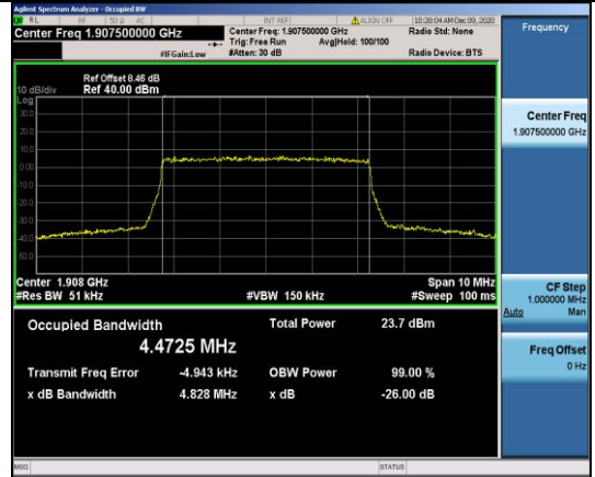
Band2-5MHz-QPSK-19175-25RB#0-4.4725
