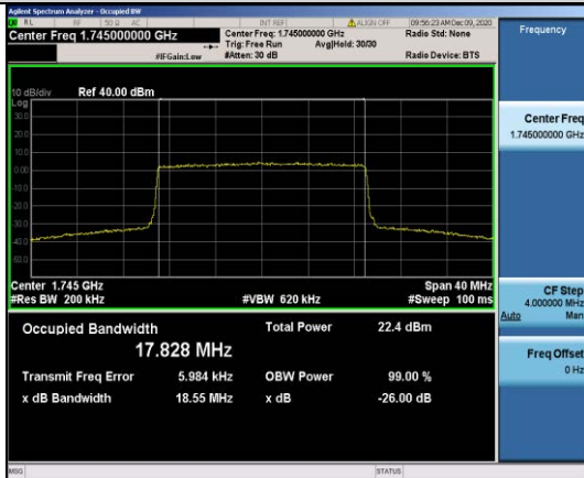
Band4-20MHz-16QAM-20300-100RB#0-17.828
