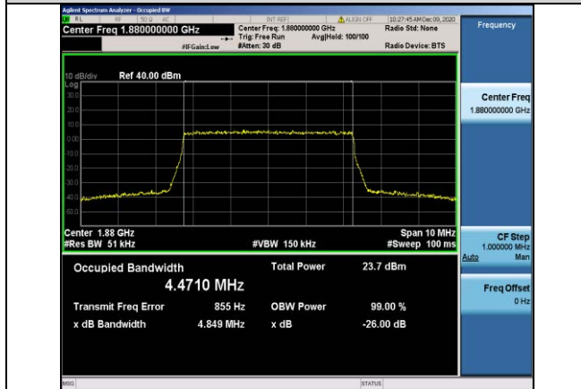
Band2-5MHz-16QAM-18900-25RB#0-4.4710
