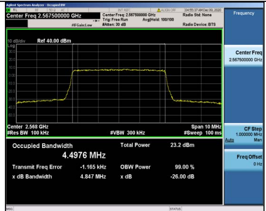
Band7-5MHz-QPSK-21425-25RB#0-4.4976
