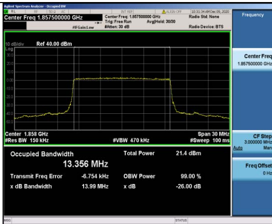
Band2-15MHz-16QAM-18675-75RB#0-13.356
