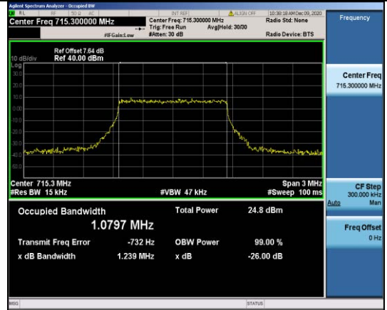
Band12-1.4MHz-QPSK-23173-6RB#0-1.0797
