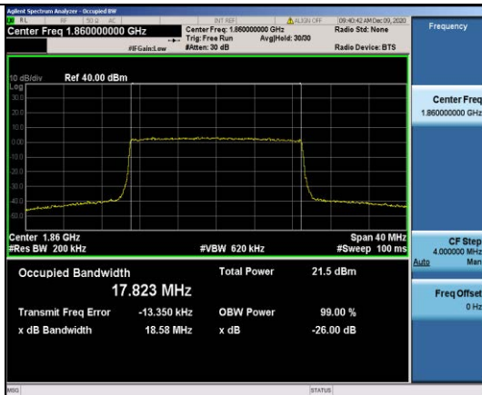
Band2-20MHz-16QAM-18700-100RB#0-17.823
