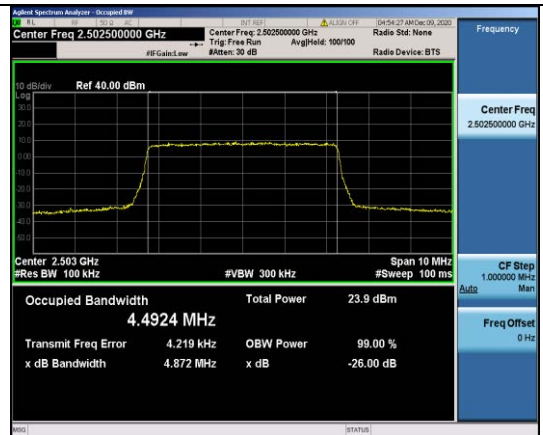
Band7-5MHz-QPSK-20775-25RB#0-4.4924
