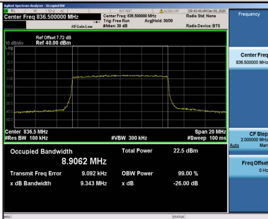
Band5-10MHz-16QAM-20525-50RB#0-8.9062
