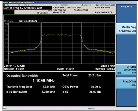
Band4-1.4MHz-QPSK-20175-6RB#0-1.1099
