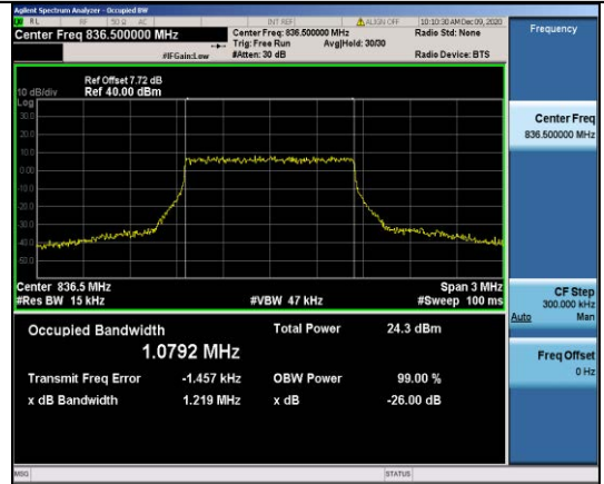
Band5-1.4MHz-QPSK-20525-6RB#0-1.0792
