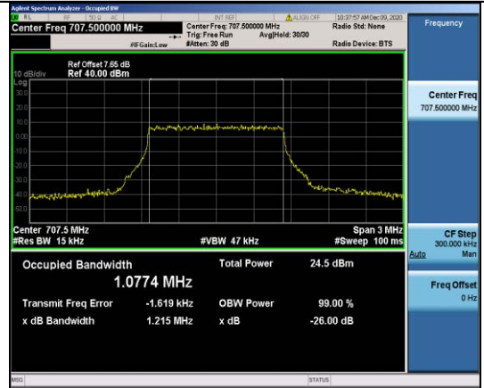
Band12-1.4MHz-QPSK-23095-6RB#0-1.0774
