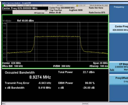
Band5-10MHz-16QAM-20450-50RB#0-8.9274
