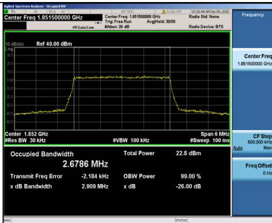
Band2-3MHz-16QAM-18615-15RB#0-2.6786
