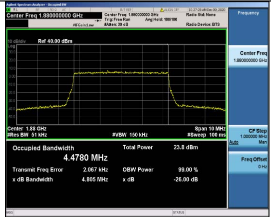
Band2-5MHz-QPSK-18900-25RB#0-4.4780
