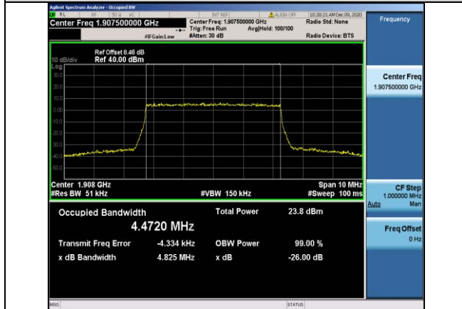
Band2-5MHz-16QAM-19175-25RB#0-4.4720
