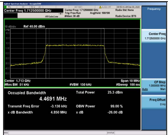
Band4-5MHz-QPSK-19975-25RB#0-4.4691
