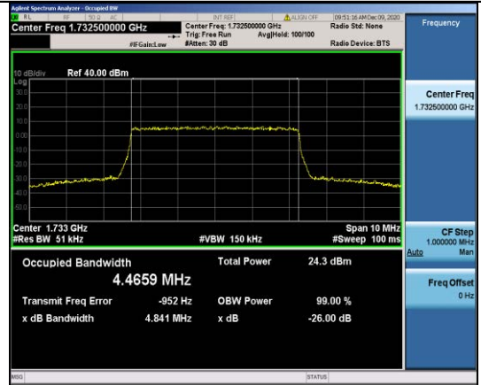
Band4-5MHz-QPSK-20175-25RB#0-4.4659
