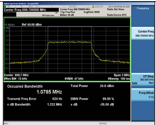
Band12-1.4MHz-QPSK-23017-6RB#0-1.0785
