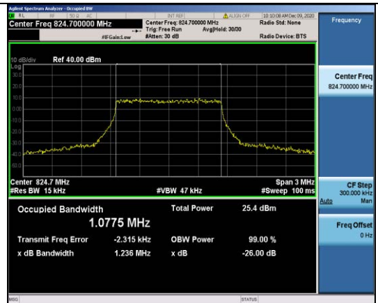
Band5-1.4MHz-QPSK-20407-6RB#0-1.0775
