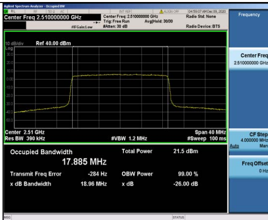
Band7-20MHz-16QAM-20850-100RB#0-17.885
