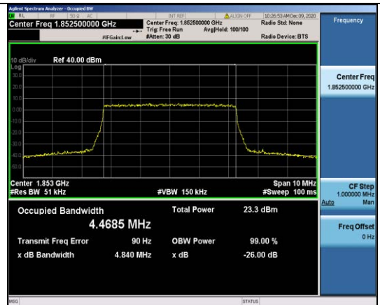
Band2-5MHz-QPSK-18625-25RB#0-4.4685
