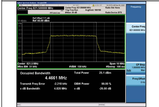
Band26-5MHz-QPSK-26765-25RB#0-4.4661
