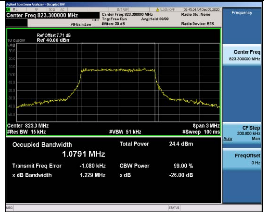
Band26-1.4MHz-16QAM-26783-6RB#0-1.0791
