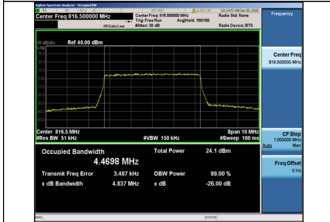
Band26-5MHz-16QAM-26715-25RB#0-4.4698
