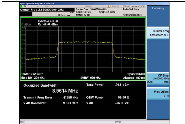
Band41-10MHz-16QAM-41190-50RB#0-8.9614
