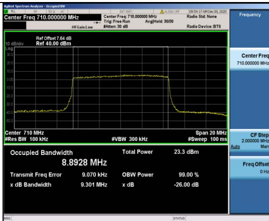
Band17-10MHz-QPSK-23790-50RB#0-8.8928
