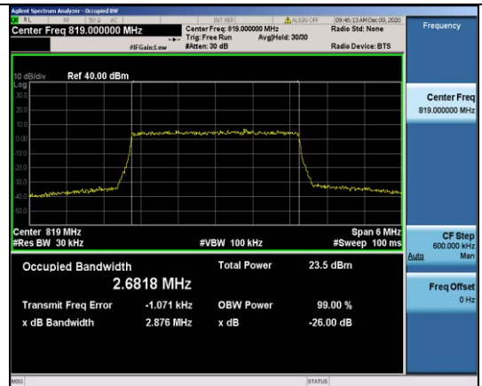
Band26-3MHz-16QAM-26740-15RB#0-2.6818
