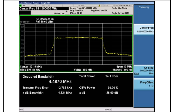
Band26-5MHz-16QAM-26765-25RB#0-4.4670
