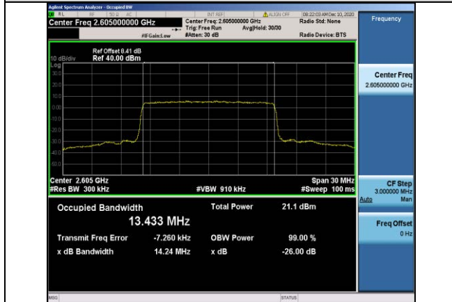
Band41-15MHz-QPSK-40740-75RB#0-13.433
