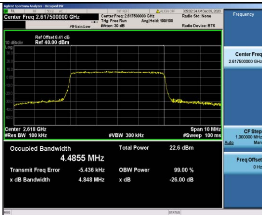
Band38-5MHz-16QAM-38225-25RB#0-4.4855
