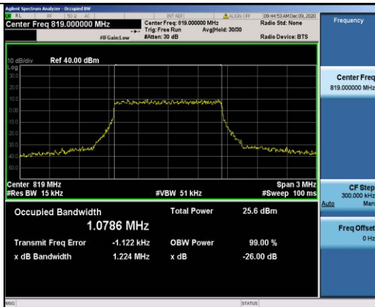
Band26-1.4MHz-QPSK-26740-6RB#0-1.0786
