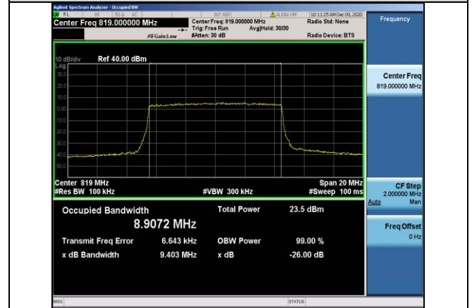
Band26-10MHz-QPSK-26740-50RB#0-8.9072
