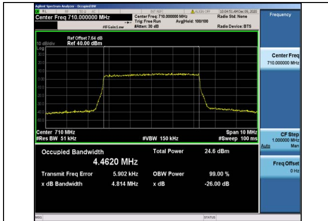
Band17-5MHz-QPSK-23790-25RB#0-4.4620
