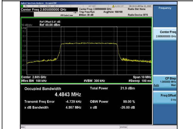
Band41-5MHz-QPSK-40740-25RB#0-4.4843
