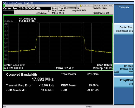
Band41-20MHz-QPSK-41140-100RB#0-17.893
