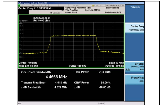
Band17-5MHz-16QAM-23790-25RB#0-4.4668
