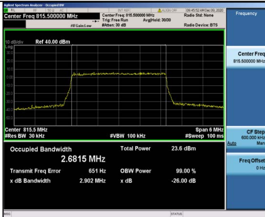
Band26-3MHz-16QAM-26705-15RB#0-2.6815
