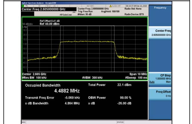
Band41-5MHz-16QAM-40740-25RB#0-4.4882
