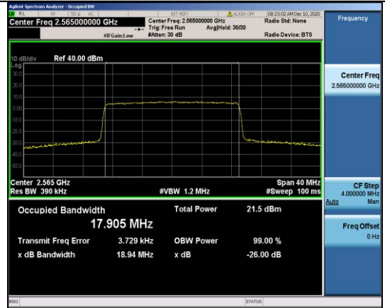
Band41-20MHz-QPSK-40340-100RB#0-17.905
