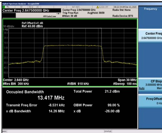
Band41-15MHz-16QAM-41165-75RB#0-13.417
