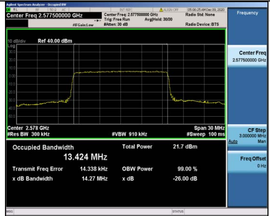
Band38-15MHz-16QAM-37825-75RB#0-13.424
