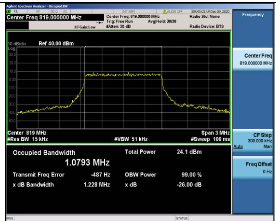
Band26-1.4MHz-16QAM-26740-6RB#0-1.0793
