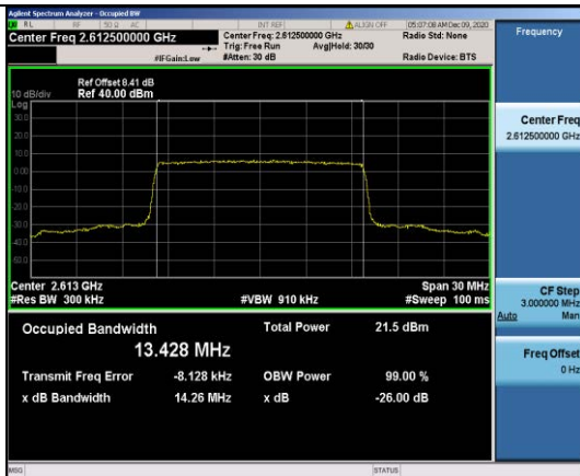
Band38-15MHz-16QAM-38175-75RB#0-13.428
