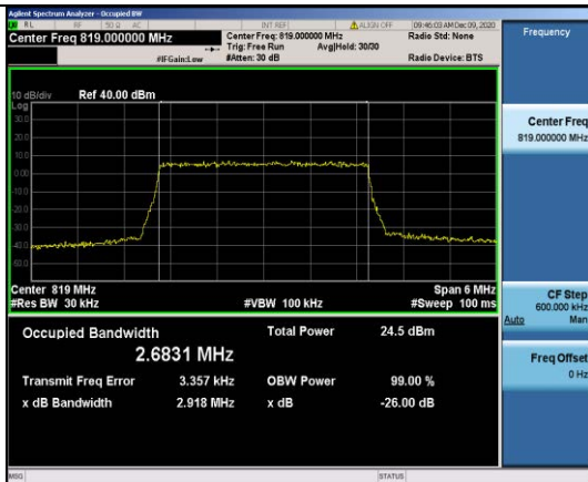
Band26-3MHz-QPSK-26740-15RB#0-2.6831
