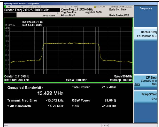
Band38-15MHz-QPSK-38175-75RB#0-13.422
