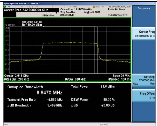
Band38-10MHz-QPSK-38200-50RB#0-8.9470
