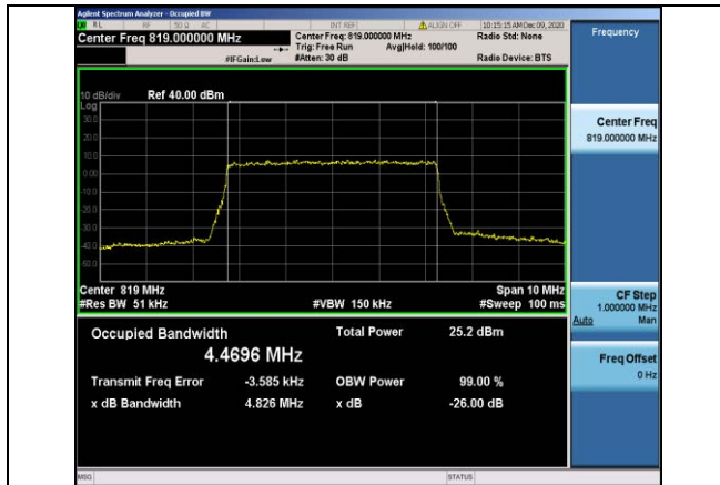
Band26-5MHz-QPSK-26740-25RB#0-4.4696
