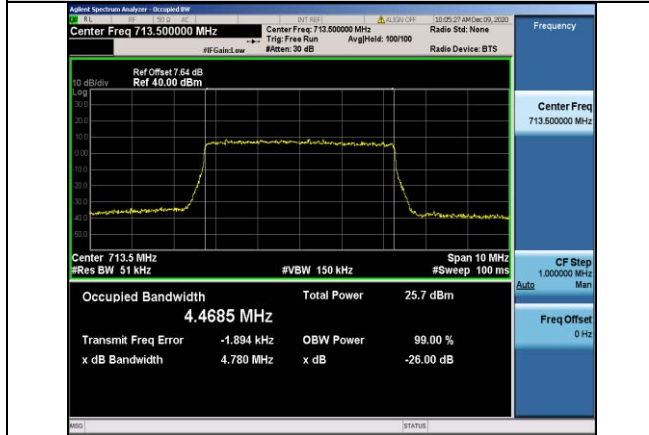
Band17-5MHz-QPSK-23825-25RB#0-4.4685
