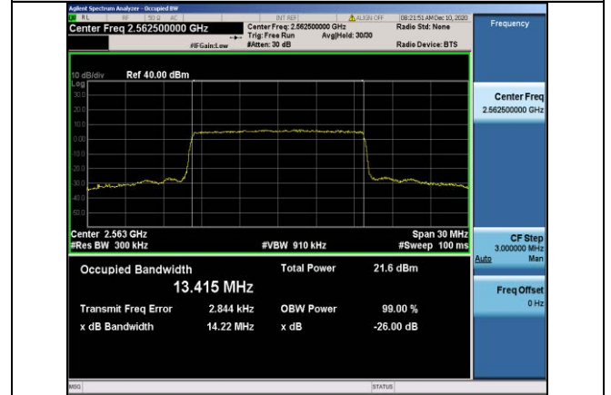
Band41-15MHz-16QAM-40315-75RB#0-13.415
