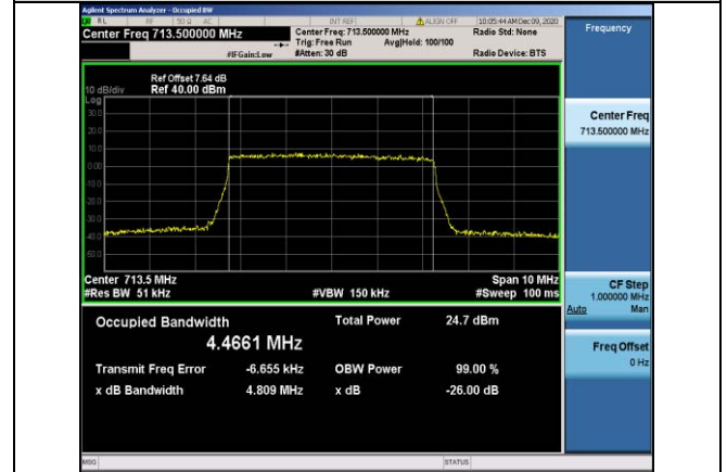
Band17-5MHz-16QAM-23825-25RB#0-4.4661
