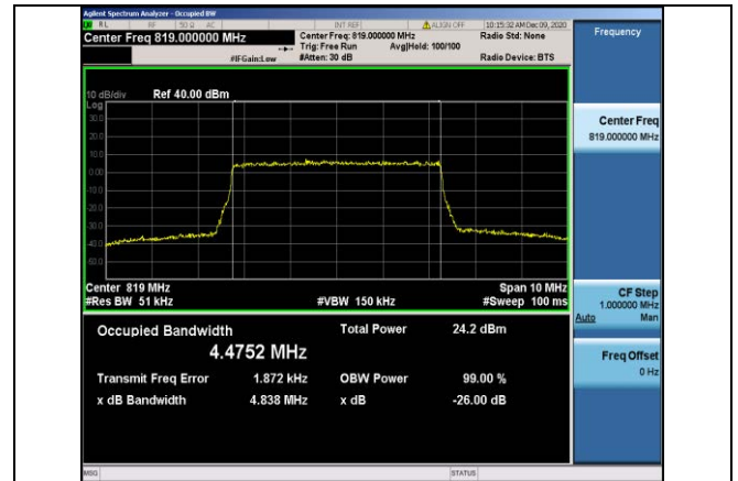
Band26-5MHz-16QAM-26740-25RB#0-4.4752
