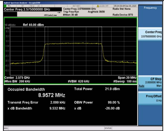
Band38-10MHz-16QAM-37800-50RB#0-8.9572
