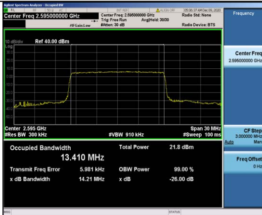
Band38-15MHz-QPSK-38000-75RB#0-13.410
