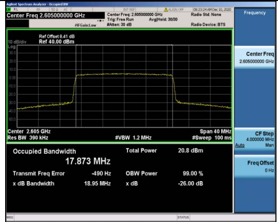
Band41-20MHz-16QAM-40740-100RB#0-17.873
