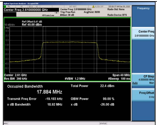
Band38-20MHz-QPSK-38150-100RB#0-17.884
