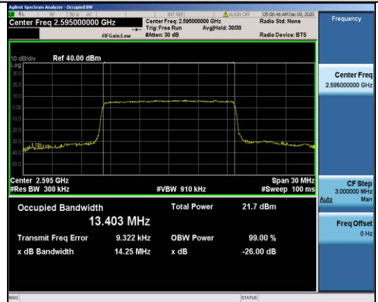
Band38-15MHz-16QAM-38000-75RB#0-13.403
