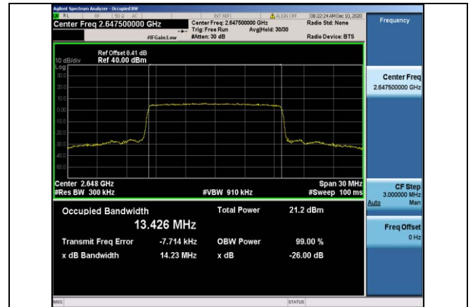
Band41-15MHz-QPSK-41165-75RB#0-13.426
