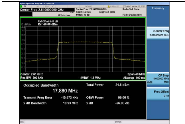
Band38-20MHz-16QAM-38150-100RB#0-17.880
