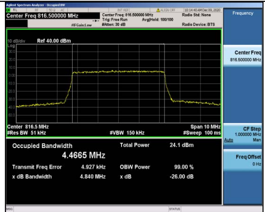
Band26-5MHz-QPSK-26715-25RB#0-4.4665
