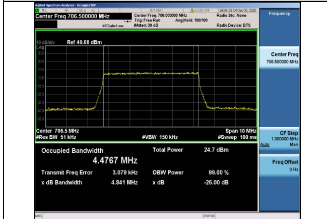
Band17-5MHz-16QAM-23755-25RB#0-4.4767
