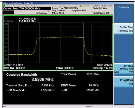
Band17-10MHz-16QAM-23790-50RB#0-8.8936
