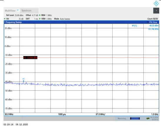
Band2-20MHz-QPSK-19100-1RB#0- Range1:30~1000MHz
