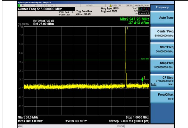
Band26-5MHz-QPSK-26715-1RB#0- Range1:30~1000MHz
