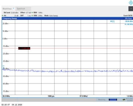
Band2-10MHz-QPSK-18900-1RB#0- Range1:30~1000MHz
