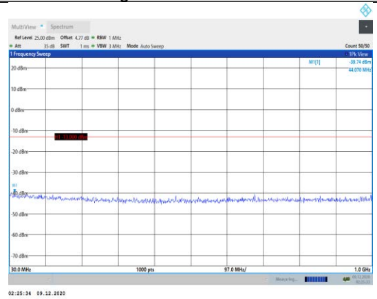
Band2-15MHz-16QAM-19125-1RB#0- Range1:30~1000MHz
