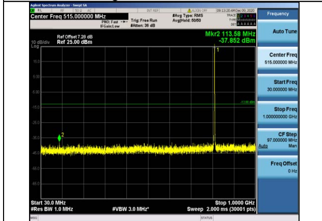
Band26-1.4MHz-16QAM-26697-1RB#0- Range1:30~1000MHz
