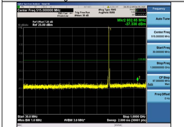
Band17-5MHz-16QAM-23755-1RB#0- Range1:30~1000MHz
