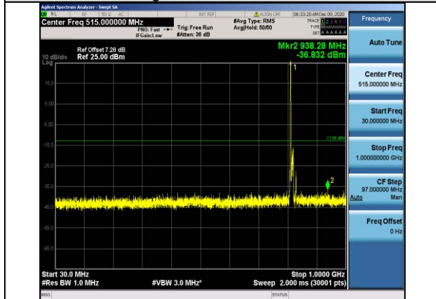
Band26-10MHz-QPSK-26740-1RB#0- Range1:30~1000MHz
