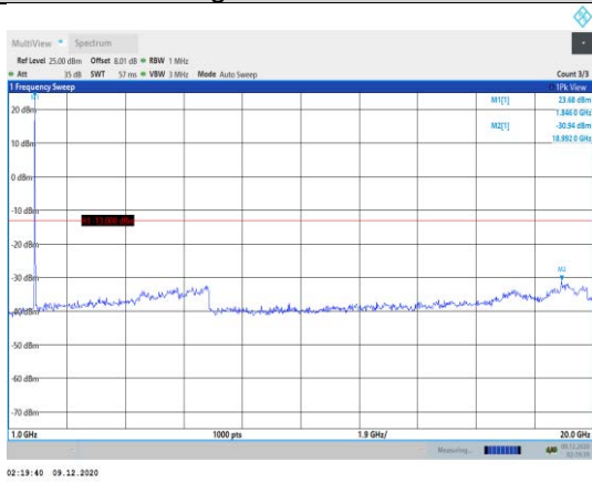
Band2-10MHz-16QAM-18650-1RB#0- Range2:1000~20000MHz
