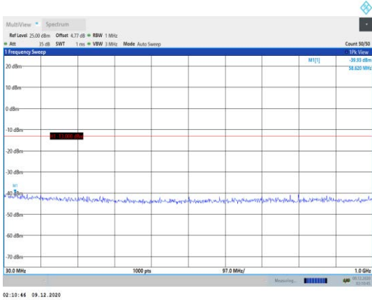
Band2-3MHz-16QAM-18900-1RB#0- Range1:30~1000MHz
