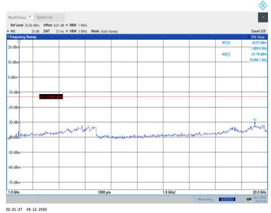
Band2-10MHz-16QAM-19150-1RB#0- Range2:1000~20000MHz
