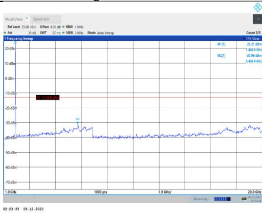
Band2-15MHz-QPSK-18675-1RB#0- Range2:1000~20000MHz
