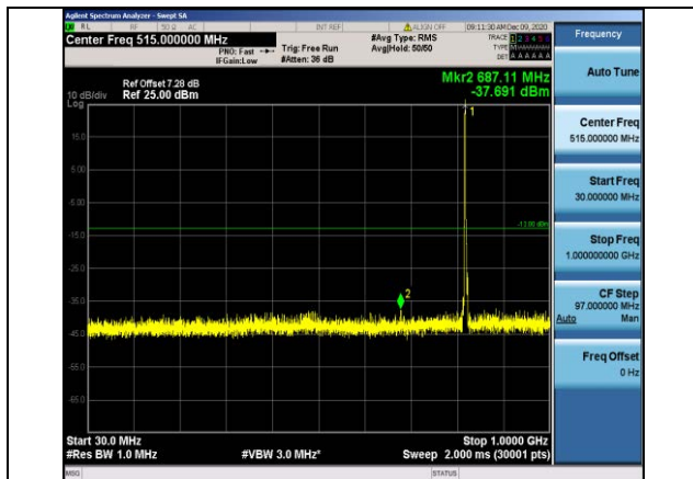
Band26-3MHz-QPSK-26775-1RB#0- Range1:30~1000MHz
