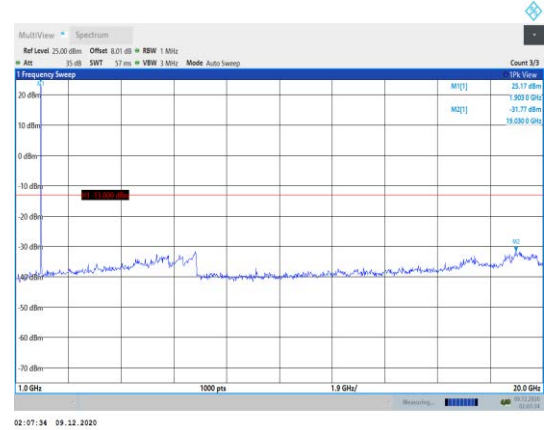
Band2-1.4MHz-16QAM-19193-1RB#0- Range2:1000~20000MHz
