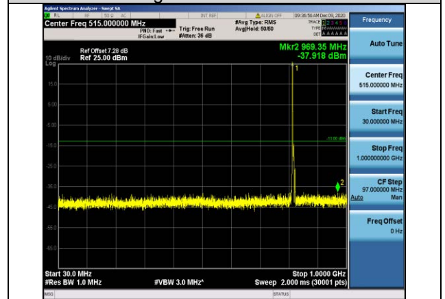
Band26-5MHz-16QAM-26740-1RB#0- Range1:30~1000MHz
