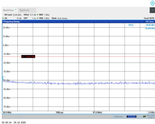
Band2-1.4MHz-QPSK-18900-1RB#0- Range1:30~1000MHz
