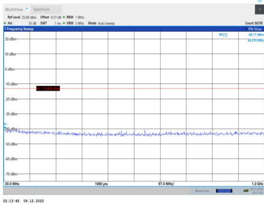
Band2-5MHz-QPSK-18625-1RB#0- Range1:30~1000MHz
