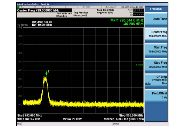
Band13-10MHz-16QAM-23230-1RB#0- Range4:793~805MHz
