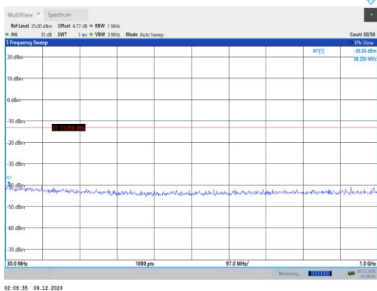
Band2-3MHz-QPSK-18615-1RB#0- Range1:30~1000MHz
