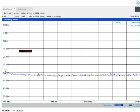
Band2-15MHz-16QAM-18900-1RB#0- Range1:30~1000MHz
