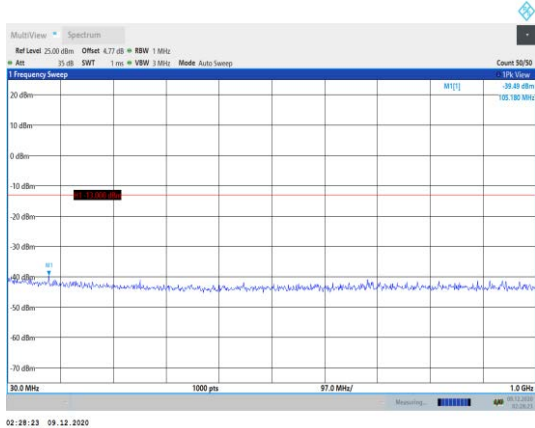
Band2-20MHz-QPSK-18900-1RB#0- Range1:30~1000MHz
