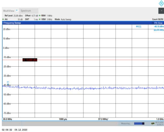
Band2-1.4MHz-16QAM-18900-1RB#0- Range1:30~1000MHz
