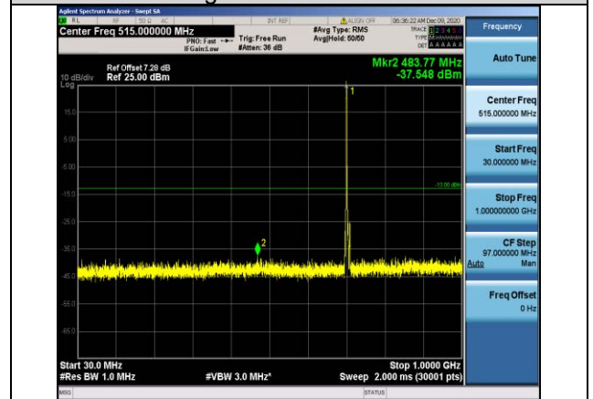
Band17-5MHz-16QAM-23790-1RB#0- Range1:30~1000MHz
