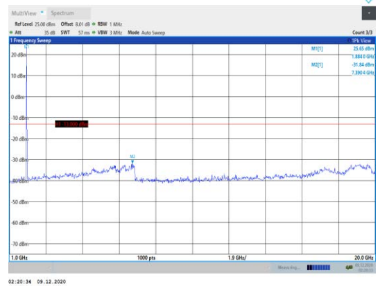
Band2-10MHz-16QAM-18900-1RB#0- Range2:1000~20000MHz
