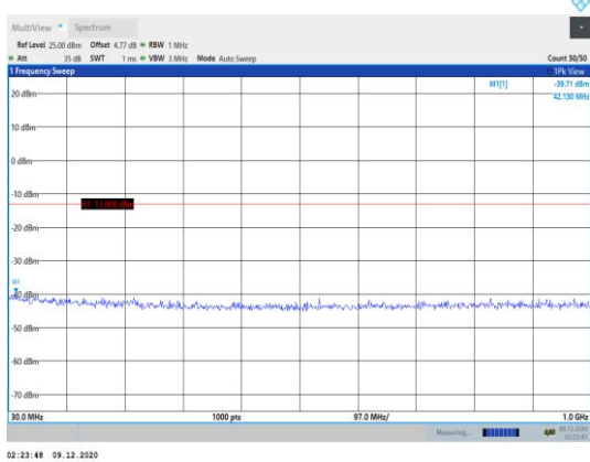
Band2-15MHz-16QAM-18675-1RB#0- Range1:30~1000MHz
