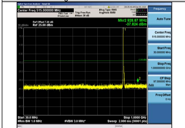
Band26-5MHz-16QAM-26715-1RB#0- Range1:30~1000MHz
