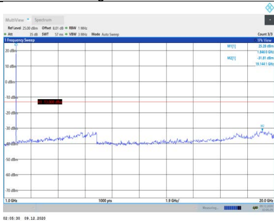
Band2-1.4MHz-QPSK-18607-1RB#0- Range2:1000~20000MHz
