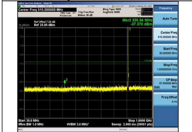
Band26-3MHz-QPSK-26705-1RB#0- Range1:30~1000MHz
