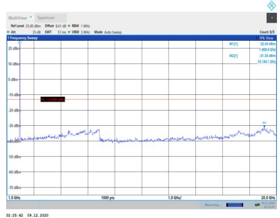
Band2-15MHz-16QAM-19125-1RB#0- Range2:1000~20000MHz
