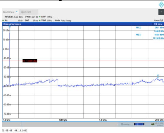
Band2-1.4MHz-16QAM-18607-1RB#0- Range2:1000~20000MHz
