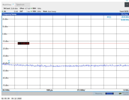
Band2-1.4MHz-16QAM-18607-1RB#0- Range1:30~1000MHz
