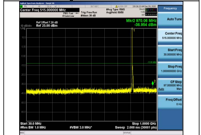
Band26-5MHz-QPSK-26740-1RB#0- Range1:30~1000MHz
