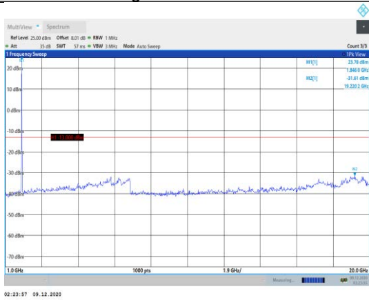
Band2-15MHz-16QAM-18675-1RB#0- Range2:1000~20000MHz
