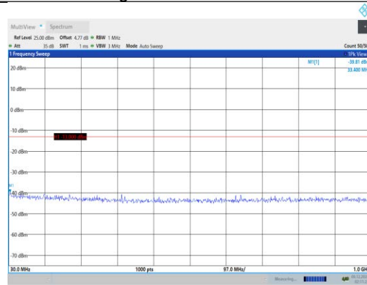
Band2-3MHz-QPSK-19185-1RB#0- Range1:30~1000MHz
