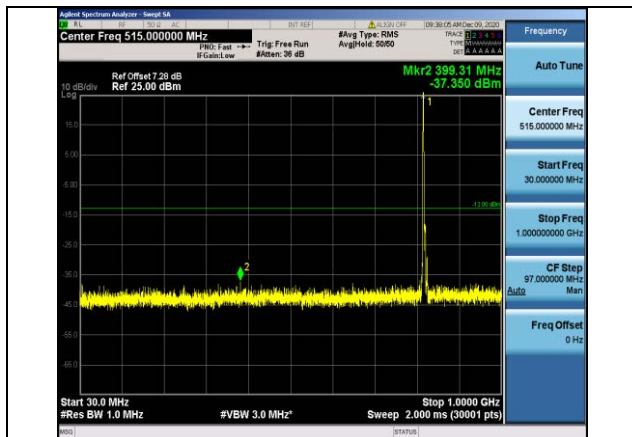
Band26-5MHz-16QAM-26765-1RB#0- Range1:30~1000MHz
