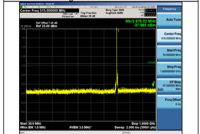
Band17-10MHz-16QAM-23790-1RB#0- Range1:30~1000MHz
