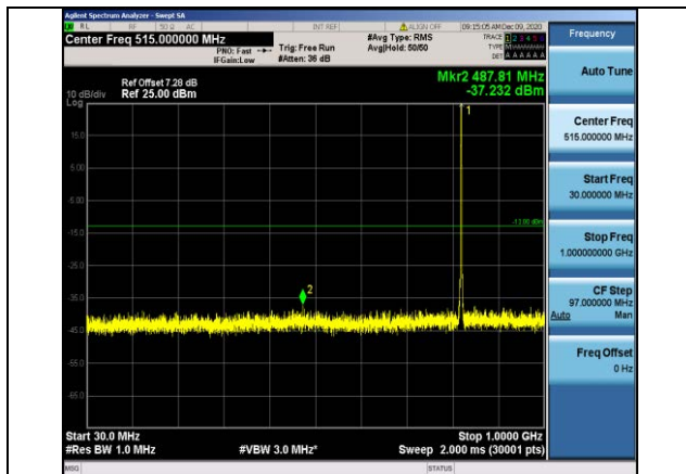
Band26-1.4MHz-QPSK-26783-1RB#0- Range1:30~1000MHz
