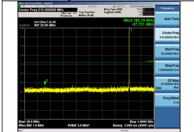
Band26-1.4MHz-QPSK-26697-1RB#0- Range1:30~1000MHz
