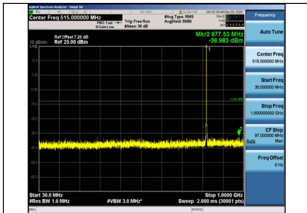
Band26-1.4MHz-16QAM-26783-1RB#0- Range1:30~1000MHz
