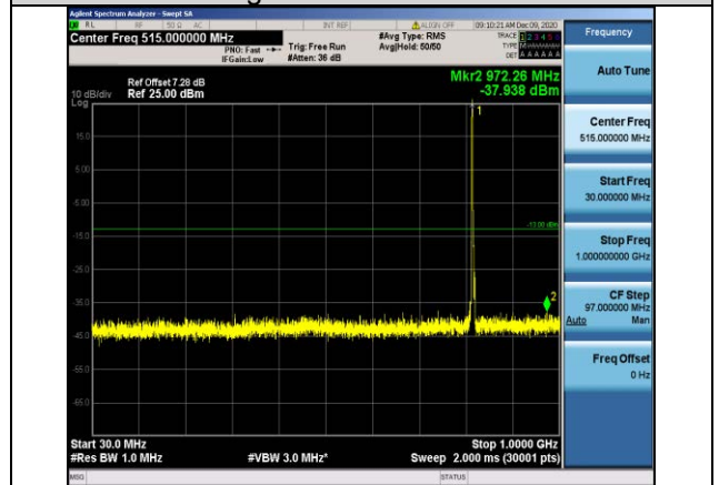
Band26-3MHz-QPSK-26740-1RB#0- Range1:30~1000MHz
