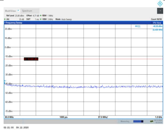
Band2-10MHz-QPSK-19150-1RB#0- Range1:30~1000MHz
