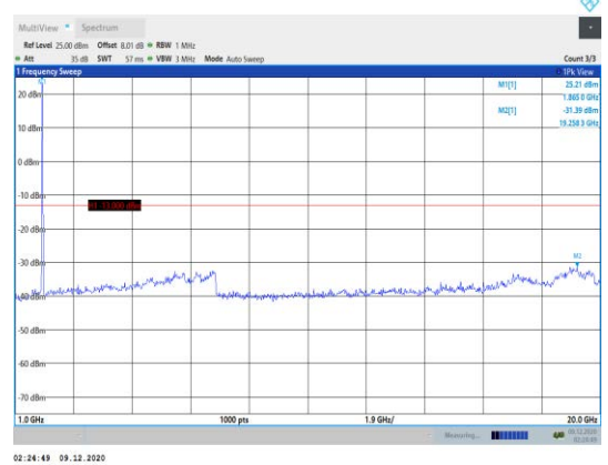
Band2-15MHz-16QAM-18900-1RB#0- Range2:1000~20000MHz
