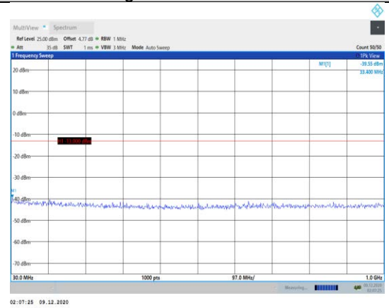
Band2-1.4MHz-16QAM-19193-1RB#0- Range1:30~1000MHz
