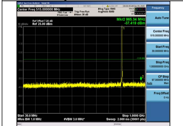
Band26-3MHz-16QAM-26705-1RB#0- Range1:30~1000MHz
