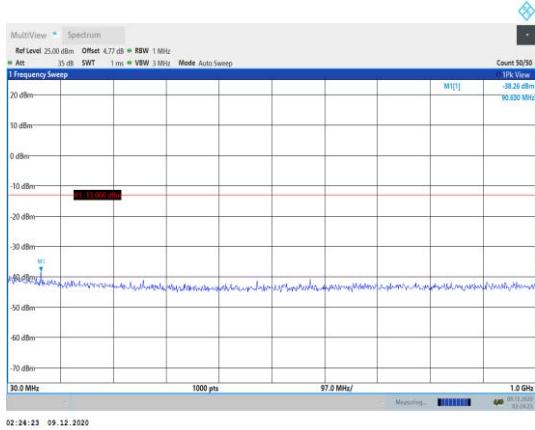
Band2-15MHz-QPSK-18900-1RB#0- Range1:30~1000MHz
