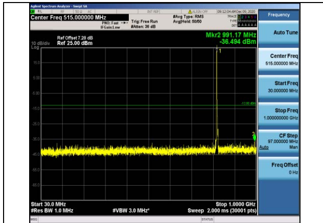
Band26-3MHz-16QAM-26775-1RB#0- Range1:30~1000MHz
