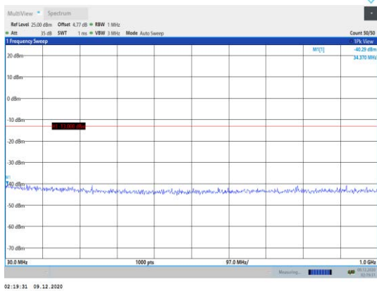
Band2-10MHz-16QAM-18650-1RB#0- Range1:30~1000MHz
