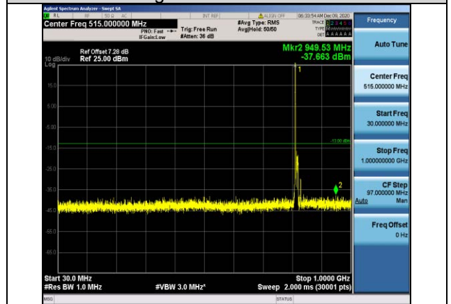
Band26-10MHz-16QAM-26740-1RB#0- Range1:30~1000MHz
