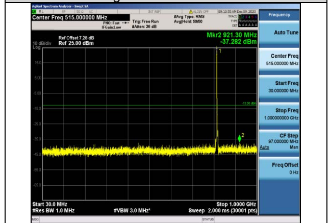
Band26-3MHz-16QAM-26740-1RB#0- Range1:30~1000MHz
