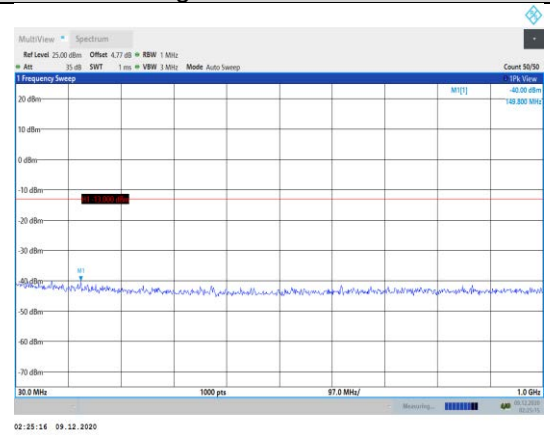
Band2-15MHz-QPSK-19125-1RB#0- Range1:30~1000MHz
