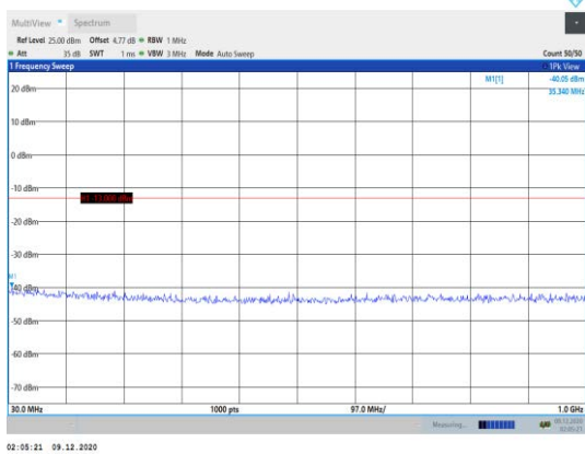
Band2-1.4MHz-QPSK-18607-1RB#0- Range1:30~1000MHz
