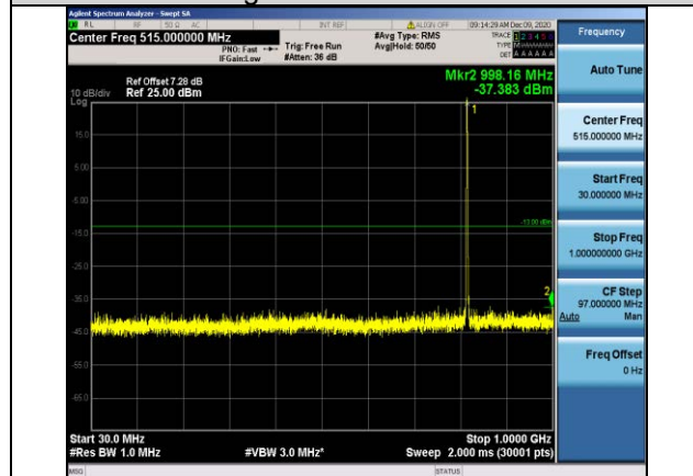
Band26-1.4MHz-16QAM-26740-1RB#0- Range1:30~1000MHz
