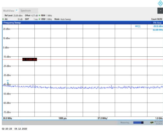
Band2-10MHz-16QAM-18900-1RB#0- Range1:30~1000MHz
