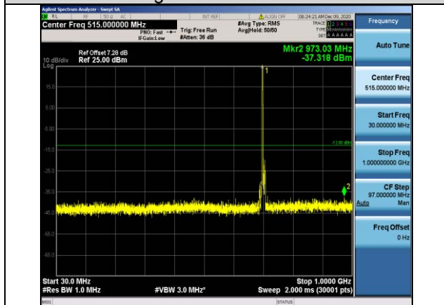
Band17-10MHz-16QAM-23780-1RB#0- Range1:30~1000MHz
