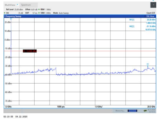
Band2-3MHz-16QAM-18900-1RB#0- Range2:1000~20000MHz
