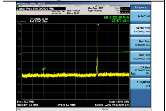
Band17-5MHz-QPSK-23790-1RB#0- Range1:30~1000MHz
