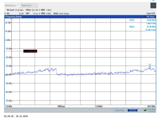
Band2-15MHz-QPSK-18900-1RB#0- Range2:1000~20000MHz
