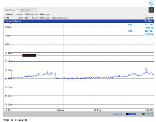
Band2-3MHz-16QAM-19185-1RB#0- Range2:1000~20000MHz
