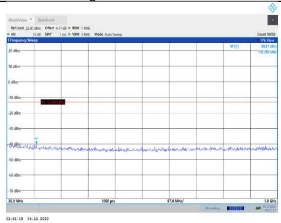
Band2-10MHz-16QAM-19150-1RB#0- Range1:30~1000MHz
