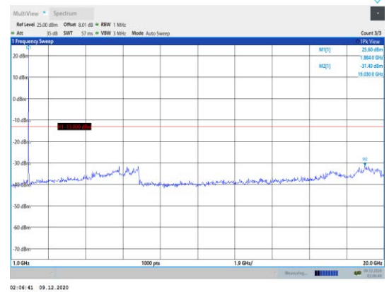
Band2-1.4MHz-16QAM-18900-1RB#0- Range2:1000~20000MHz
