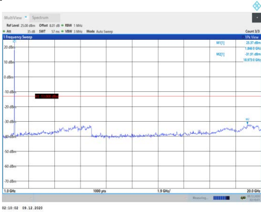
Band2-3MHz-16QAM-18615-1RB#0- Range2:1000~20000MHz
