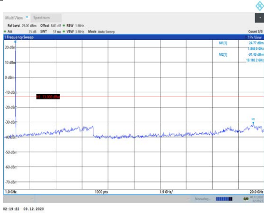
Band2-10MHz-QPSK-18650-1RB#0- Range2:1000~20000MHz
