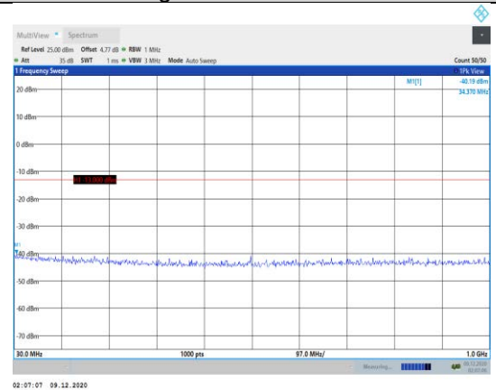
Band2-1.4MHz-QPSK-19193-1RB#0- Range1:30~1000MHz
