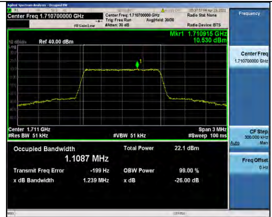
Band4-1.4MHz-16QAM-19957-6RB#0-1.1087
