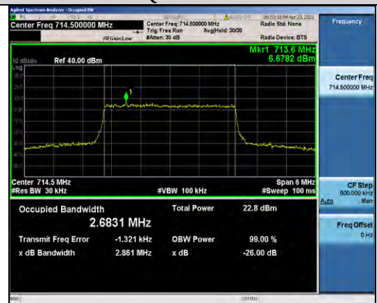
Band12-3MHz-16QAM-23165-15RB#0-2.6831
