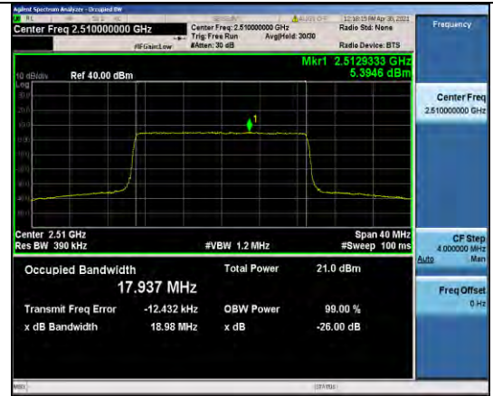
Band7-20MHz-16QAM-20850-100RB#0-17.937
