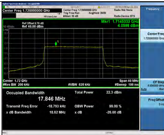
Band4-20MHz-QPSK-20050-100RB#0-17.846
