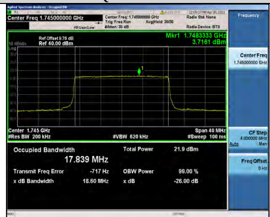
Band4-20MHz-16QAM-20300-100RB#0-17.839
