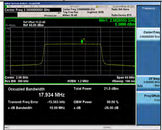
Band7-20MHz-16QAM-21350-100RB#0-17.934
