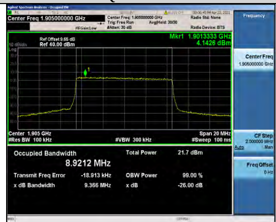
Band2-10MHz-16QAM-19150-50RB#0-8.9212
