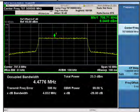
Band12-5MHz-16QAM-23095-25RB#0-4.4776
