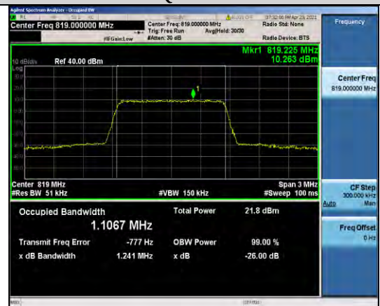
Band26-1.4MHz-16QAM-26740-6RB#0-1.1067
