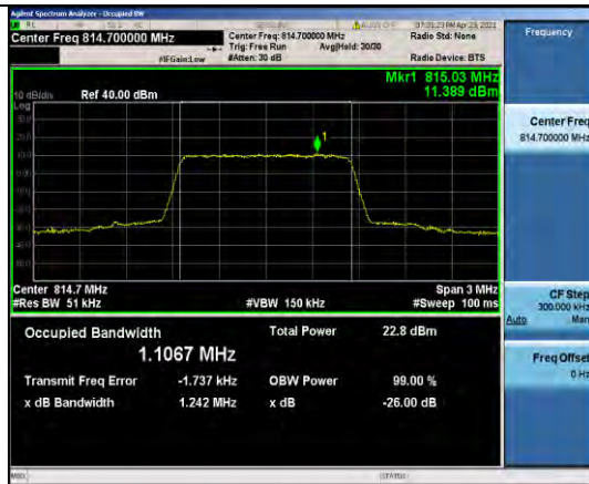
Band26-1.4MHz-QPSK-26697-6RB#0-1.1067
