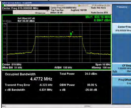
Band26-5MHz-QPSK-26740-25RB#0-4.4772
