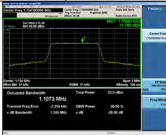
Band4-1.4MHz-QPSK-20393-6RB#0-1.1073
