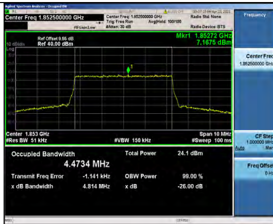
Band2-5MHz-QPSK-18625-25RB#0-4.4734
