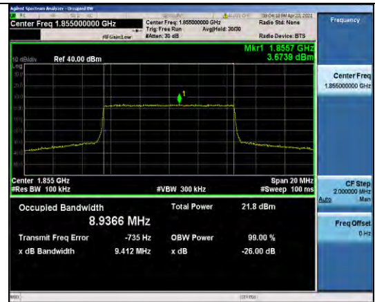
Band2-10MHz-16QAM-18650-50RB#0-8.9366
