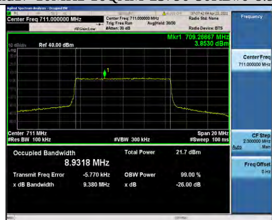
Band17-10MHz-16QAM-23800-50RB#0-8.9318
