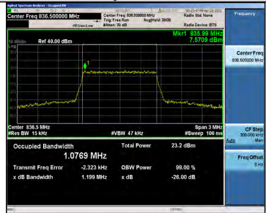
Band5-1.4MHz-16QAM-20525-6RB#0-1.0769
