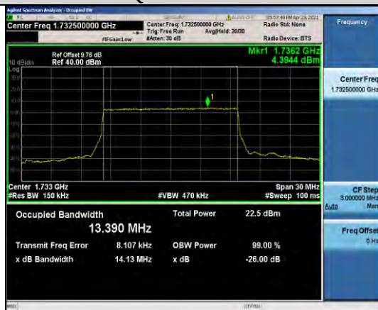
Band4-15MHz-QPSK-20175-75RB#0-13.390
