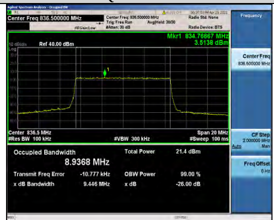
Band5-10MHz-16QAM-20525-50RB#0-8.9368
