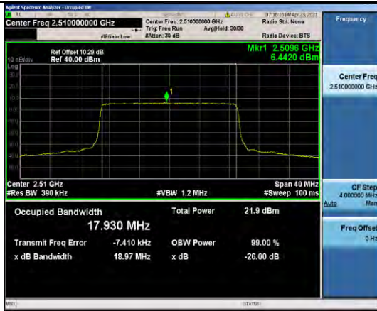
Band7-20MHz-QPSK-20850-100RB#0-17.930
