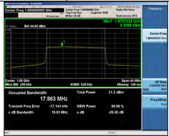
Band2-20MHz-16QAM-18900-100RB#0-17.863
