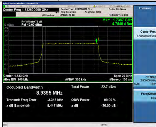
Band4-10MHz-QPSK-20175-50RB#0-8.9395
