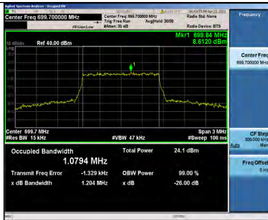
Band12-1.4MHz-QPSK-23017-6RB#0-1.0794
