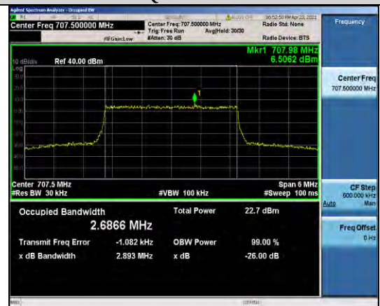
Band12-3MHz-16QAM-23095-15RB#0-2.6866
