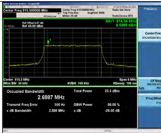
Band26-3MHz-QPSK-26705-15RB#0-2.6887
