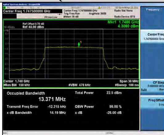
Band4-15MHz-QPSK-20325-75RB#0-13.371
