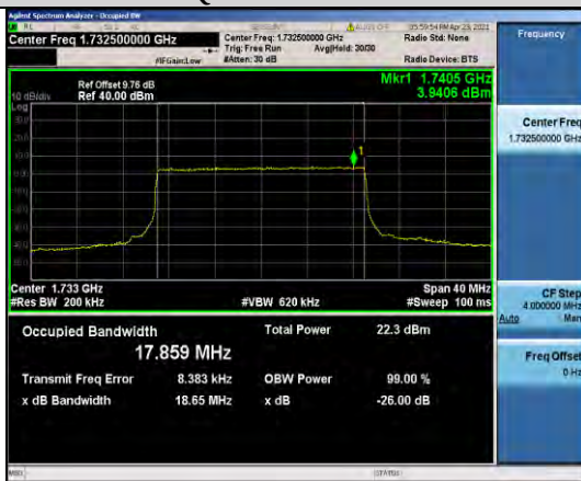
Band4-20MHz-QPSK-20175-100RB#0-17.859
