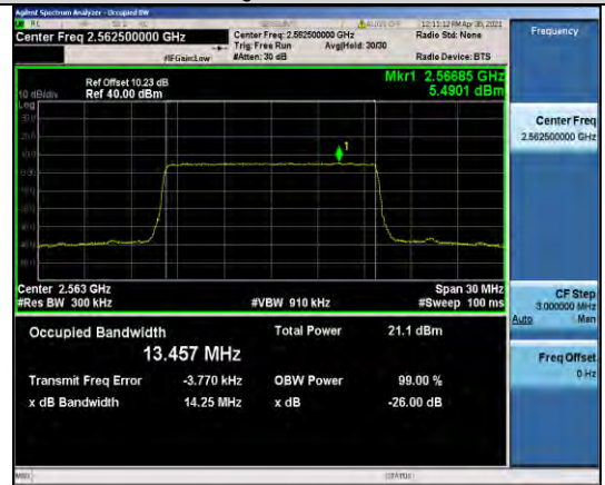
Band7-15MHz-16QAM-21375-75RB#0-13.457
