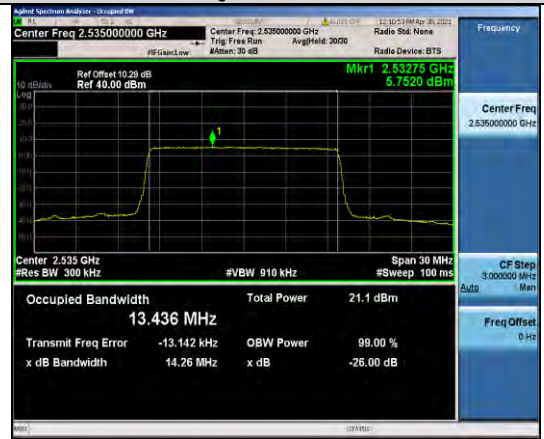
Band7-15MHz-16QAM-21100-75RB#0-13.436
