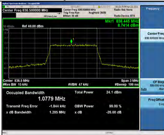
Band5-1.4MHz-QPSK-20525-6RB#0-1.0779
