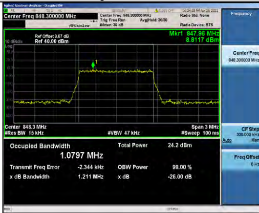
Band5-1.4MHz-QPSK-20643-6RB#0-1.0797
