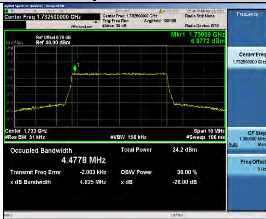
Band4-5MHz-QPSK-20175-25RB#0-4.4778
