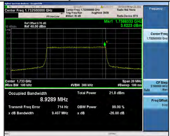
Band4-10MHz-16QAM-20175-50RB#0-8.9289
