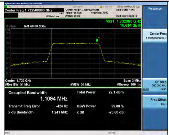
Band4-1.4MHz-16QAM-20175-6RB#0-1.1094
