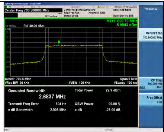
Band12-3MHz-16QAM-23025-15RB#0-2.6837
