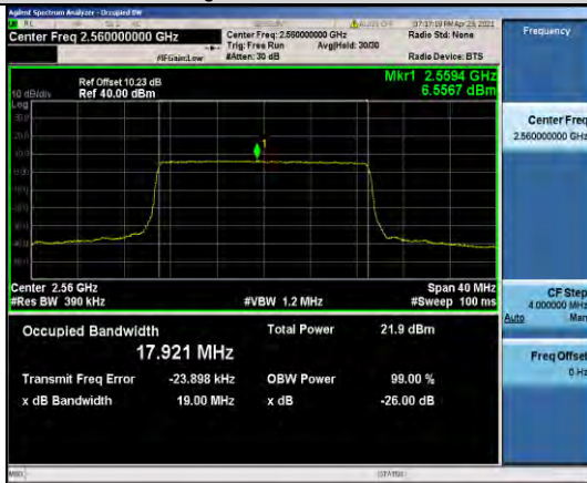
Band7-20MHz-QPSK-21350-100RB#0-17.921
