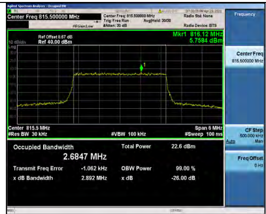
Band26-3MHz-16QAM-26705-15RB#0-2.6847
