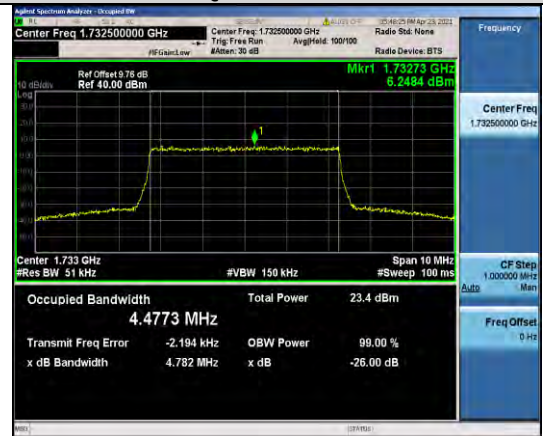
Band4-5MHz-16QAM-20175-25RB#0-4.4773
