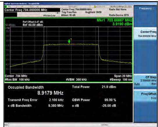
Band12-10MHz-16QAM-23060-50RB#0-8.9179
