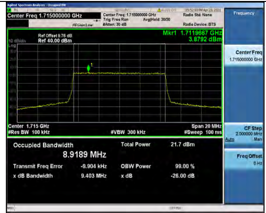
Band4-10MHz-16QAM-20000-50RB#0-8.9189
