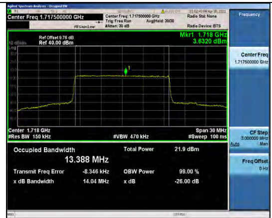
Band4-15MHz-16QAM-20025-75RB#0-13.388
