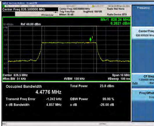
Band5-5MHz-QPSK-20425-25RB#0-4.4776
