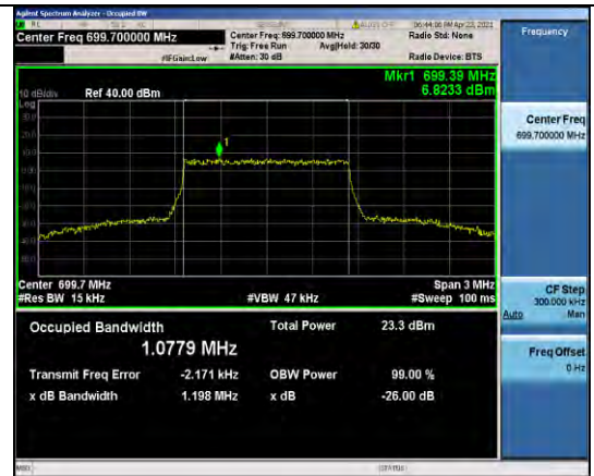
Band12-1.4MHz-16QAM-23017-6RB#0-1.0779
