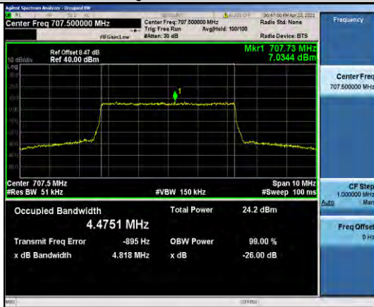
Band12-5MHz-QPSK-23095-25RB#0-4.4751
