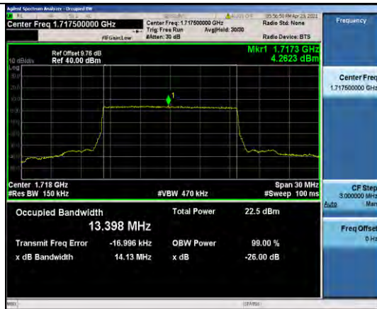
Band4-15MHz-QPSK-20025-75RB#0-13.398
