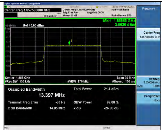
Band2-15MHz-16QAM-18675-75RB#0-13.397
