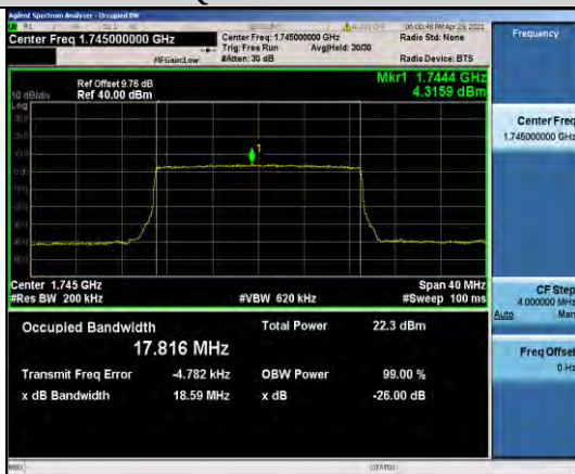
Band4-20MHz-QPSK-20300-100RB#0-17.816
