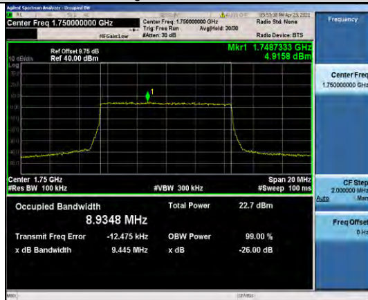
Band4-10MHz-QPSK-20350-50RB#0-8.9348
