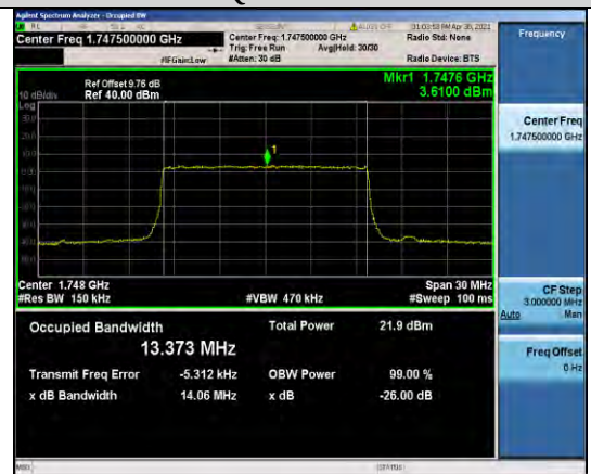
Band4-15MHz-16QAM-20325-75RB#0-13.373
