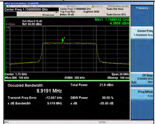
Band4-10MHz-16QAM-20350-50RB#0-8.9191
