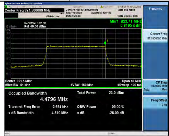
Band26-5MHz-16QAM-26765-25RB#0-4.4796
