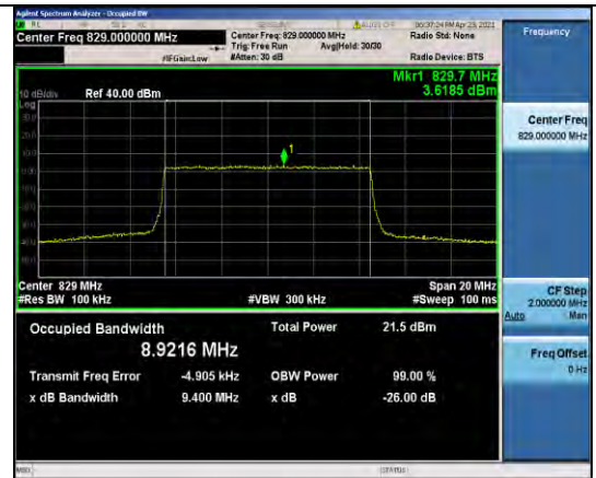
Band5-10MHz-16QAM-20450-50RB#0-8.9216
