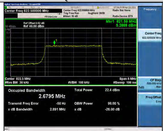
Band26-3MHz-16QAM-26775-15RB#0-2.6795
