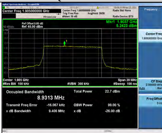
Band2-10MHz-QPSK-19150-50RB#0-8.9313
