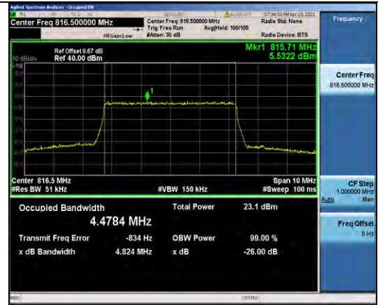
Band26-5MHz-16QAM-26715-25RB#0-4.4784
