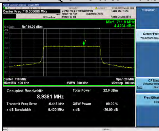
Band17-10MHz-QPSK-23790-50RB#0-8.9381
