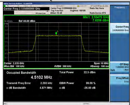
Band7-5MHz-16QAM-21100-25RB#0-4.5102
