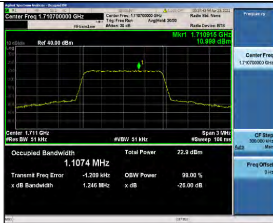
Band4-1.4MHz-QPSK-19957-6RB#0-1.1074
