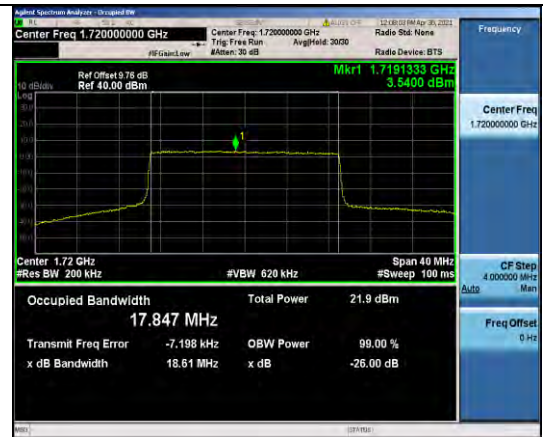
Band4-20MHz-16QAM-20050-100RB#0-17.847
