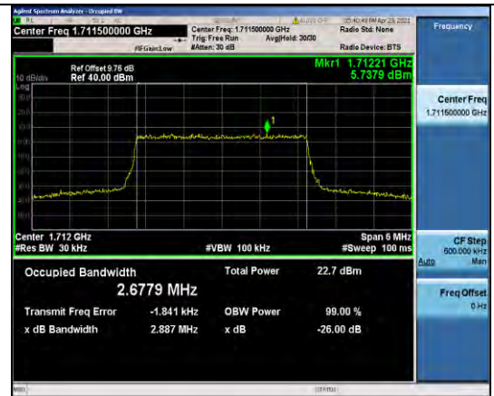
Band4-3MHz-16QAM-19965-15RB#0-2.6779
