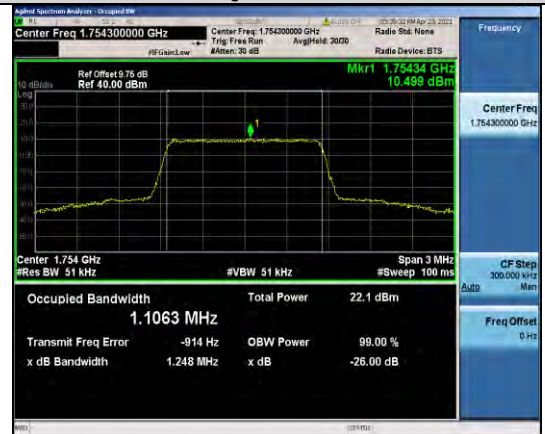
Band4-1.4MHz-16QAM-20393-6RB#0-1.1063
