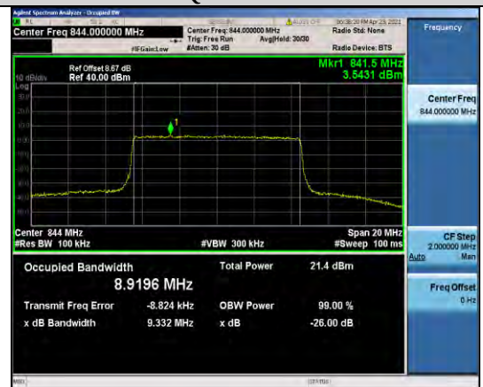
Band5-10MHz-16QAM-20600-50RB#0-8.9196
