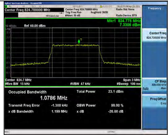
Band5-1.4MHz-16QAM-20407-6RB#0-1.0786
