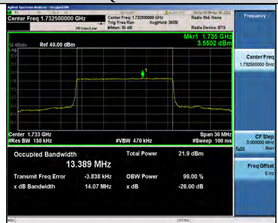
Band4-15MHz-16QAM-20175-75RB#0-13.389
