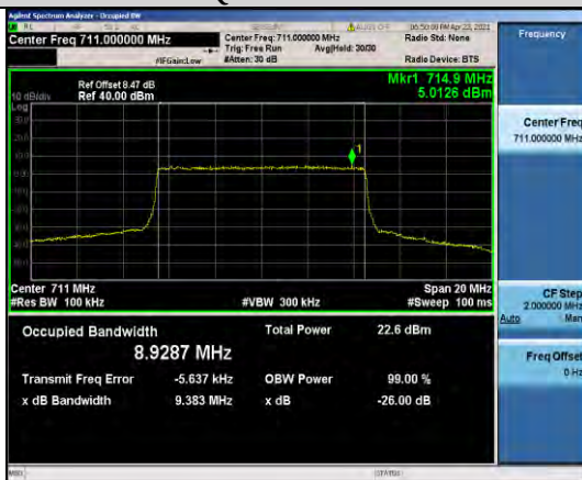
Band12-10MHz-QPSK-23130-50RB#0-8.9287
