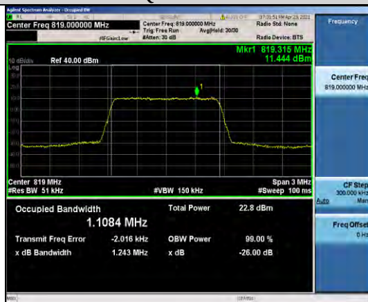
Band26-1.4MHz-QPSK-26740-6RB#0-1.1084
