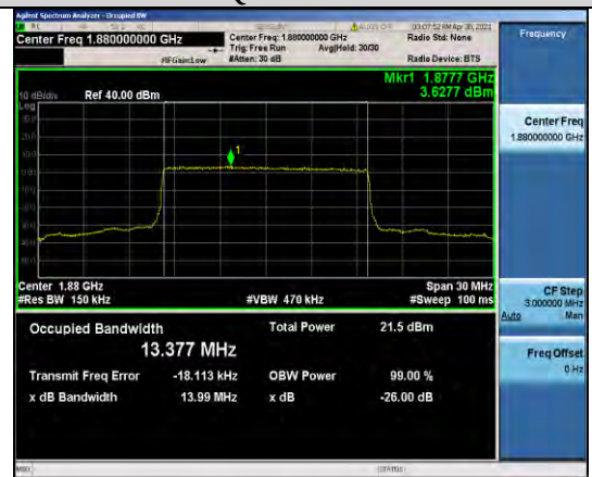
Band2-15MHz-16QAM-18900-75RB#0-13.377
