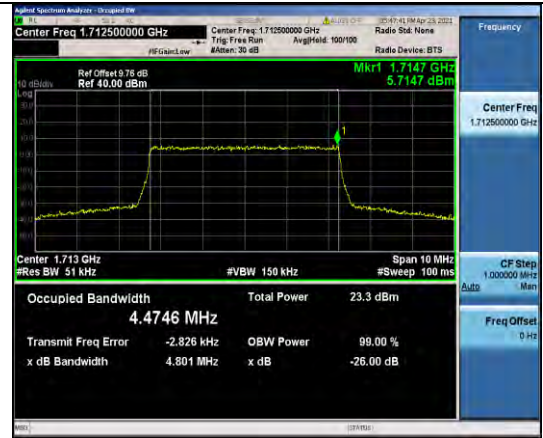
Band4-5MHz-16QAM-19975-25RB#0-4.4746
