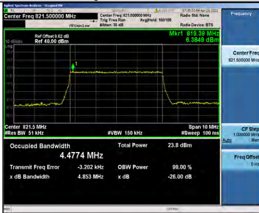
Band26-5MHz-QPSK-26765-25RB#0-4.4774
