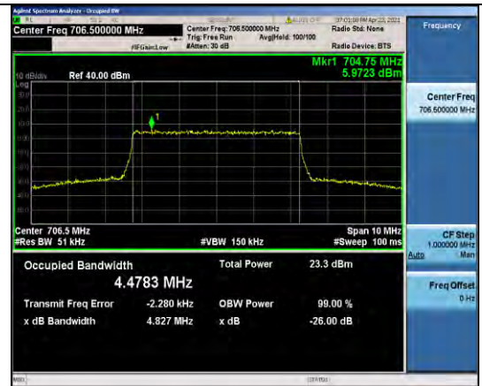
Band17-5MHz-16QAM-23755-25RB#0-4.4783
