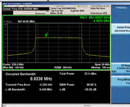
Band5-10MHz-QPSK-20525-50RB#0-8.9236
