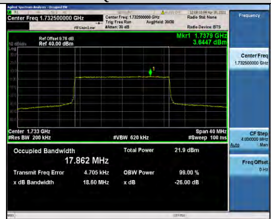
Band4-20MHz-16QAM-20175-100RB#0-17.862
