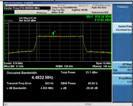
Band26-5MHz-16QAM-26740-25RB#0-4.4832
