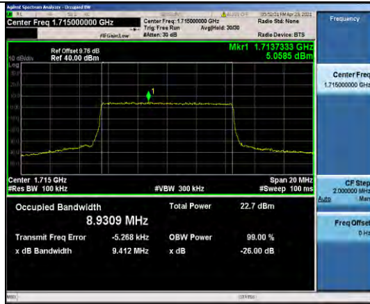
Band4-10MHz-QPSK-20000-50RB#0-8.9309
