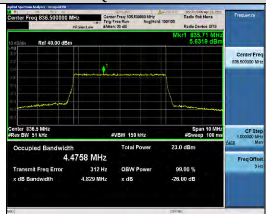
Band5-5MHz-16QAM-20525-25RB#0-4.4758
