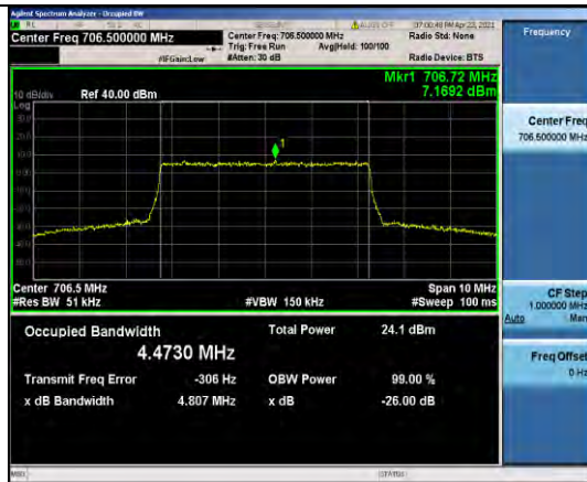
Band17-5MHz-QPSK-23755-25RB#0-4.4730
