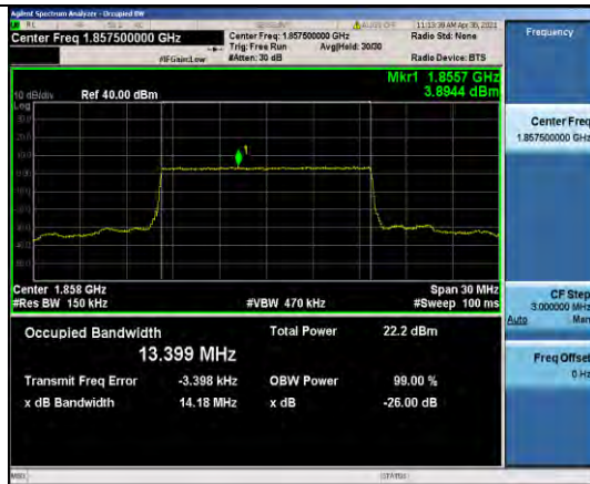
Band2-15MHz-QPSK-18675-75RB#0-13.399
