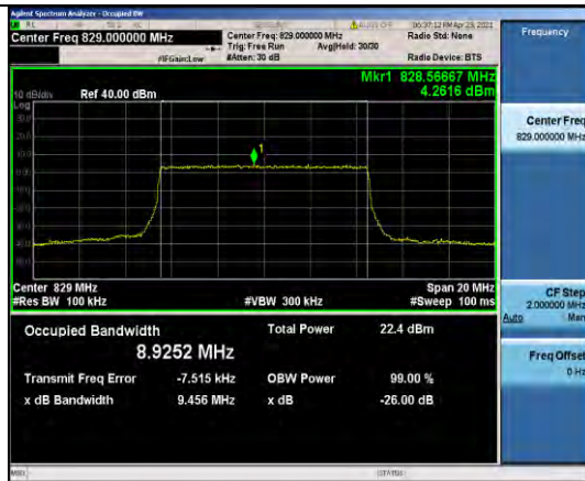
Band5-10MHz-QPSK-20450-50RB#0-8.9252
