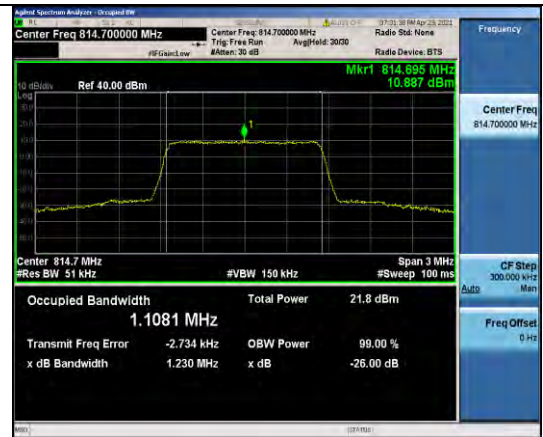
Band26-1.4MHz-16QAM-26697-6RB#0-1.1081
