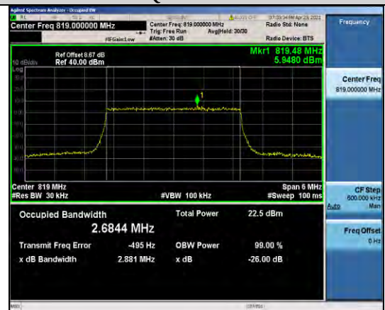
Band26-3MHz-16QAM-26740-15RB#0-2.6844
