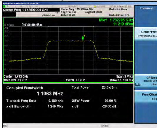
Band4-1.4MHz-QPSK-20175-6RB#0-1.1063
