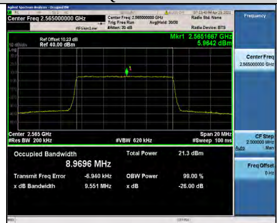
Band7-10MHz-16QAM-21400-50RB#0-8.9696
