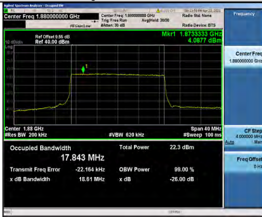
Band2-20MHz-QPSK-18900-100RB#0-17.843
