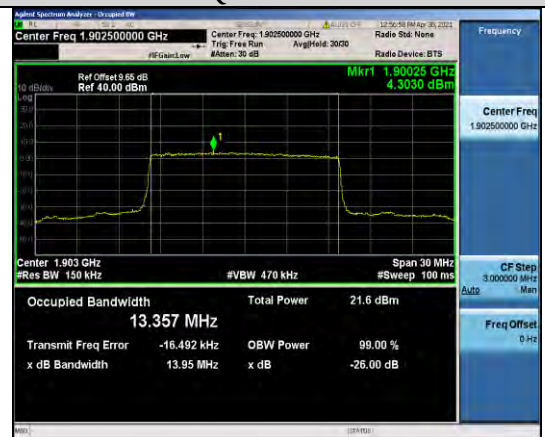
Band2-15MHz-16QAM-19125-75RB#0-13.357
