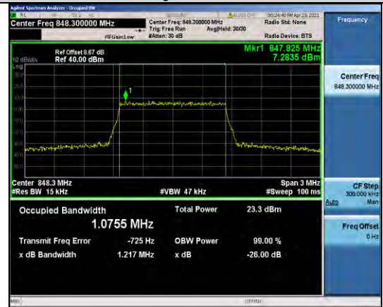
Band5-1.4MHz-16QAM-20643-6RB#0-1.0755
