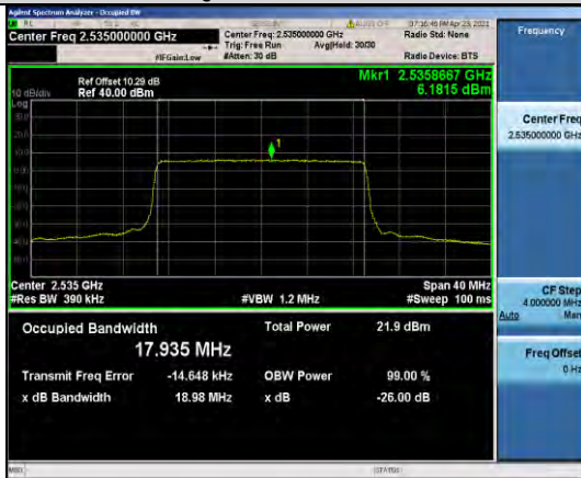
Band7-20MHz-QPSK-21100-100RB#0-17.935
