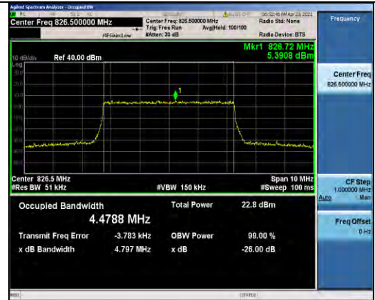
Band5-5MHz-16QAM-20425-25RB#0-4.4788
