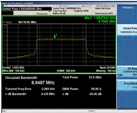
Band2-10MHz-QPSK-18650-50RB#0-8.9457
