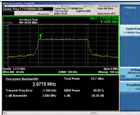
Band4-3MHz-QPSK-19965-15RB#0-2.6779
