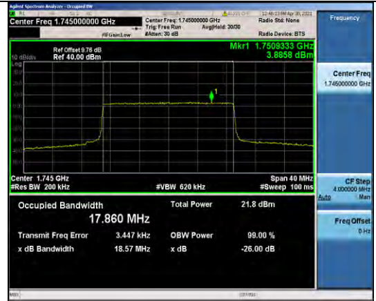
Band66-20MHz-16QAM-132322-100RB#0-17.860
