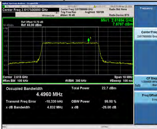
Band38-5MHz-16QAM-38225-25RB#0-4.4960
