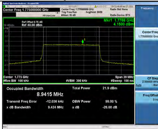
Band66-10MHz-16QAM-132622-50RB#0-8.9415
