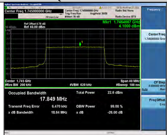
Band66-20MHz-QPSK-132322-100RB#0-17.849
