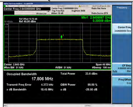
Band41-20MHz-QPSK-41140-100RB#0-17.806
