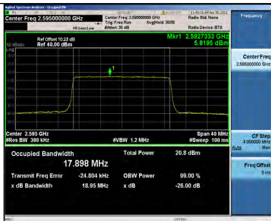
Band38-20MHz-16QAM-38000-100RB#0-17.898
