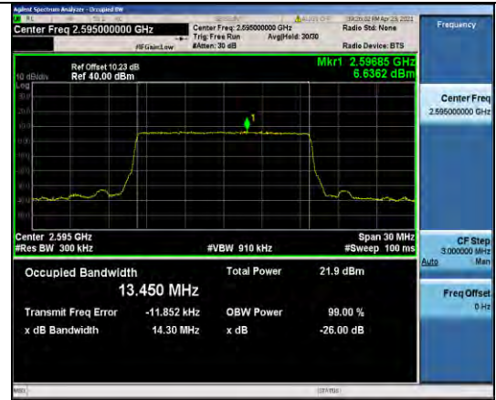
Band38-15MHz-QPSK-38000-75RB#0-13.450
