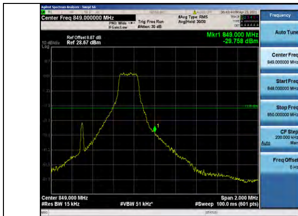
Band5-1.4MHz-16QAM-20643-1RB#5
