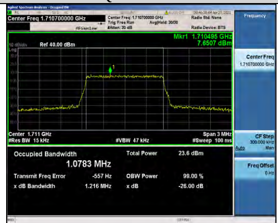
Band66-1.4MHz-16QAM-131979-6RB#0-1.0783
