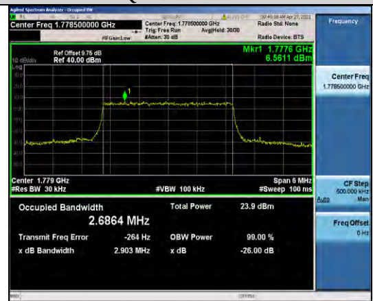
Band66-3MHz-QPSK-132657-15RB#0-2.6864
