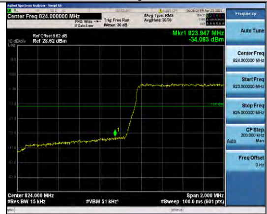
Band5-1.4MHz-16QAM-20407-6RB#0
