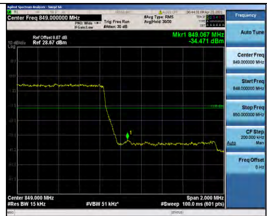
Band5-1.4MHz-QPSK-20643-6RB#0
