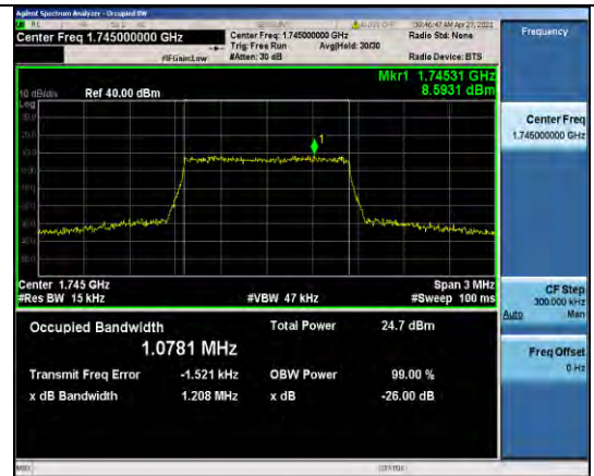
Band66-1.4MHz-QPSK-132322-6RB#0-1.0781
