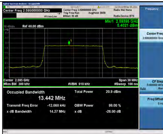
Band38-15MHz-16QAM-38000-75RB#0-13.442
