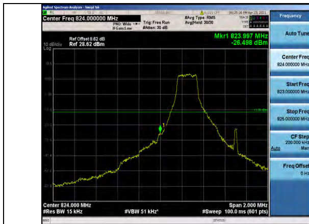
Band5-1.4MHz-QPSK-20407-1RB#0
