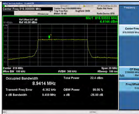
Band26-10MHz-QPSK-26740-50RB#0-8.9414
