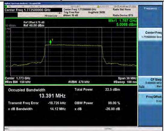
Band66-15MHz-QPSK-132597-75RB#0-13.391
