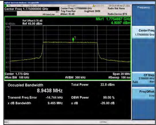
Band66-10MHz-QPSK-132622-50RB#0-8.9438
