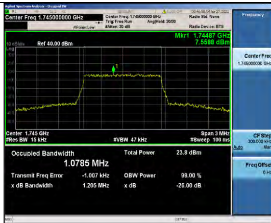
Band66-1.4MHz-16QAM-132322-6RB#0-1.0785
