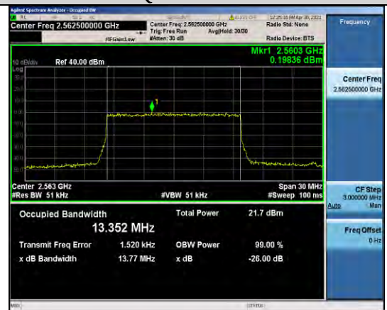
Band41-15MHz-16QAM-40315-75RB#0-13.352
