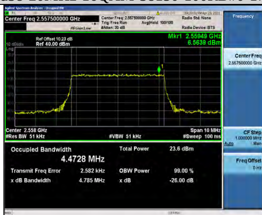
Band41-5MHz-QPSK-40265-25RB#0-4.4728
