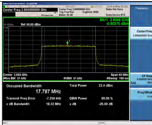
Band41-20MHz-16QAM-40740-100RB#0-17.787
