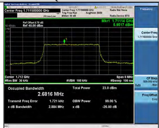
Band66-3MHz-16QAM-131987-15RB#0-2.6816
