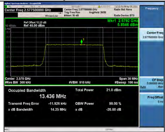
Band38-15MHz-16QAM-37825-75RB#0-13.436
