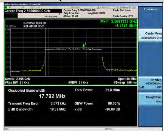
Band41-20MHz-16QAM-40340-100RB#0-17.782
