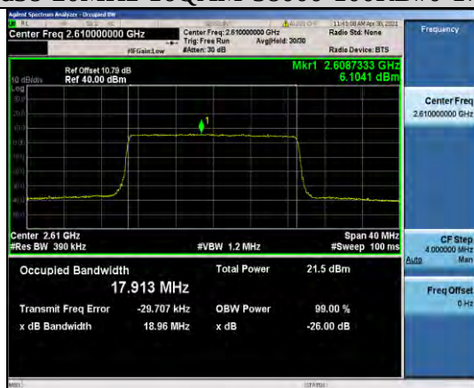
Band38-20MHz-16QAM-38150-100RB#0-17.913
