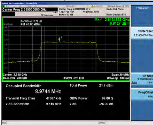
Band38-10MHz-16QAM-38200-50RB#0-8.9744
