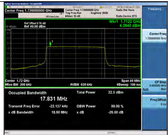
Band66-20MHz-QPSK-132072-100RB#0-17.831
