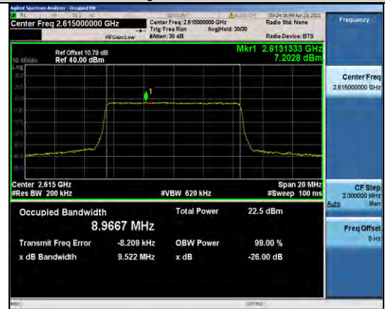
Band38-10MHz-QPSK-38200-50RB#0-8.9667
