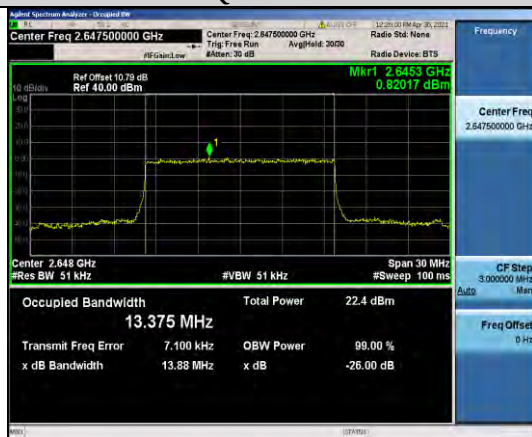
Band41-15MHz-16QAM-41165-75RB#0-13.375
