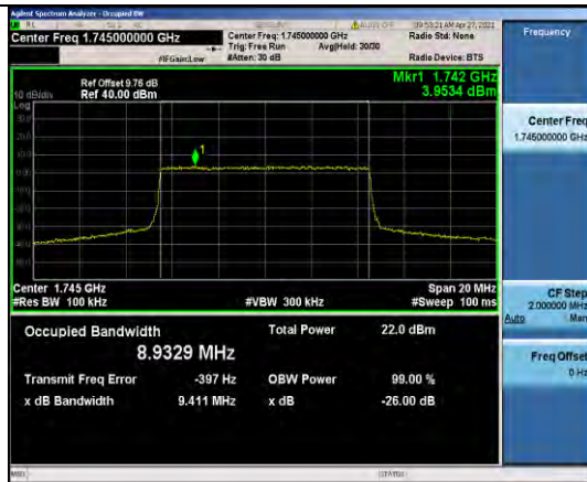
Band66-10MHz-16QAM-132322-50RB#0-8.9329
