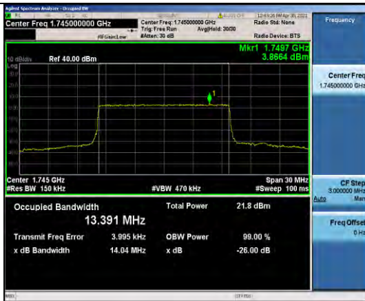
Band66-15MHz-16QAM-132322-75RB#0-13.391
