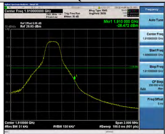
Band2-5MHz-16QAM-18625-25RB#0
