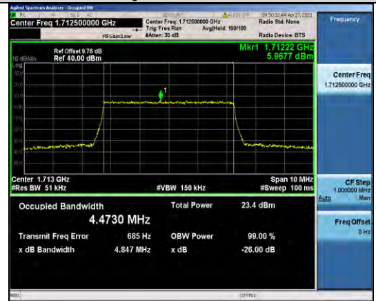
Band66-5MHz-16QAM-131997-25RB#0-4.4730
