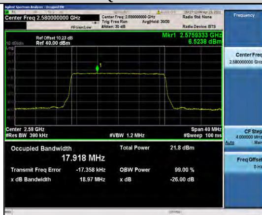
Band38-20MHz-QPSK-37850-100RB#0-17.918
