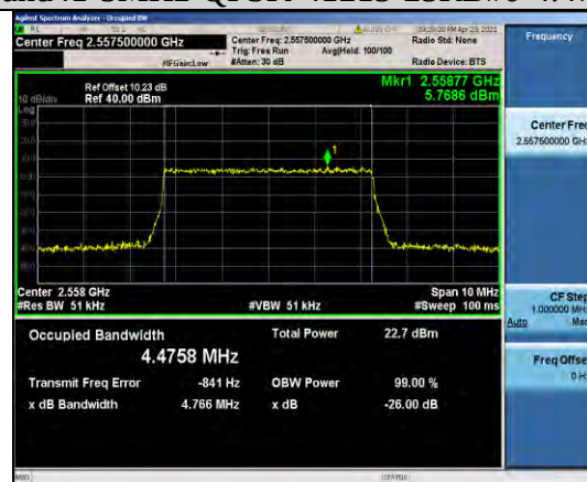
Band41-5MHz-16QAM-40265-25RB#0-4.4758
