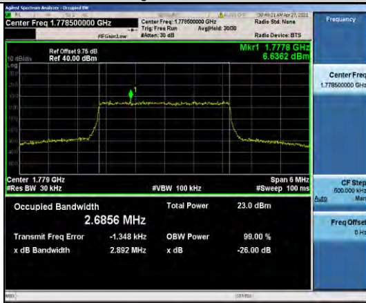
Band66-3MHz-16QAM-132657-15RB#0-2.6856
