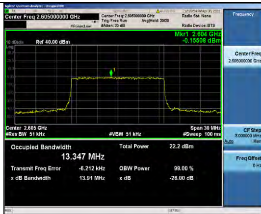
Band41-15MHz-16QAM-40740-75RB#0-13.347
