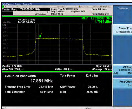
Band66-20MHz-QPSK-132572-100RB#0-17.851
