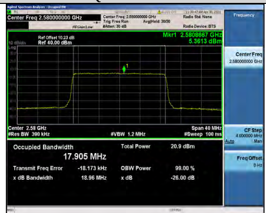
Band38-20MHz-16QAM-37850-100RB#0-17.905
