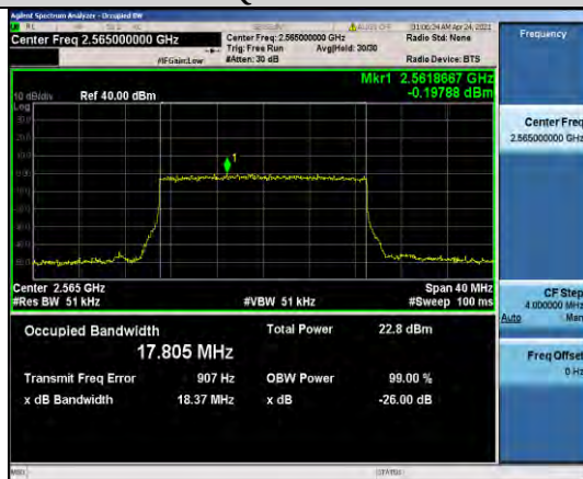
Band41-20MHz-QPSK-40340-100RB#0-17.805
