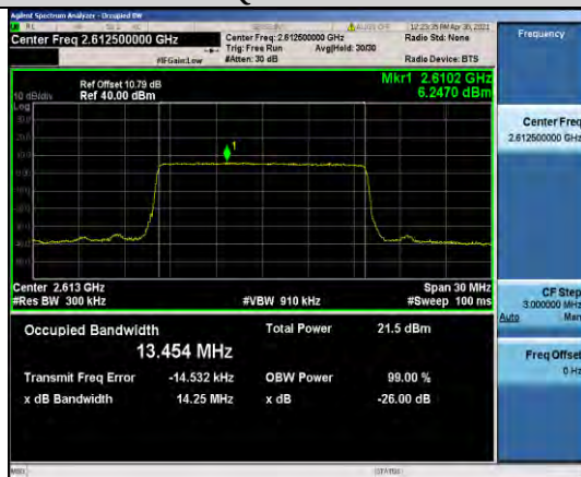
Band38-15MHz-16QAM-38175-75RB#0-13.454
