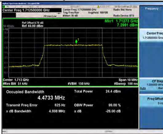
Band66-5MHz-QPSK-131997-25RB#0-4.4733
