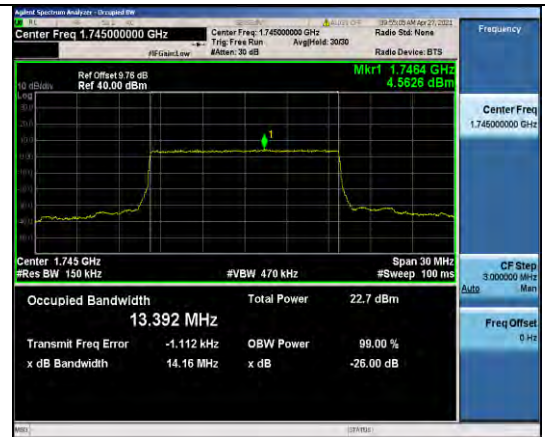
Band66-15MHz-QPSK-132322-75RB#0-13.392
