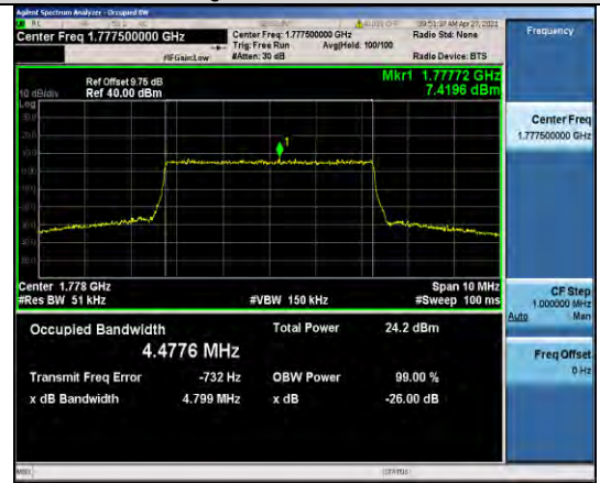
Band66-5MHz-QPSK-132647-25RB#0-4.4776
