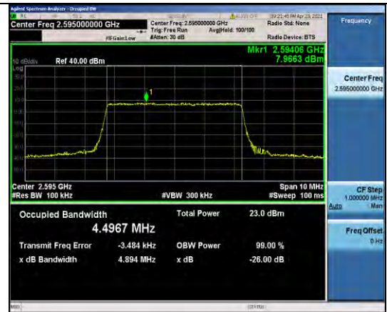
Band38-5MHz-QPSK-38000-25RB#0-4.4967
