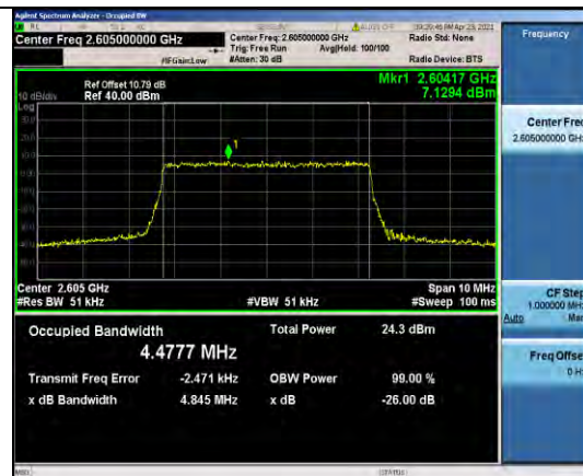
Band41-5MHz-QPSK-40740-25RB#0-4.4777
