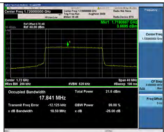
Band66-20MHz-16QAM-132072-100RB#0-17.841
