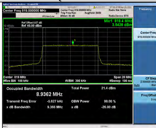
Band26-10MHz-16QAM-26740-50RB#0-8.9362
