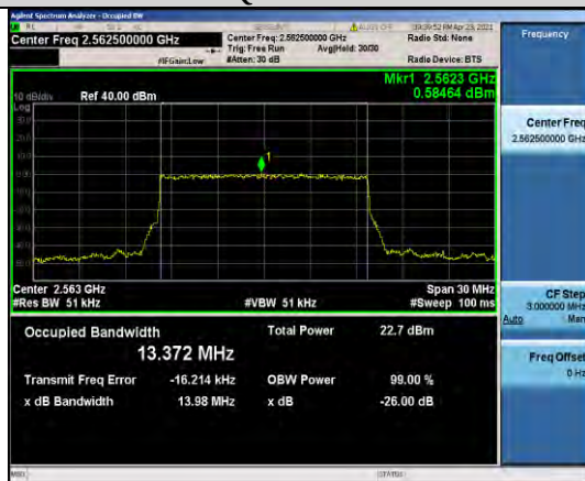
Band41-15MHz-QPSK-40315-75RB#0-13.372
