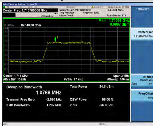
Band66-1.4MHz-QPSK-131979-6RB#0-1.0768
