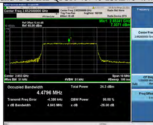
Band41-5MHz-QPSK-41215-25RB#0-4.4796
