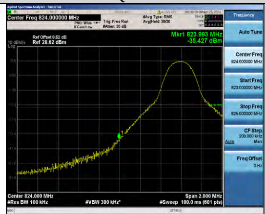
Band5-10MHz-16QAM-20450-1RB#0
