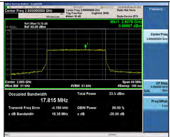
Band41-20MHz-QPSK-40740-100RB#0-17.815
