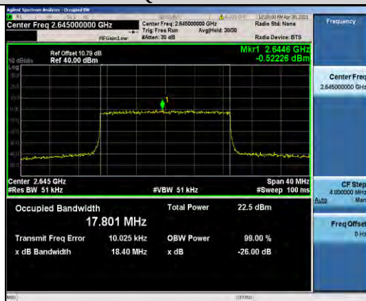
Band41-20MHz-16QAM-41140-100RB#0-17.801
