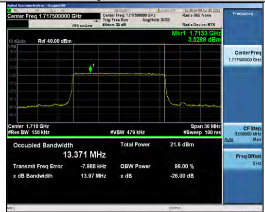
Band66-15MHz-16QAM-132047-75RB#0-13.371
