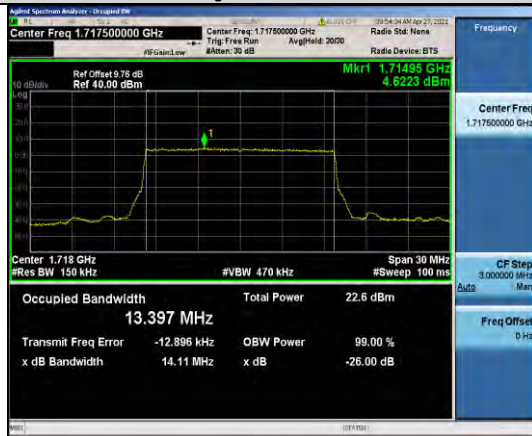
Band66-15MHz-QPSK-132047-75RB#0-13.397
