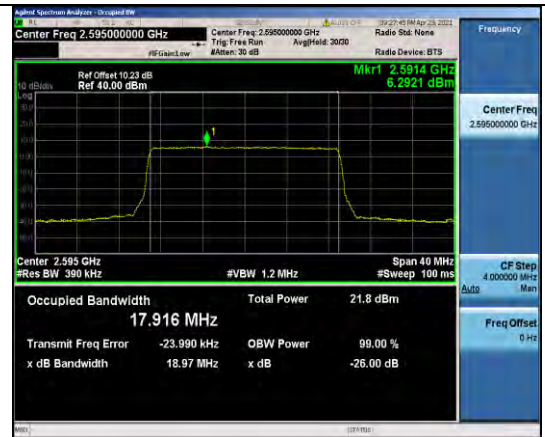
Band38-20MHz-QPSK-38000-100RB#0-17.916
