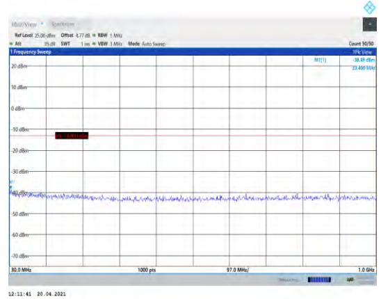
Band4-3MHz-16QAM-20385-1RB#0- Range1:30~1000MHz
