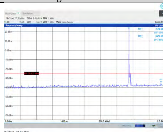
Band7-20MHz-16QAM-21350-1RB#0- Range2:1000~3000MHz
