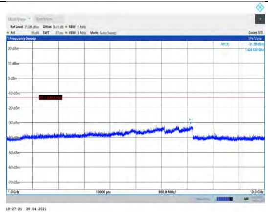
Band5-1.4MHz-16QAM-20525-1RB#0- Range2:1000~10000MHz
