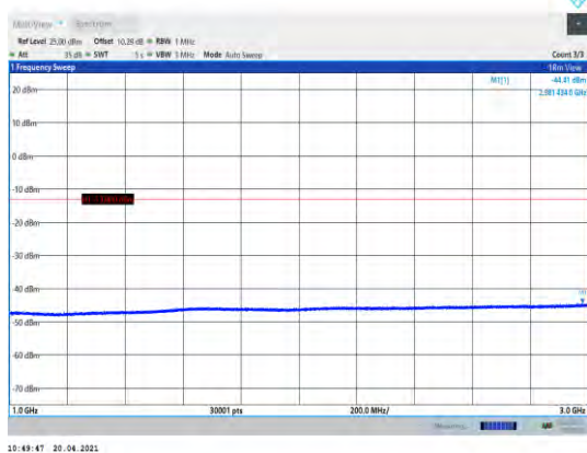
Band5-4132-1000~3000MHz
