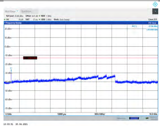
Band12-1.4MHz-QPSK-23095-1RB#0- Range2:1000~10000MHz
