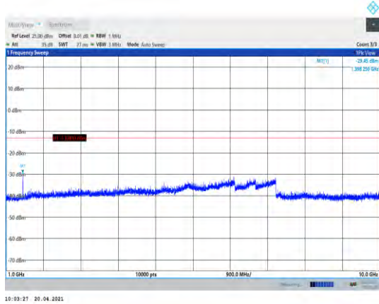
Band12-1.4MHz-16QAM-23017-1RB#0- Range2:1000~10000MHz
