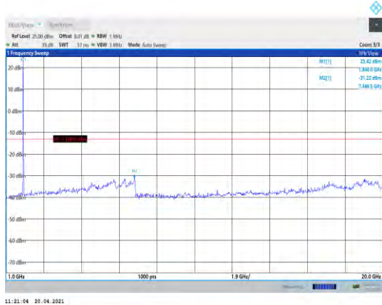
Band2-15MHz-16QAM-18675-1RB#0- Range2:1000~20000MHz
