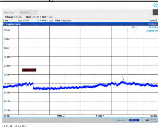
Band7-15MHz-16QAM-21100-1RB#0-Range3:3000~26000MHz
