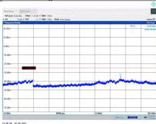
Band7-20MHz-16QAM-21100-1RB#0- Range3:3000~26000MHz
