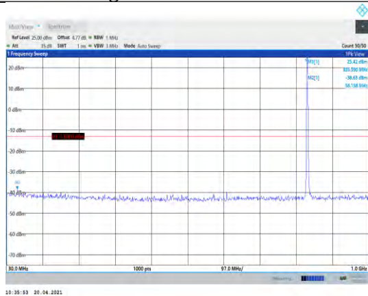
Band5-3MHz-16QAM-20525-1RB#0-Range1:30~1000MHz
