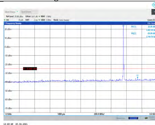
Band7-10MHz-16QAM-21400-1RB#0-Range2:1000~3000MHz
