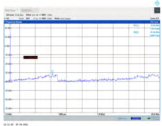
Band4-3MHz-16QAM-20385-1RB#0- Range2:1000~20000MHz
