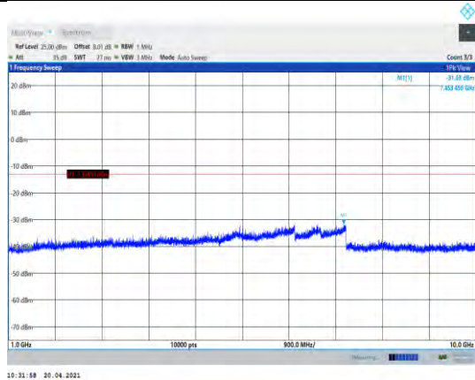
Band5-10MHz-QPSK-20450-1RB#0-Range2:1000~10000MHz
