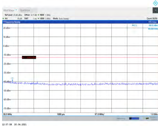
Band4-5MHz-16QAM-20175-1RB#0- Range1:30~1000MHz
