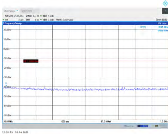
Band4-3MHz-16QAM-20175-1RB#0- Range1:30~1000MHz
