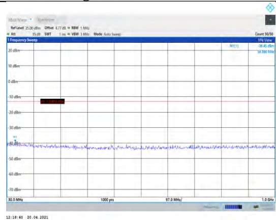
Band4-1.4MHz-16QAM-20393-1RB#0- Range1:30~1000MHz
