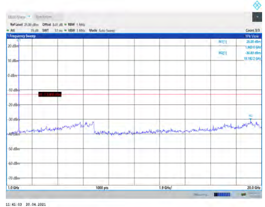
Band2-10MHz-16QAM-19150-1RB#0- Range2:1000~20000MHz
