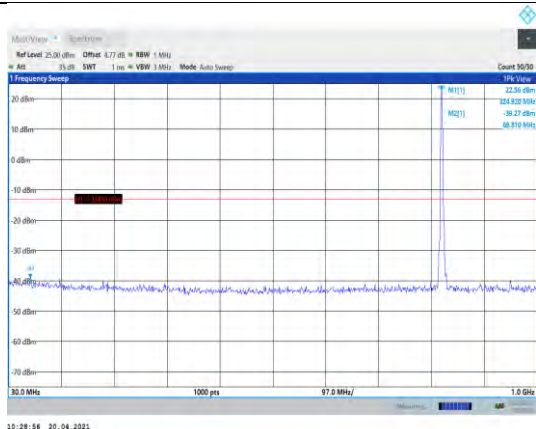
Band5-5MHz-QPSK-20425-1RB#0- Range1:30~1000MHz
