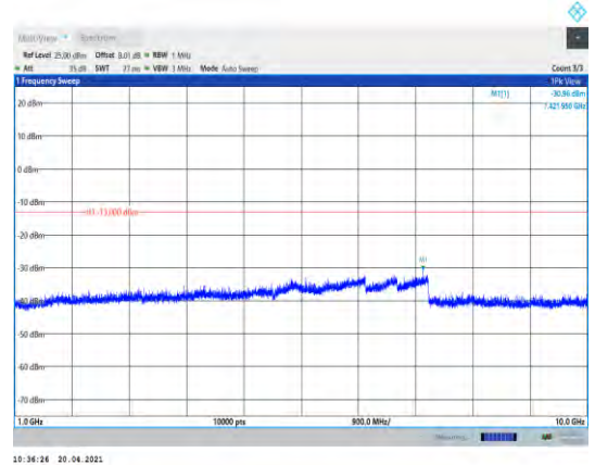
Band5-3MHz-QPSK-20635-1RB#0- Range2:1000~10000MHz
