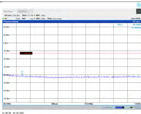
Band2-10MHz-QPSK-18650-1RB#0-Range1:30~1000MHz
