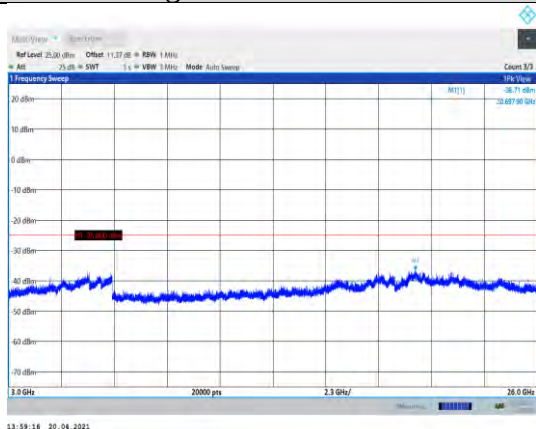
Band7-20MHz-QPSK-21350-1RB#0-Range3:3000~26000MHz
