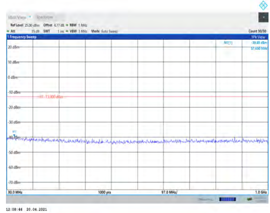
Band4-5MHz-16QAM-20375-1RB#0- Range1:30~1000MHz
