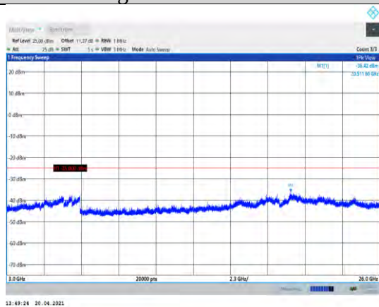
Band7-10MHz-QPSK-21400-1RB#0- Range3:3000~26000MHz
