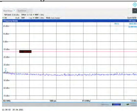
Band2-3MHz-QPSK-18900-1RB#0- Range1:30~1000MHz
