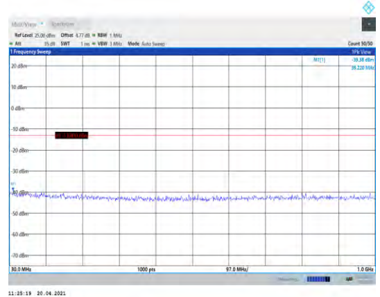
Band2-1.4MHz-16QAM-19193-1RB#0- Range1:30~1000MHz
