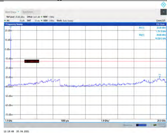
Band4-1.4MHz-16QAM-20393-1RB#0- Range2:1000~20000MHz
