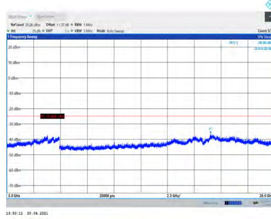
Band7-10MHz-16QAM-21400-1RB#0-Range3:3000~26000MHz
