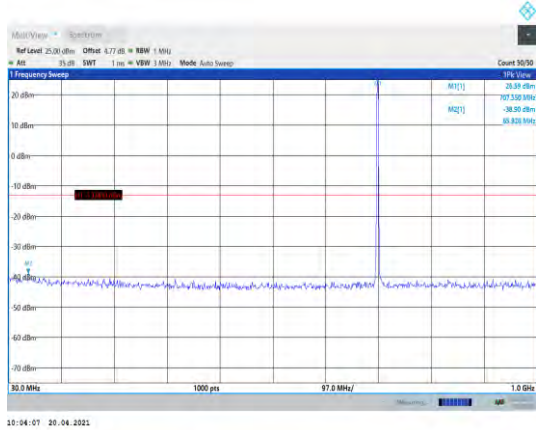
Band12-1.4MHz-16QAM-23095-1RB#0- Range1:30~1000MHz
