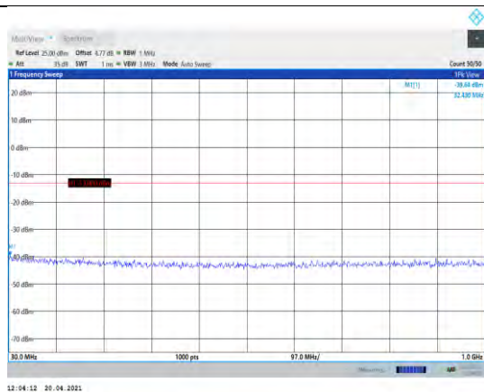
Band4-10MHz-16QAM-20000-1RB#0- Range1:30~1000MHz
