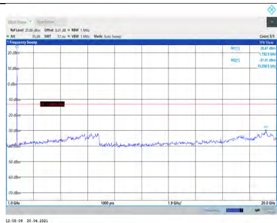
Band4-10MHz-16QAM-20175-1RB#0- Range2:1000~20000MHz
