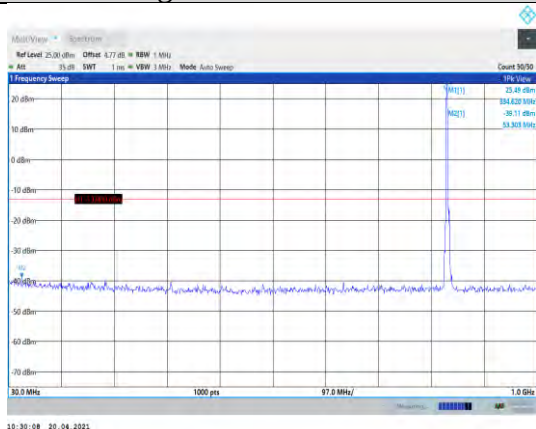
Band5-5MHz-16QAM-20525-1RB#0- Range1:30~1000MHz
