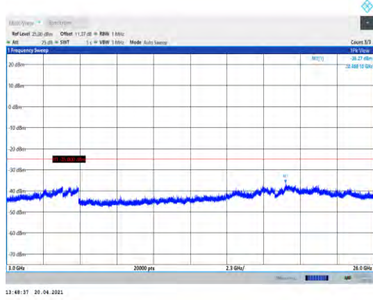
Band7-10MHz-16QAM-21100-1RB#0-Range3:3000~26000MHz
