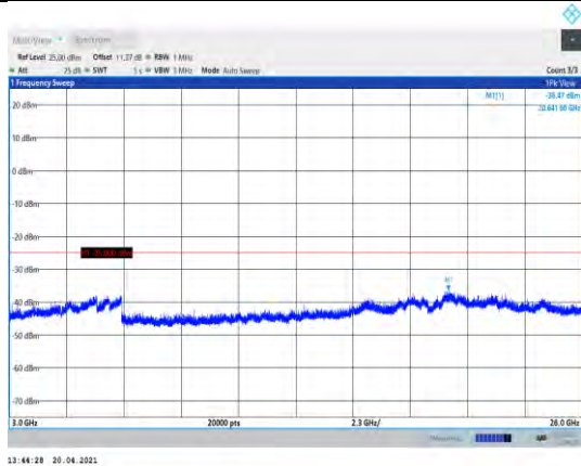
Band7-5MHz-QPSK-21425-1RB#0- Range3:3000~26000MHz
