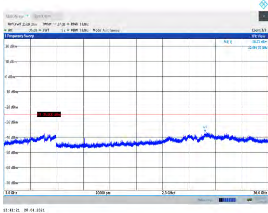
Band7-5MHz-QPSK-20775-1RB#0- Range3:3000~26000MHz
