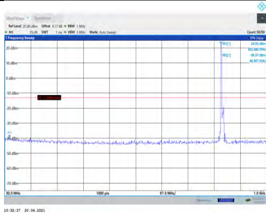
Band5-10MHz-QPSK-20525-1RB#0-Range1:30~1000MHz
