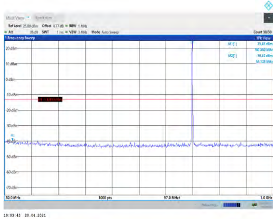
Band12-1.4MHz-QPSK-23095-1RB#0- Range1:30~1000MHz
