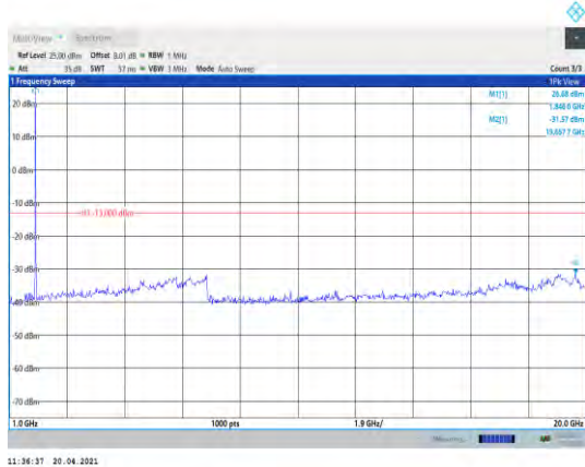
Band2-5MHz-16QAM-18625-1RB#0- Range2:1000~20000MHz
