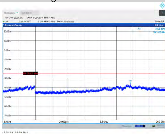
Band7-15MHz-QPSK-20825-1RB#0- Range3:3000~26000MHz
