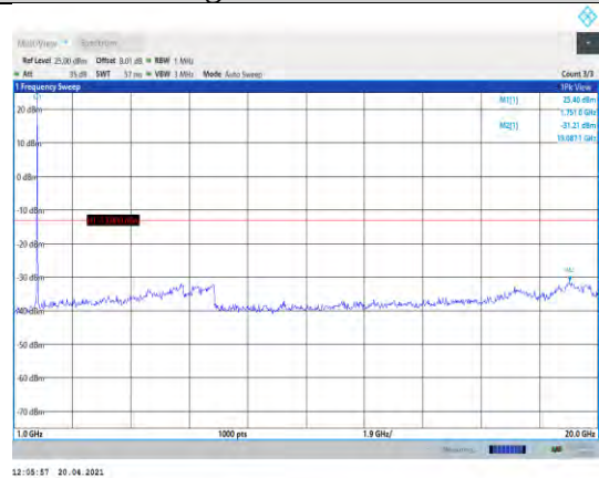
Band4-10MHz-16QAM-20350-1RB#0- Range2:1000~20000MHz
