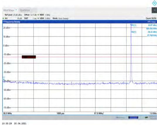
Band5-3MHz-QPSK-20525-1RB#0- Range1:30~1000MHz
