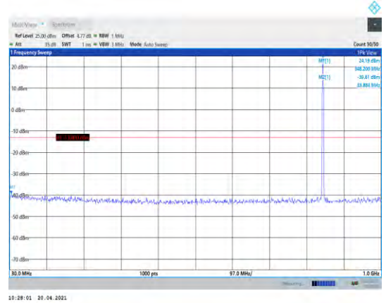
Band5-1.4MHz-16QAM-20643-1RB#0- Range1:30~1000MHz
