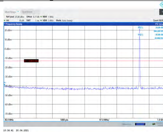
Band5-3MHz-16QAM-20635-1RB#0-Range1:30~1000MHz
