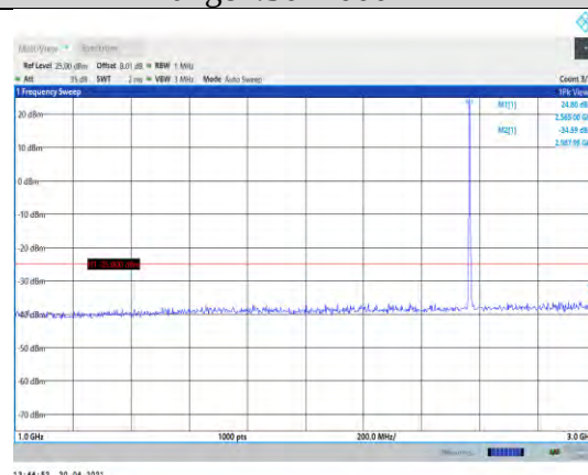
Band7-5MHz-16QAM-21425-1RB#0- Range2:1000~3000MHz
