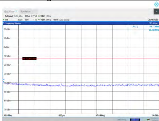
Band2-3MHz-16QAM-18900-1RB#0- Range1:30~1000MHz
