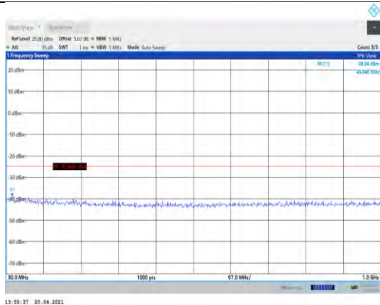
Band7-20MHz-QPSK-20850-1RB#0-Range1:30~1000MHz
