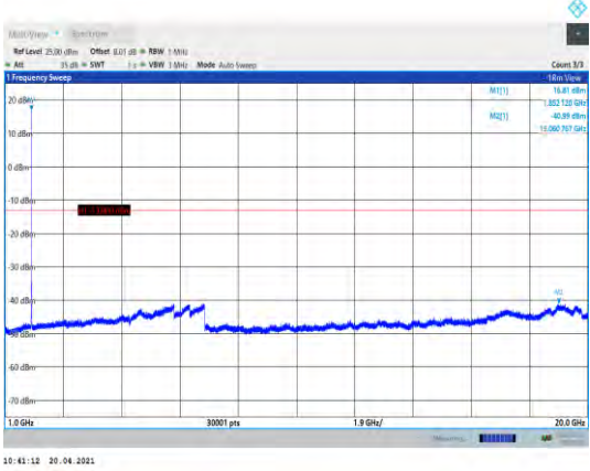
Band2-9262-1000~20000MHz
