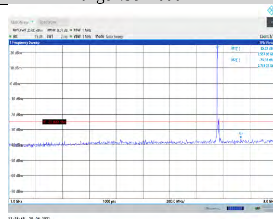
Band7-15MHz-16QAM-21375-1RB#0-Range2:1000~3000MHz
