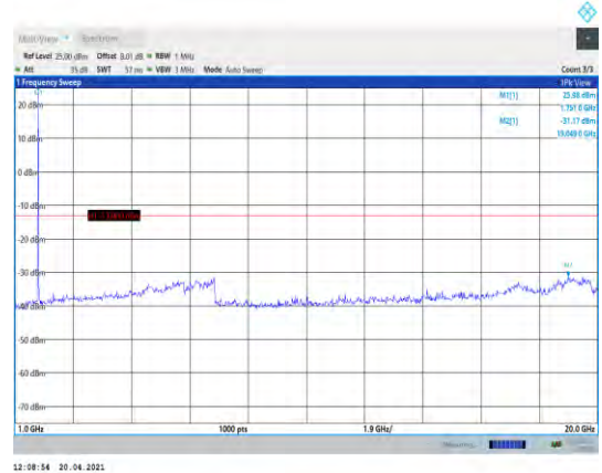
Band4-5MHz-16QAM-20375-1RB#0- Range2:1000~20000MHz
