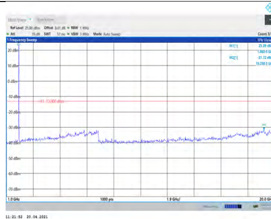
Band2-15MHz-16QAM-18900-1RB#0- Range2:1000~20000MHz
