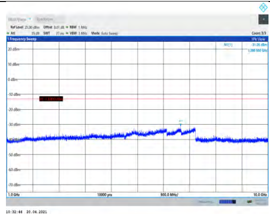
Band5-10MHz-QPSK-20525-1RB#0-Range2:1000~10000MHz
