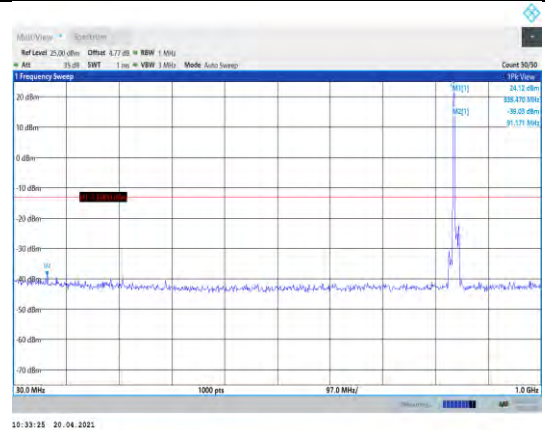
Band5-10MHz-QPSK-20600-1RB#0-Range1:30~1000MHz
