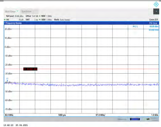
Band7-5MHz-QPSK-21100-1RB#0- Range1:30~1000MHz
