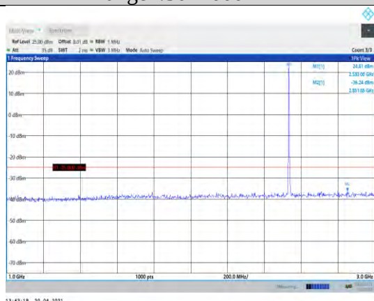
Band7-5MHz-16QAM-21100-1RB#0- Range2:1000~3000MHz
