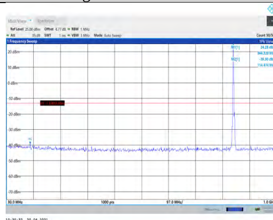
Band5-5MHz-QPSK-20625-1RB#0- Range1:30~1000MHz
