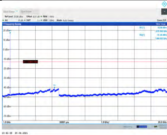
Band2-9400-1000~20000MHz
