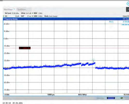
Band5-5MHz-16QAM-20525-1RB#0- Range2:1000~10000MHz
