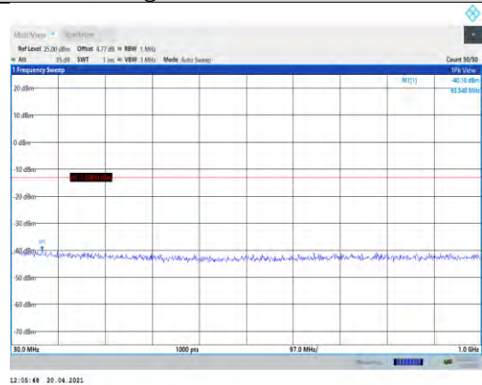
Band4-10MHz-16QAM-20350-1RB#0- Range1:30~1000MHz
