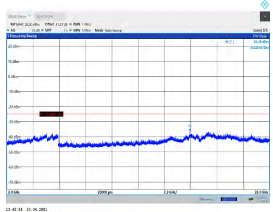
Band7-5MHz-QPSK-21100-1RB#0- Range3:3000~26000MHz
