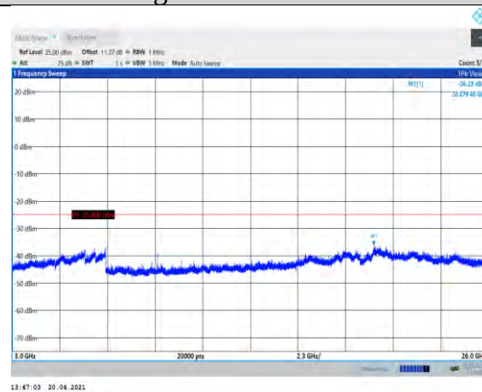
Band7-10MHz-16QAM-20800-1RB#0- Range3:3000~26000MHz
