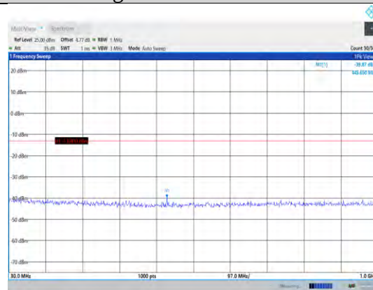
Band2-3MHz-16QAM-19185-1RB#0- Range1:30~1000MHz
