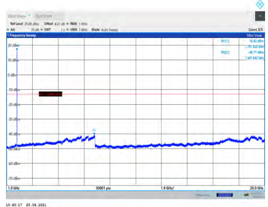
Band4-1513-1000~20000MHz
