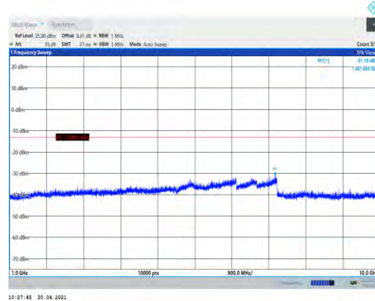
Band5-1.4MHz-QPSK-20643-1RB#0- Range2:1000~10000MHz
