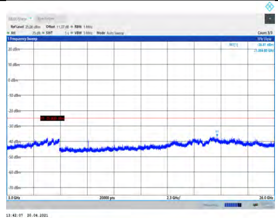
Band7-5MHz-16QAM-20775-1RB#0- Range3:3000~26000MHz
