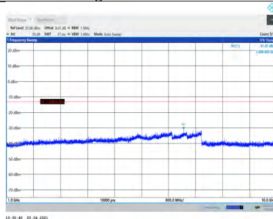
Band5-5MHz-QPSK-20625-1RB#0- Range2:1000~10000MHz
