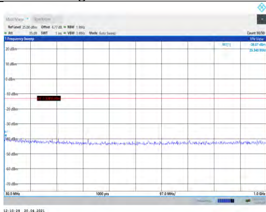
Band4-3MHz-QPSK-20175-1RB#0- Range1:30~1000MHz
