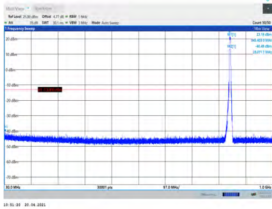
Band5-4233-30~1000MHz
