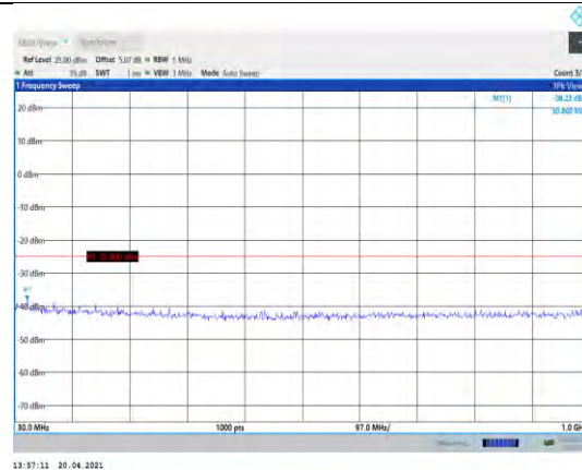
Band7-20MHz-QPSK-21100-1RB#0-Range1:30~1000MHz
