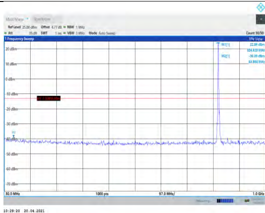
Band5-5MHz-16QAM-20425-1RB#0- Range1:30~1000MHz
