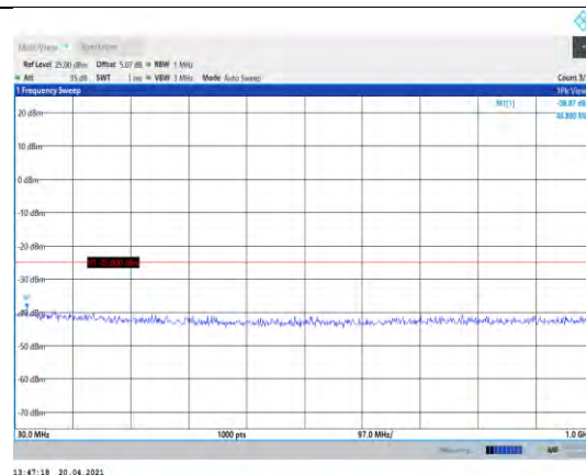
Band7-10MHz-QPSK-21100-1RB#0- Range1:30~1000MHz
