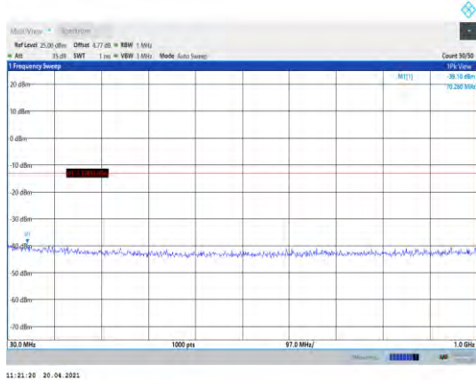
Band2-15MHz-QPSK-18900-1RB#0- Range1:30~1000MHz
