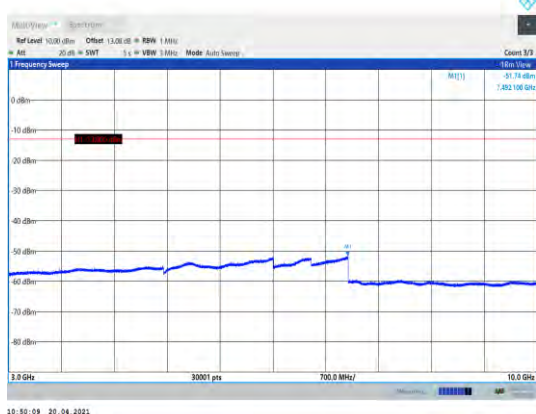
Band5-4132-3000~10000MHz
