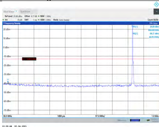
Band5-5MHz-QPSK-20525-1RB#0- Range1:30~1000MHz
