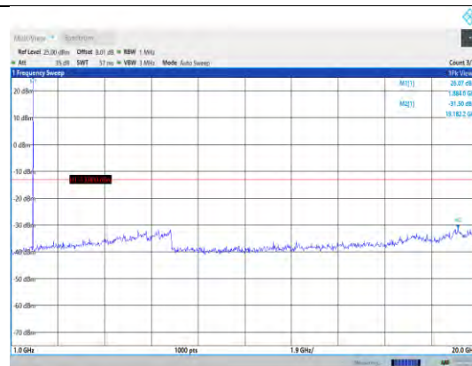
Band2-3MHz-16QAM-18900-1RB#0- Range2:1000~20000MHz
