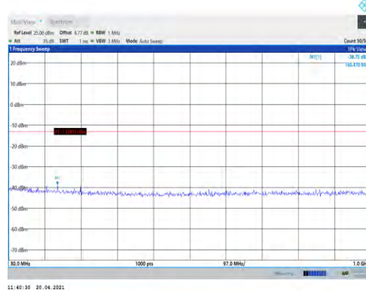
Band2-10MHz-QPSK-19150-1RB#0-Range1:30~1000MHz
