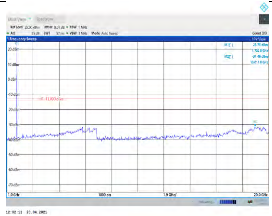
Band4-15MHz-16QAM-20175-1RB#0- Range2:1000~20000MHz
