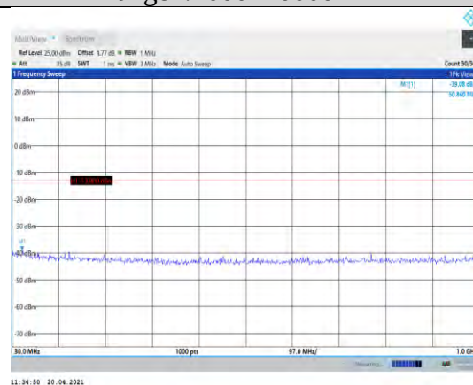
Band2-3MHz-QPSK-19185-1RB#0- Range1:30~1000MHz
