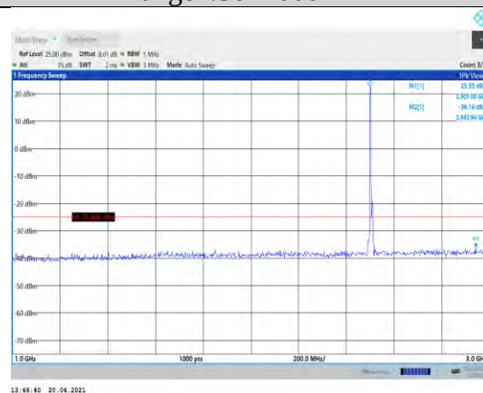
Band7-10MHz-16QAM-20800-1RB#0- Range2:1000~3000MHz
