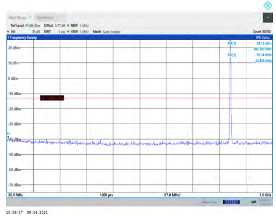
Band5-3MHz-QPSK-20635-1RB#0- Range1:30~1000MHz
