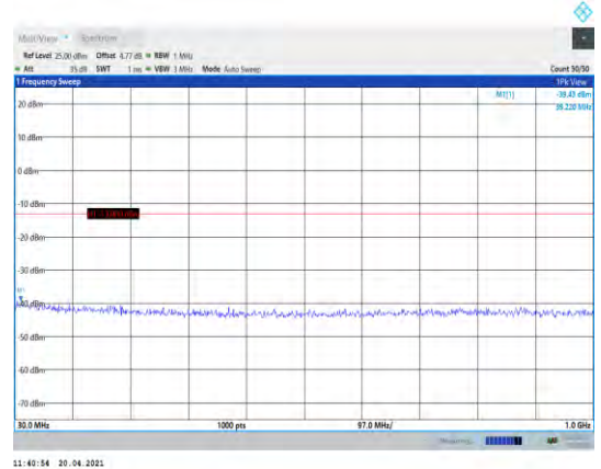
Band2-10MHz-16QAM-19150-1RB#0- Range1:30~1000MHz
