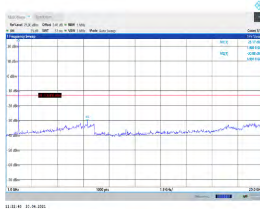
Band2-15MHz-16QAM-19125-1RB#0- Range2:1000~20000MHz
