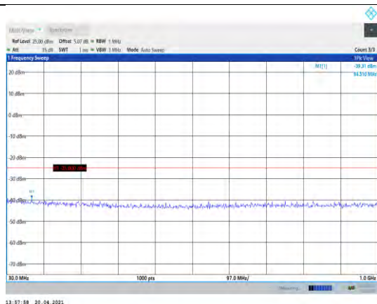
Band7-20MHz-16QAM-21100-1RB#0- Range1:30~1000MHz
