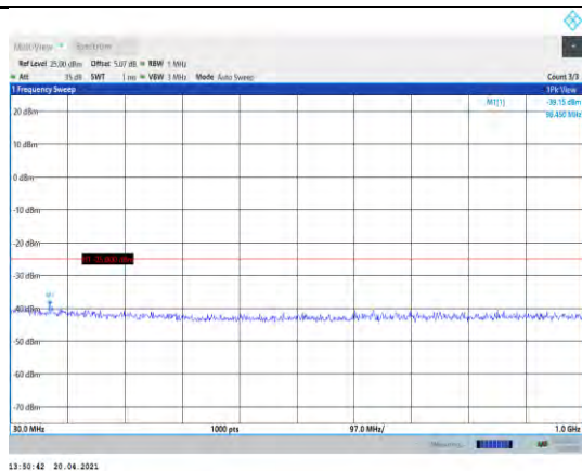
Band7-15MHz-QPSK-20825-1RB#0- Range1:30~1000MHz
