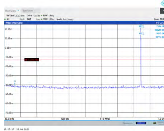
Band5-1.4MHz-QPSK-20643-1RB#0- Range1:30~1000MHz
