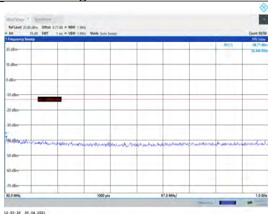
Band4-20MHz-16QAM-20175-1RB#0- Range1:30~1000MHz
