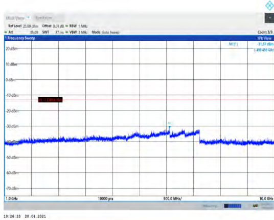
Band5-1.4MHz-16QAM-20407-1RB#0- Range2:1000~10000MHz
