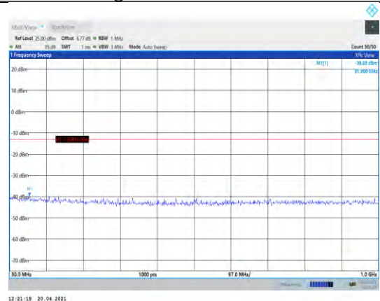
Band4-20MHz-16QAM-20300-1RB#0- Range1:30~1000MHz
