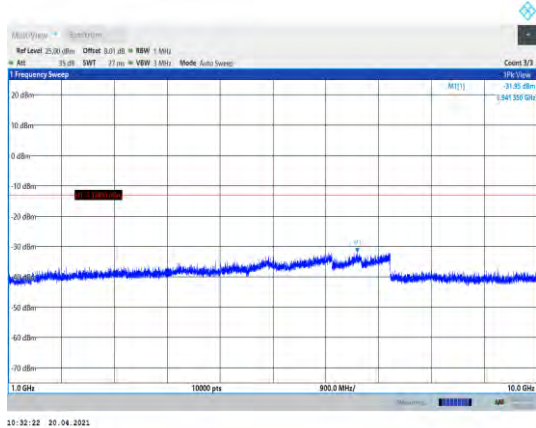
Band5-10MHz-16QAM-20450-1RB#0- Range2:1000~10000MHz
