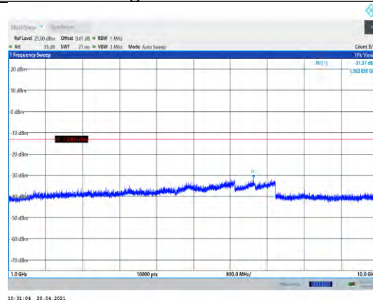
Band5-5MHz-16QAM-20625-1RB#0- Range2:1000~10000MHz
