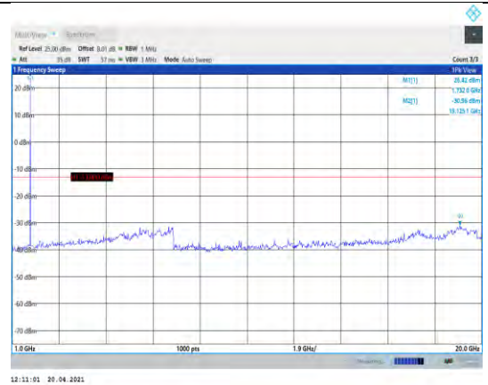
Band4-3MHz-16QAM-20175-1RB#0- Range2:1000~20000MHz
