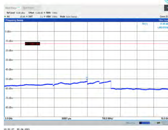
Band5-4182-3000~10000MHz
