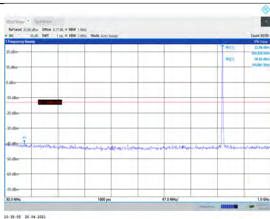
Band5-3MHz-16QAM-20415-1RB#0-Range1:30~1000MHz
