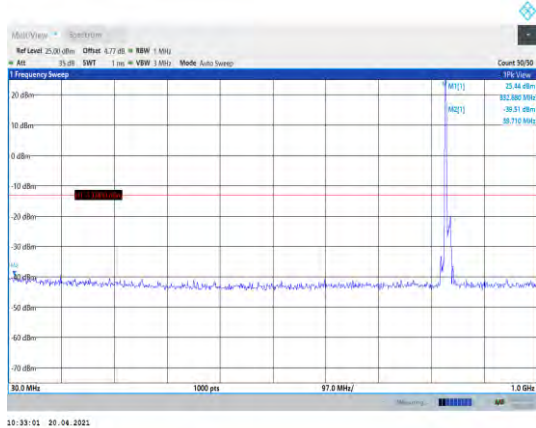
Band5-10MHz-16QAM-20525-1RB#0- Range1:30~1000MHz
