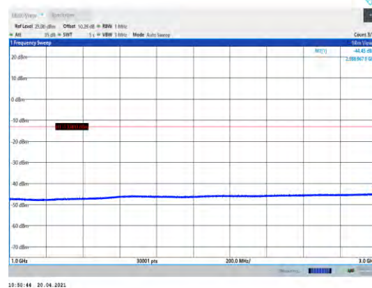
Band5-4182-1000~3000MHz
