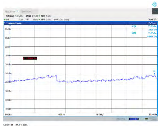
Band4-20MHz-16QAM-20175-1RB#0- Range2:1000~20000MHz
