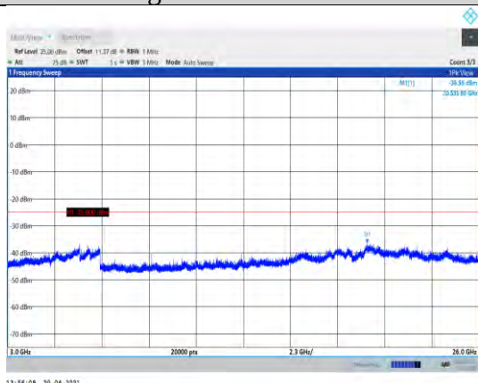
Band7-20MHz-QPSK-20850-1RB#0-Range3:3000~26000MHz
