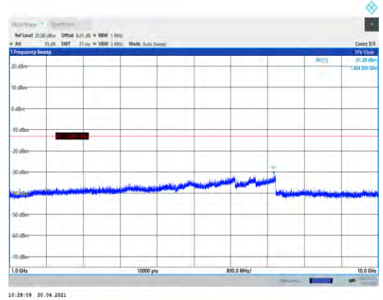
Band5-1.4MHz-16QAM-20643-1RB#0- Range2:1000~10000MHz
