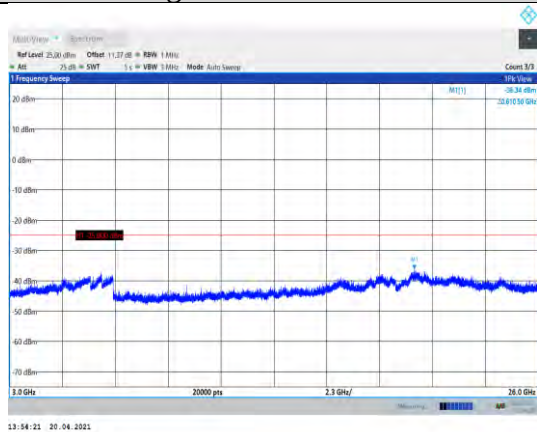
Band7-15MHz-QPSK-21375-1RB#0-Range3:3000~26000MHz
