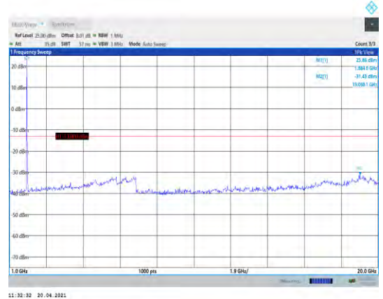
Band2-20MHz-16QAM-19100-1RB#0- Range2:1000~20000MHz
