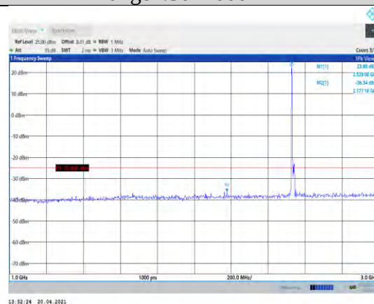
Band7-15MHz-QPSK-21100-1RB#0- Range2:1000~3000MHz
