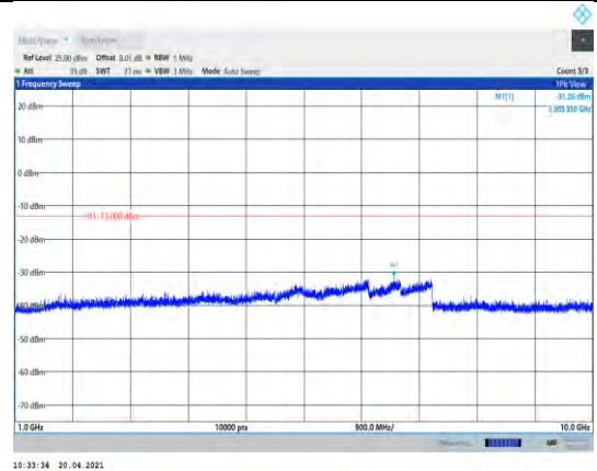
Band5-10MHz-QPSK-20600-1RB#0-Range2:1000~10000MHz
