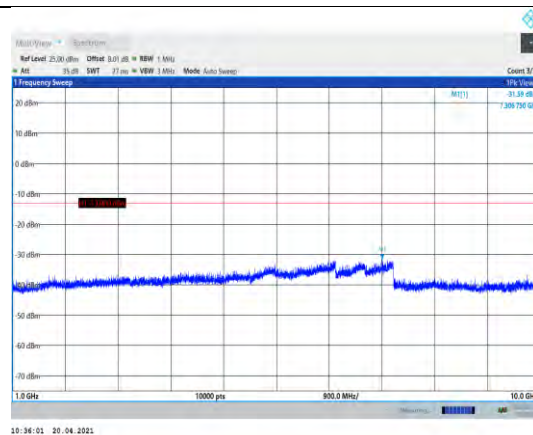
Band5-3MHz-16QAM-20525-1RB#0-Range2:1000~10000MHz
