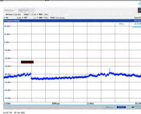
Band7-10MHz-QPSK-21100-1RB#0- Range3:3000~26000MHz
