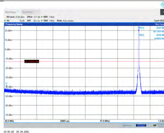
Band5-4182-30~1000MHz
