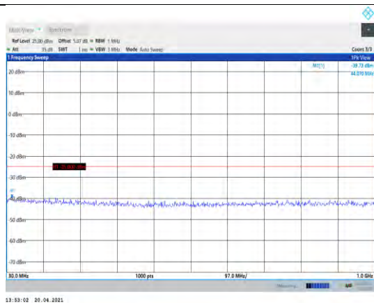
Band7-15MHz-16QAM-21100-1RB#0-Range1:30~1000MHz
