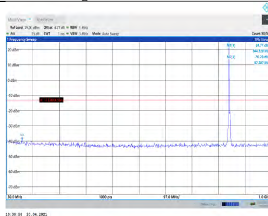
Band5-5MHz-16QAM-20625-1RB#0- Range1:30~1000MHz
