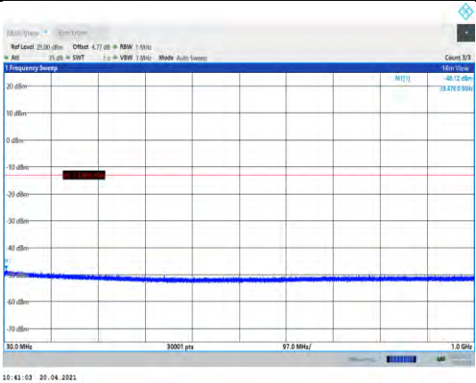
Band2-9262-30~1000MHz
