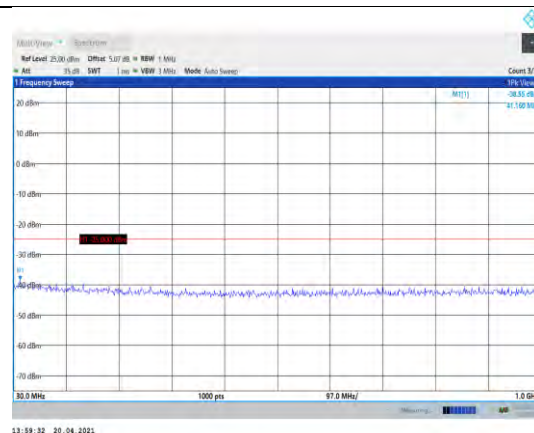
Band7-20MHz-16QAM-21350-1RB#0- Range1:30~1000MHz
