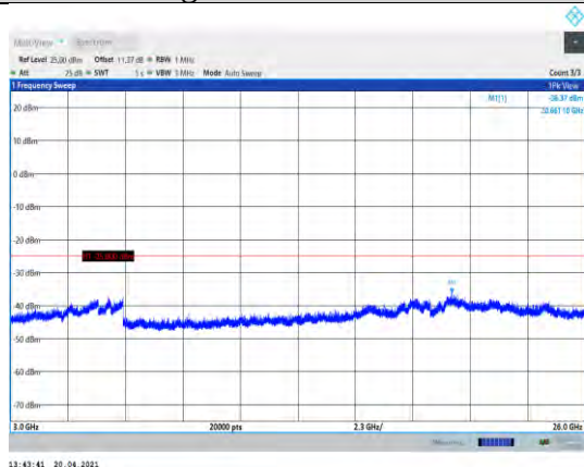
Band7-5MHz-16QAM-21100-1RB#0- Range3:3000~26000MHz
