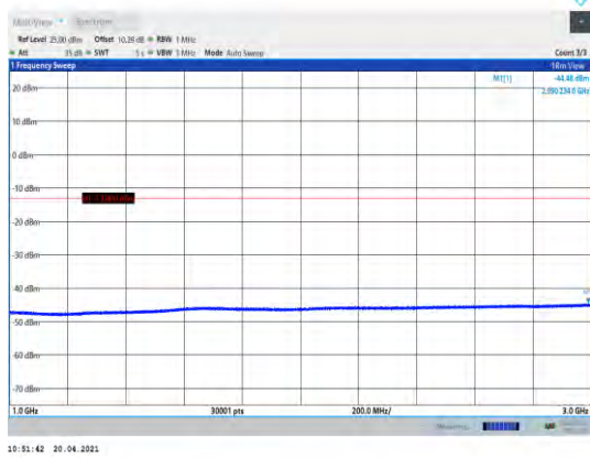
Band5-4233-1000~3000MHz
