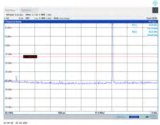
Band12-1.4MHz-16QAM-23173-1RB#0- Range1:30~1000MHz
