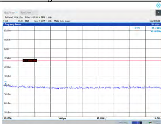
Band4-10MHz-QPSK-20175-1RB#0- Range1:30~1000MHz
