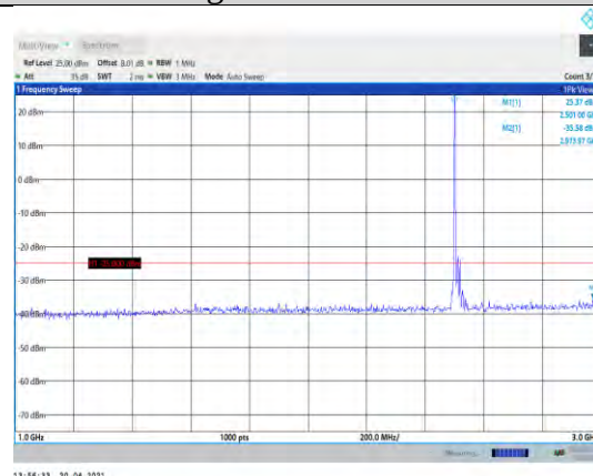
Band7-20MHz-16QAM-20850-1RB#0-Range2:1000~3000MHz
