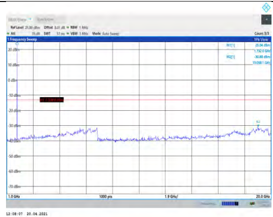
Band4-5MHz-16QAM-20175-1RB#0- Range2:1000~20000MHz
