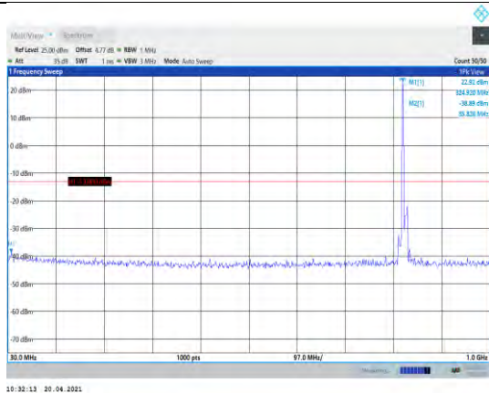
Band5-10MHz-16QAM-20450-1RB#0- Range1:30~1000MHz
