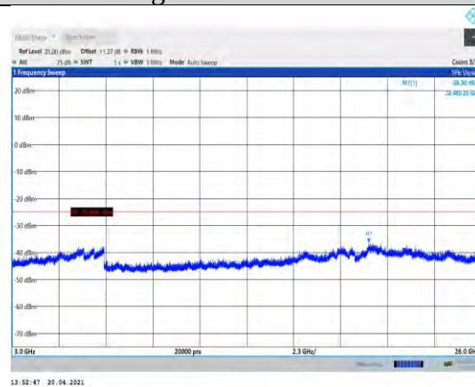
Band7-15MHz-QPSK-21100-1RB#0- Range3:3000~26000MHz
