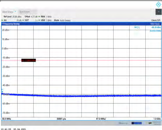
Band2-9400-30~1000MHz
