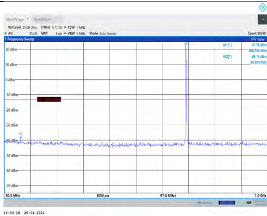
Band12-1.4MHz-16QAM-23017-1RB#0- Range1:30~1000MHz
