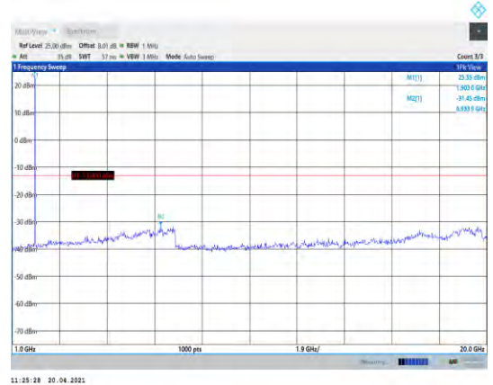
Band2-1.4MHz-16QAM-19193-1RB#0- Range2:1000~20000MHz
