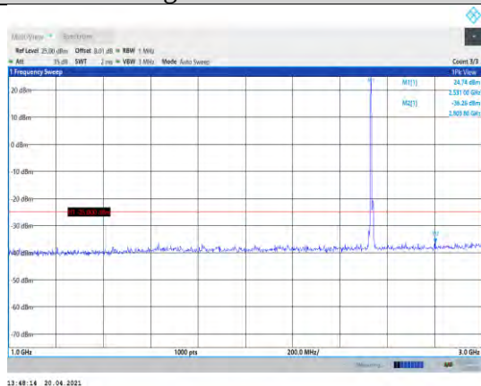
Band7-10MHz-16QAM-21100-1RB#0-Range2:1000~3000MHz
