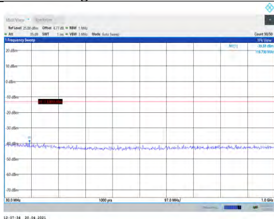
Band4-5MHz-QPSK-20175-1RB#0- Range1:30~1000MHz
