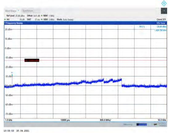
Band12-1.4MHz-16QAM-23173-1RB#0- Range2:1000~10000MHz
