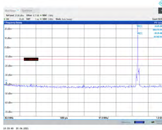
Band5-10MHz-16QAM-20600-1RB#0- Range1:30~1000MHz
