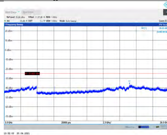
Band7-15MHz-16QAM-20825-1RB#0-Range3:3000~26000MHz
