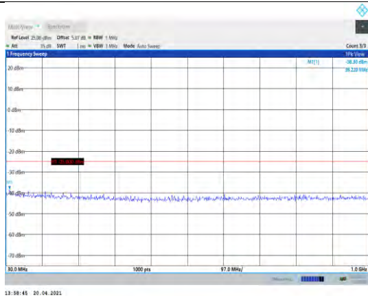
Band7-20MHz-QPSK-21350-1RB#0-Range1:30~1000MHz
