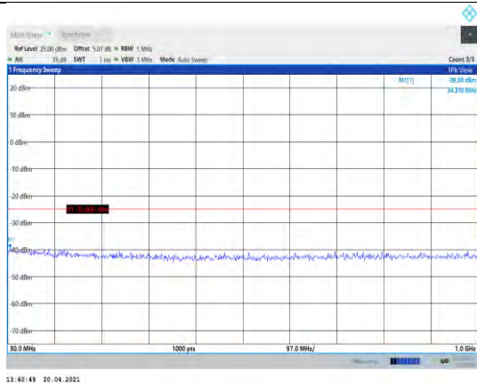
Band7-5MHz-QPSK-20775-1RB#0- Range1:30~1000MHz
