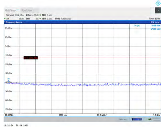
Band2-20MHz-16QAM-19100-1RB#0- Range1:30~1000MHz
