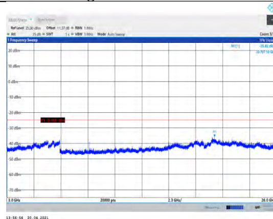
Band7-20MHz-16QAM-20850-1RB#0-Range3:3000~26000MHz
