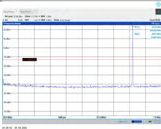
Band5-1.4MHz-QPSK-20407-1RB#0- Range1:30~1000MHz
