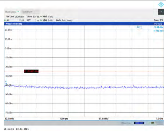
Band7-5MHz-16QAM-20775-1RB#0- Range1:30~1000MHz
