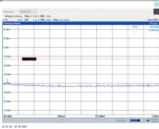
Band4-15MHz-16QAM-20025-1RB#0- Range1:30~1000MHz
