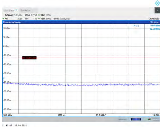
Band2-10MHz-16QAM-18900-1RB#0- Range1:30~1000MHz
