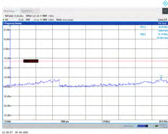
Band2-10MHz-16QAM-18650-1RB#0- Range2:1000~20000MHz
