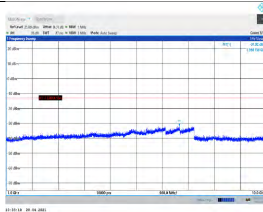
Band5-10MHz-16QAM-20525-1RB#0- Range2:1000~10000MHz
