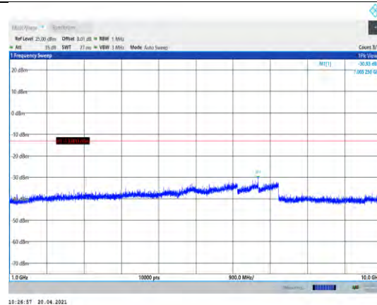
Band5-1.4MHz-QPSK-20525-1RB#0- Range2:1000~10000MHz
