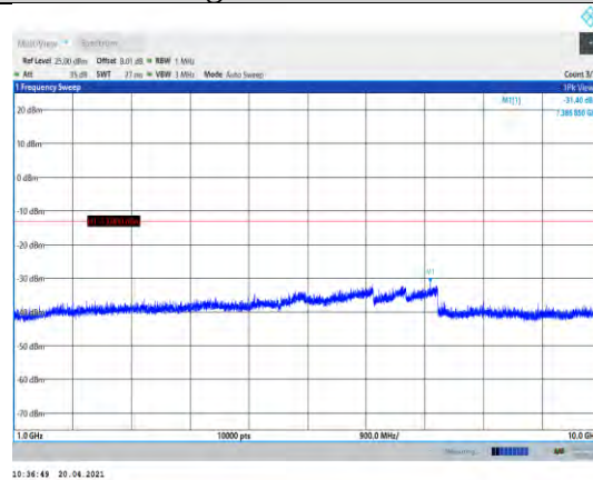
Band5-3MHz-16QAM-20635-1RB#0-Range2:1000~10000MHz
