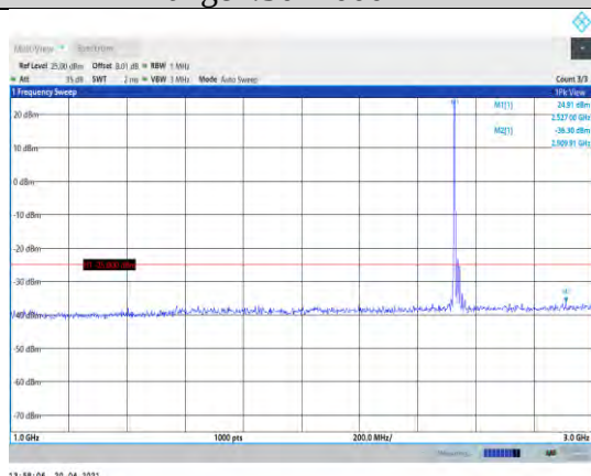
Band7-20MHz-16QAM-21100-1RB#0- Range2:1000~3000MHz
