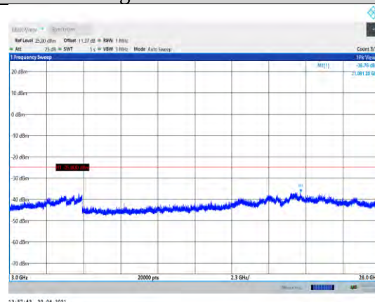
Band7-20MHz-QPSK-21100-1RB#0-Range3:3000~26000MHz
