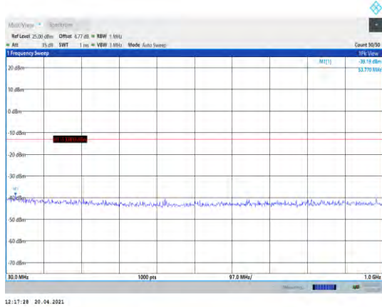
Band4-1.4MHz-QPSK-20175-1RB#0- Range1:30~1000MHz
