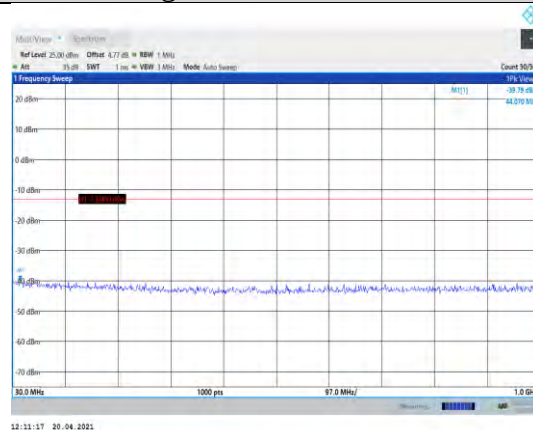
Band4-3MHz-QPSK-20385-1RB#0- Range1:30~1000MHz
