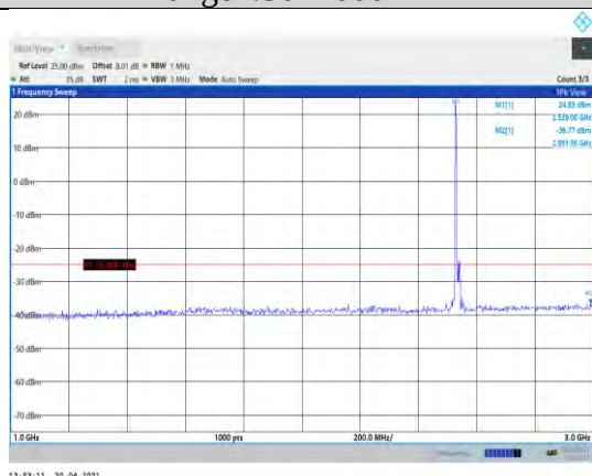
Band7-15MHz-16QAM-21100-1RB#0-Range2:1000~3000MHz
