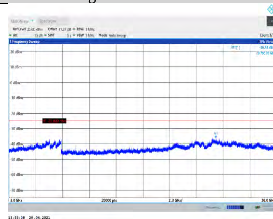
Band7-15MHz-16QAM-21375-1RB#0-Range3:3000~26000MHz
