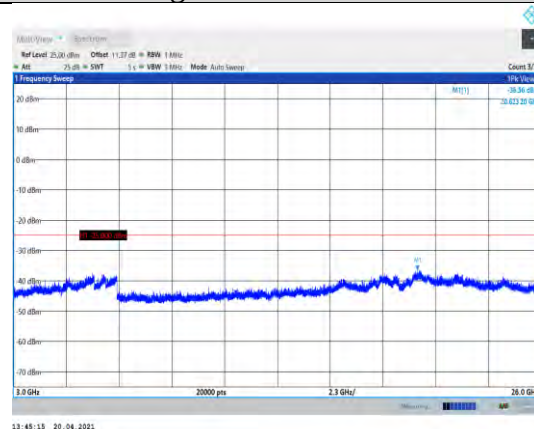
Band7-5MHz-16QAM-21425-1RB#0- Range3:3000~26000MHz
