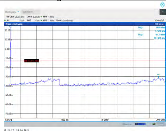
Band4-20MHz-16QAM-20300-1RB#0- Range2:1000~20000MHz
