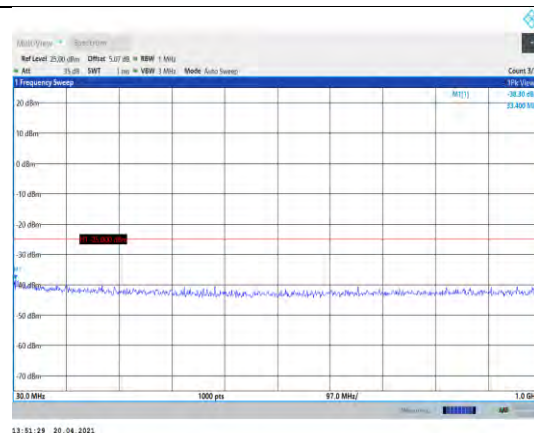
Band7-15MHz-16QAM-20825-1RB#0-Range1:30~1000MHz
