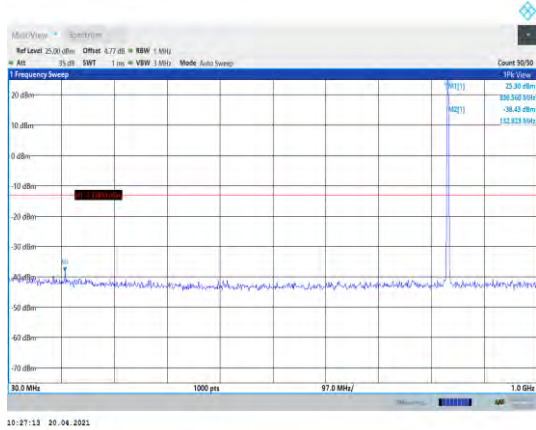
Band5-1.4MHz-16QAM-20525-1RB#0- Range1:30~1000MHz
