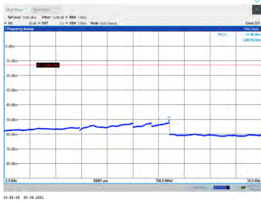
Band5-4233-3000~10000MHz
