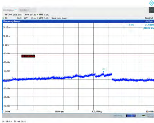
Band5-1.4MHz-QPSK-20407-1RB#0- Range2:1000~10000MHz
