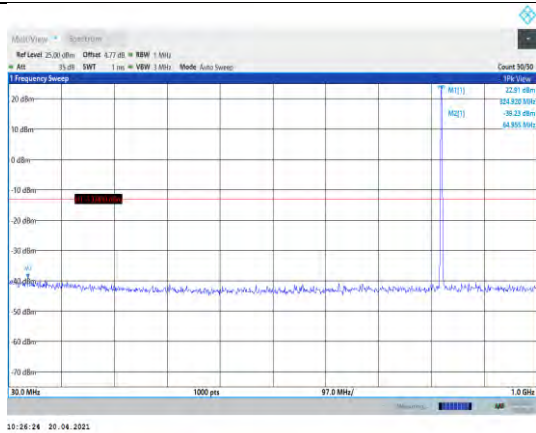
Band5-1.4MHz-16QAM-20407-1RB#0- Range1:30~1000MHz
