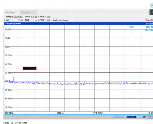
Band7-15MHz-QPSK-21100-1RB#0- Range1:30~1000MHz
