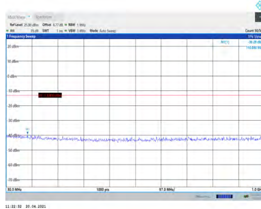
Band2-15MHz-16QAM-19125-1RB#0- Range1:30~1000MHz
