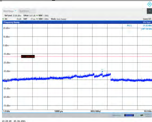
Band5-5MHz-16QAM-20425-1RB#0- Range2:1000~10000MHz
