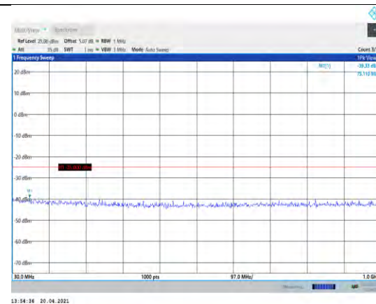
Band7-15MHz-16QAM-21375-1RB#0-Range1:30~1000MHz
