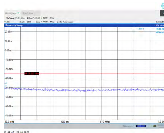
Band7-5MHz-16QAM-21425-1RB#0- Range1:30~1000MHz
