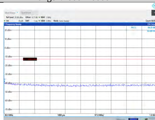
Band4-10MHz-QPSK-20350-1RB#0- Range1:30~1000MHz
