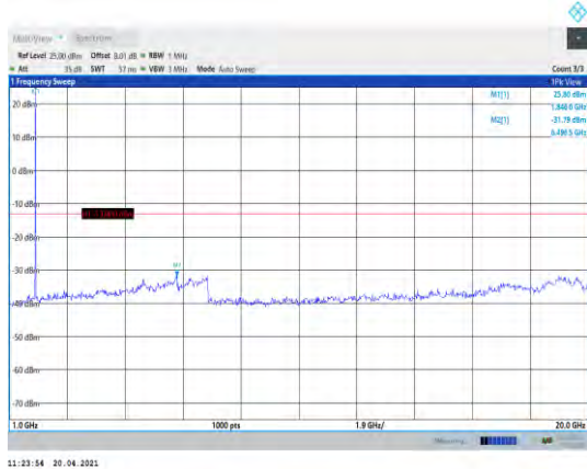
Band2-1.4MHz-16QAM-18607-1RB#0- Range2:1000~20000MHz
