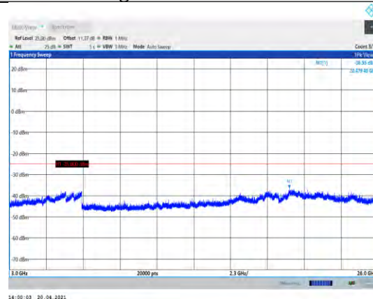
Band7-20MHz-16QAM-21350-1RB#0- Range3:3000~26000MHz
