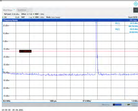
Band12-10MHz-QPSK-23060-1RB#0- Range1:30~1000MHz
