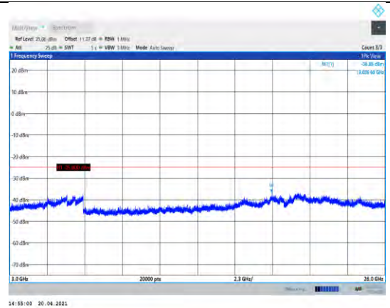
Band41-20MHz-16QAM-41140-1RB#0- Range3:3000~26000MHz
