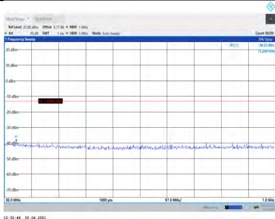
Band66-1.4MHz-QPSK-132665-1RB#0- Range1:30~1000MHz
