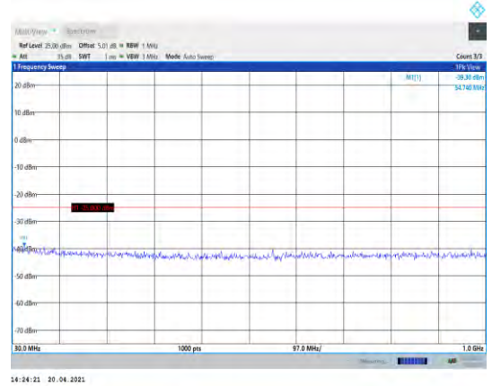
Band38-20MHz-QPSK-37850-1RB#0- Range1:30~1000MHz
