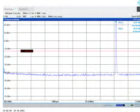
Band26-5MHz-16QAM-26765-1RB#0- Range1:30~1000MHz
