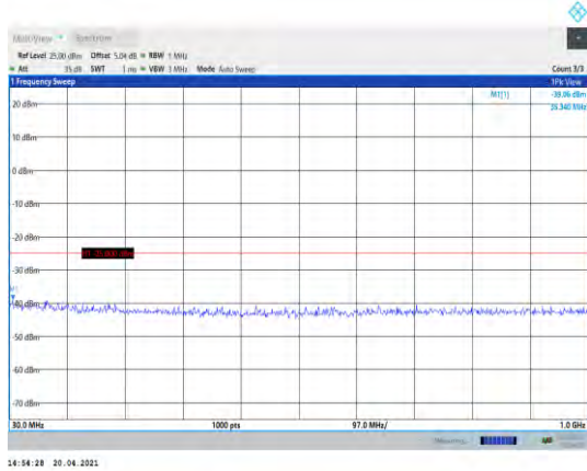
Band41-20MHz-16QAM-41140-1RB#0- Range1:30~1000MHz
