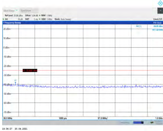
Band41-5MHz-16QAM-40265-1RB#0- Range1:30~1000MHz
