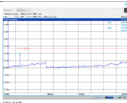
Band66-3MHz-16QAM-132657-1RB#0-Range2:1000~20000MHz
