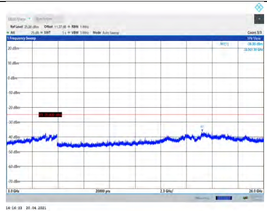
Band38-10MHz-QPSK-38000-1RB#0- Range3:3000~26000MHz
