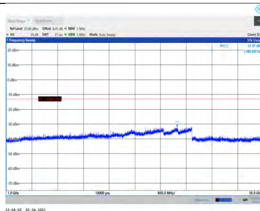
Band26-3MHz-QPSK-26740-1RB#0- Range2:1000~10000MHz
