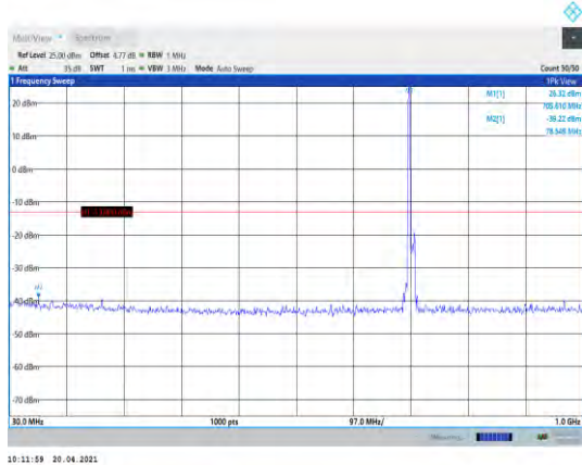
Band17-10MHz-16QAM-23790-1RB#0- Range1:30~1000MHz
