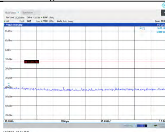
Band66-5MHz-QPSK-131997-1RB#0-Range1:30~1000MHz
