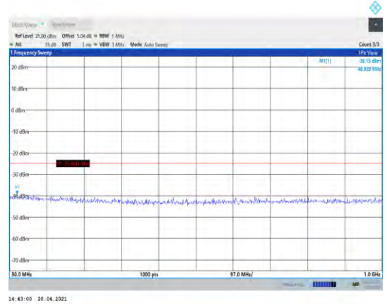
Band41-10MHz-16QAM-40740-1RB#0- Range1:30~1000MHz
