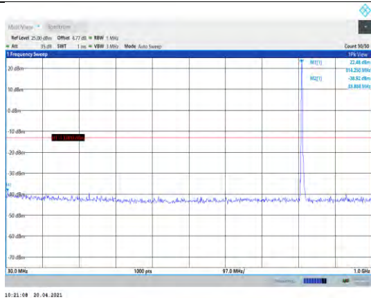
Band26-5MHz-16QAM-26715-1RB#0- Range1:30~1000MHz
