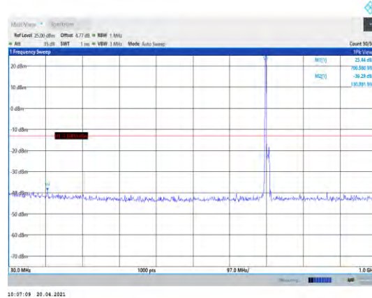
Band12-10MHz-QPSK-23130-1RB#0- Range1:30~1000MHz
