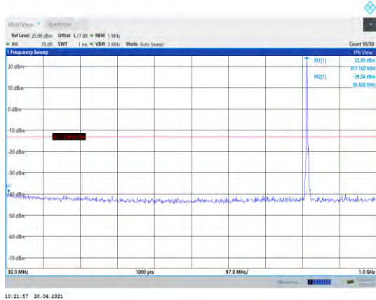
Band26-5MHz-16QAM-26740-1RB#0- Range1:30~1000MHz
