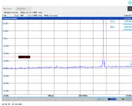
Band41-5MHz-16QAM-40265-1RB#0- Range2:1000~3000MHz
