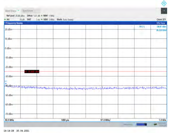
Band38-10MHz-QPSK-37800-1RB#0- Range1:30~1000MHz
