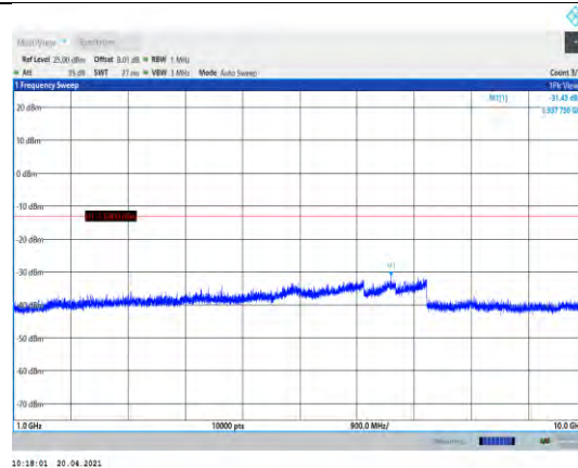
Band26-1.4MHz-QPSK-26740-1RB#0-Range2:1000~10000MHz
