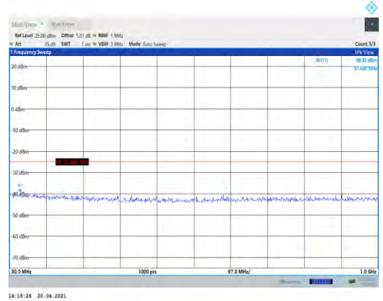
Band38-15MHz-QPSK-37825-1RB#0- Range1:30~1000MHz
