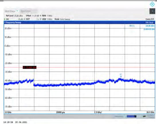
Band38-10MHz-16QAM-38200-1RB#0- Range3:3000~26000MHz
