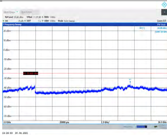
Band38-20MHz-QPSK-37850-1RB#0- Range3:3000~26000MHz
