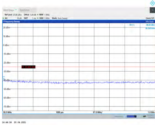
Band41-10MHz-16QAM-41190-1RB#0- Range1:30~1000MHz
