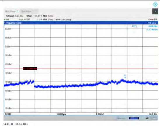
Band38-15MHz-QPSK-38000-1RB#0- Range3:3000~26000MHz
