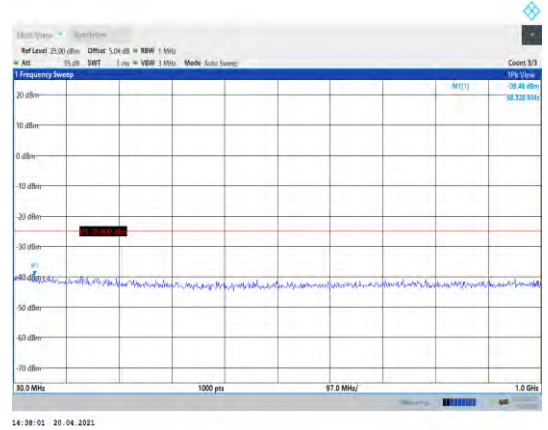
Band41-5MHz-16QAM-40740-1RB#0- Range1:30~1000MHz
