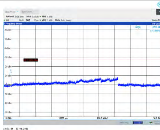
Band12-3MHz-16QAM-23095-1RB#0- Range2:1000~10000MHz
