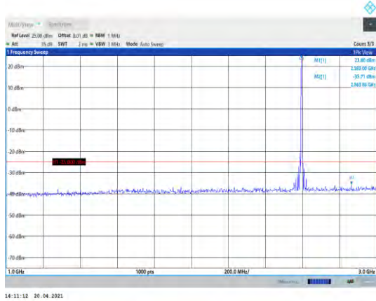
Band38-5MHz-QPSK-38000-1RB#0-Range2:1000~3000MHz
