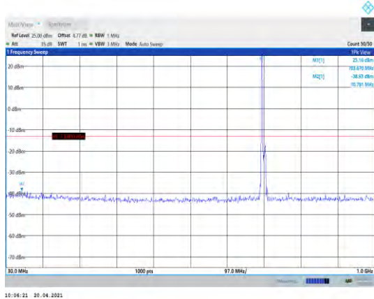
Band12-10MHz-QPSK-23095-1RB#0- Range1:30~1000MHz
