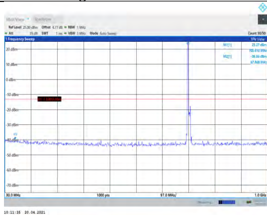
Band17-10MHz-QPSK-23790-1RB#0- Range1:30~1000MHz
