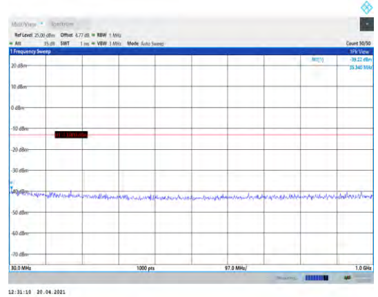
Band66-1.4MHz-QPSK-131979-1RB#0- Range1:30~1000MHz
