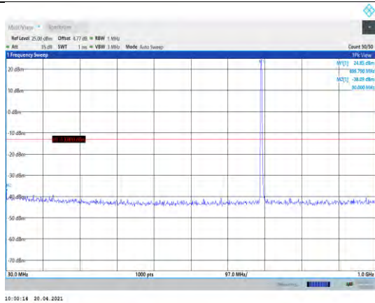
Band12-3MHz-QPSK-23025-1RB#0- Range1:30~1000MHz
