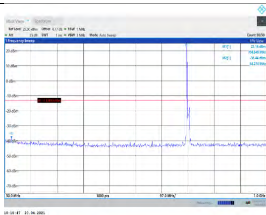
Band17-10MHz-QPSK-23780-1RB#0- Range1:30~1000MHz
