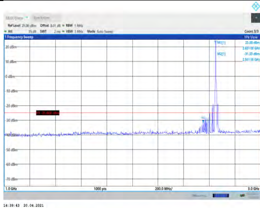
Band41-5MHz-16QAM-41215-1RB#0- Range2:1000~3000MHz
