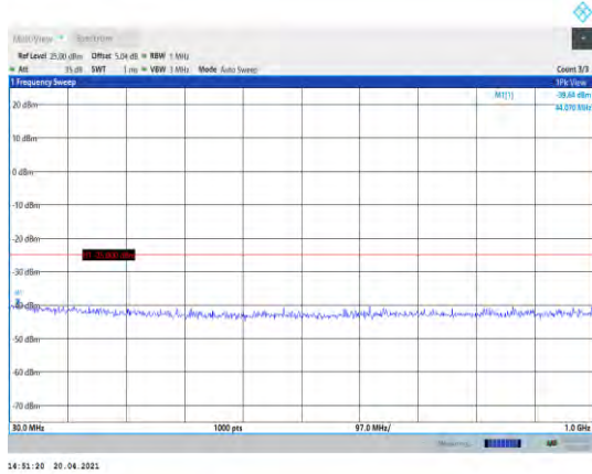
Band41-20MHz-16QAM-40340-1RB#0-Range1:30~1000MHz
