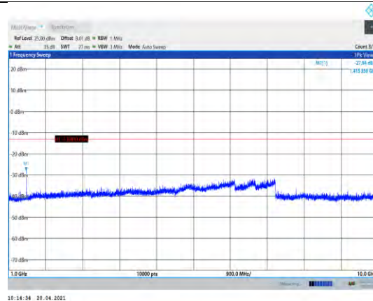
Band17-5MHz-QPSK-23790-1RB#0- Range2:1000~10000MHz
