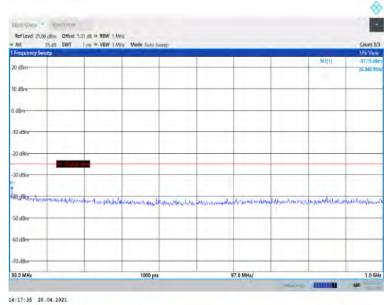
Band38-10MHz-QPSK-38200-1RB#0- Range1:30~1000MHz
