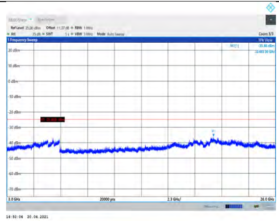
Band41-15MHz-16QAM-41165-1RB#0- Range3:3000~26000MHz
