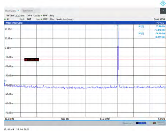
Band12-3MHz-QPSK-23165-1RB#0- Range1:30~1000MHz
