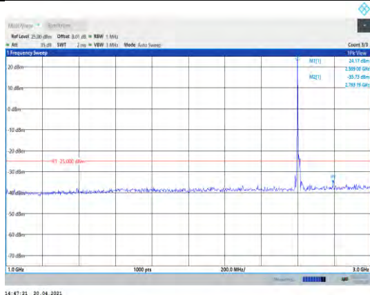
Band41-15MHz-QPSK-40740-1RB#0- Range2:1000~3000MHz
