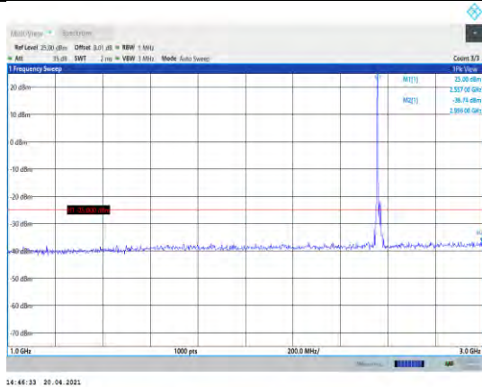
Band41-15MHz-16QAM-40315-1RB#0- Range2:1000~3000MHz
