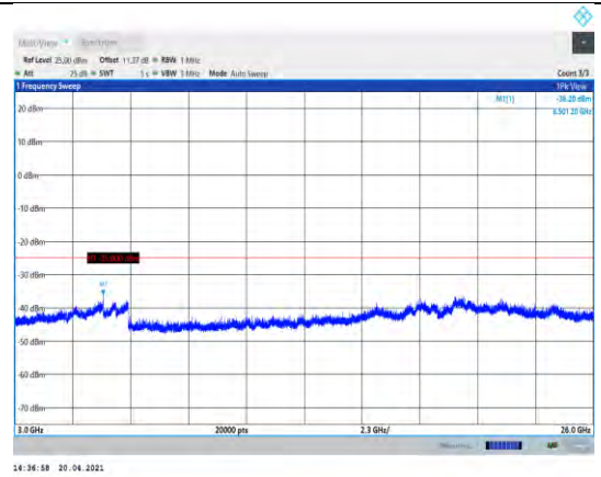
Band41-5MHz-16QAM-40265-1RB#0- Range3:3000~26000MHz
