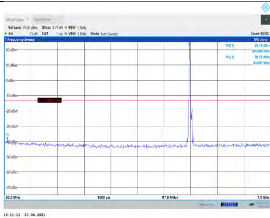
Band17-10MHz-16QAM-23780-1RB#0- Range1:30~1000MHz
