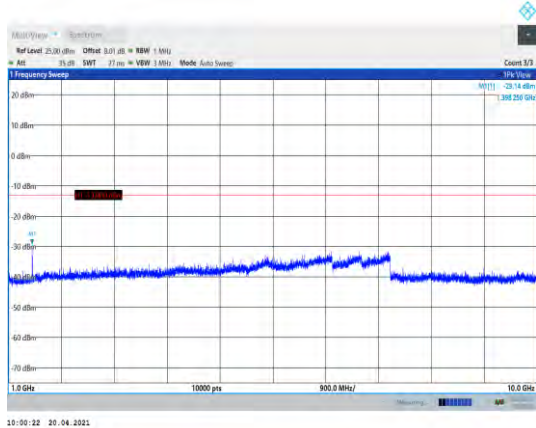
Band12-3MHz-QPSK-23025-1RB#0- Range2:1000~10000MHz
