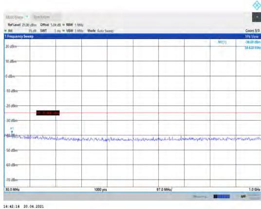
Band41-10MHz-QPSK-40740-1RB#0- Range1:30~1000MHz
