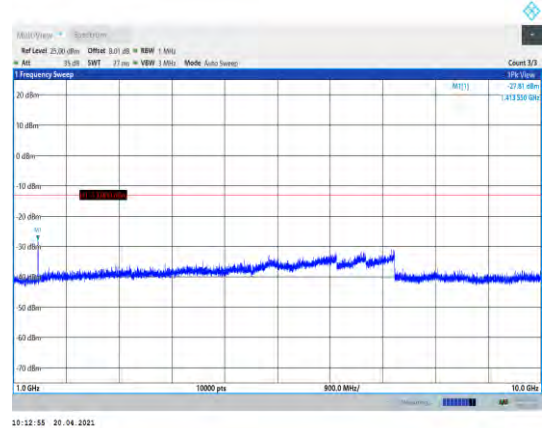
Band17-10MHz-16QAM-23800-1RB#0- Range2:1000~10000MHz
