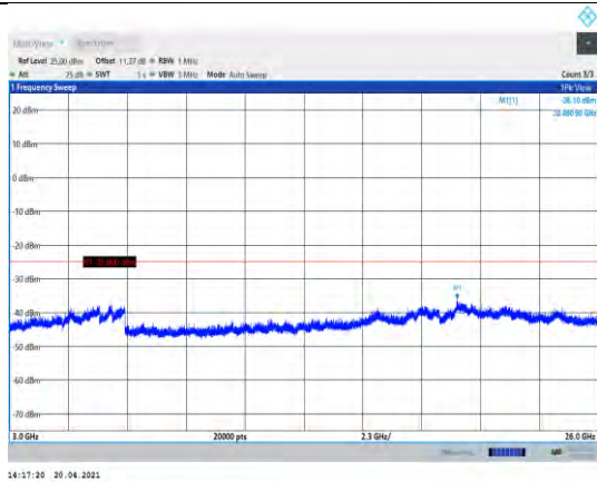
Band38-10MHz-16QAM-38000-1RB#0- Range3:3000~26000MHz
