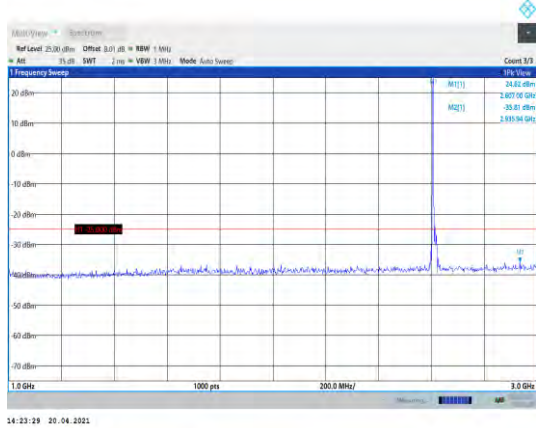
Band38-15MHz-16QAM-38175-1RB#0- Range2:1000~3000MHz
