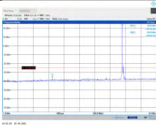
Band41-20MHz-16QAM-40340-1RB#0-Range2:1000~3000MHz
