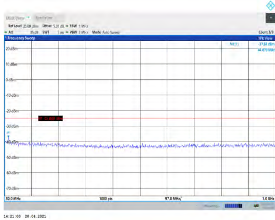
Band38-15MHz-QPSK-38000-1RB#0- Range1:30~1000MHz
