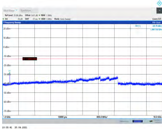
Band12-10MHz-QPSK-23060-1RB#0- Range2:1000~10000MHz
