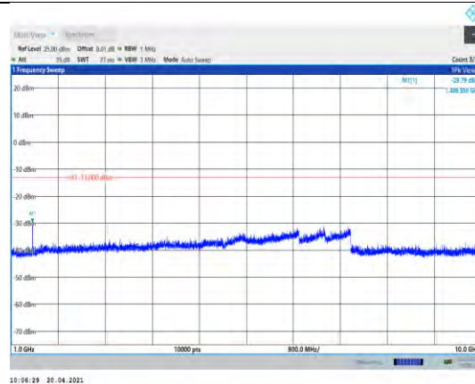
Band12-10MHz-QPSK-23095-1RB#0- Range2:1000~10000MHz
