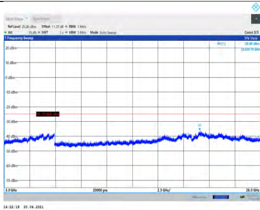
Band38-15MHz-16QAM-38000-1RB#0- Range3:3000~26000MHz
