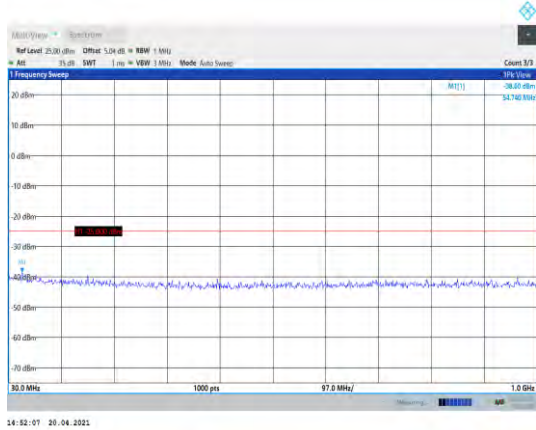
Band41-20MHz-QPSK-40740-1RB#0-Range1:30~1000MHz
