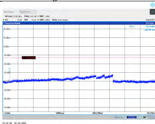
Band17-10MHz-QPSK-23780-1RB#0- Range2:1000~10000MHz
