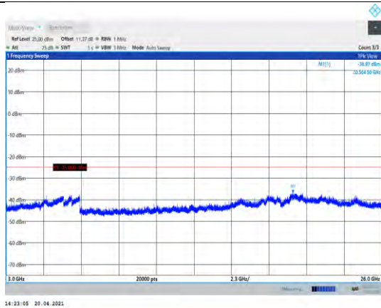
Band38-15MHz-QPSK-38175-1RB#0- Range3:3000~26000MHz
