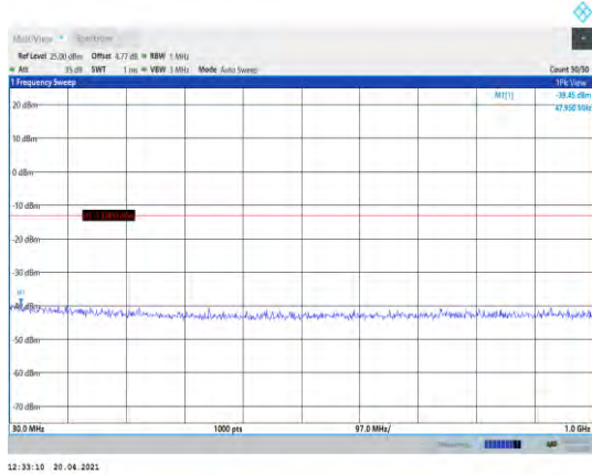
Band66-1.4MHz-16QAM-132665-1RB#0- Range1:30~1000MHz
