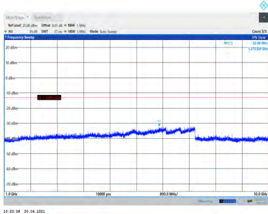
Band26-3MHz-16QAM-26705-1RB#0-Range2:1000~10000MHz
