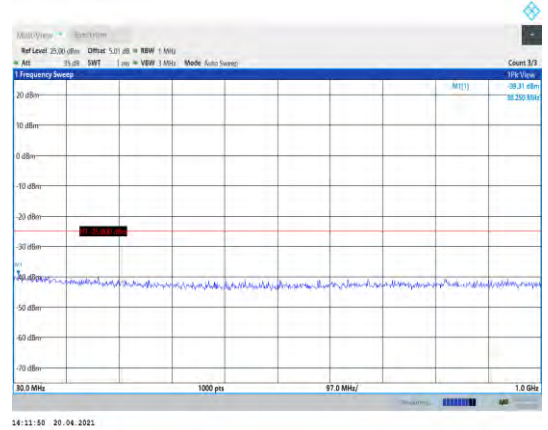
Band38-5MHz-16QAM-38000-1RB#0-Range1:30~1000MHz
