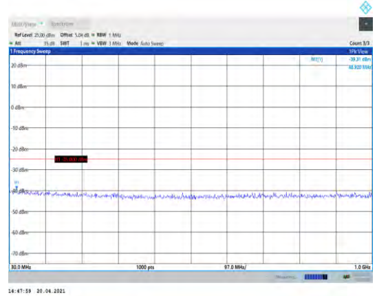
Band41-15MHz-16QAM-40740-1RB#0- Range1:30~1000MHz
