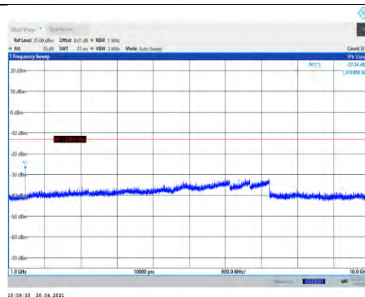
Band12-5MHz-16QAM-23095-1RB#0-Range2:1000~10000MHz
