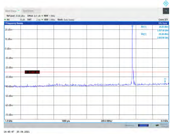
Band41-15MHz-QPSK-40315-1RB#0- Range2:1000~3000MHz
