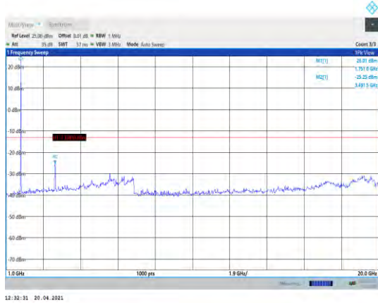
Band66-1.4MHz-16QAM-132322-1RB#0- Range2:1000~20000MHz
