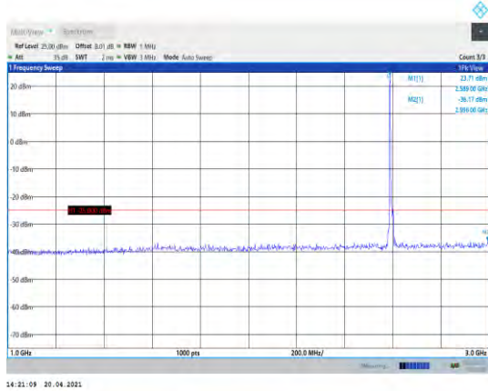
Band38-15MHz-QPSK-38000-1RB#0- Range2:1000~3000MHz
