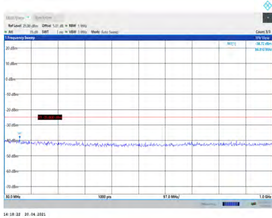
Band38-10MHz-16QAM-38200-1RB#0- Range1:30~1000MHz
