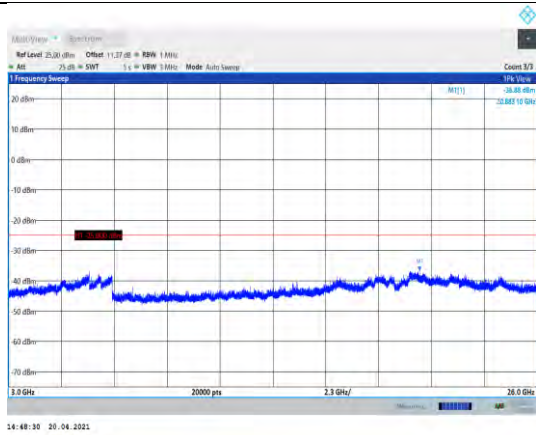
Band41-15MHz-16QAM-40740-1RB#0- Range3:3000~26000MHz
