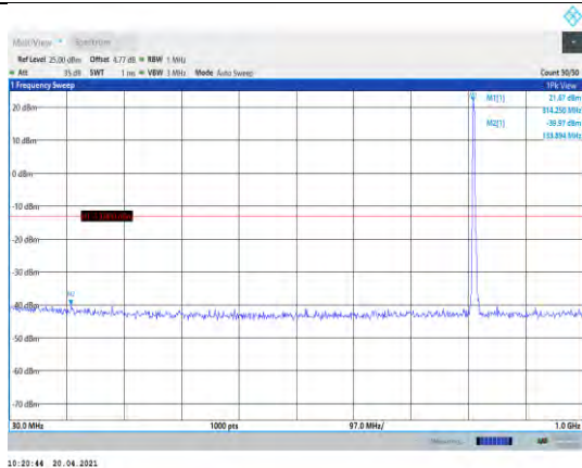
Band26-5MHz-QPSK-26715-1RB#0- Range1:30~1000MHz
