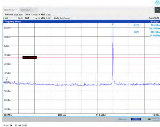
Band17-5MHz-QPSK-23790-1RB#0- Range1:30~1000MHz
