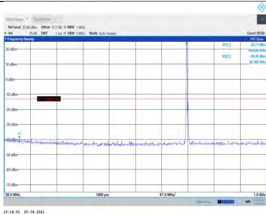
Band17-5MHz-16QAM-23755-1RB#0- Range1:30~1000MHz
