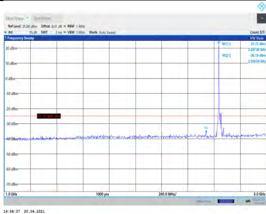
Band41-20MHz-16QAM-41140-1RB#0- Range2:1000~3000MHz
