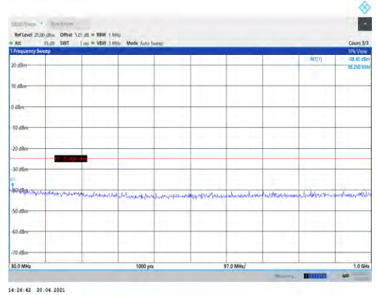
Band38-20MHz-16QAM-38000-1RB#0- Range1:30~1000MHz
