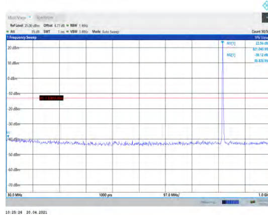
Band26-3MHz-16QAM-26775-1RB#0-Range1:30~1000MHz
