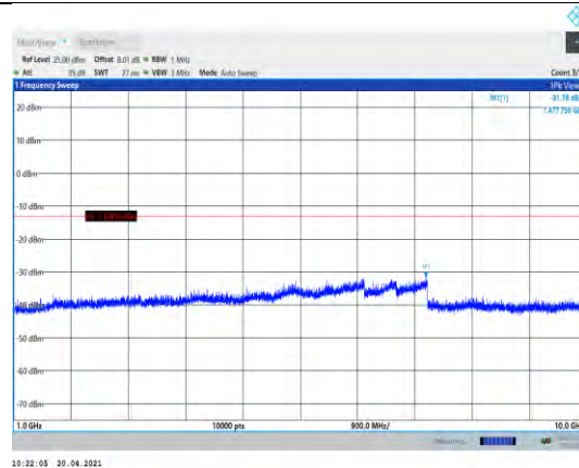
Band26-5MHz-16QAM-26740-1RB#0- Range2:1000~10000MHz
