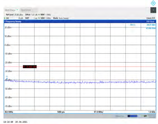
Band38-10MHz-16QAM-38000-1RB#0- Range1:30~1000MHz
