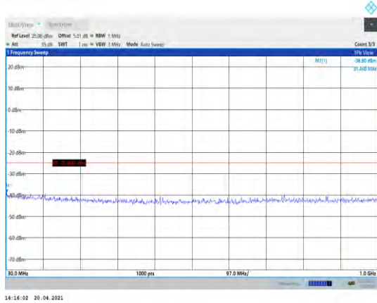
Band38-10MHz-QPSK-38000-1RB#0- Range1:30~1000MHz
