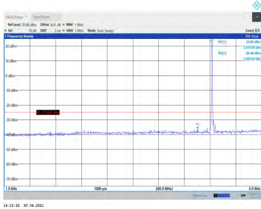
Band38-5MHz-16QAM-38225-1RB#0- Range2:1000~3000MHz
