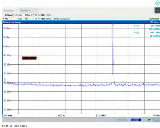
Band17-5MHz-16QAM-23790-1RB#0- Range1:30~1000MHz
