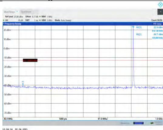
Band26-3MHz-QPSK-26740-1RB#0- Range1:30~1000MHz
