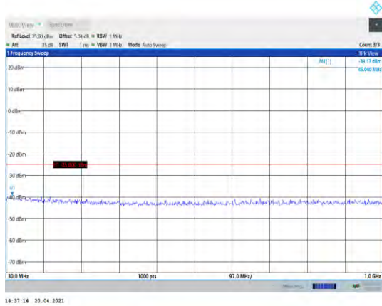
Band41-5MHz-QPSK-40740-1RB#0- Range1:30~1000MHz
