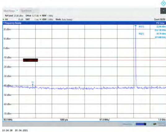
Band26-3MHz-16QAM-26740-1RB#0-Range1:30~1000MHz
