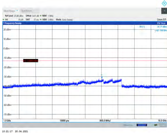
Band26-5MHz-16QAM-26715-1RB#0- Range2:1000~10000MHz
