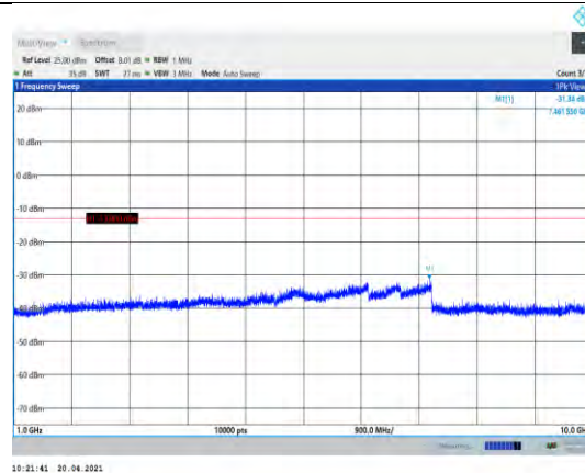
Band26-5MHz-QPSK-26740-1RB#0- Range2:1000~10000MHz
