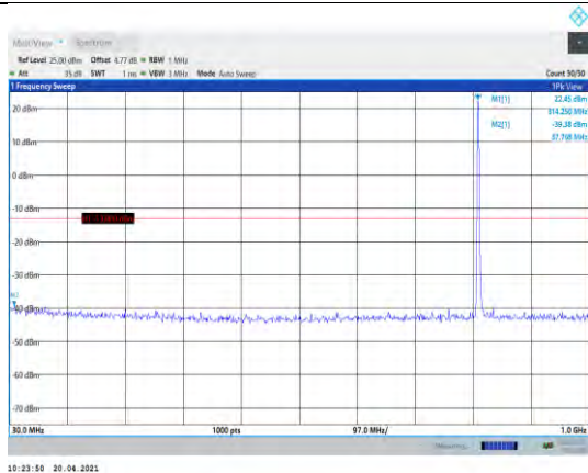
Band26-3MHz-16QAM-26705-1RB#0-Range1:30~1000MHz
