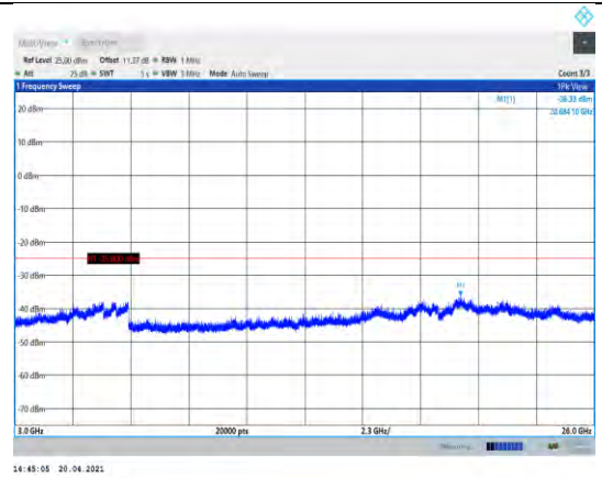
Band41-10MHz-16QAM-41190-1RB#0- Range3:3000~26000MHz
