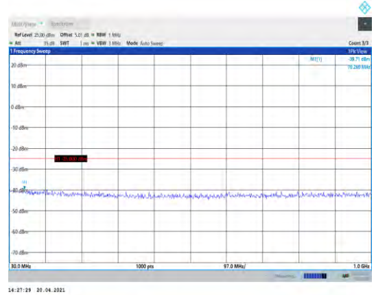
Band38-20MHz-QPSK-38150-1RB#0- Range1:30~1000MHz
