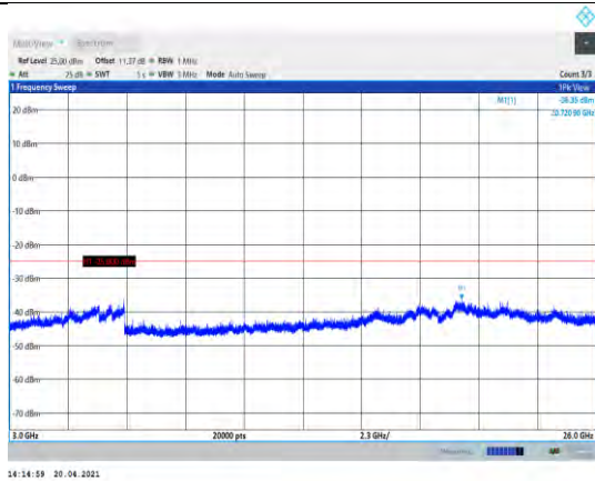
Band38-10MHz-QPSK-37800-1RB#0- Range3:3000~26000MHz
