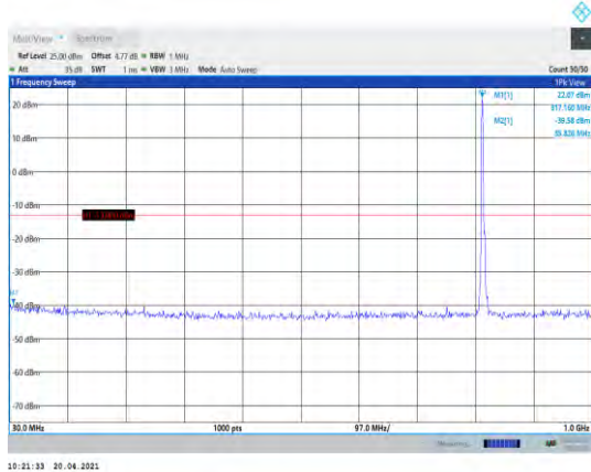
Band26-5MHz-QPSK-26740-1RB#0- Range1:30~1000MHz
