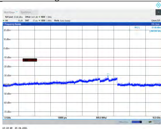
Band26-10MHz-QPSK-26740-1RB#0- Range2:1000~10000MHz
