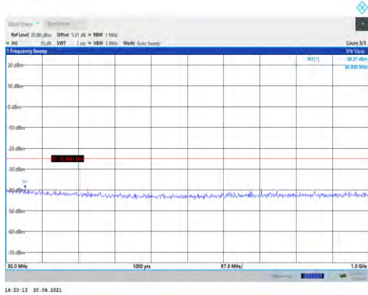
Band38-15MHz-16QAM-37825-1RB#0- Range1:30~1000MHz
