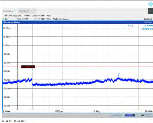
Band41-15MHz-QPSK-41165-1RB#0- Range3:3000~26000MHz
