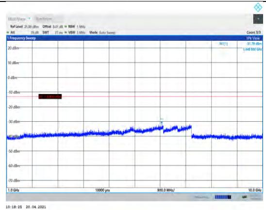
Band26-1.4MHz-16QAM-26740-1RB#0- Range2:1000~10000MHz
