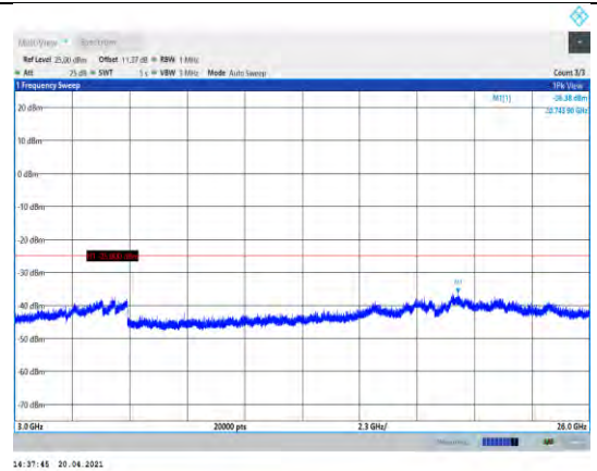
Band41-5MHz-QPSK-40740-1RB#0- Range3:3000~26000MHz
