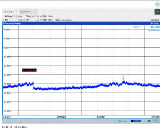
Band41-15MHz-QPSK-40315-1RB#0- Range3:3000~26000MHz
