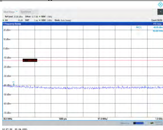
Band66-3MHz-QPSK-132657-1RB#0- Range1:30~1000MHz
