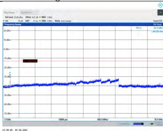
Band12-5MHz-16QAM-23035-1RB#0-Range2:1000~10000MHz
