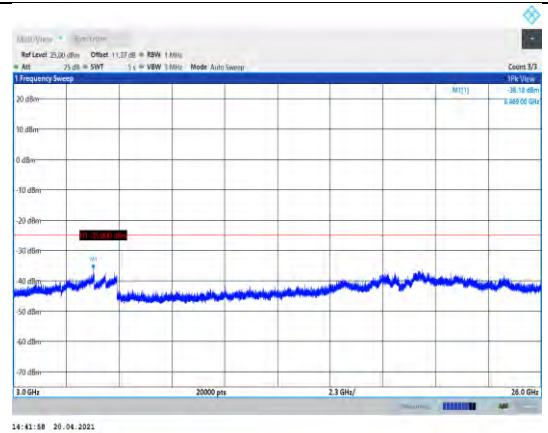
Band41-10MHz-16QAM-40290-1RB#0- Range3:3000~26000MHz
