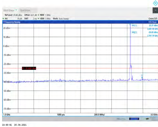
Band41-15MHz-16QAM-41165-1RB#0- Range2:1000~3000MHz
