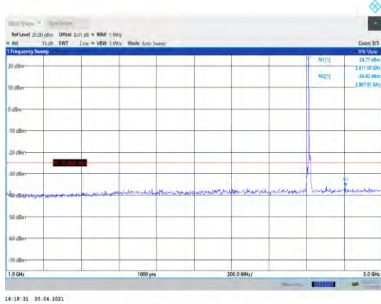
Band38-10MHz-16QAM-38200-1RB#0- Range2:1000~3000MHz
