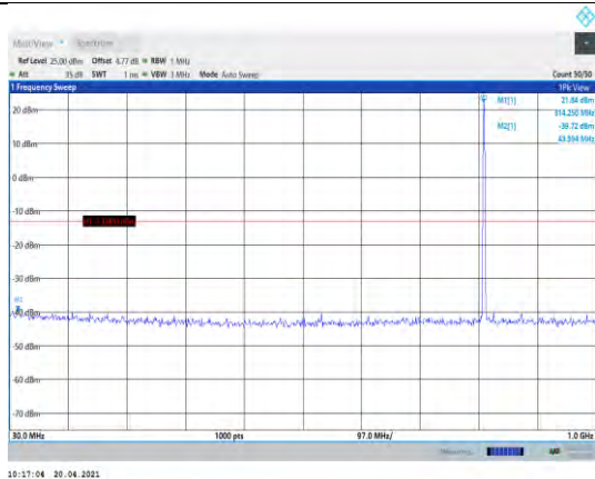
Band26-1.4MHz-QPSK-26697-1RB#0-Range1:30~1000MHz
