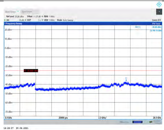
Band38-20MHz-QPSK-38000-1RB#0- Range3:3000~26000MHz
