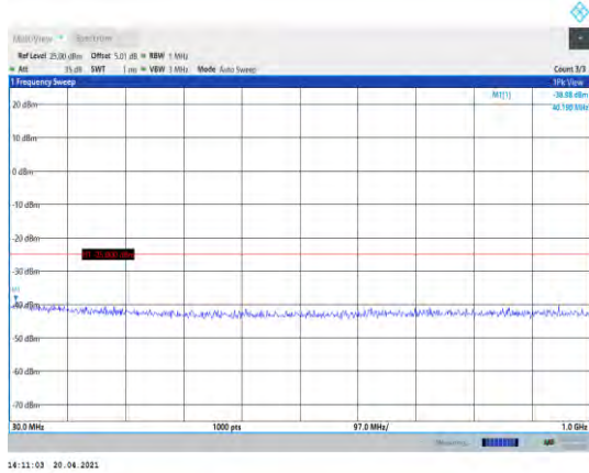
Band38-5MHz-QPSK-38000-1RB#0-Range1:30~1000MHz
