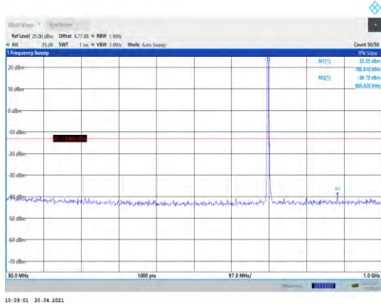
Band12-5MHz-QPSK-23095-1RB#0- Range1:30~1000MHz
