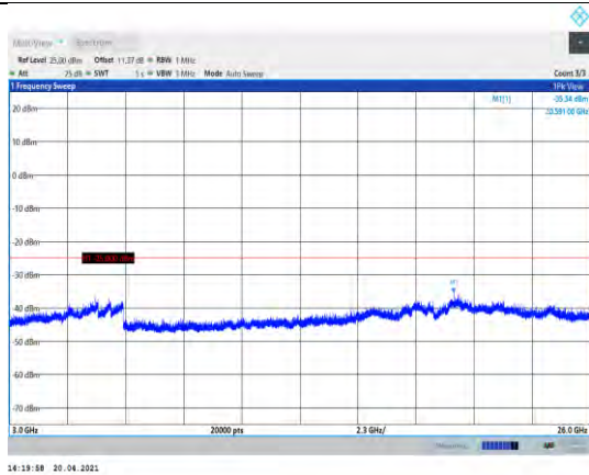
Band38-15MHz-QPSK-37825-1RB#0- Range3:3000~26000MHz
