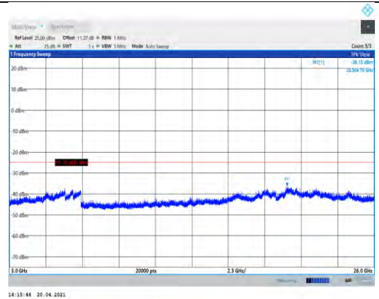
Band38-10MHz-16QAM-37800-1RB#0- Range3:3000~26000MHz
