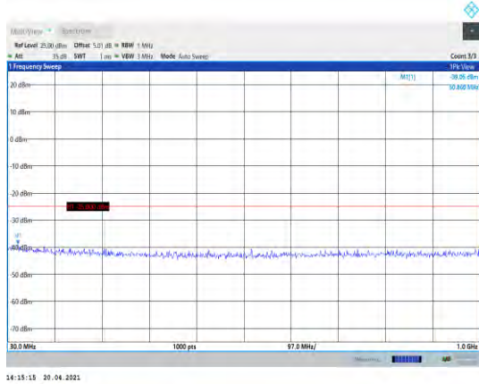
Band38-10MHz-16QAM-37800-1RB#0- Range1:30~1000MHz
