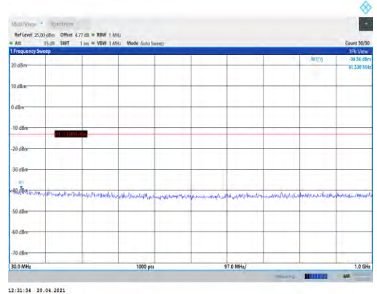
Band66-1.4MHz-16QAM-131979-1RB#0- Range1:30~1000MHz
