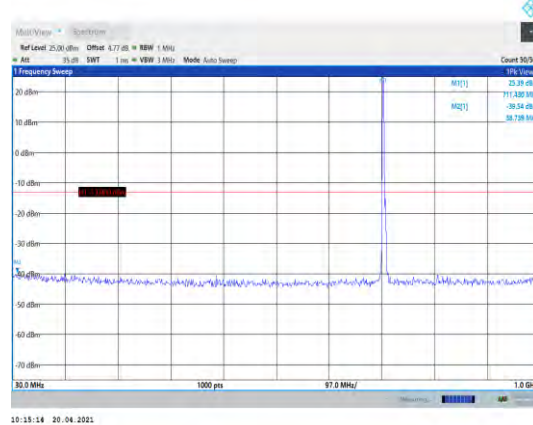
Band17-5MHz-QPSK-23825-1RB#0- Range1:30~1000MHz
