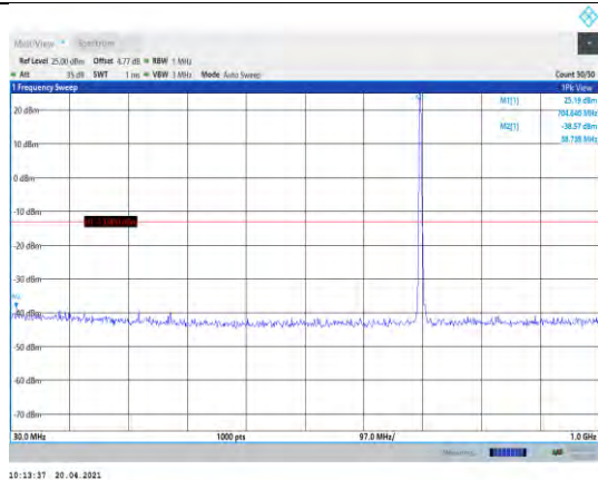
Band17-5MHz-QPSK-23755-1RB#0- Range1:30~1000MHz
