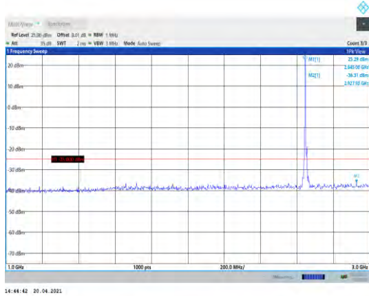
Band41-10MHz-16QAM-41190-1RB#0- Range2:1000~3000MHz
