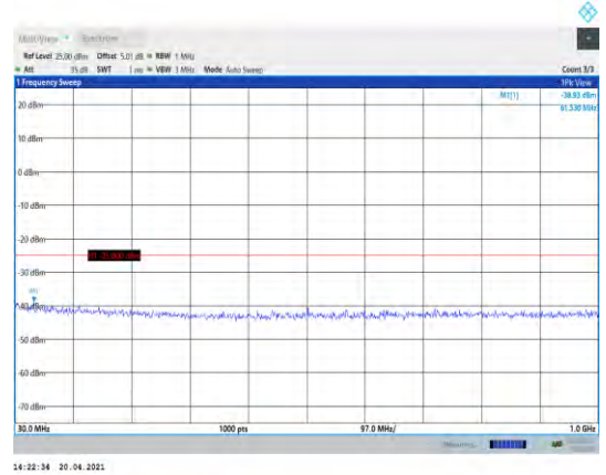
Band38-15MHz-QPSK-38175-1RB#0- Range1:30~1000MHz
