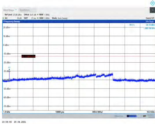
Band12-10MHz-16QAM-23060-1RB#0- Range2:1000~10000MHz
