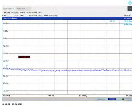
Band41-5MHz-16QAM-41215-1RB#0- Range1:30~1000MHz
