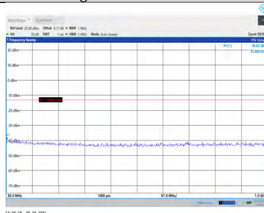
Band66-3MHz-16QAM-131987-1RB#0- Range1:30~1000MHz
