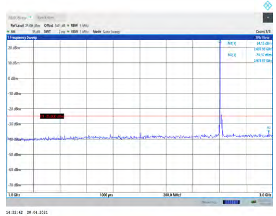
Band38-15MHz-QPSK-38175-1RB#0- Range2:1000~3000MHz
