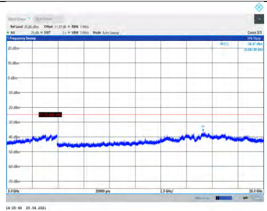
Band38-20MHz-16QAM-37850-1RB#0- Range3:3000~26000MHz
