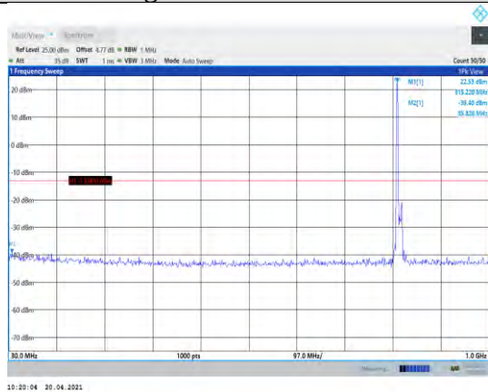
Band26-10MHz-16QAM-26740-1RB#0- Range1:30~1000MHz
