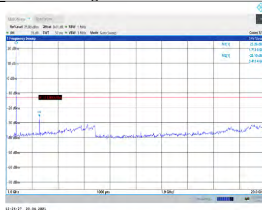
Band66-3MHz-16QAM-131987-1RB#0- Range2:1000~20000MHz
