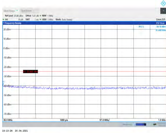
Band38-5MHz-16QAM-38225-1RB#0- Range1:30~1000MHz
