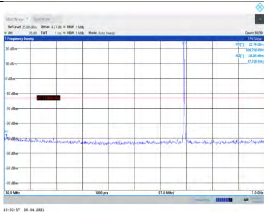
Band12-3MHz-16QAM-23025-1RB#0- Range1:30~1000MHz
