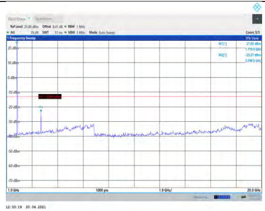
Band66-1.4MHz-16QAM-132665-1RB#0- Range2:1000~20000MHz
