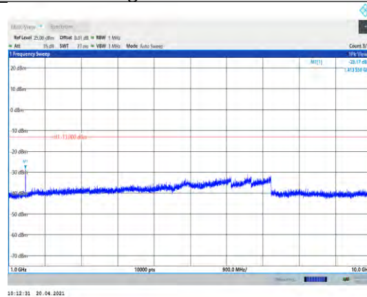
Band17-10MHz-QPSK-23800-1RB#0- Range2:1000~10000MHz
