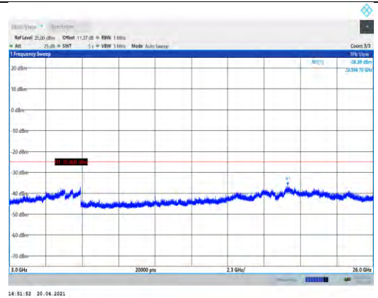
Band41-20MHz-16QAM-40340-1RB#0-Range3:3000~26000MHz
