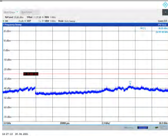
Band38-20MHz-16QAM-38000-1RB#0-Range3:3000~26000MHz
