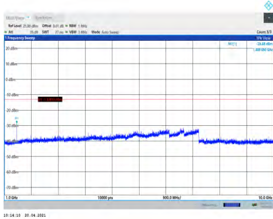
Band17-5MHz-16QAM-23755-1RB#0- Range2:1000~10000MHz
