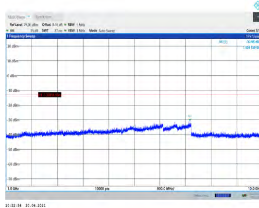
Band26-5MHz-16QAM-26765-1RB#0- Range2:1000~10000MHz
