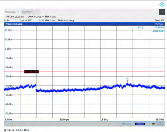
Band38-5MHz-16QAM-37775-1RB#0-Range3:3000~26000MHz
