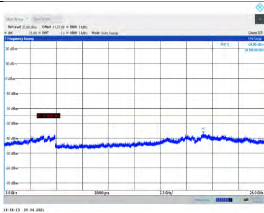
Band41-20MHz-QPSK-41140-1RB#0-Range3:3000~26000MHz
