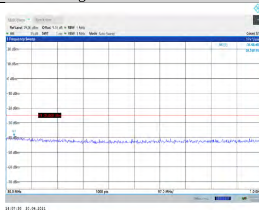
Band38-5MHz-QPSK-37775-1RB#0- Range1:30~1000MHz
