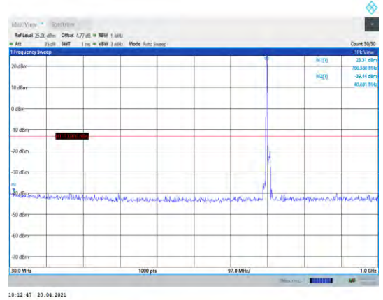
Band17-10MHz-16QAM-23800-1RB#0- Range1:30~1000MHz
