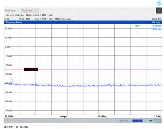
Band41-20MHz-QPSK-41140-1RB#0-Range1:30~1000MHz
