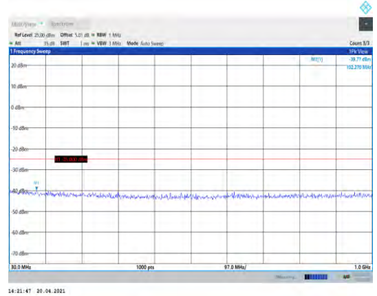
Band38-15MHz-16QAM-38000-1RB#0- Range1:30~1000MHz
