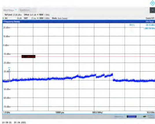
Band12-5MHz-QPSK-23035-1RB#0- Range2:1000~10000MHz
