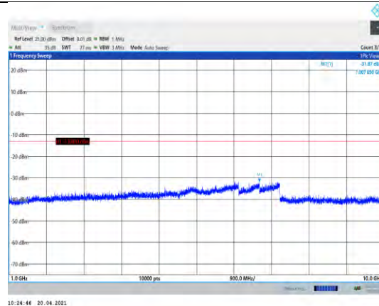
Band26-3MHz-16QAM-26740-1RB#0-Range2:1000~10000MHz
