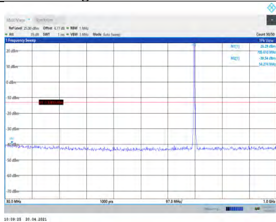
Band12-5MHz-16QAM-23095-1RB#0-Range1:30~1000MHz
