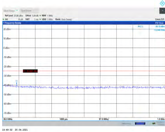
Band41-15MHz-16QAM-41165-1RB#0- Range1:30~1000MHz
