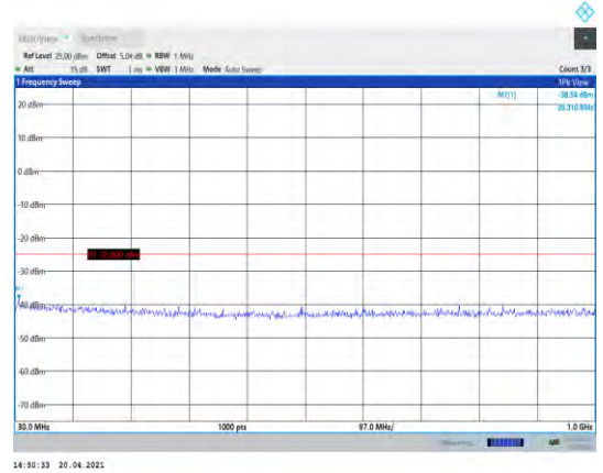
Band41-20MHz-QPSK-40340-1RB#0- Range1:30~1000MHz
