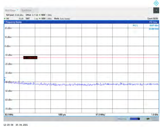
Band66-3MHz-QPSK-131987-1RB#0- Range1:30~1000MHz
