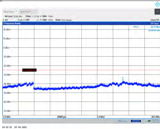
Band38-5MHz-16QAM-38000-1RB#0- Range3:3000~26000MHz
