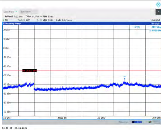
Band41-20MHz-QPSK-40340-1RB#0-Range3:3000~26000MHz
