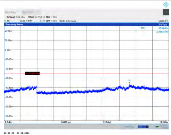
Band41-5MHz-16QAM-41215-1RB#0- Range3:3000~26000MHz
