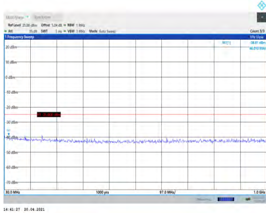
Band41-10MHz-16QAM-40290-1RB#0- Range1:30~1000MHz
