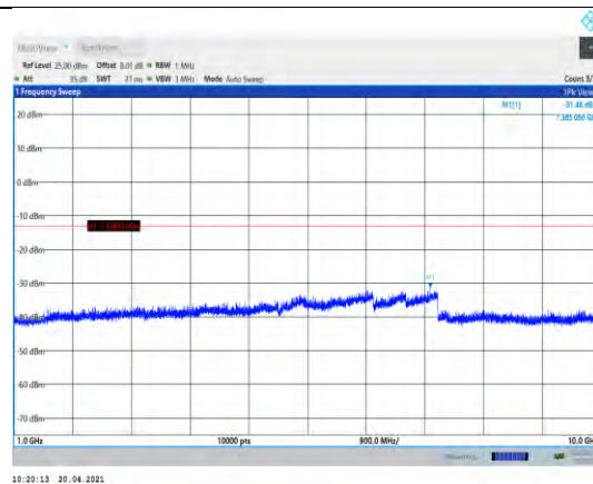
Band26-10MHz-16QAM-26740-1RB#0- Range2:1000~10000MHz
