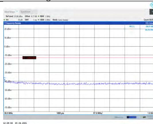
Band66-5MHz-16QAM-131997-1RB#0- Range1:30~1000MHz
