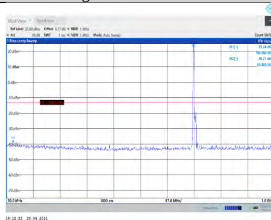
Band17-10MHz-QPSK-23800-1RB#0- Range1:30~1000MHz
