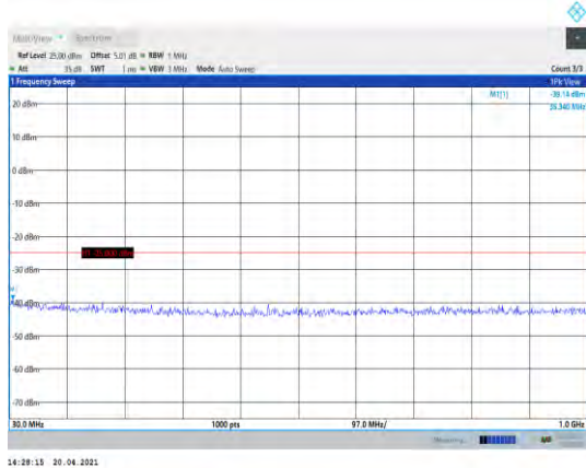
Band38-20MHz-16QAM-38150-1RB#0-Range1:30~1000MHz
