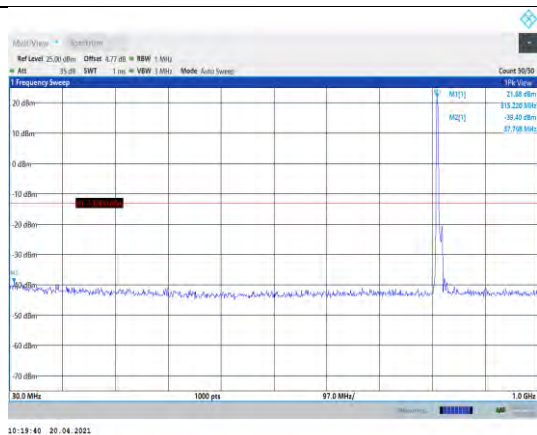
Band26-10MHz-QPSK-26740-1RB#0- Range1:30~1000MHz
