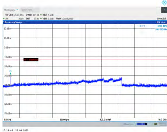
Band17-5MHz-QPSK-23755-1RB#0- Range2:1000~10000MHz
