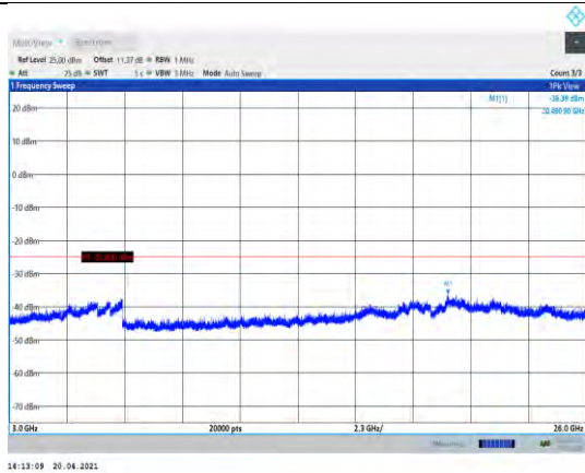
Band38-5MHz-QPSK-38225-1RB#0-Range3:3000~26000MHz
