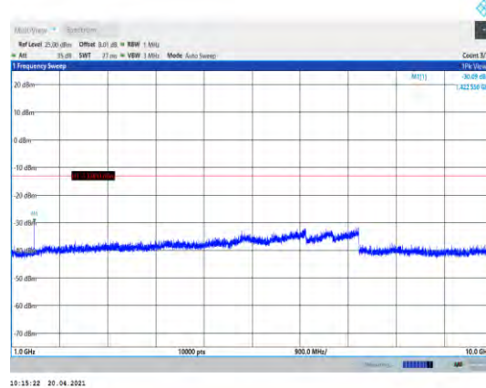
Band17-5MHz-QPSK-23825-1RB#0- Range2:1000~10000MHz
