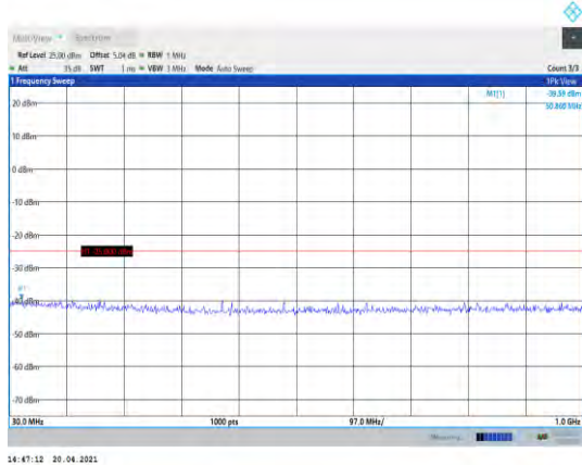
Band41-15MHz-QPSK-40740-1RB#0- Range1:30~1000MHz
