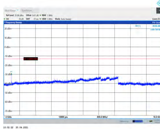
Band12-3MHz-16QAM-23165-1RB#0- Range2:1000~10000MHz
