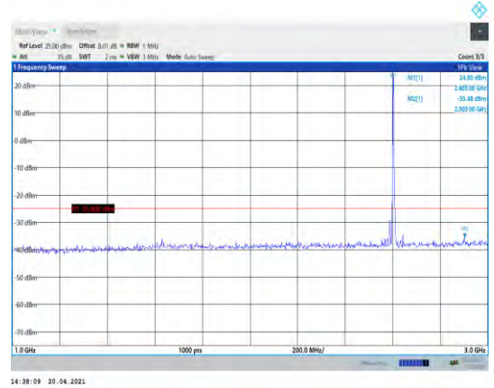
Band41-5MHz-16QAM-40740-1RB#0- Range2:1000~3000MHz
