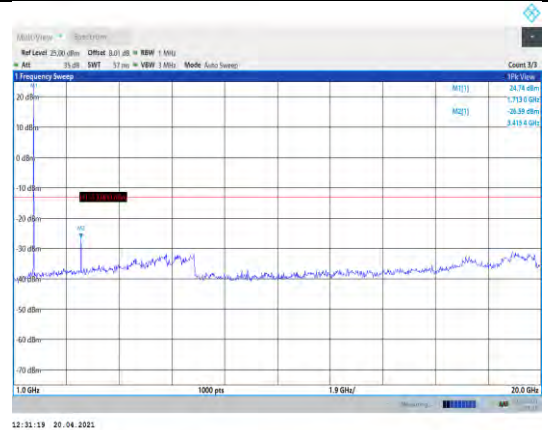
Band66-1.4MHz-QPSK-131979-1RB#0- Range2:1000~20000MHz
