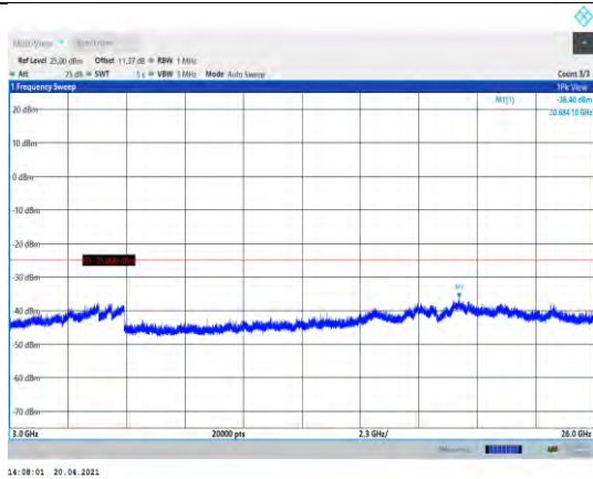
Band38-5MHz-QPSK-37775-1RB#0-Range3:3000~26000MHz
