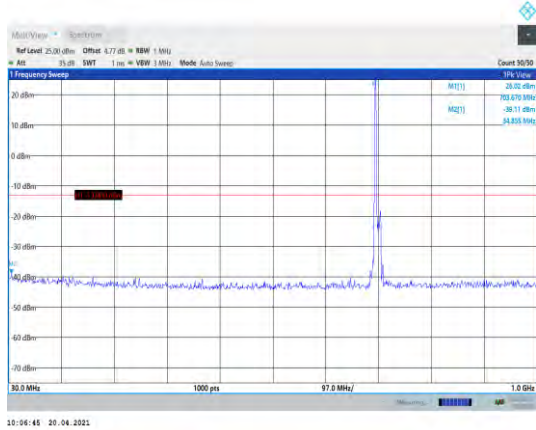
Band12-10MHz-16QAM-23095-1RB#0- Range1:30~1000MHz
