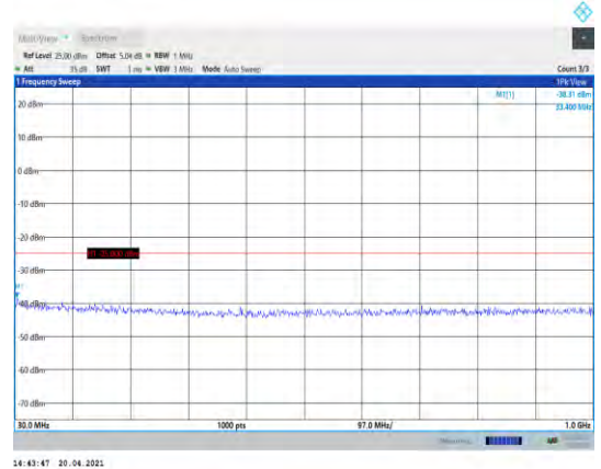
Band41-10MHz-QPSK-41190-1RB#0- Range1:30~1000MHz
