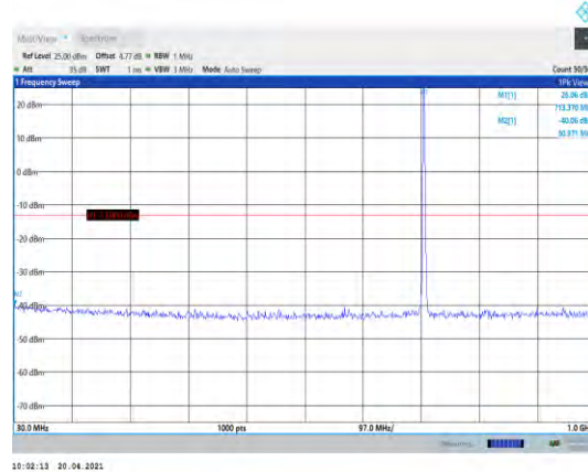
Band12-3MHz-16QAM-23165-1RB#0- Range1:30~1000MHz
