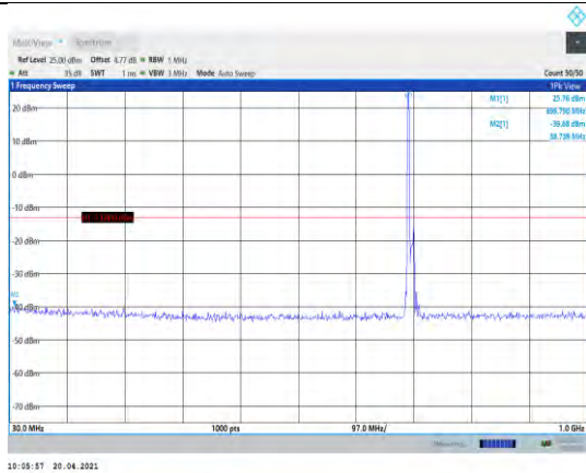
Band12-10MHz-16QAM-23060-1RB#0- Range1:30~1000MHz
