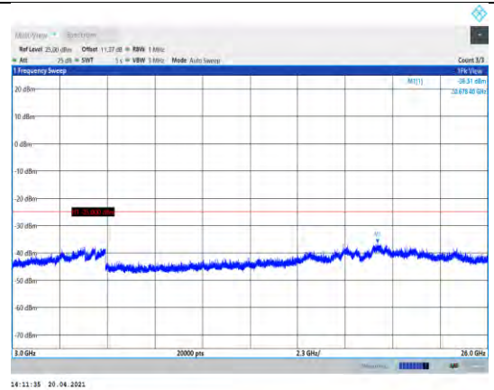
Band38-5MHz-QPSK-38000-1RB#0-Range3:3000~26000MHz
