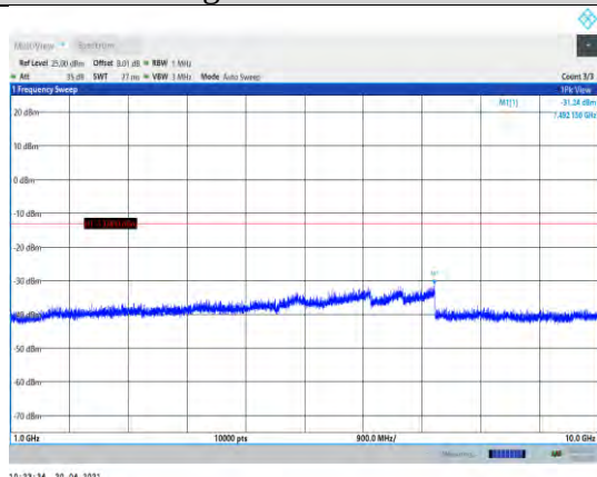
Band26-3MHz-QPSK-26705-1RB#0- Range2:1000~10000MHz
