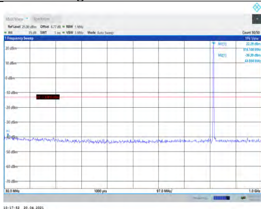
Band26-1.4MHz-QPSK-26740-1RB#0-Range1:30~1000MHz
