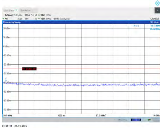
Band38-20MHz-16QAM-37850-1RB#0- Range1:30~1000MHz
