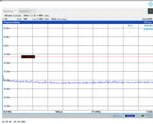
Band66-1.4MHz-16QAM-132322-1RB#0- Range1:30~1000MHz
