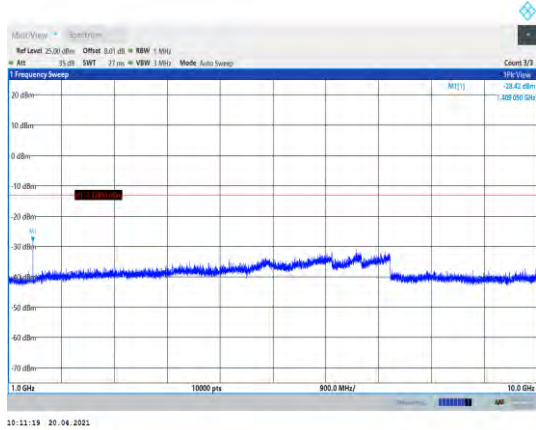
Band17-10MHz-16QAM-23780-1RB#0- Range2:1000~10000MHz
