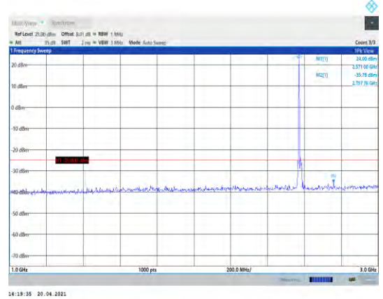
Band38-15MHz-QPSK-37825-1RB#0- Range2:1000~3000MHz
