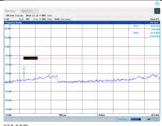
Band66-1.4MHz-16QAM-131979-1RB#0- Range2:1000~20000MHz
