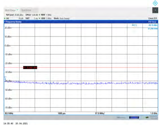
Band41-5MHz-QPSK-40265-1RB#0-Range1:30~1000MHz
