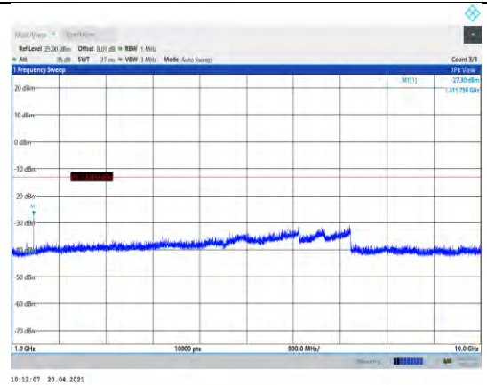
Band17-10MHz-16QAM-23790-1RB#0- Range2:1000~10000MHz
