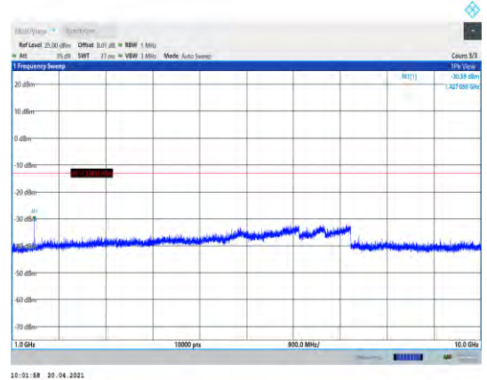
Band12-3MHz-QPSK-23165-1RB#0- Range2:1000~10000MHz
