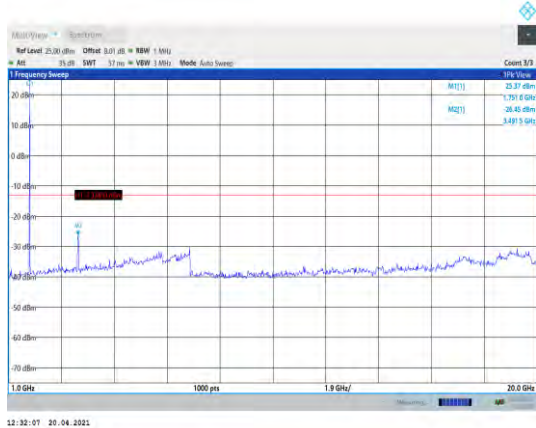
Band66-1.4MHz-QPSK-132322-1RB#0- Range2:1000~20000MHz
