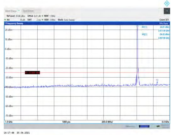
Band38-10MHz-QPSK-38200-1RB#0- Range2:1000~3000MHz
