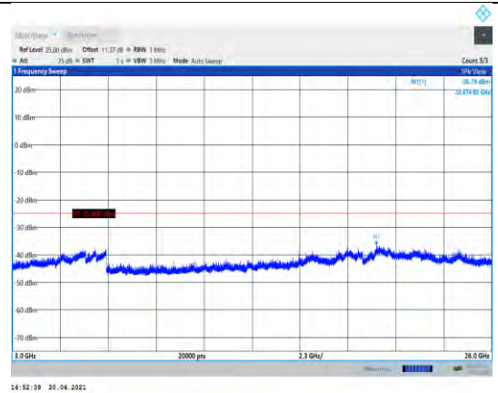
Band41-20MHz-QPSK-40740-1RB#0-Range3:3000~26000MHz
