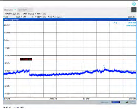
Band41-10MHz-QPSK-40740-1RB#0- Range3:3000~26000MHz
