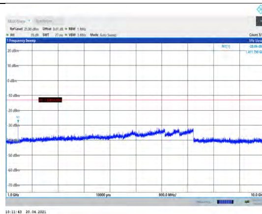
Band17-10MHz-QPSK-23790-1RB#0- Range2:1000~10000MHz
