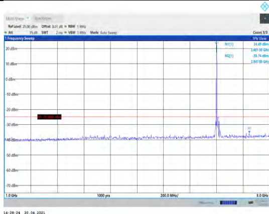
Band38-20MHz-16QAM-38150-1RB#0-Range2:1000~3000MHz
