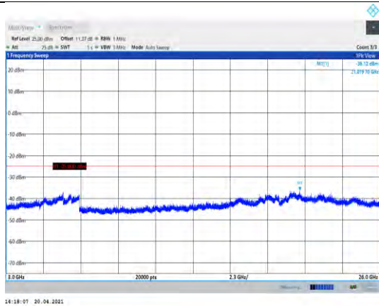
Band38-10MHz-QPSK-38200-1RB#0- Range3:3000~26000MHz
