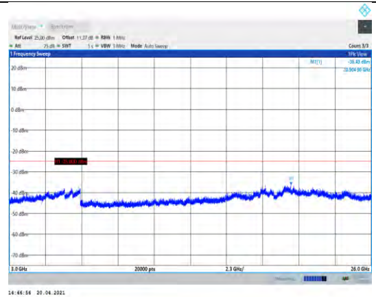
Band41-15MHz-16QAM-40315-1RB#0- Range3:3000~26000MHz
