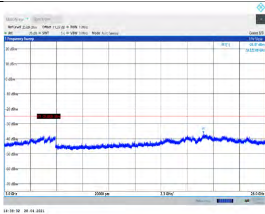
Band41-5MHz-16QAM-40740-1RB#0- Range3:3000~26000MHz
