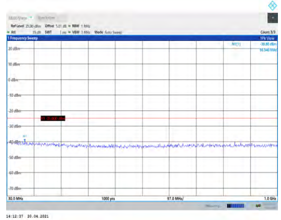
Band38-5MHz-QPSK-38225-1RB#0-Range1:30~1000MHz
