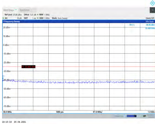
Band38-5MHz-16QAM-37775-1RB#0-Range1:30~1000MHz
