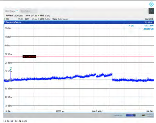
Band12-10MHz-16QAM-23095-1RB#0- Range2:1000~10000MHz
