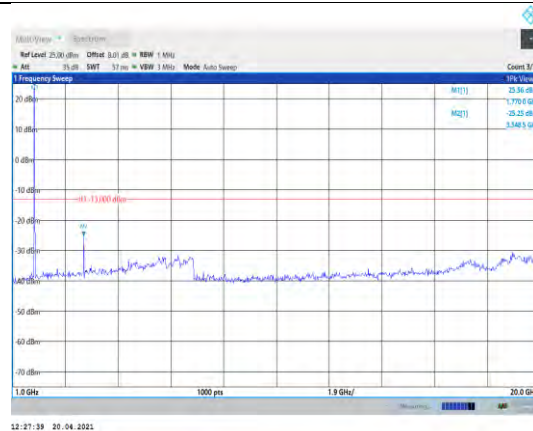
Band66-3MHz-QPSK-132657-1RB#0- Range2:1000~20000MHz
