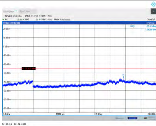
Band41-20MHz-16QAM-40740-1RB#0- Range3:3000~26000MHz
