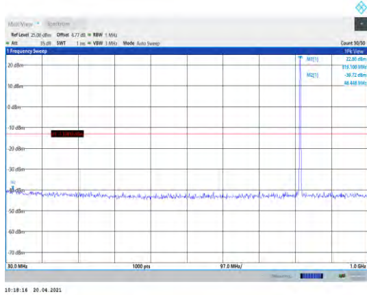
Band26-1.4MHz-16QAM-26740-1RB#0- Range1:30~1000MHz
