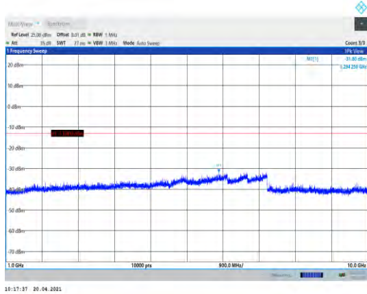
Band26-1.4MHz-16QAM-26697-1RB#0- Range2:1000~10000MHz
