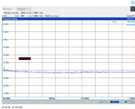
Band41-15MHz-16QAM-40315-1RB#0- Range1:30~1000MHz
