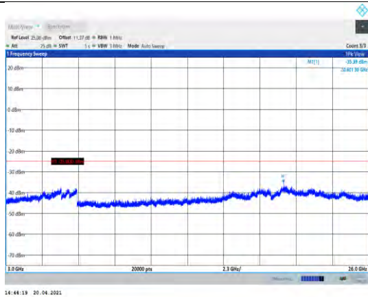
Band41-10MHz-QPSK-41190-1RB#0- Range3:3000~26000MHz
