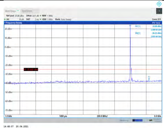
Band41-15MHz-16QAM-40740-1RB#0- Range2:1000~3000MHz
