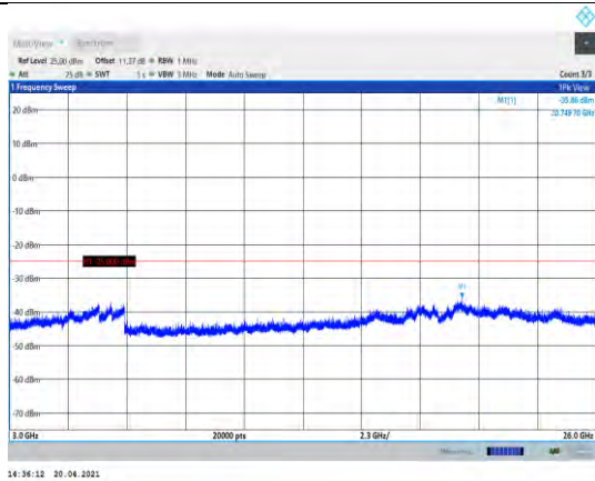
Band41-5MHz-QPSK-40265-1RB#0- Range3:3000~26000MHz
