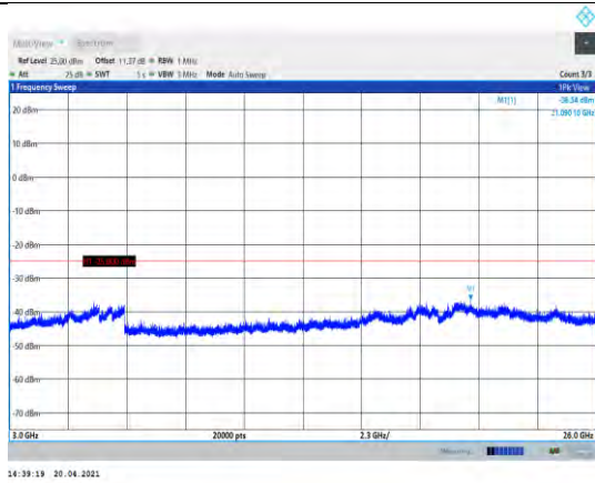
Band41-5MHz-QPSK-41215-1RB#0- Range3:3000~26000MHz
