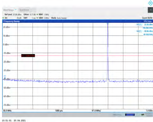
Band12-3MHz-QPSK-23095-1RB#0- Range1:30~1000MHz
