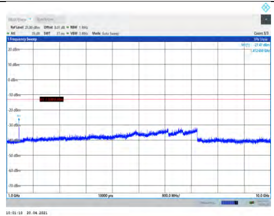
Band12-3MHz-QPSK-23095-1RB#0- Range2:1000~10000MHz
