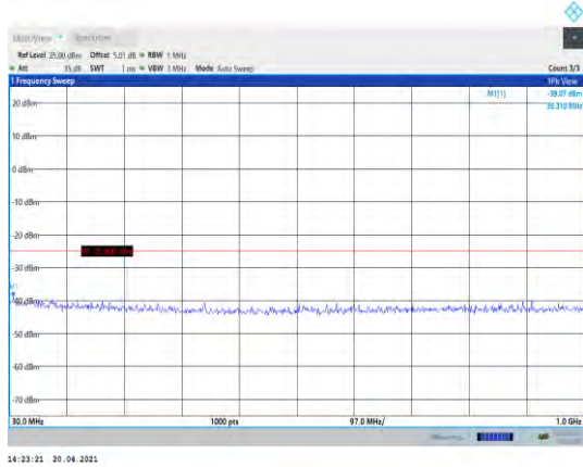
Band38-15MHz-16QAM-38175-1RB#0- Range1:30~1000MHz
