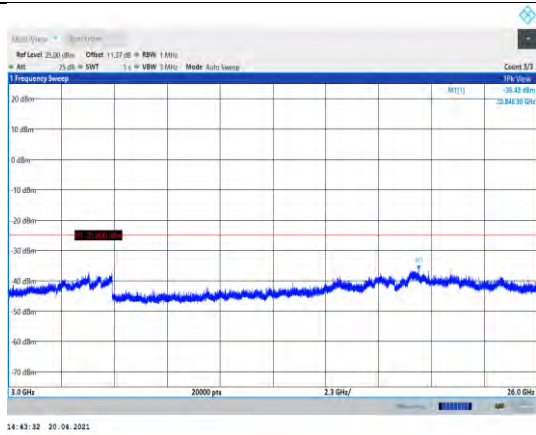
Band41-10MHz-16QAM-40740-1RB#0- Range3:3000~26000MHz
