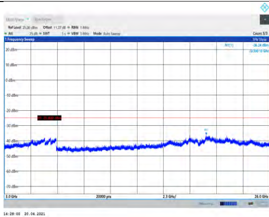
Band38-20MHz-QPSK-38150-1RB#0- Range3:3000~26000MHz
