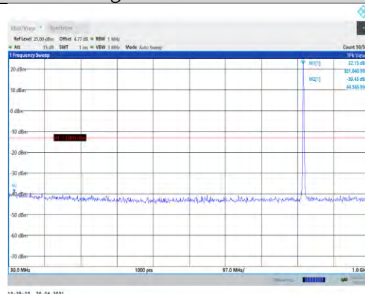
Band26-3MHz-QPSK-26775-1RB#0- Range1:30~1000MHz
