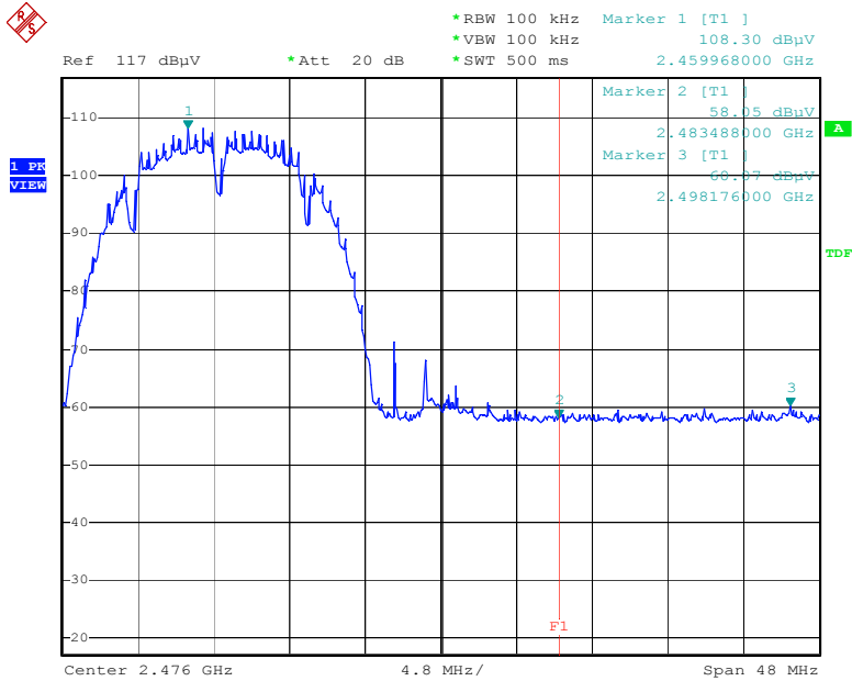
IEEE 802.11b Channel: High
