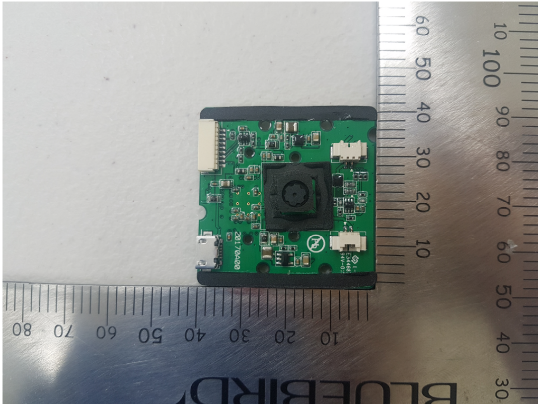
QR Module board
