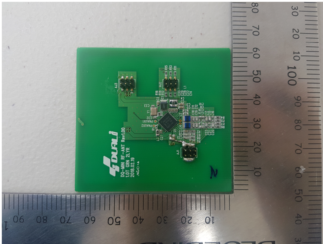
RF-ANT board
