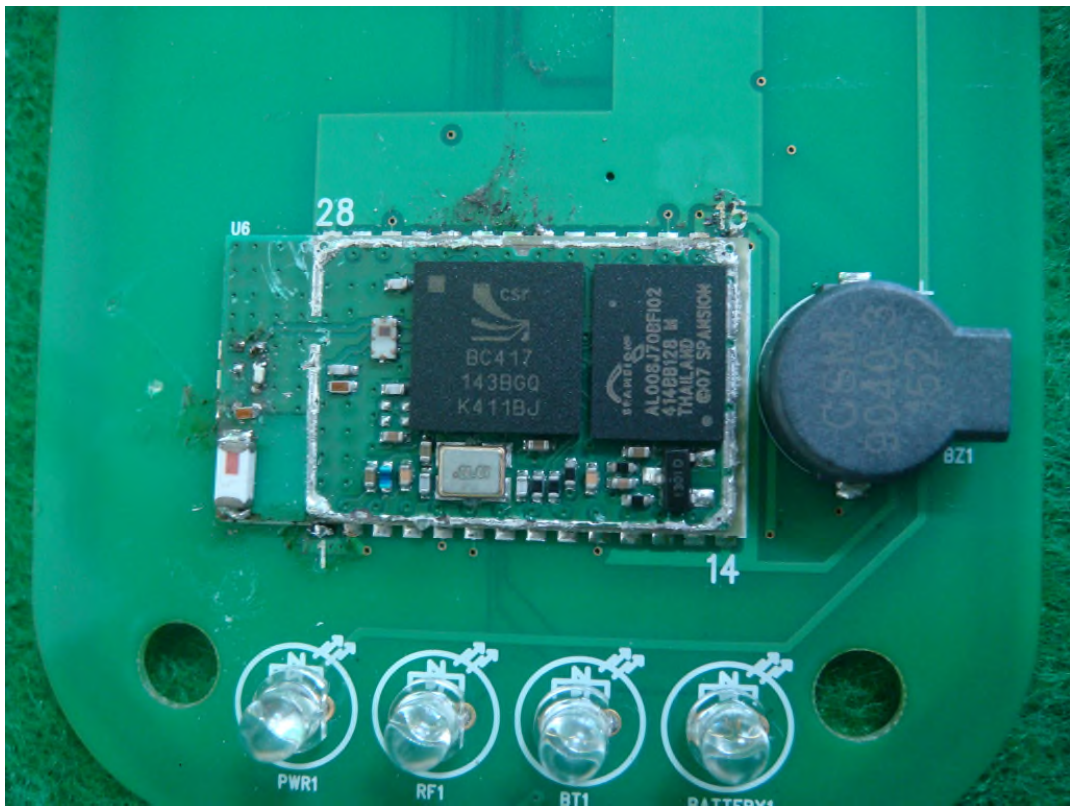
Bluetooth module (remove shield)
