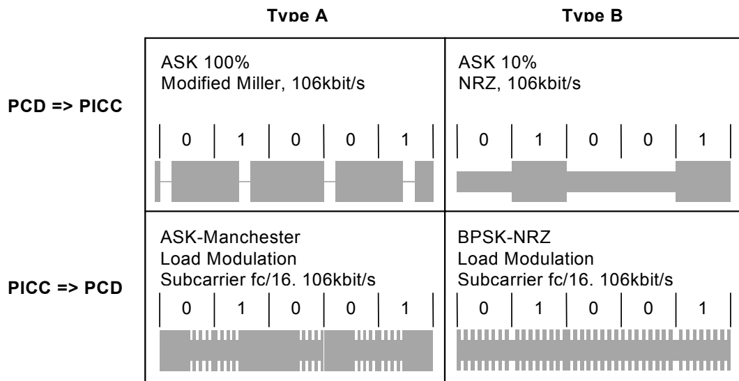
ISO-14443 Type-A/B transmission
