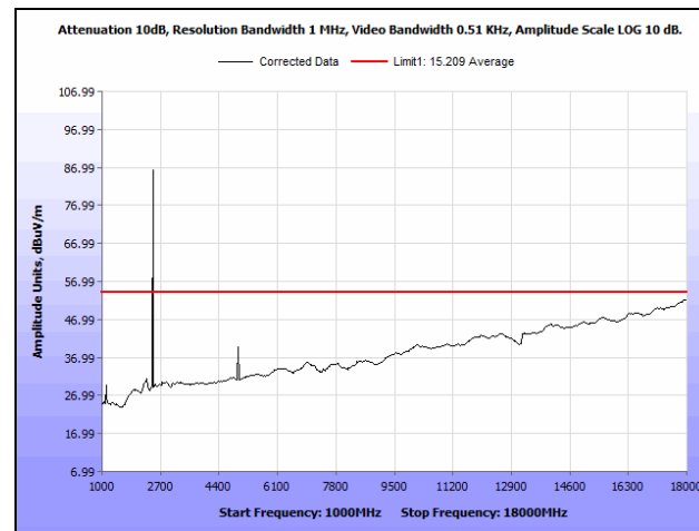
Plot 262. Radiated Spurious Emissions, High Channel, 5 MHz, 24 dBi Antenna, 1 GHz - 18 GHz, Average
