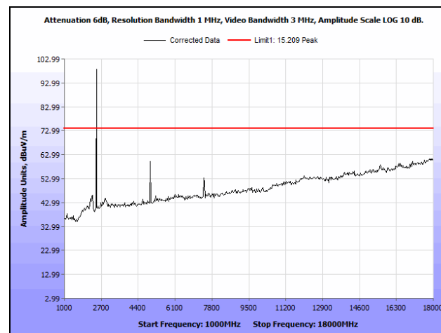
Plot 254. Radiated Spurious Emissions, High Channel, 3.5 MHz, 24 dBi Antenna, 1 GHz - 18 GHz, Peak
