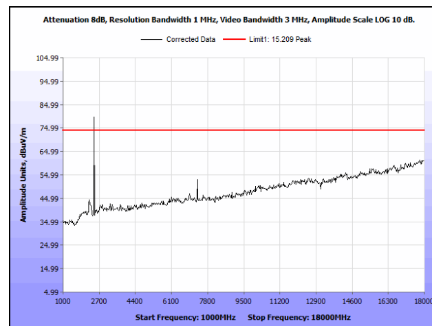
Plot 188. Radiated Spurious Emissions, Mid Channel, 7 MHz, 6 dBi Antenna, 1 GHz - 18 GHz, Peak
