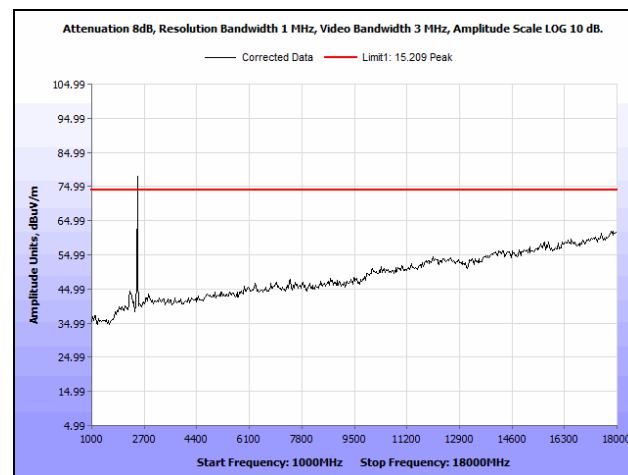
Plot 218. Radiated Spurious Emissions, High Channel, 20 MHz, 6 dBi Antenna, 1 GHz - 18 GHz, Peak
