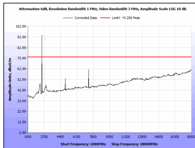
Plot 251. Radiated Spurious Emissions, Mid Channel, 3.5 MHz, 24 dBi Antenna, 1 GHz - 18 GHz, Peak
