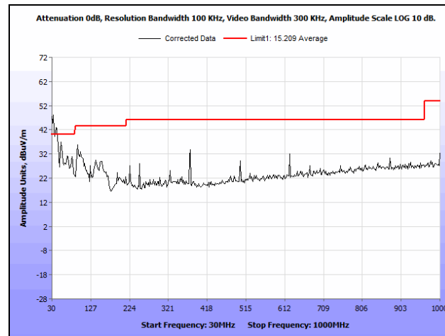
Plot 168. Radiated Spurious Emissions, Mid Channel, 3.5 MHz, 6 dBi Antenna, 30 MHz - 1 GHz
