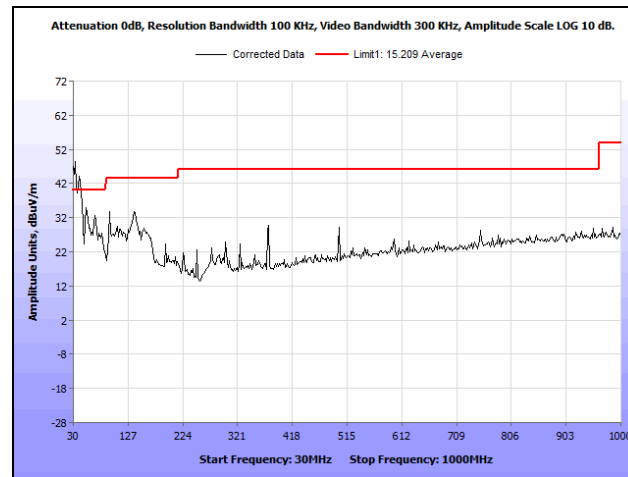
Plot 186. Radiated Spurious Emissions, Mid Channel, 7 MHz, 6 dBi Antenna, 30 MHz - 1 GHz
