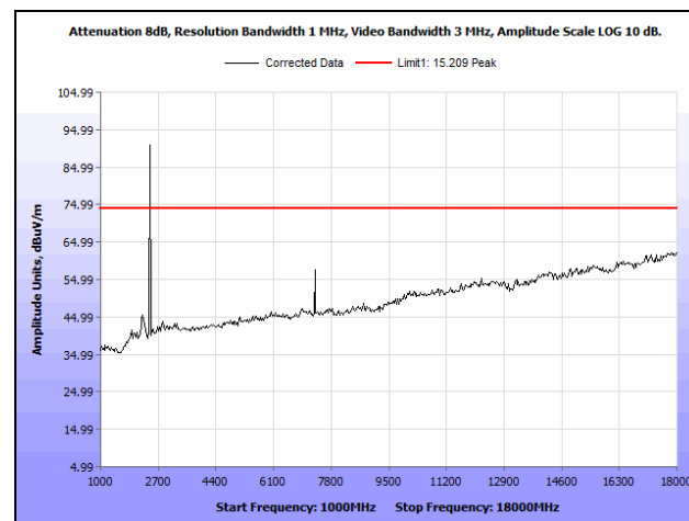
Plot 170. Radiated Spurious Emissions, Mid Channel, 3.5 MHz, 6 dBi Antenna, 1 GHz - 18 GHz, Peak
