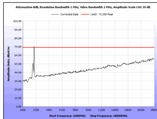
Plot 242. Radiated Spurious Emissions, Mid Channel, 40 MHz, 6 dBi Antenna, 1 GHz - 18 GHz, Peak
