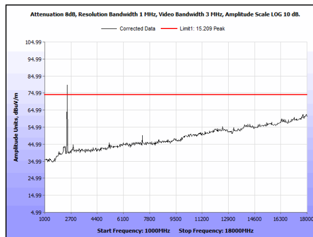
Plot 206. Radiated Spurious Emissions, Mid Channel, 14 MHz, 6 dBi Antenna, 1 GHz - 18 GHz, Peak
