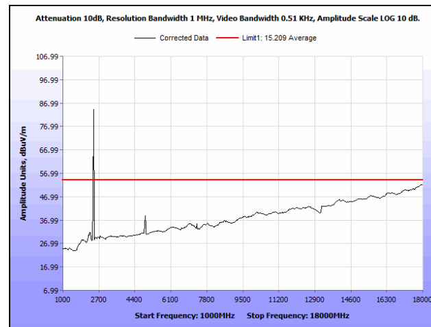
Plot 295. Radiated Spurious Emissions, Mid Channel, 20 MHz, 24 dBi Antenna, 1 GHz - 18 GHz, Average
