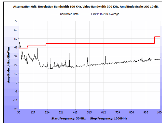
Plot 261. Radiated Spurious Emissions, High Channel, 5 MHz, 24 dBi Antenna, 30 MHz - 1 GHz
