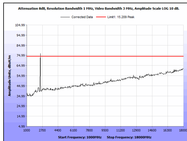
Plot 227. Radiated Spurious Emissions, High Channel, 28 MHz, 6 dBi Antenna, 1 GHz - 18 GHz, Peak
