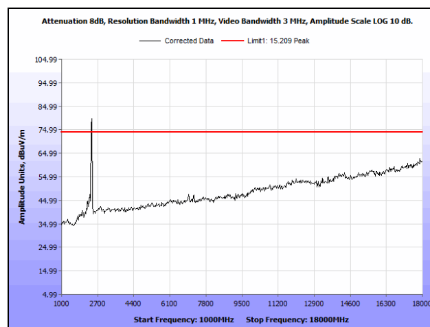
Plot 212. Radiated Spurious Emissions, Low Channel, 20 MHz, 6 dBi Antenna, 1 GHz - 18 GHz, Peak
