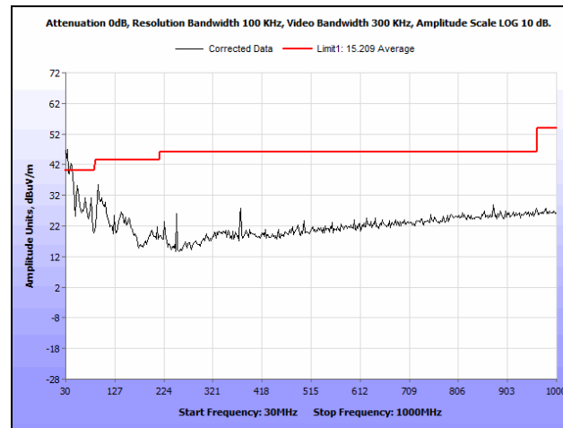
Plot 270. Radiated Spurious Emissions, High Channel, 7 MHz, 24 dBi Antenna, 30 MHz - 1 GHz
