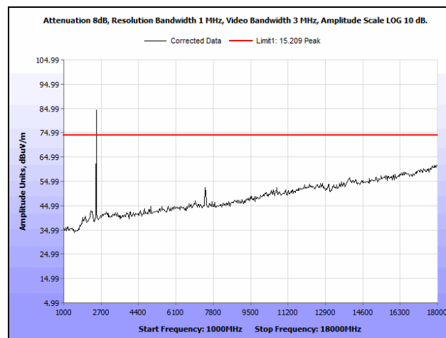
Plot 182. Radiated Spurious Emissions, High Channel, 5 MHz, 6 dBi Antenna, 1 GHz - 18 GHz, Peak
