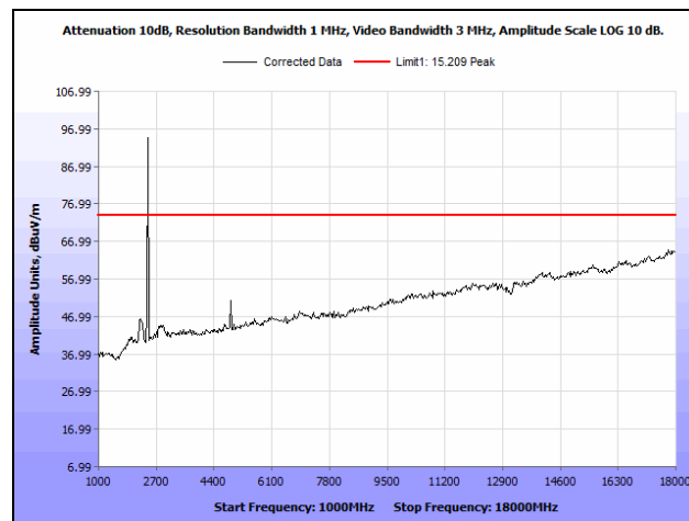
Plot 278. Radiated Spurious Emissions, Mid Channel, 10 MHz, 24 dBi Antenna, 1 GHz - 18 GHz, Peak
