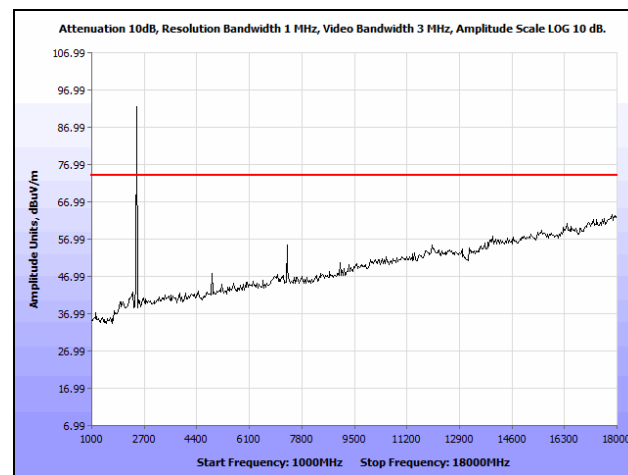
Plot 287. Radiated Spurious Emissions, Mid Channel, 14 MHz, 24 dBi Antenna, 1 GHz - 18 GHz, Peak
