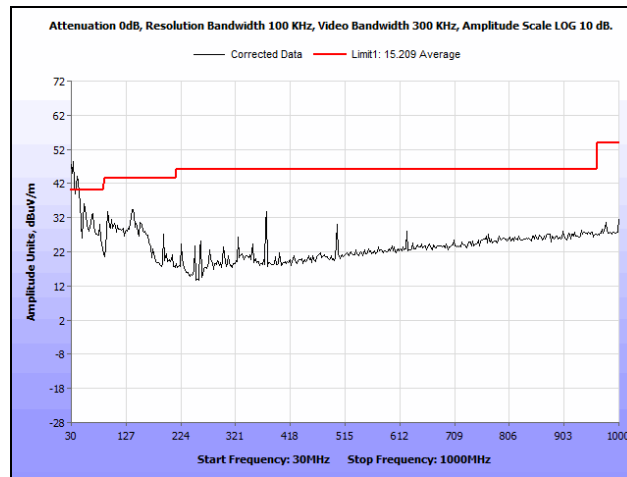
Plot 171. Radiated Spurious Emissions, High Channel, 3.5 MHz, 6 dBi Antenna, 30 MHz - 1 GHz
