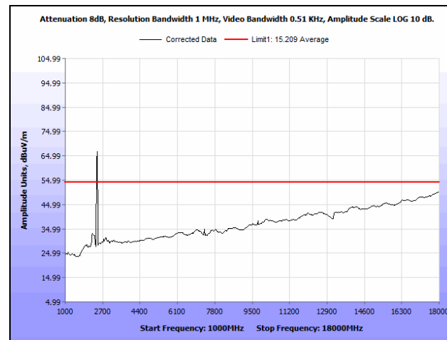
Plot 223. Radiated Spurious Emissions, Mid Channel, 28 MHz, 6 dBi Antenna, 1 GHz - 18 GHz, Average
