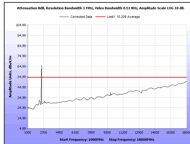
Plot 235. Radiated Spurious Emissions, High Channel, 30 MHz, 6 dBi Antenna, 1 GHz - 18 GHz, Average
