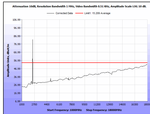
Plot 286. Radiated Spurious Emissions, Mid Channel, 14 MHz, 24 dBi Antenna, 1 GHz - 18 GHz, Average
