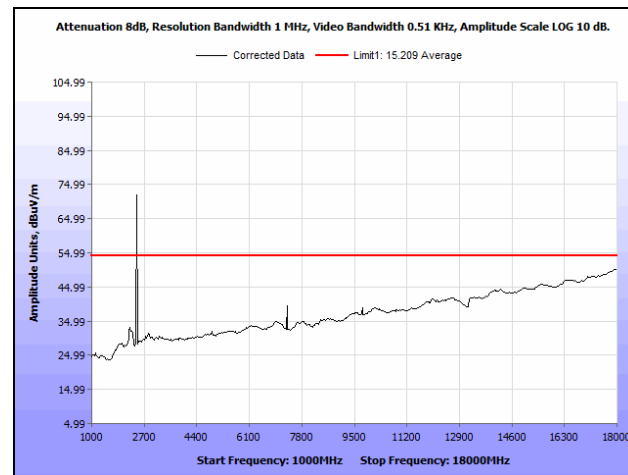
Plot 169. Radiated Spurious Emissions, Mid Channel, 3.5 MHz, 6 dBi Antenna, 1 GHz - 18 GHz, Average
