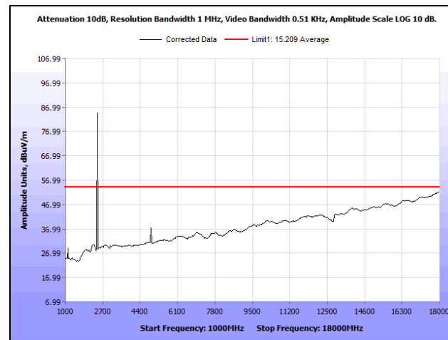
Plot 268. Radiated Spurious Emissions, Mid Channel, 7 MHz, 24 dBi Antenna, 1 GHz - 18 GHz, Average
