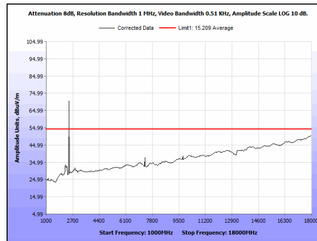
Plot 187. Radiated Spurious Emissions, Mid Channel, 7 MHz, 6 dBi Antenna, 1 GHz - 18 GHz, Average
