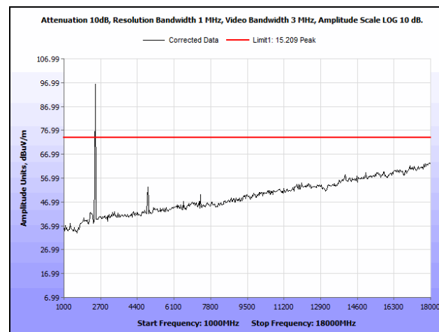
Plot 296. Radiated Spurious Emissions, Mid Channel, 20 MHz, 24 dBi Antenna, 1 GHz - 18 GHz, Peak
