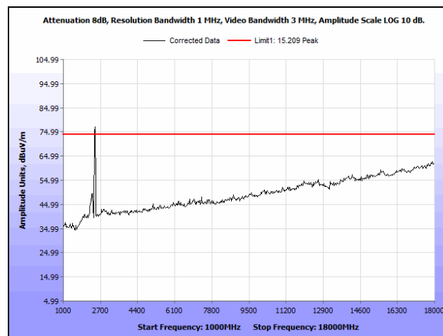
Plot 233. Radiated Spurious Emissions, Mid Channel, 30 MHz, 6 dBi Antenna, 1 GHz - 18 GHz, Peak
