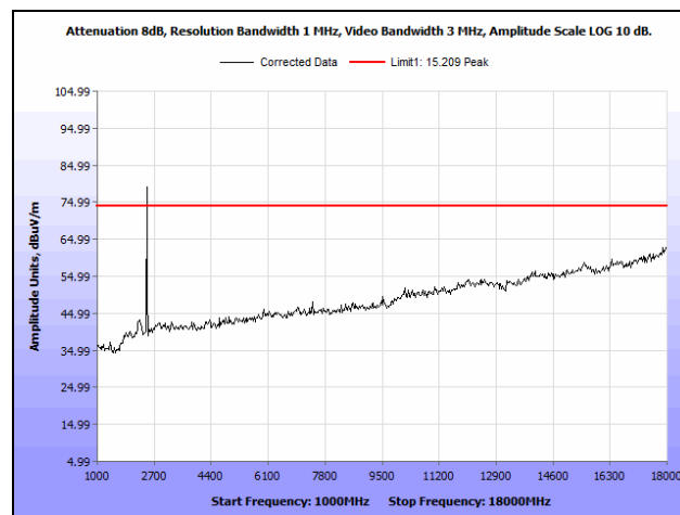
Plot 209. Radiated Spurious Emissions, High Channel, 14 MHz, 6 dBi Antenna, 1 GHz - 18 GHz, Peak
