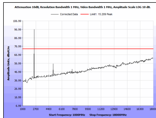
Plot 263. Radiated Spurious Emissions, High Channel, 5 MHz, 24 dBi Antenna, 1 GHz - 18 GHz, Peak
