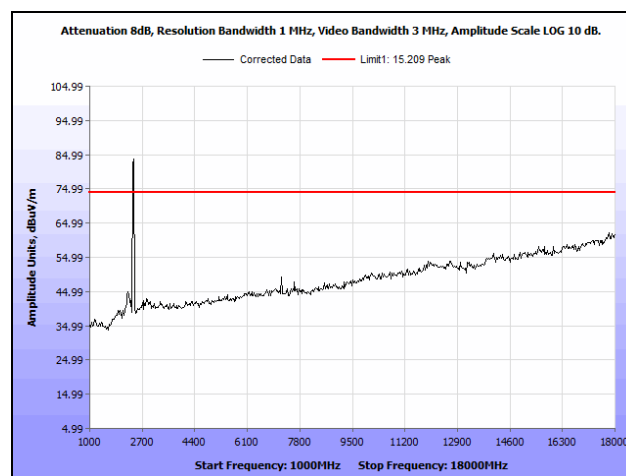
Plot 185. Radiated Spurious Emissions, Low Channel, 7 MHz, 6 dBi Antenna, 1 GHz - 18 GHz, Peak
