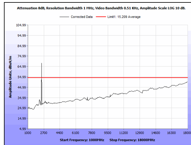
Plot 214. Radiated Spurious Emissions, Mid Channel, 20 MHz, 6 dBi Antenna, 1 GHz - 18 GHz, Average
