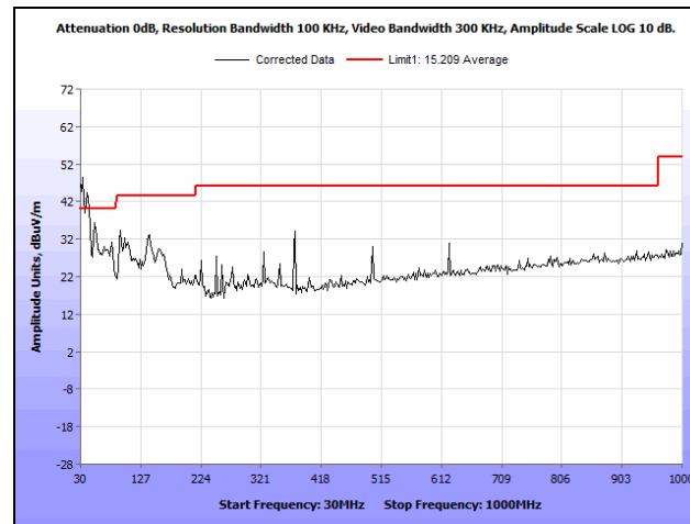
Plot 285. Radiated Spurious Emissions, Mid Channel, 14 MHz, 24 dBi Antenna, 30 MHz - 1 GHz
