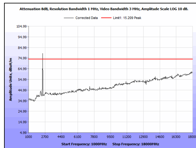
Plot 215. Radiated Spurious Emissions, Mid Channel, 20 MHz, 6 dBi Antenna, 1 GHz - 18 GHz, Peak
