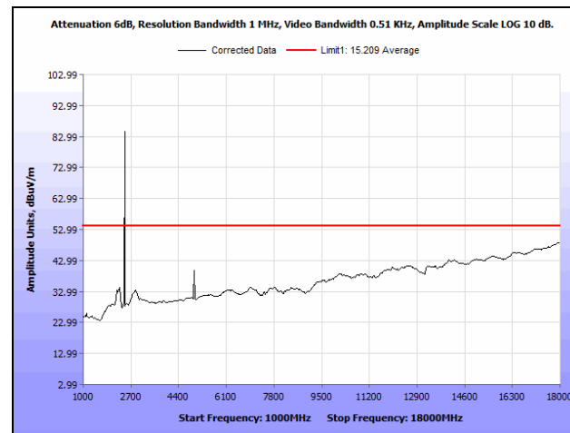
Plot 253. Radiated Spurious Emissions, High Channel, 3.5 MHz, 24 dBi Antenna, 1 GHz - 18 GHz, Average
