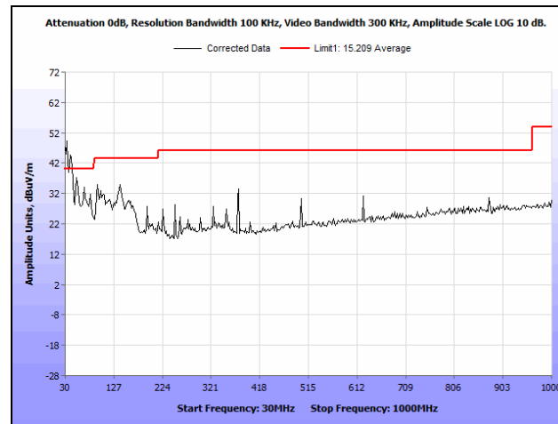
Plot 240. Radiated Spurious Emissions, Mid Channel, 40 MHz, 6 dBi Antenna, 30 MHz - 1 GHz
