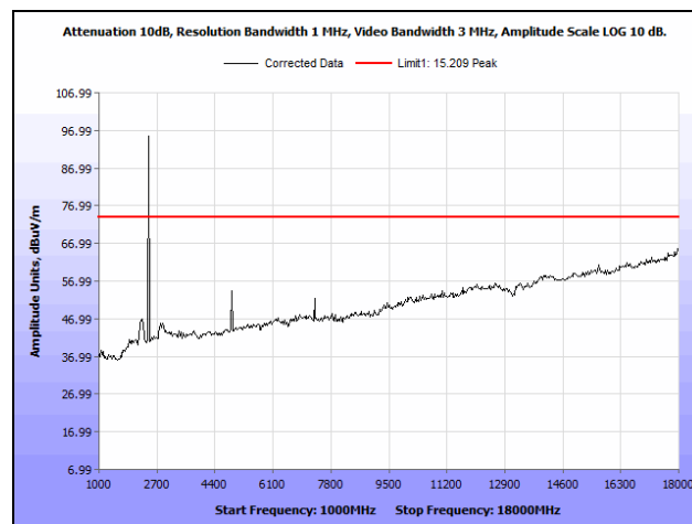
Plot 260. Radiated Spurious Emissions, Mid Channel, 5 MHz, 24 dBi Antenna, 1 GHz - 18 GHz, Peak
