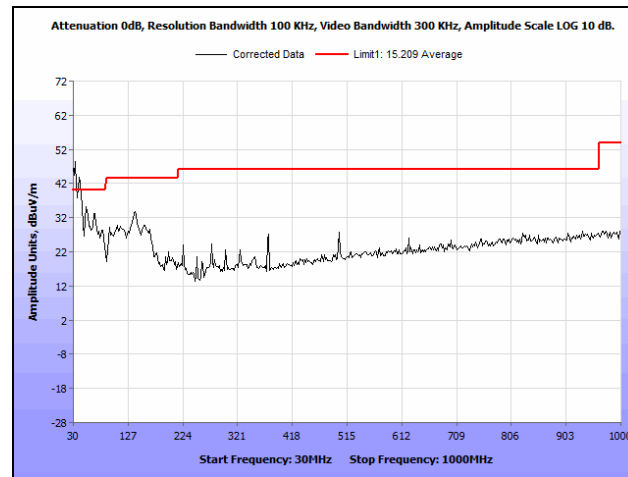
Plot 213. Radiated Spurious Emissions, Mid Channel, 20 MHz, 6 dBi Antenna, 30 MHz - 1 GHz
