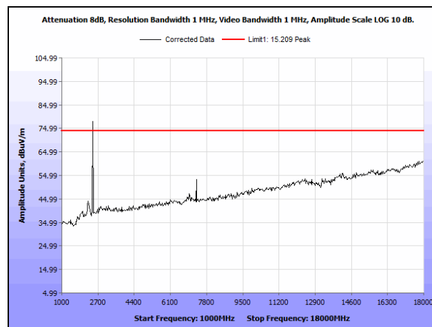
Plot 179. Radiated Spurious Emissions, Mid Channel, 5 MHz, 6 dBi Antenna, 1 GHz - 18 GHz, Peak
