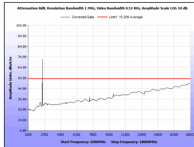
Plot 190. Radiated Spurious Emissions, High Channel, 7 MHz, 6 dBi Antenna, 1 GHz - 18 GHz, Average
