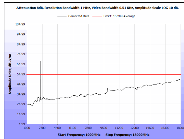
Plot 217. Radiated Spurious Emissions, High Channel, 20 MHz, 6 dBi Antenna, 1 GHz - 18 GHz, Average
