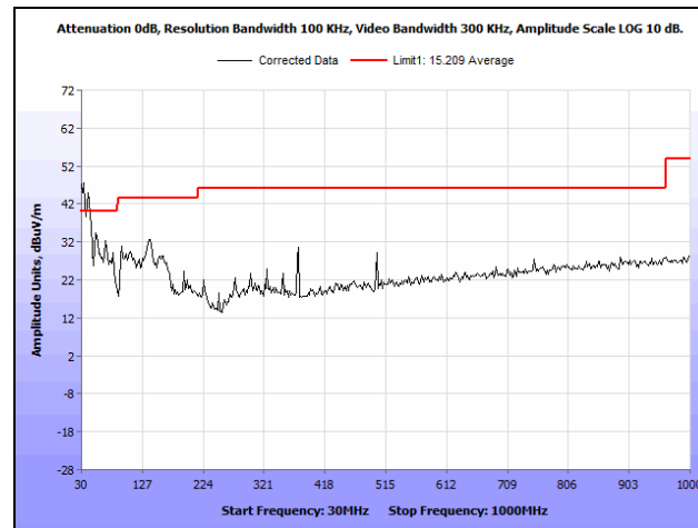
Plot 216. Radiated Spurious Emissions, High Channel, 20 MHz, 6 dBi Antenna, 30 MHz - 1 GHz
