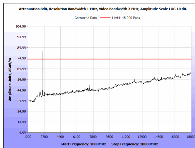
Plot 200. Radiated Spurious Emissions, High Channel, 10 MHz, 6 dBi Antenna, 1 GHz - 18 GHz, Peak
