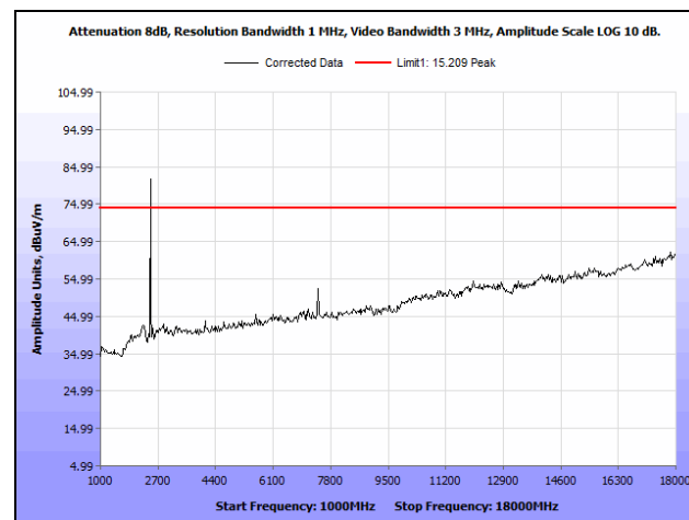
Plot 191. Radiated Spurious Emissions, High Channel, 7 MHz, 6 dBi Antenna, 1 GHz - 18 GHz, Peak
