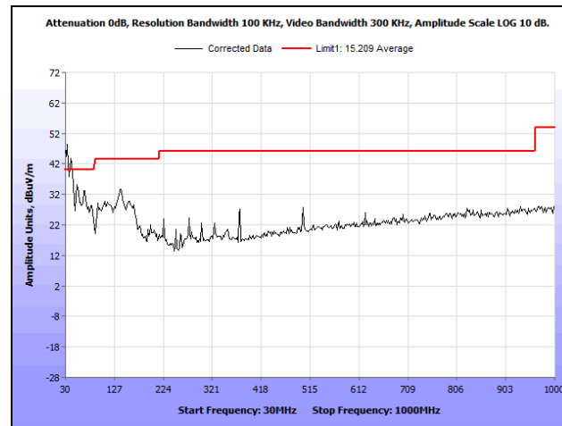
Plot 294. Radiated Spurious Emissions, Mid Channel, 20 MHz, 24 dBi Antenna, 30 MHz - 1 GHz
