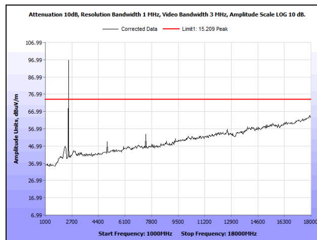
Plot 281. Radiated Spurious Emissions, High Channel, 10 MHz, 24 dBi Antenna, 1 GHz - 18 GHz, Peak
