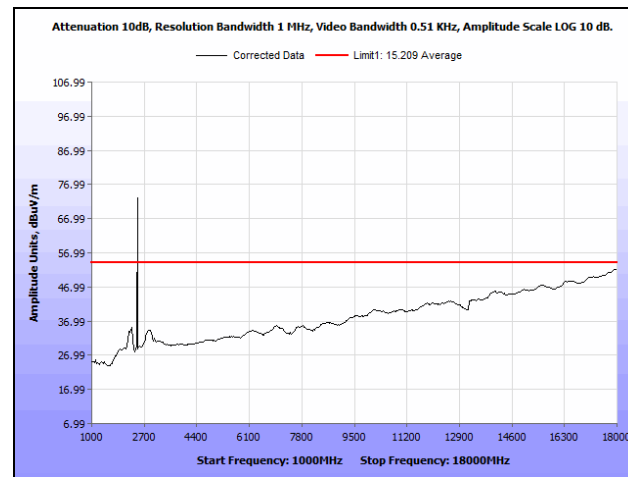
Plot 271. Radiated Spurious Emissions, High Channel, 7 MHz, 24 dBi Antenna, 1 GHz - 18 GHz, Average
