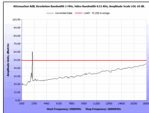
Plot 241. Radiated Spurious Emissions, Mid Channel, 40 MHz, 6 dBi Antenna, 1 GHz - 18 GHz, Average
