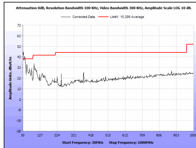
Plot 189. Radiated Spurious Emissions, High Channel, 7 MHz, 6 dBi Antenna, 30 MHz - 1 GHz
