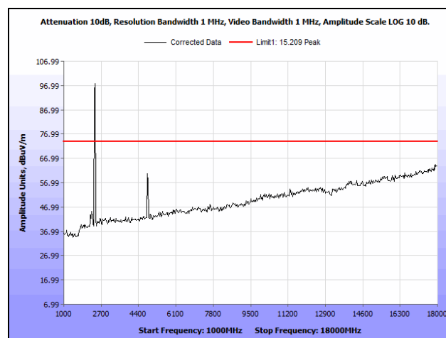
Plot 266. Radiated Spurious Emissions, Low Channel, 7 MHz, 24 dBi Antenna, 1 GHz - 18 GHz, Peak
