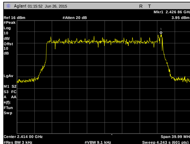
Plot 527. Peak Power Spectral Density, Low Channel, 28 MHz, Chain 0, 6 dBi Antenna
