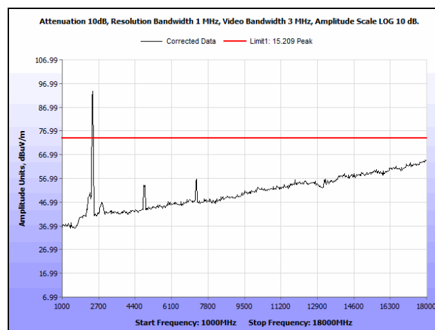
Plot 311. Radiated Spurious Emissions, Low Channel, 30 MHz, 24 dBi Antenna, 1 GHz - 18 GHz, Peak
