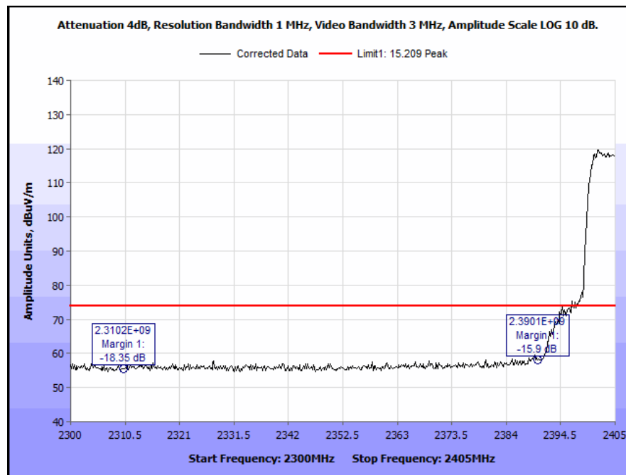
Plot 342. Radiated Restricted Band Edge, Low Channel, 10 MHz, 6 dBi Antenna, Peak
