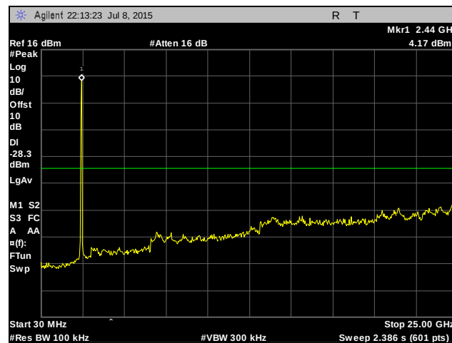
Plot 450. Conducted Spurious Emissions, Mid Channel, 40 MHz, Chain 0
