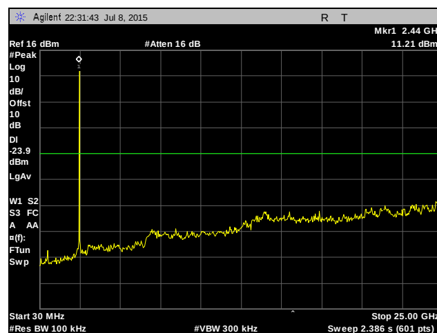
Plot 409. Conducted Spurious Emissions, High Channel, 5 MHz, Chain 0
