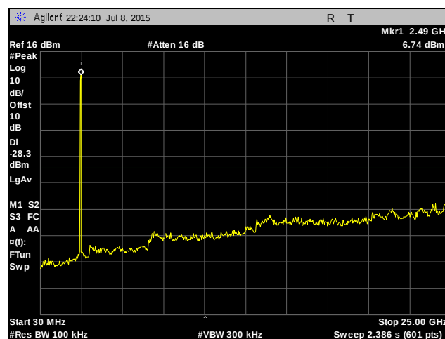
Plot 427. Conducted Spurious Emissions, High Channel, 14 MHz, Chain 0
