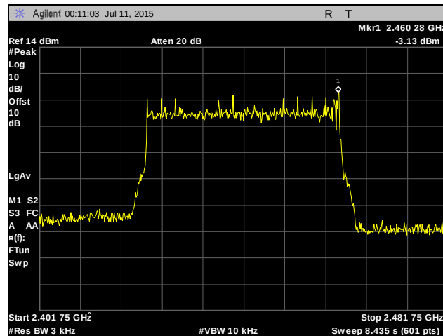
Plot 597. Peak Power Spectral Density, Mid Channel, 40 MHz, Chain 1, 24 dBi Antenna
