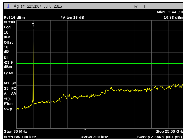
Plot 408. Conducted Spurious Emissions, Mid Channel, 5 MHz, Chain 0
