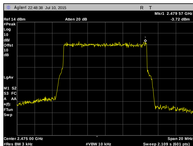
Plot 565. Peak Power Spectral Density, High Channel, 10 MHz, Chain 0, 24 dBi Antenna
