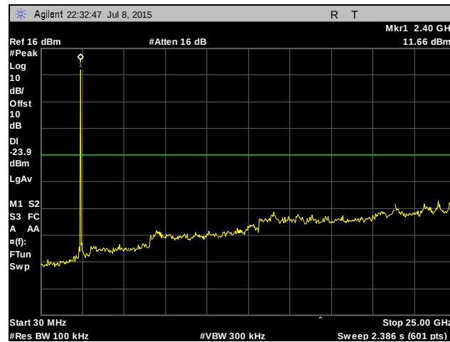
Plot 401. Conducted Spurious Emissions, Low Channel, 3.5 MHz, Chain 0
