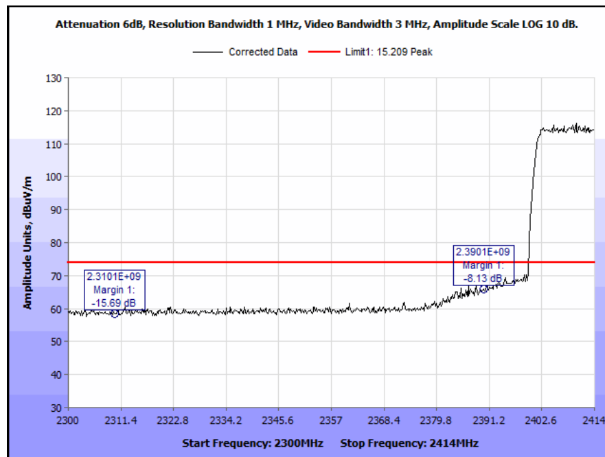
Plot 390. Radiated Restricted Band Edge, Low Channel, 28 MHz, 24 dBi Antenna, Peak
