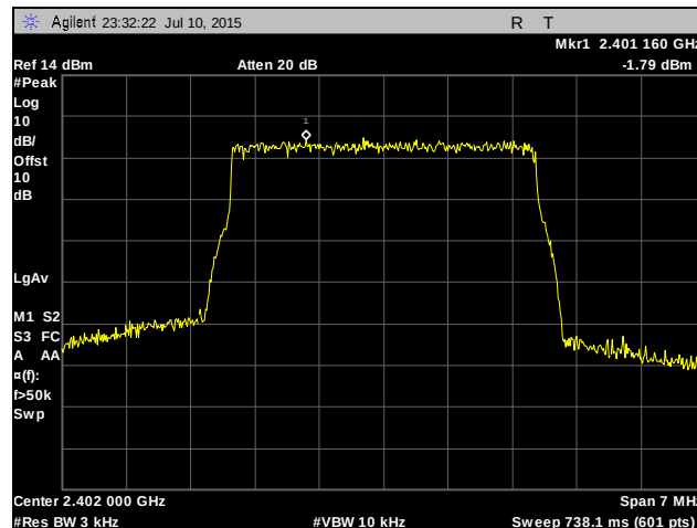
Plot 548. Peak Power Spectral Density, Low Channel, 3.5 MHz, Chain 1, 24 dBi Antenna
