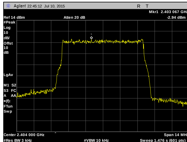
Plot 557. Peak Power Spectral Density, Low Channel, 7 MHz, Chain 0, 24 dBi Antenna
