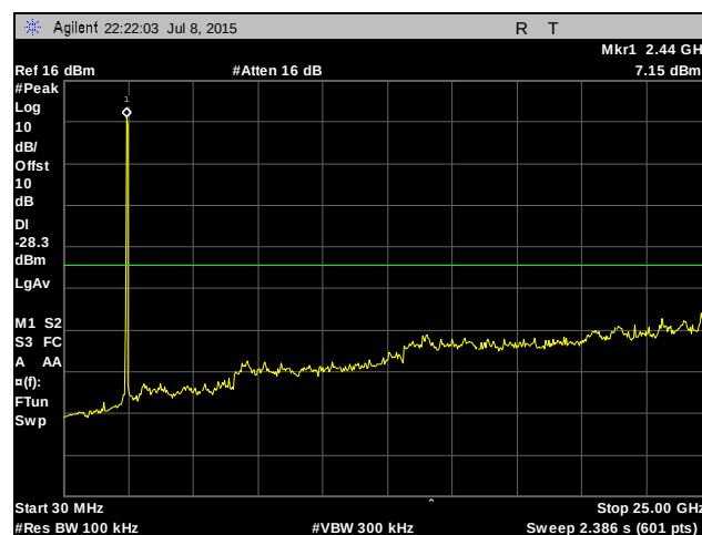
Plot 433. Conducted Spurious Emissions, High Channel, 20 MHz, Chain 0
