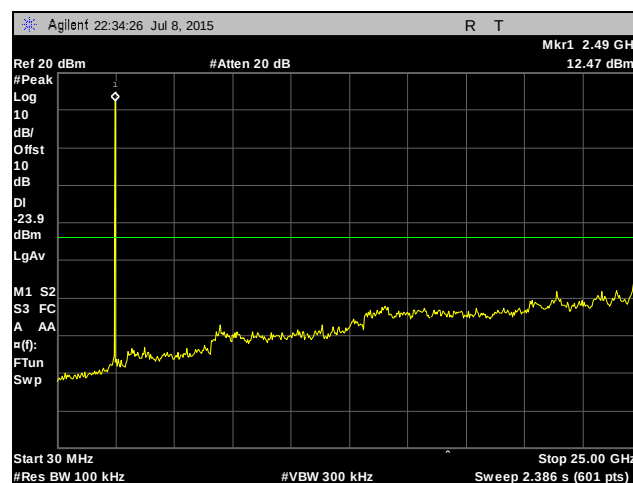
Plot 403. Conducted Spurious Emissions, High Channel, 3.5 MHz, Chain 0
