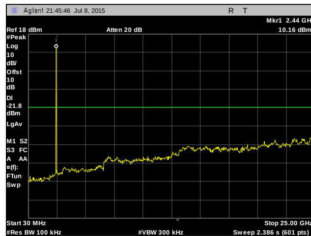
Plot 417. Conducted Spurious Emissions, Mid Channel, 7 MHz, Chain 1
