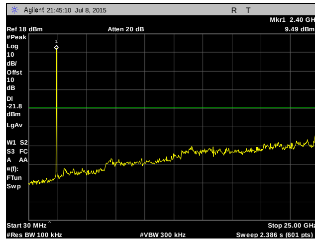
Plot 416. Conducted Spurious Emissions, Low Channel, 7 MHz, Chain 1
