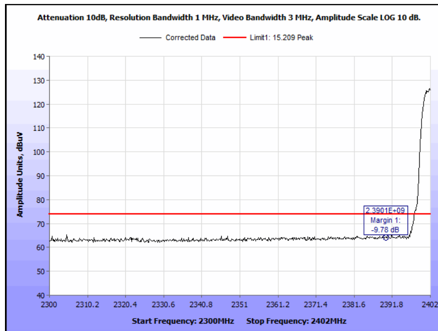
Plot 366. Radiated Restricted Band Edge, Low Channel, 3.5 MHz, 24 dBi Antenna, Peak
