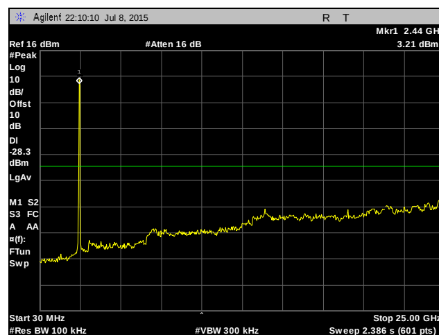
Plot 454. Conducted Spurious Emissions, High Channel, 40 MHz, Chain 1
