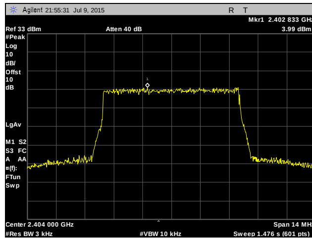
Plot 506. Peak Power Spectral Density, Low Channel, 7 MHz, Chain 1, 6 dBi Antenna
