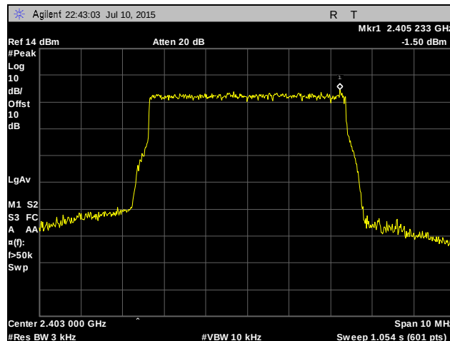
Plot 551. Peak Power Spectral Density, Low Channel, 5 MHz, Chain 0, 24 dBi Antenna
