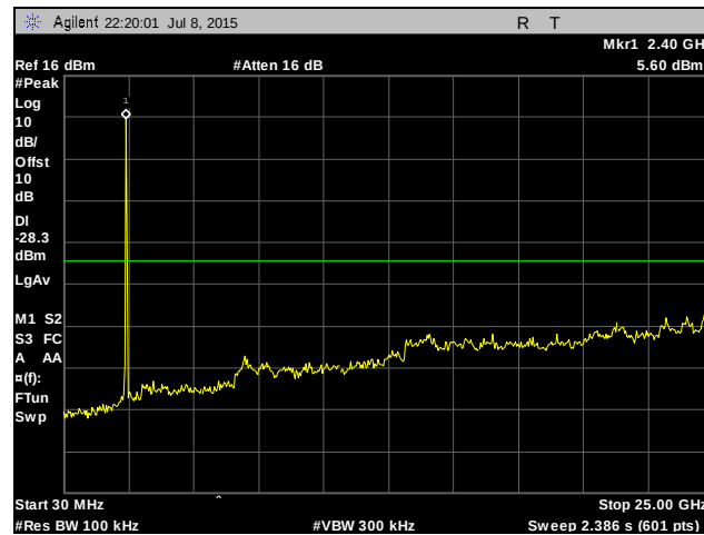
Plot 431. Conducted Spurious Emissions, Low Channel, 20 MHz, Chain 0
