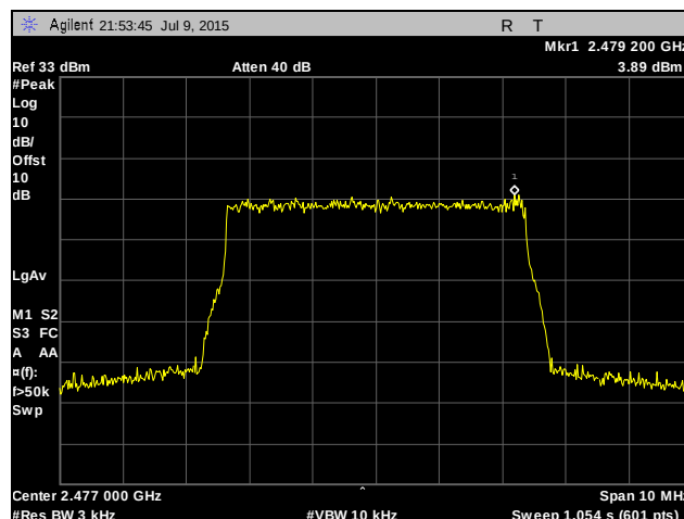
Plot 502. Peak Power Spectral Density, High Channel, 5 MHz, Chain 1, 6 dBi Antenna
