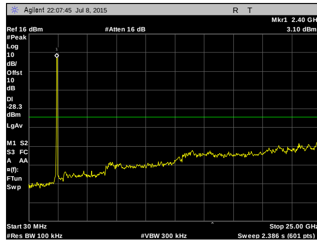
Plot 452. Conducted Spurious Emissions, Low Channel, 40 MHz, Chain 1
