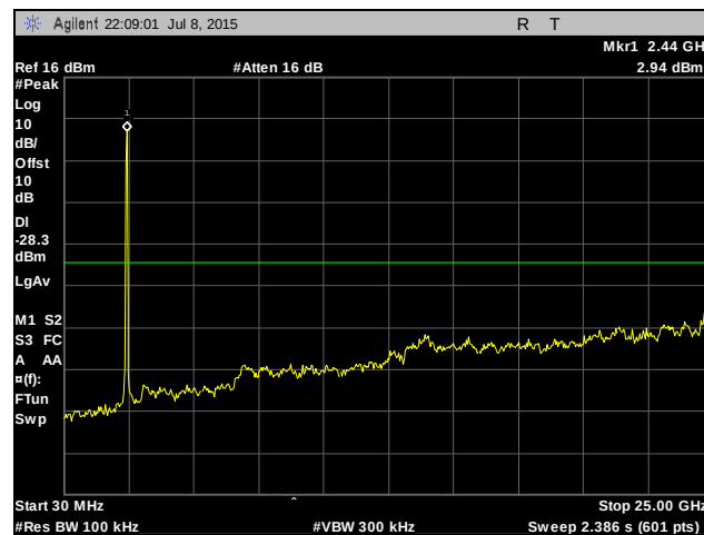
Plot 453. Conducted Spurious Emissions, Mid Channel, 40 MHz, Chain 1
