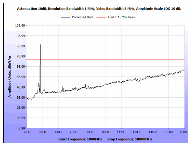
Plot 323. Radiated Spurious Emissions, Mid Channel, 40 MHz, 24 dBi Antenna, 1 GHz - 18 GHz, Peak
