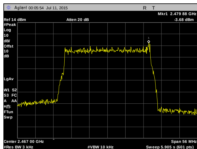
Plot 586. Peak Power Spectral Density, High Channel, 28 MHz, Chain 1, 24 dBi Antenna
