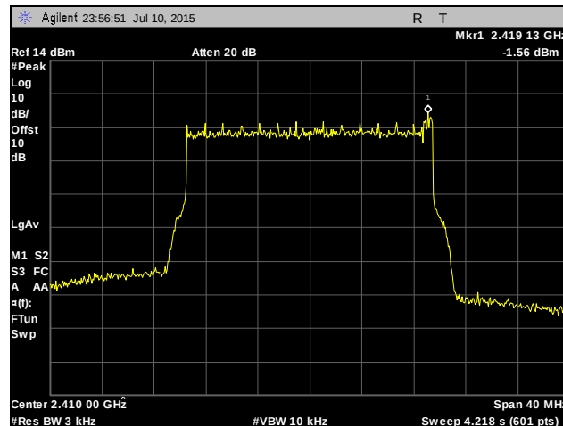
Plot 578. Peak Power Spectral Density, Low Channel, 20 MHz, Chain 1, 24 dBi Antenna
