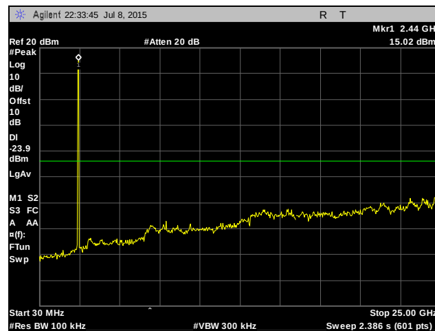
Plot 402. Conducted Spurious Emissions, Mid Channel, 3.5 MHz, Chain 0
