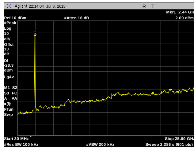
Plot 449. Conducted Spurious Emissions, Low Channel, 40 MHz, Chain 0
