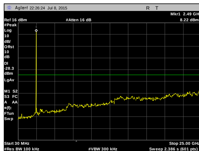
Plot 421. Conducted Spurious Emissions, High Channel, 10 MHz, Chain 0
