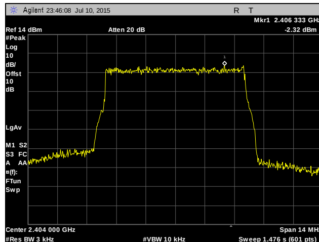
Plot 560. Peak Power Spectral Density, Low Channel, 7 MHz, Chain 1, 24 dBi Antenna
