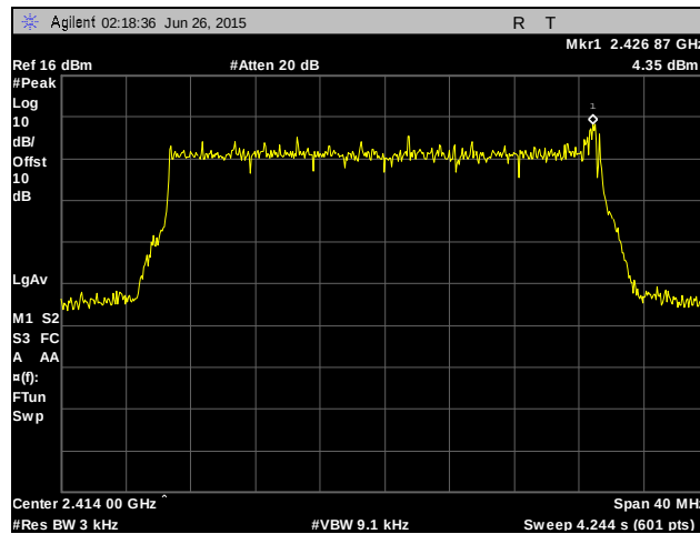
Plot 530. Peak Power Spectral Density, Low Channel, 28 MHz, Chain 1, 6 dBi Antenna
