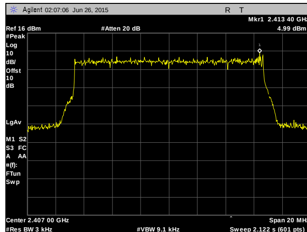
Plot 518. Peak Power Spectral Density, Low Channel, 14 MHz, Chain 1, 6 dBi Antenna
