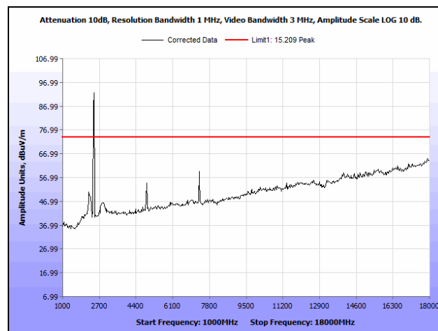
Plot 314. Radiated Spurious Emissions, Mid Channel, 30 MHz, 24 dBi Antenna, 1 GHz - 18 GHz, Peak
