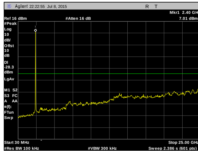
Plot 425. Conducted Spurious Emissions, Low Channel, 14 MHz, Chain 0
