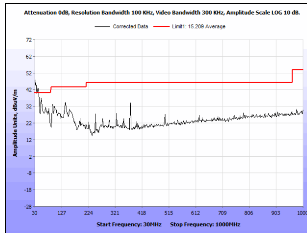
Plot 303. Radiated Spurious Emissions, Mid Channel, 28 MHz, 24 dBi Antenna, 30 MHz - 1 GHz
