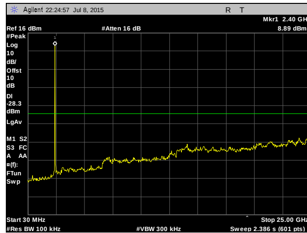
Plot 419. Conducted Spurious Emissions, Low Channel, 10 MHz, Chain 0
