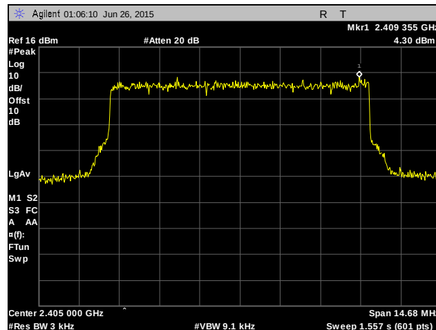
Plot 509. Peak Power Spectral Density, Low Channel, 10 MHz, Chain 0, 6 dBi Antenna
