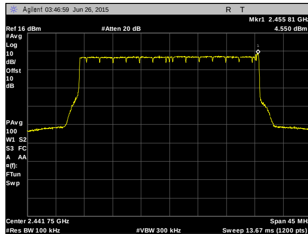
Plot 537. Peak Power Spectral Density, Mid Channel, 30 MHz, Chain 1, 6 dBi Antenna
