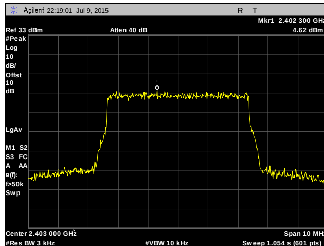
Plot 497. Peak Power Spectral Density, Low Channel, 5 MHz, Chain 0, 6 dBi Antenna
