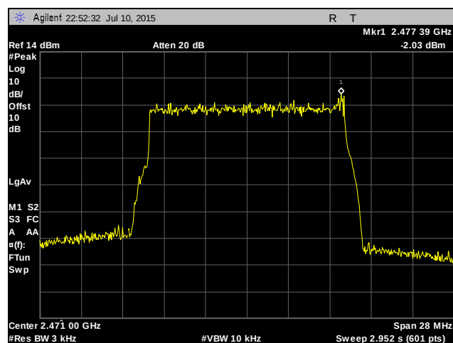
Plot 571. Peak Power Spectral Density, High Channel, 14 MHz, Chain 0, 24 dBi Antenna
