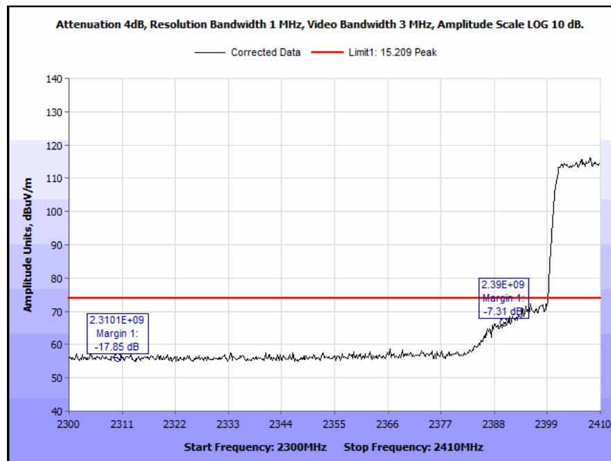
Plot 350. Radiated Restricted Band Edge, Low Channel, 20 MHz, 6 dBi Antenna, Peak
