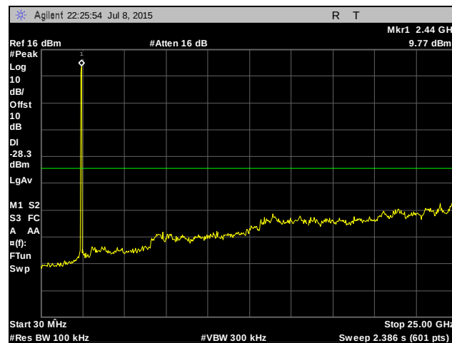
Plot 420. Conducted Spurious Emissions, Mid Channel, 10 MHz, Chain 0
