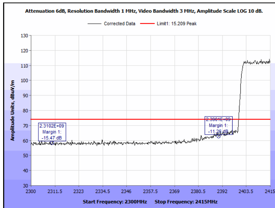
Plot 394. Radiated Restricted Band Edge, Low Channel, 30 MHz, 24 dBi Antenna, Peak
