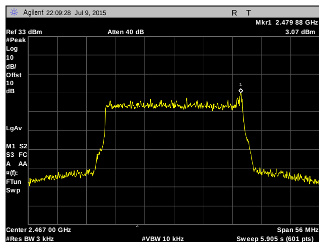
Plot 529. Peak Power Spectral Density, High Channel, 28 MHz, Chain 0, 6 dBi Antenna
