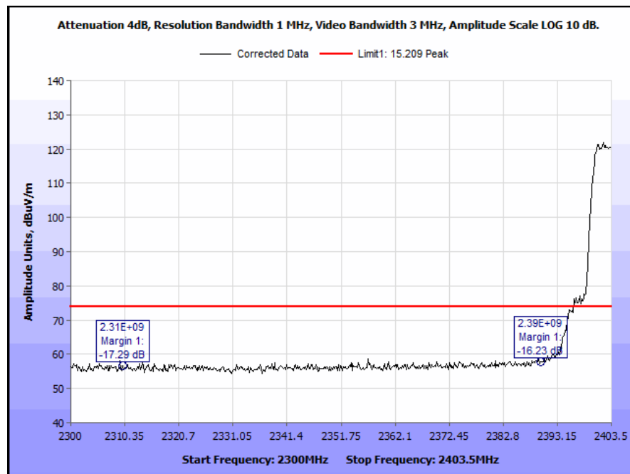
Plot 338. Radiated Restricted Band Edge, Low Channel, 7 MHz, 6 dBi Antenna, Peak
