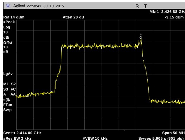
Plot 581. Peak Power Spectral Density, Low Channel, 28 MHz, Chain 0, 24 dBi Antenna
