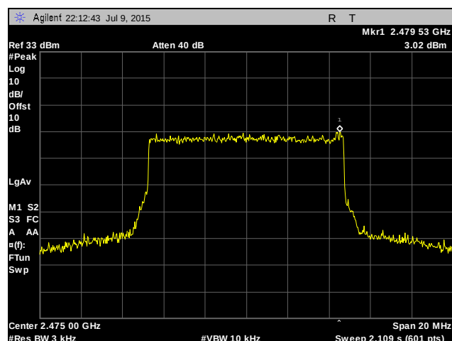
Plot 511. Peak Power Spectral Density, High Channel, 10 MHz, Chain 0, 6 dBi Antenna
