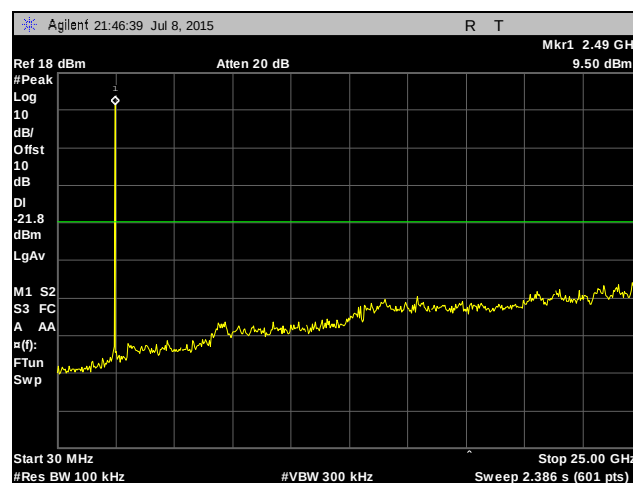
Plot 418. Conducted Spurious Emissions, High Channel, 7 MHz, Chain 1
