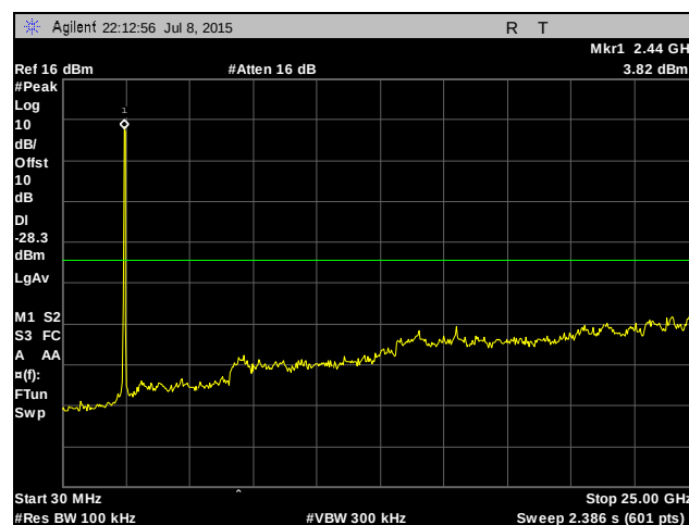
Plot 451. Conducted Spurious Emissions, High Channel, 40 MHz, Chain 0
