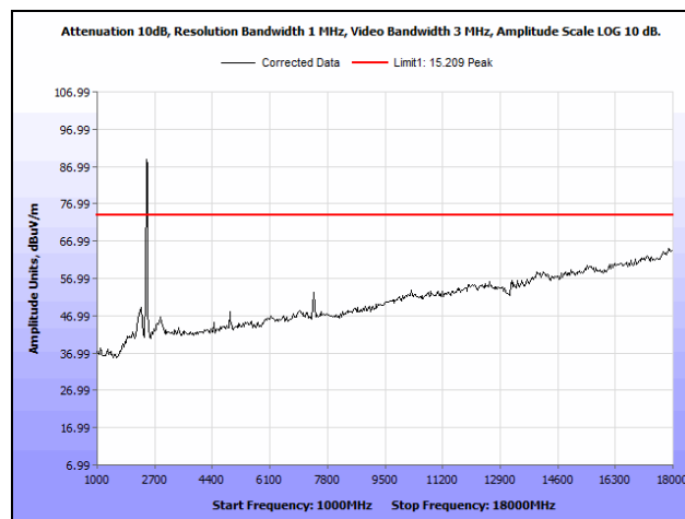
Plot 326. Radiated Spurious Emissions, High Channel, 40 MHz, 24 dBi Antenna, 1 GHz - 18 GHz, Peak
