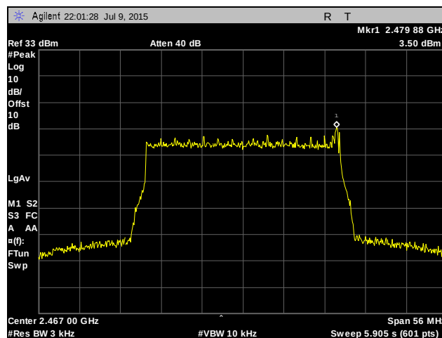
Plot 532. Peak Power Spectral Density, High Channel, 28 MHz, Chain 1, 6 dBi Antenna
