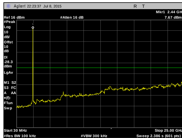
Plot 426. Conducted Spurious Emissions, Mid Channel, 14 MHz, Chain 0
