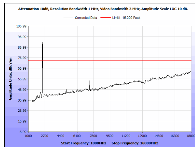
Plot 317. Radiated Spurious Emissions, High Channel, 30 MHz, 24 dBi Antenna, 1 GHz - 18 GHz, Peak
