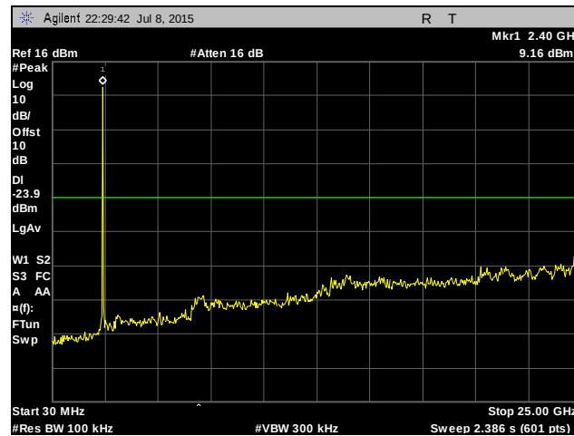
Plot 407. Conducted Spurious Emissions, Low Channel, 5 MHz, Chain 0
