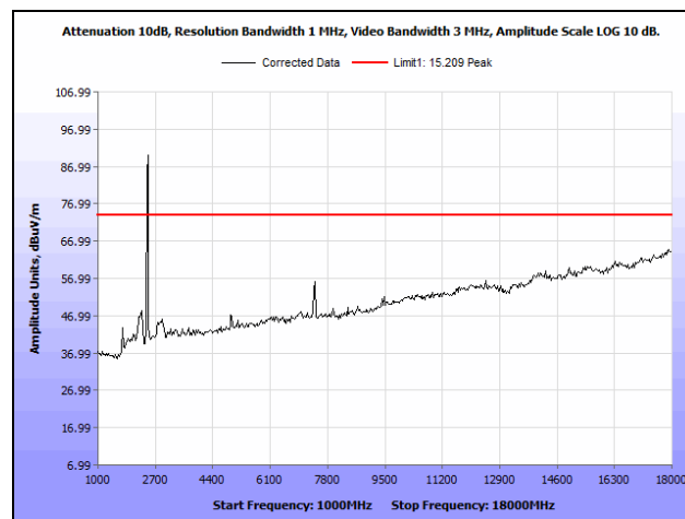
Plot 308. Radiated Spurious Emissions, High Channel, 28 MHz, 24 dBi Antenna, 1 GHz - 18 GHz, Peak
