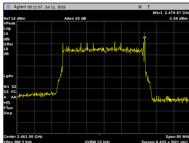
Plot 598. Peak Power Spectral Density, High Channel, 40 MHz, Chain 1, 24 dBi Antenna
