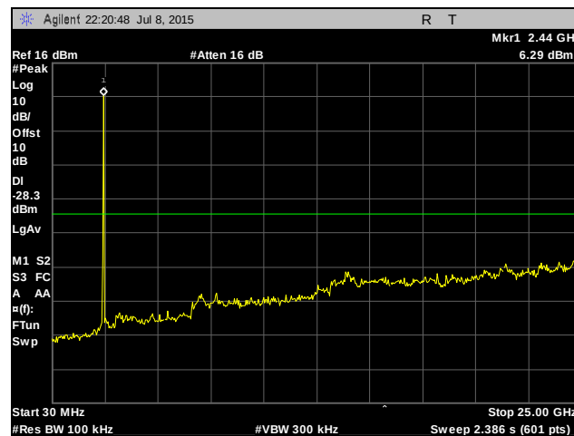
Plot 432. Conducted Spurious Emissions, Mid Channel, 20 MHz, Chain 0
