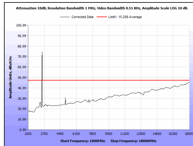
Plot 316. Radiated Spurious Emissions, High Channel, 30 MHz, 24 dBi Antenna, 1 GHz - 18 GHz, Average
