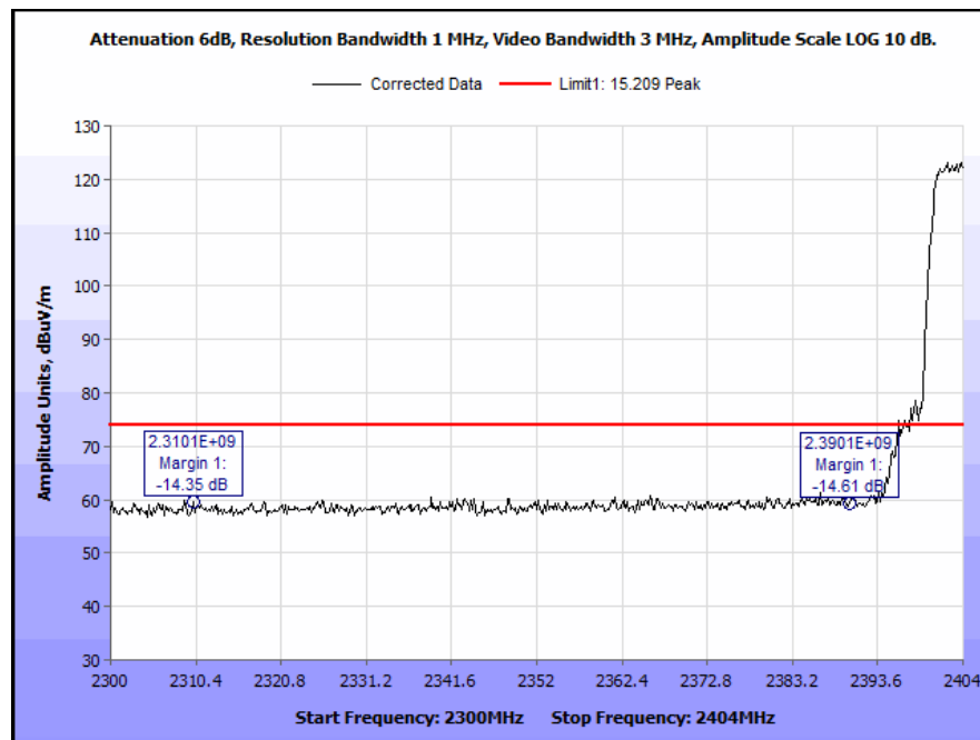
Plot 374. Radiated Restricted Band Edge, Low Channel, 7 MHz, 24 dBi Antenna, Peak
