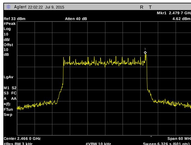
Plot 538. Peak Power Spectral Density, High Channel, 30 MHz, Chain 1, 6 dBi Antenna
