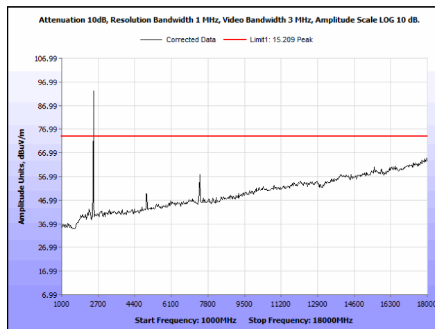
Plot 299. Radiated Spurious Emissions, High Channel, 20 MHz, 24 dBi Antenna, 1 GHz - 18 GHz, Peak
