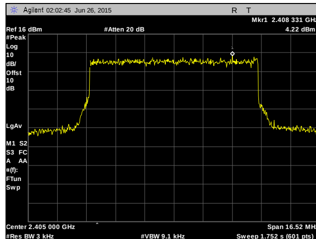
Plot 512. Peak Power Spectral Density, Low Channel, 10 MHz, Chain 1, 6 dBi Antenna
