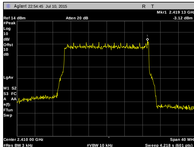
Plot 575. Peak Power Spectral Density, Low Channel, 20 MHz, Chain 0, 24 dBi Antenna
