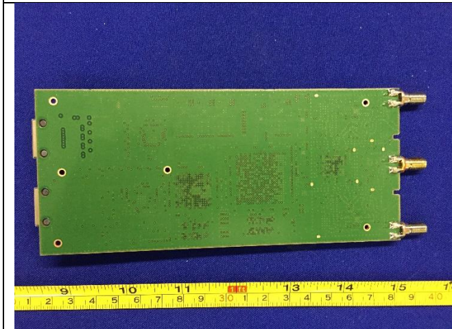
EUT - Mainboard bottom View
