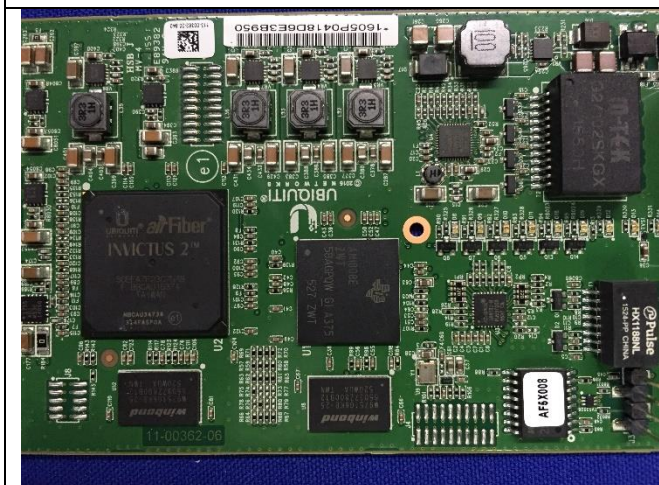
EUT - Mainboard View
