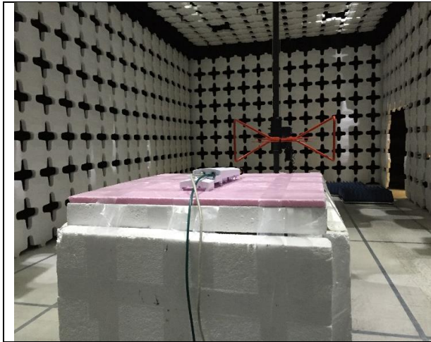
Radiated Spurious Emissions below 1GHz – Front View
