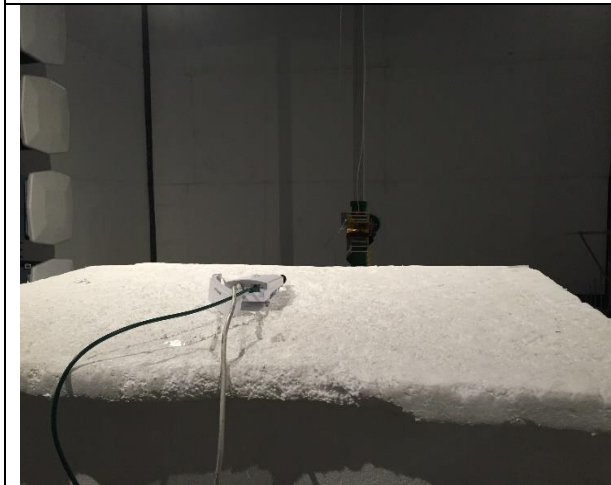
Radiated Spurious Emissions above 1GHz – Front View
