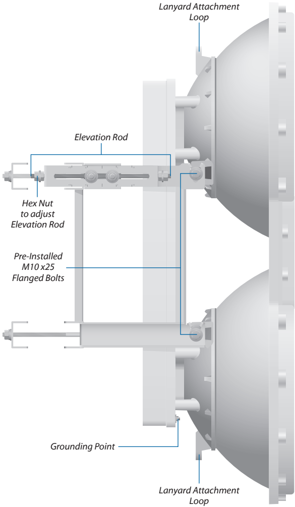
Assembled View
