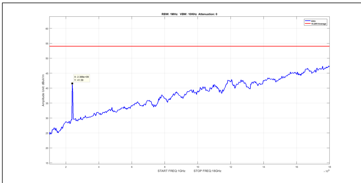
Plot 47. Radiated Spurious Emissions, Average, Nonhopping, 1G – 18G, DH1, 2402MHz
