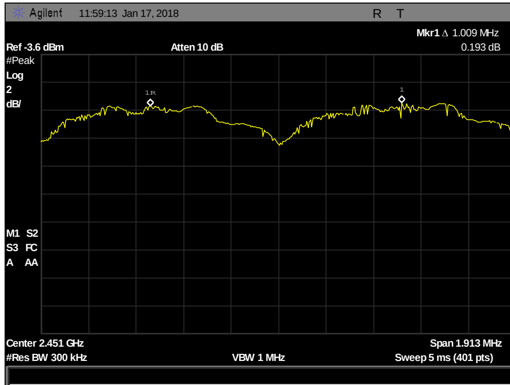
Plot 34. Channel Separation, 3-DH5
