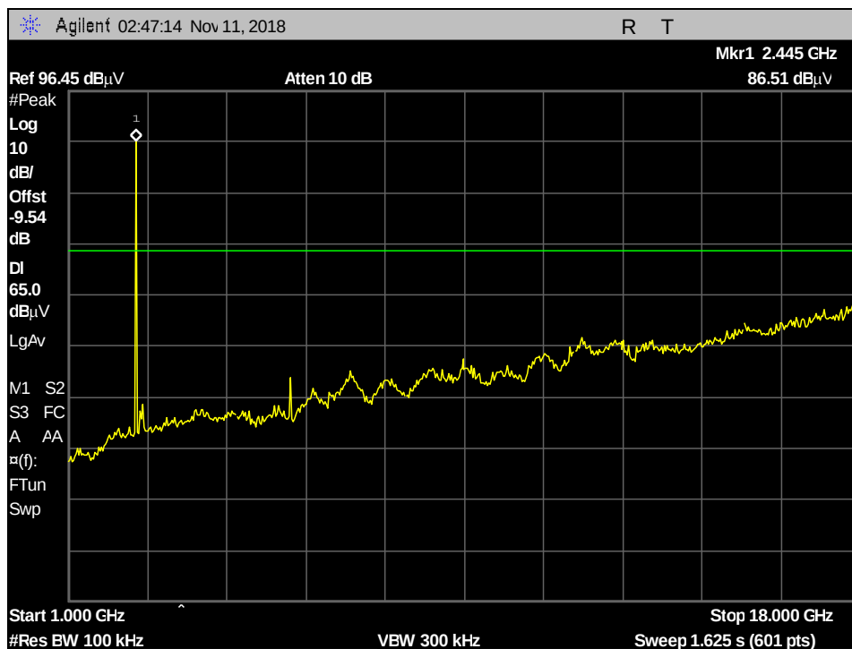
Plot 114. Conducted Spurious Emissions, Nonhopping, 2441MHz, 3-DH5, 1 GHz – 18 GHz
