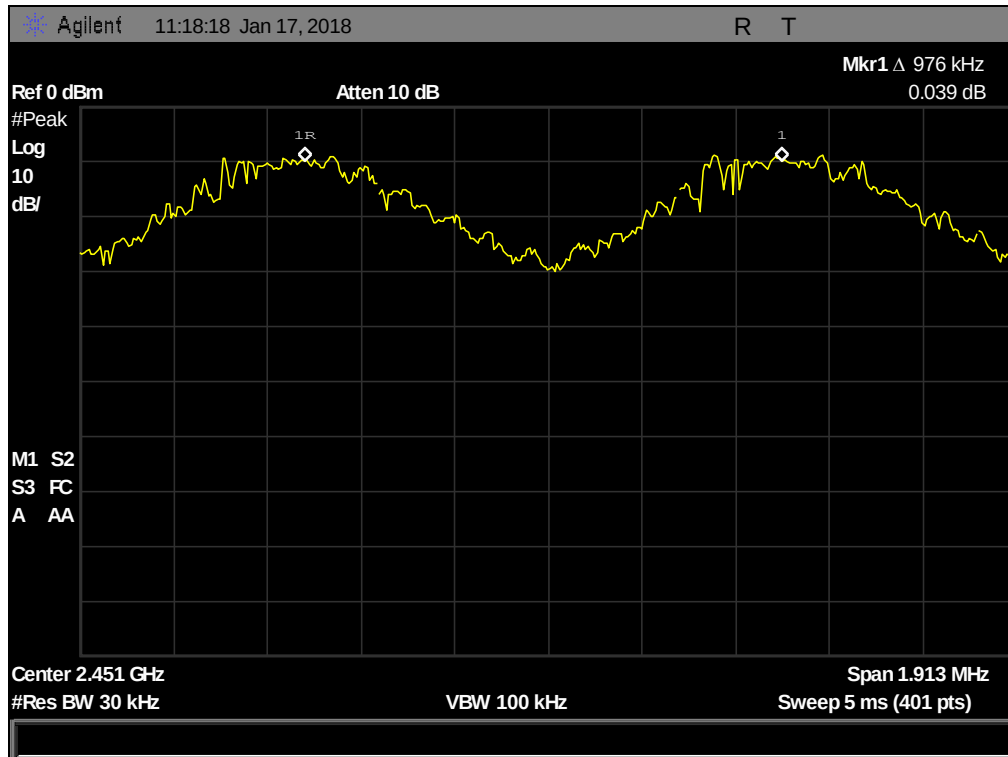
Plot 32. Channel Separation, DH5
