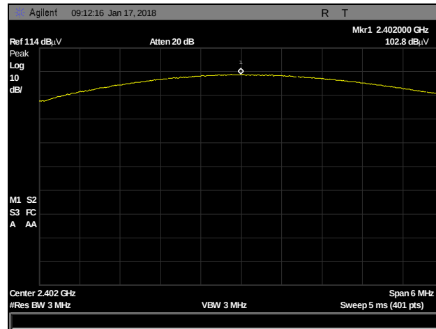
Plot 44. Peak Power Output, 3-DH5, 2402MHz
