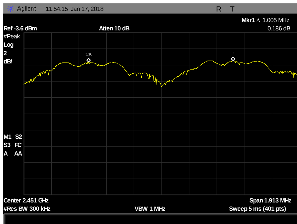
Plot 33. Channel Separation, 3-DH1
