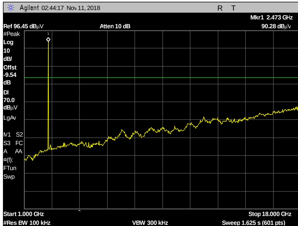
Plot 117. Conducted Spurious Emissions, Nonhopping, 2480MHz, 3-DH1, 1 GHz – 18 GHz
