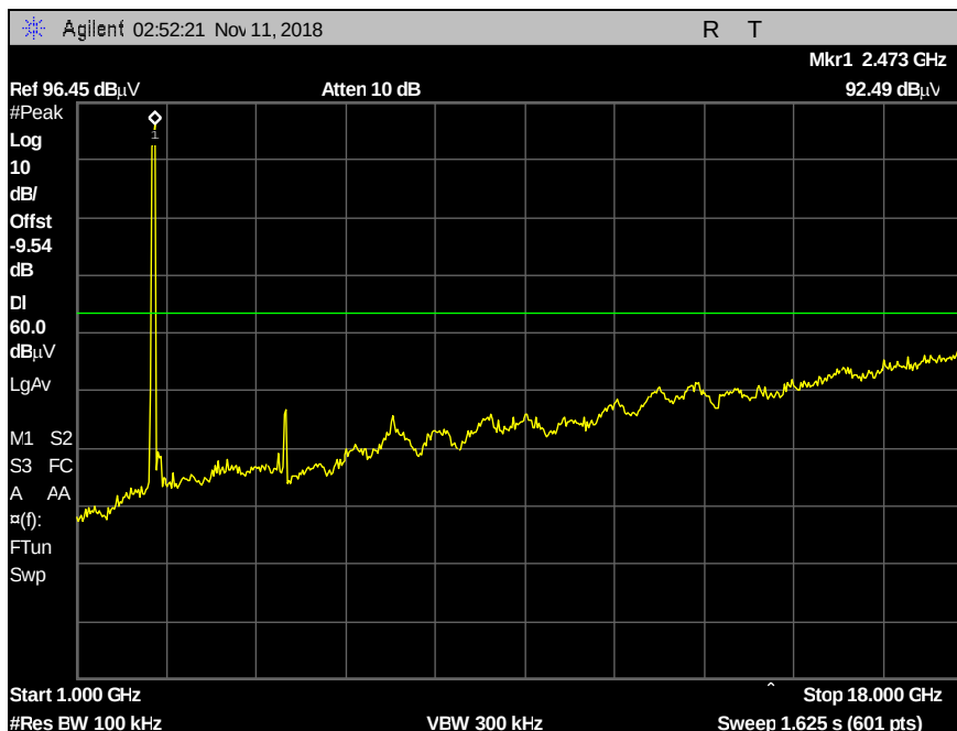
Plot 104. Conducted Spurious Emissions, Hopping, DH5, 1 GHz – 18 GHz
