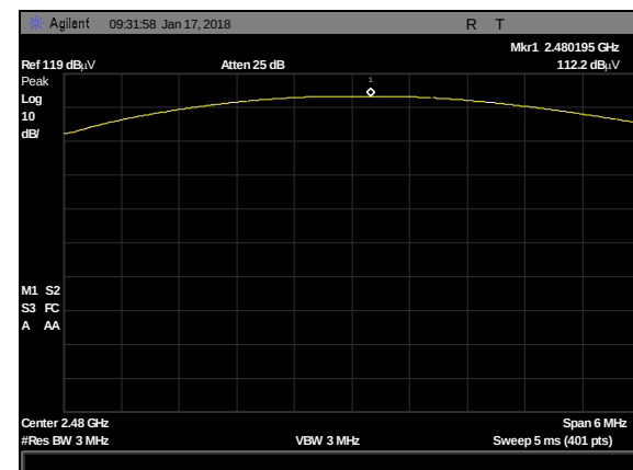
Plot 40. Peak Power Output, DH5, 2480MHz
