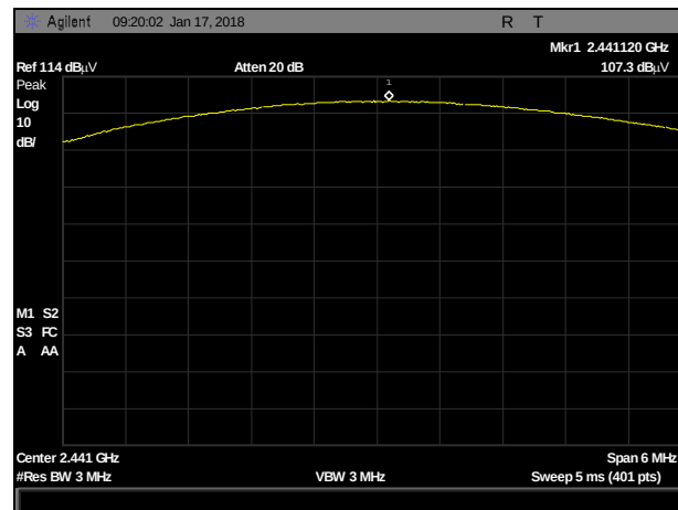
Plot 42. Peak Power Output, 3-DH1, 2441MHz
