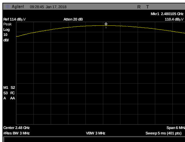
Plot 43. Peak Power Output, 3-DH1, 2480MHz
