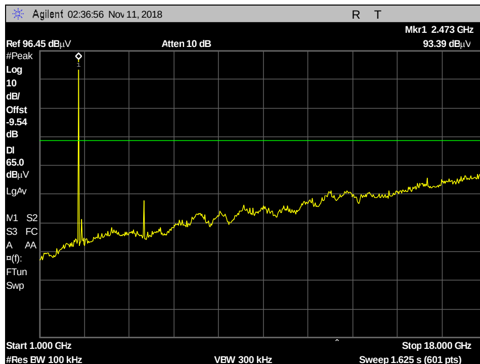
Plot 116. Conducted Spurious Emissions, Nonhopping, 2480MHz, DH5, 1 GHz – 18 GHz
