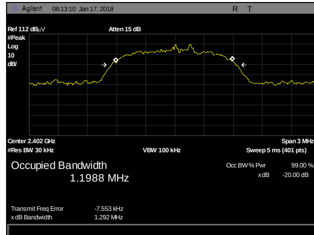
Plot 12. 20 dB Occupied Bandwidth, 3-DH5, 2402 MHz
