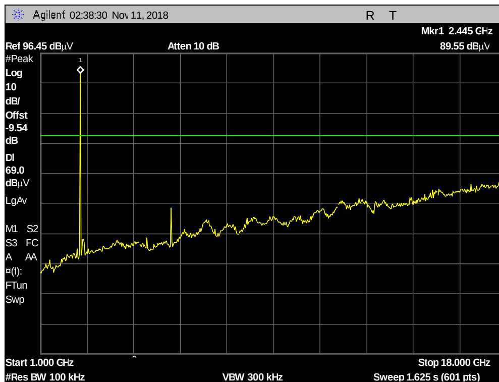
Plot 112. Conducted Spurious Emissions, Nonhopping, 2441MHz, DH5, 1 GHz – 18 GHz
