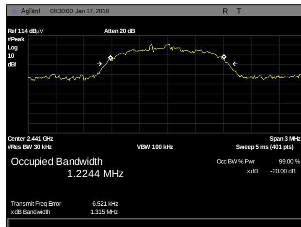
Plot 13. 20 dB Occupied Bandwidth, 3-DH5, 2441 MHz
