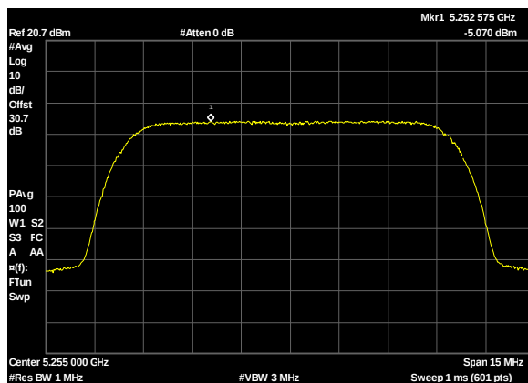
Plot 241. Power Spectral Density, UNII 2A, BW 10M, CF 5255M, c0, 19dBi
