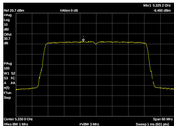
Plot 263. Power Spectral Density, UNII 2A, BW 40M, CF 5330M, c0, 19dBi
