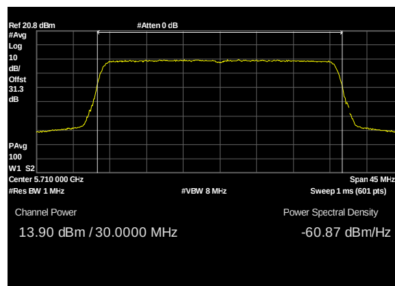
Plot 138. Conducted Transmitter Output Power, UNII 2C, BW 30M, CF 5710M, c1, 13dBi
