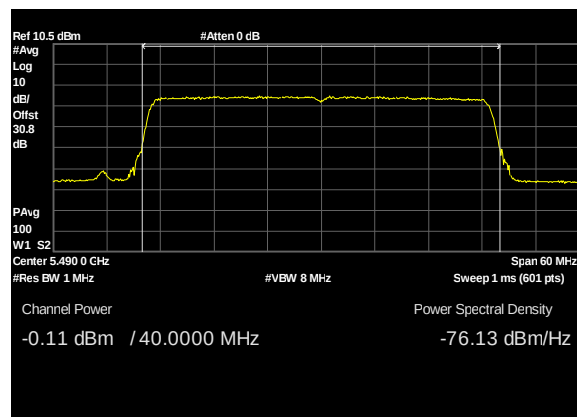
Plot 200. Conducted Transmitter Output Power, UNII 2C, BW 40W, CF 5490M, c1, 27dBi
