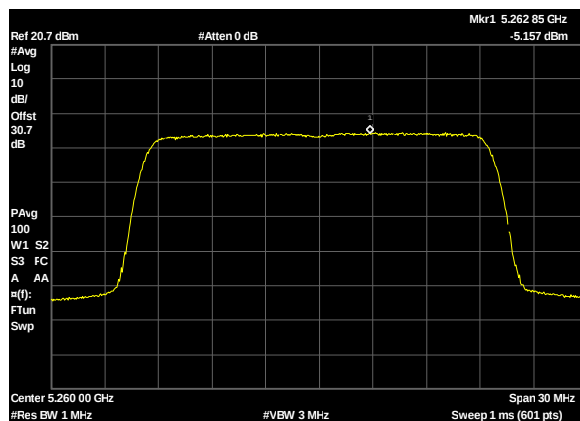
Plot 248. Power Spectral Density, UNII 2A, BW 20M, CF 5260M, c1, 19dBi
