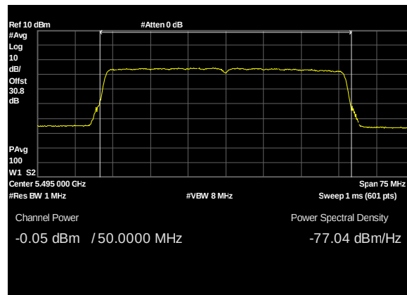
Plot 205. Conducted Transmitter Output Power, UNII 2C, BW 50W, CF 5495M, c0, 27dBi
