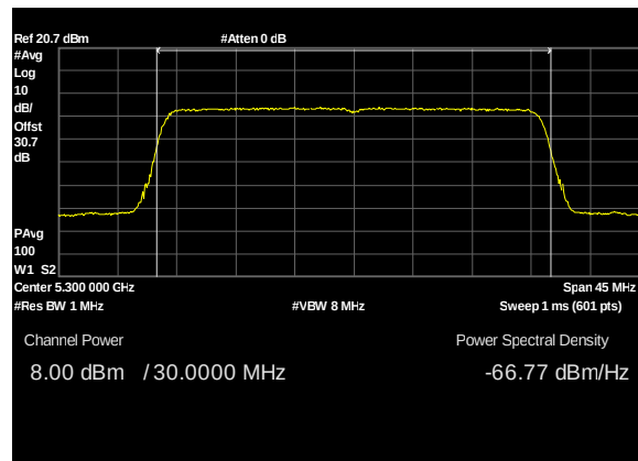
Plot 76. Conducted Transmitter Output Power, UNII 2A, BW 30M, CF 5300M, c1, 19dBi
