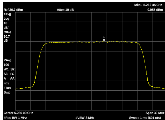
Plot 217. Power Spectral Density, UNII 2A, BW 20M, CF 5260M, c0, 13dBi
