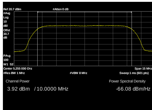
Plot 61. Conducted Transmitter Output Power, UNII 2A, BW 10M, CF 5255M, c0, 19dBi
