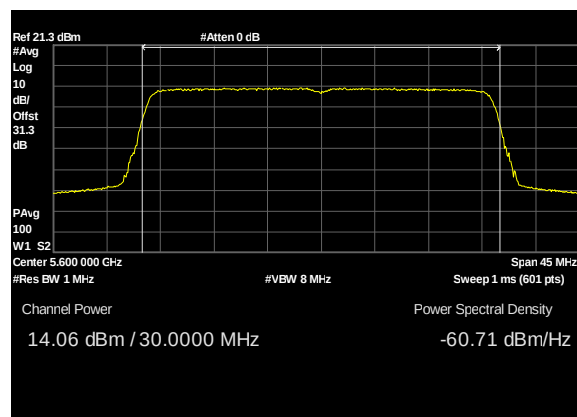
Plot 135. Conducted Transmitter Output Power, UNII 2C, BW 30M, CF 5600M, c0, 13dBi
