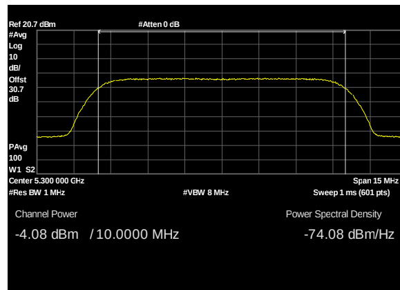
Plot 94. Conducted Transmitter Output Power, UNII 2A, BW 10M, CF 5300M, c1, 27dBi
