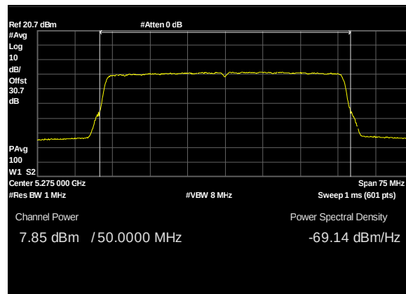
Plot 86. Conducted Transmitter Output Power, UNII 2A, BW 50M, CF 5275M, c1, 19dBi
