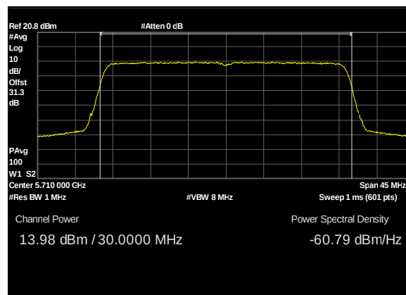
Plot 137. Conducted Transmitter Output Power, UNII 2C, BW 30M, CF 5710M, c0, 13dBi
