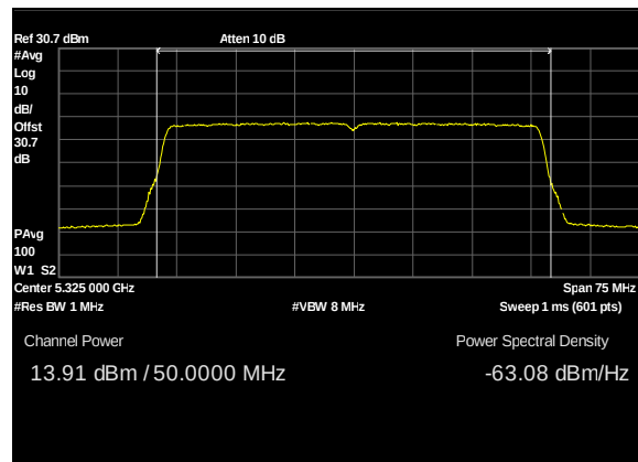
Plot 59. Conducted Transmitter Output Power, UNII 2A, BW 50M, CF 5325M, c0, 13dBi
