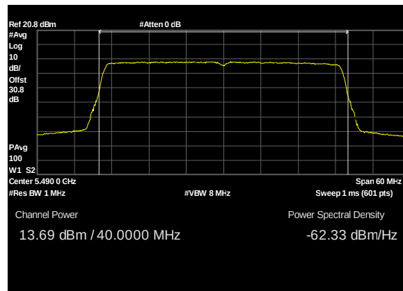
Plot 139. Conducted Transmitter Output Power, UNII 2C, BW 40M, CF 5490M, c0, 13dBi
