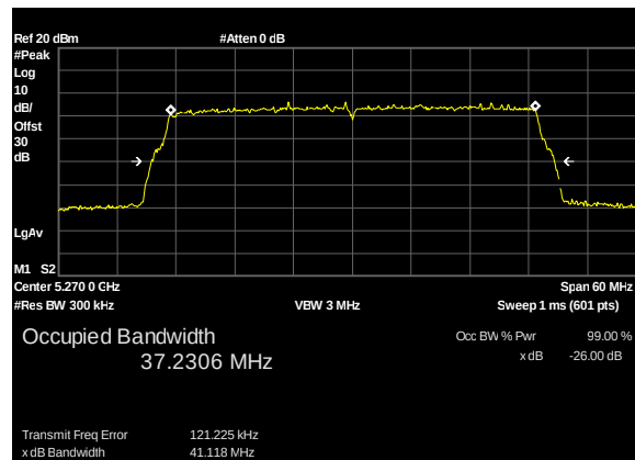
Plot 10. 26 dB Occupied Bandwidth, UNII 2A, 40M, 5270M, c1
