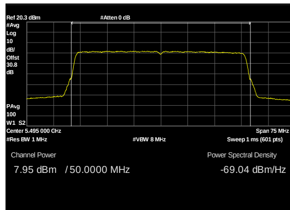
Plot 176. Conducted Transmitter Output Power, UNII 2C, BW 50M, CF 5495M, c1, 19dBi
