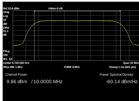
Plot 125. Conducted Transmitter Output Power, UNII 2C, BW 10M, CF 5720M, c0, 13dBi
