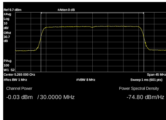
Plot 104. Conducted Transmitter Output Power, UNII 2A, BW 30M, CF 5265M, c1, 27dBi
