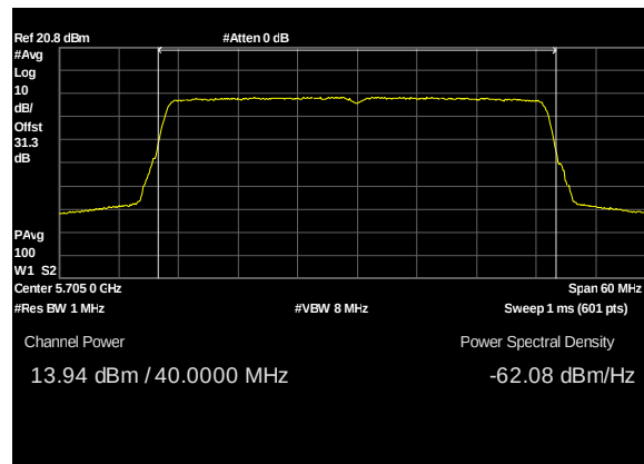
Plot 143. Conducted Transmitter Output Power, UNII 2C, BW 40M, CF 5705M, c0, 13dB
