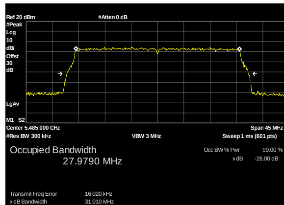
Plot 22. 26 dB Occupied Bandwidth, UNII 2C, 30M, 5485M, c1
