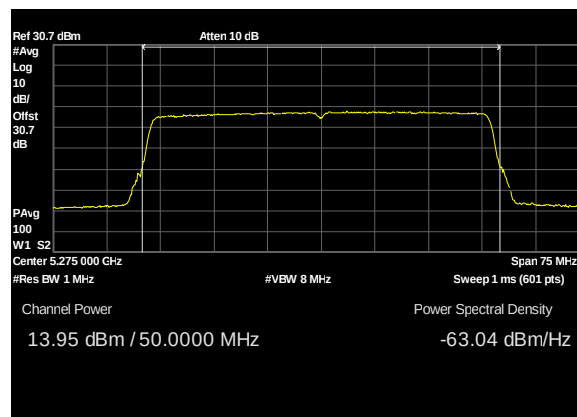
Plot 56. Conducted Transmitter Output Power, UNII 2A, BW 50M, CF 5275M, c1, 13dBi
