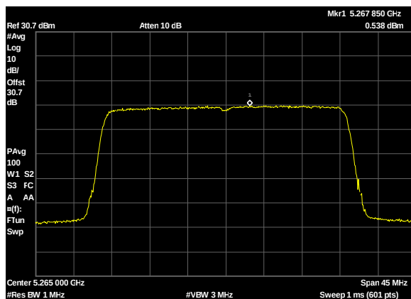
Plot 224. Power Spectral Density, UNII 2A, BW 30M, CF 5265M, c1, 13dBi
