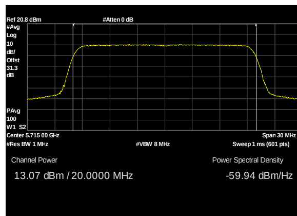
Plot 132. Conducted Transmitter Output Power, UNII 2C, BW 20M, CF 5715M, c1, 13dBi
