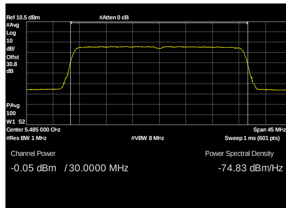
Plot 193. Conducted Transmitter Output Power, UNII 2C, BW 30W, CF 5485M, c0, 27dBi
