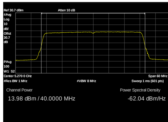
Plot 50. Conducted Transmitter Output Power, UNII 2A, BW 40M, CF 5270M, c1, 13dBi
