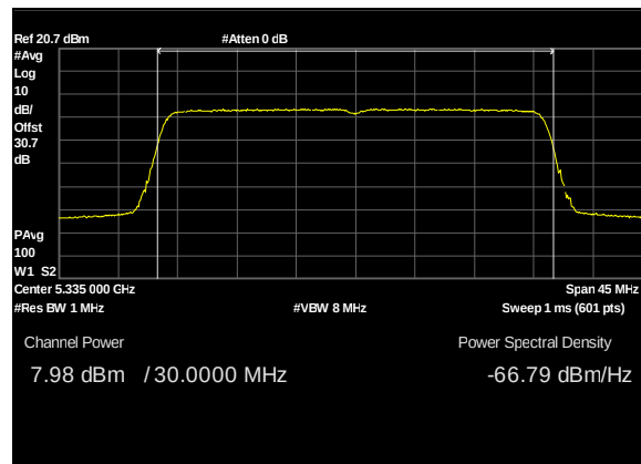
Plot 77. Conducted Transmitter Output Power, UNII 2A, BW 30M, CF 5335M, c0, 19dBi
