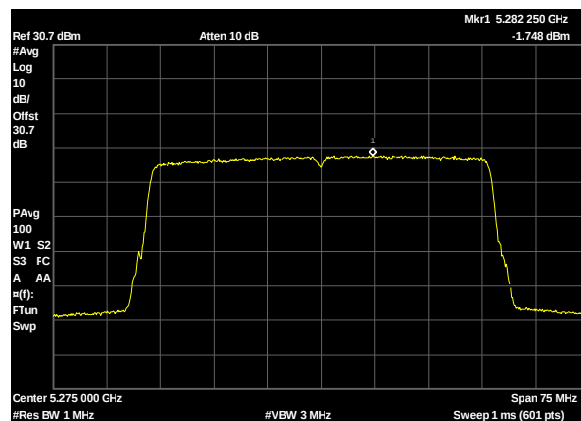
Plot 236. Power Spectral Density, UNII 2A, BW 50M, CF 5275M, c1, 13dBi
