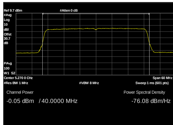
Plot 110. Conducted Transmitter Output Power, UNII 2A, BW 40M, CF 5270M, c1, 27dBi
