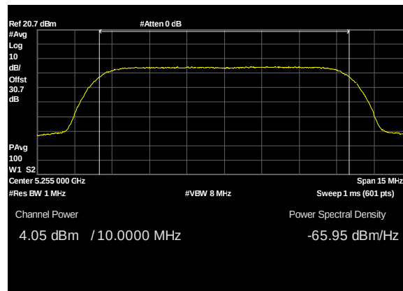
Plot 62. Conducted Transmitter Output Power, UNII 2A, BW 10M, CF 5255M, c1, 19dBi
