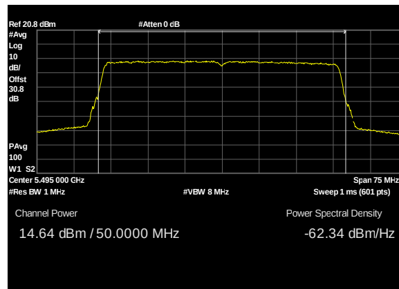
Plot 145. Conducted Transmitter Output Power, UNII 2C, BW 50M, CF 5495M, c0, 13dBi
