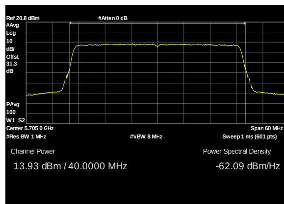
Plot 144. Conducted Transmitter Output Power, UNII 2C, BW 40M, CF 5705M, c1, 13dB
