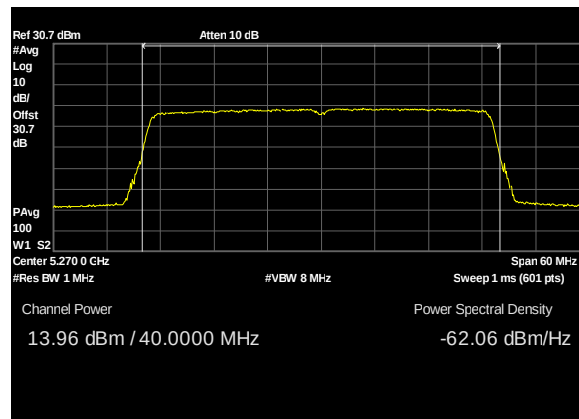
Plot 49. Conducted Transmitter Output Power, UNII 2A, BW 40M, CF 5270M, c0, 13dBi
