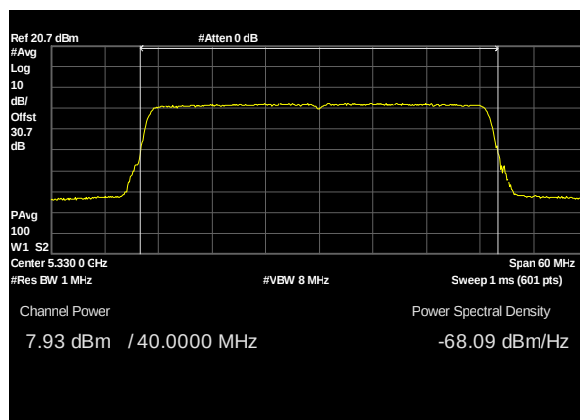
Plot 84. Conducted Transmitter Output Power, UNII 2A, BW 40M, CF 5330M, c1, 19dBi
