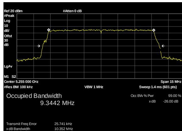
Plot 1. 26 dB Occupied Bandwidth, UNII 2A, 10M, 5255M, c1
