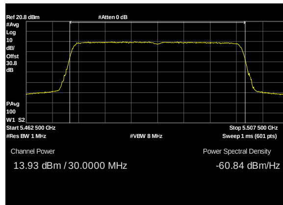
Plot 133. Conducted Transmitter Output Power, UNII 2C, BW 30M, CF 5485M, c0, 13dBi
