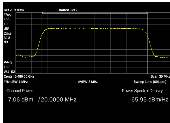
Plot 158. Conducted Transmitter Output Power, UNII 2C, BW 20M, CF 5480M, c1, 19dBi
