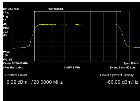
Plot 68. Conducted Transmitter Output Power, UNII 2A, BW 20M, CF 5260M, c1, 19dBi
