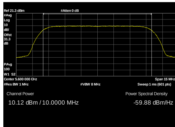
Plot 124. Conducted Transmitter Output Power, UNII 2C, BW 10M, CF 5600M, c1, 13dBi
