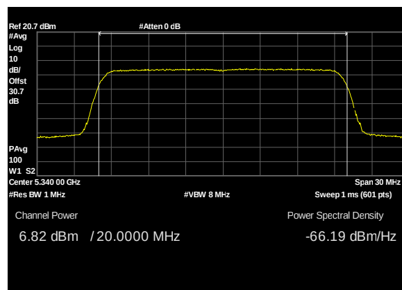
Plot 72. Conducted Transmitter Output Power, UNII 2A, BW 20M, CF 5340M, c1, 19dBi
