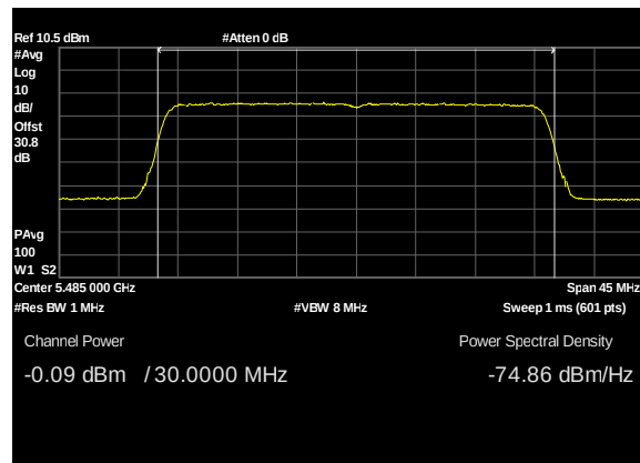
Plot 194. Conducted Transmitter Output Power, UNII 2C, BW 30W, CF 5485M, c1, 27dBi
