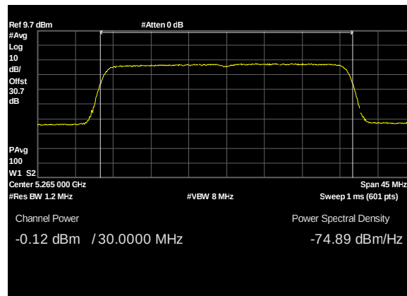
Plot 103. Conducted Transmitter Output Power, UNII 2A, BW 30M, CF 5265M, c0, 27dBi
