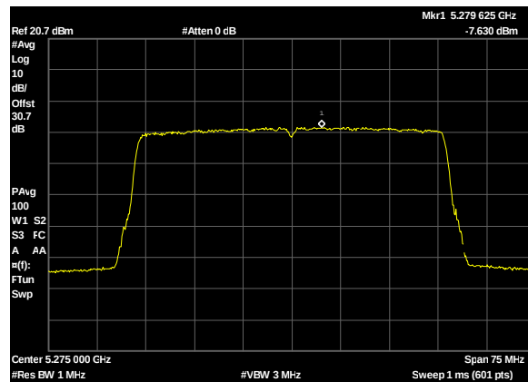
Plot 266. Power Spectral Density, UNII 2A, BW 50M, CF 5275M, c1, 19dBi
