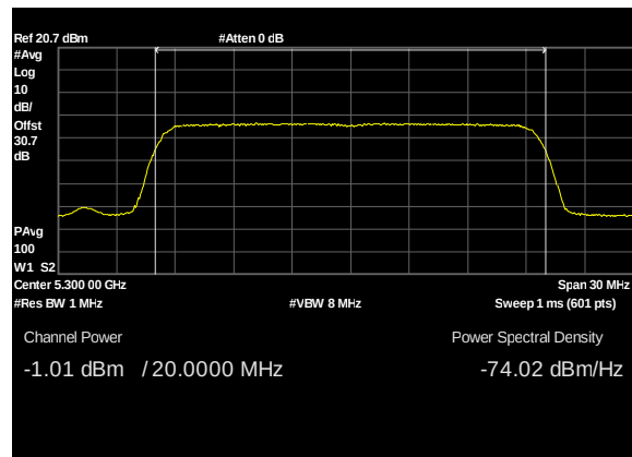
Plot 100. Conducted Transmitter Output Power, UNII 2A, BW 20M, CF 5300M, c1, 27dBi
