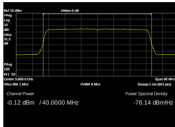
Plot 202. Conducted Transmitter Output Power, UNII 2C, BW 40W, CF 5600M, c1, 27dBi
