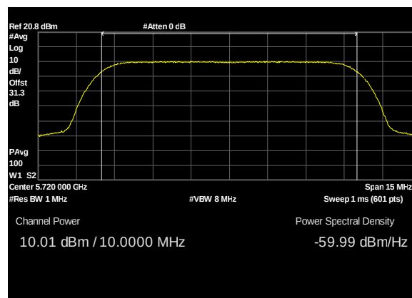
Plot 126. Conducted Transmitter Output Power, UNII 2C, BW 10M, CF 5720M, c1, 13dBi
