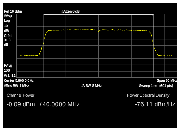
Plot 201. Conducted Transmitter Output Power, UNII 2C, BW 40W, CF 5600M, c0, 27dBi
