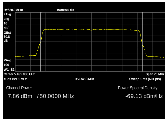
Plot 175. Conducted Transmitter Output Power, UNII 2C, BW 50M, CF 5495M, c0, 19dBi
