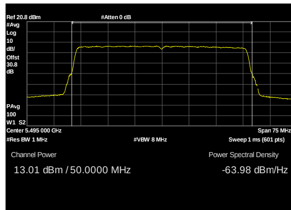
Plot 146. Conducted Transmitter Output Power, UNII 2C, BW 50M, CF 5495M, c1, 13dBi
