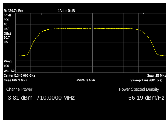
Plot 66. Conducted Transmitter Output Power, UNII 2A, BW 10M, CF 5345M, c1, 19dBi
