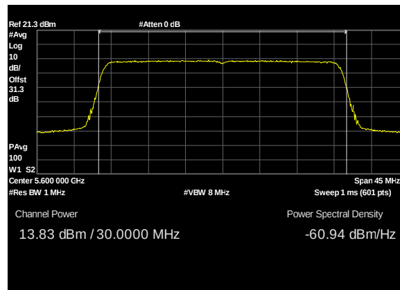
Plot 136. Conducted Transmitter Output Power, UNII 2C, BW 30M, CF 5600M, c1, 13dBi
