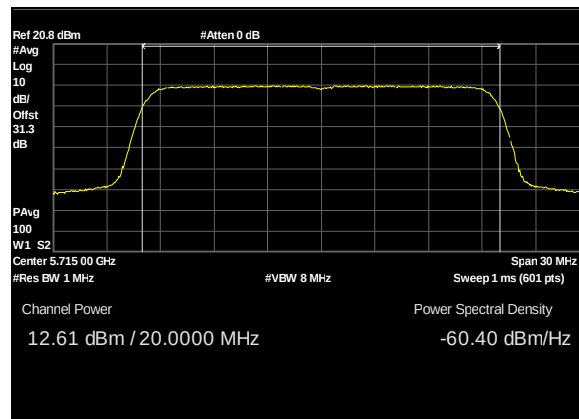
Plot 131. Conducted Transmitter Output Power, UNII 2C, BW 20M, CF 5715M, c0, 13dBi
