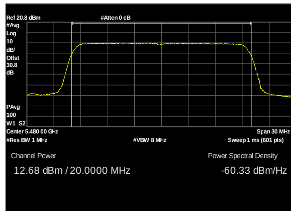
Plot 128. Conducted Transmitter Output Power, UNII 2C, BW 20M, CF 5480M, c1, 13dBi
