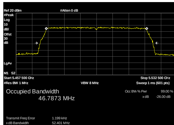
Plot 28. 26 dB Occupied Bandwidth, UNII 2C, 50M, 5495M, c1
