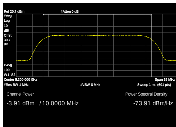
Plot 93. Conducted Transmitter Output Power, UNII 2A, BW 10M, CF 5300M, c0, 27dBi
