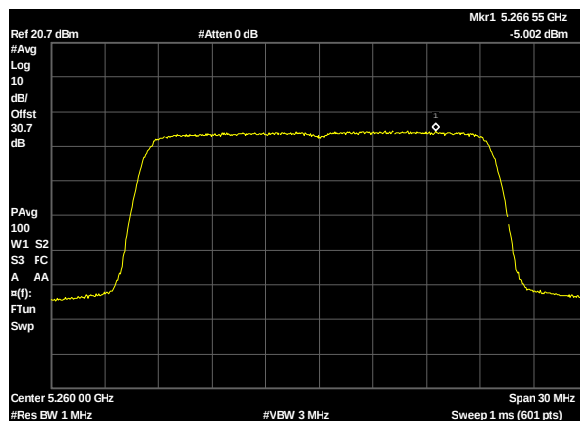
Plot 247. Power Spectral Density, UNII 2A, BW 20M, CF 5260M, c0, 19dBi
