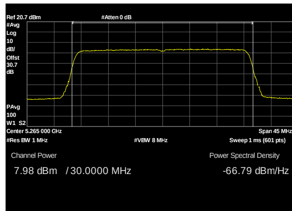
Plot 74. Conducted Transmitter Output Power, UNII 2A, BW 30M, CF 5265M, c1, 19dBi
