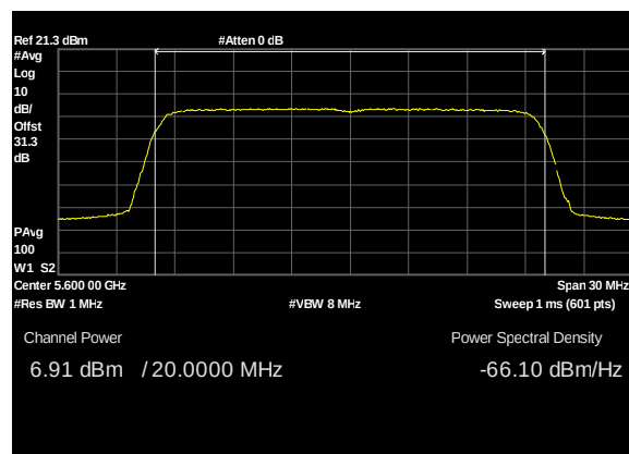
Plot 159. Conducted Transmitter Output Power, UNII 2C, BW 20M, CF 5600M, c0, 19dBi
