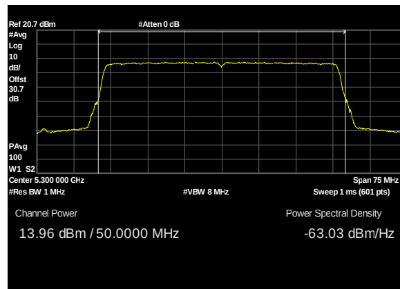
Plot 58. Conducted Transmitter Output Power, UNII 2A, BW 50M, CF 5300M, c1, 13dBi
