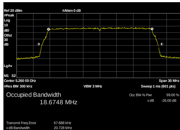
Plot 4. 26 dB Occupied Bandwidth, UNII 2A, 20M, 5260M, c1
