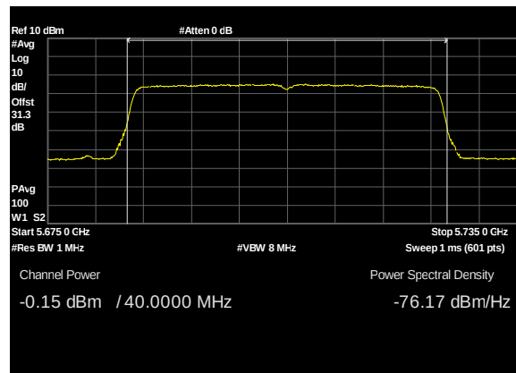
Plot 203. Conducted Transmitter Output Power, UNII 2C, BW 40W, CF 5705M, c0, 27dBi
