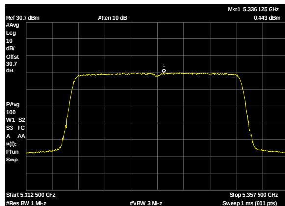
Plot 227. Power Spectral Density, UNII 2A, BW 30M, CF 5335M, c0, 13dBi
