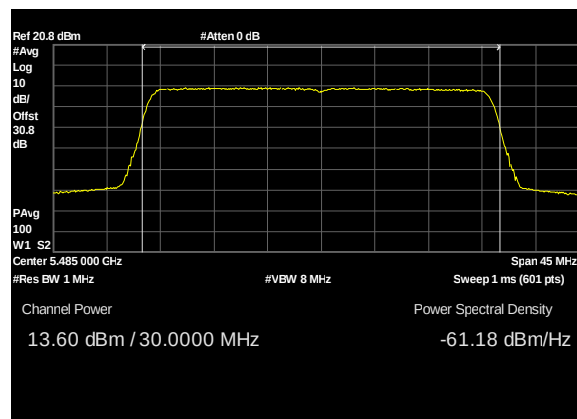
Plot 134. Conducted Transmitter Output Power, UNII 2C, BW 30M, CF 5485M, c1, 13dBi
