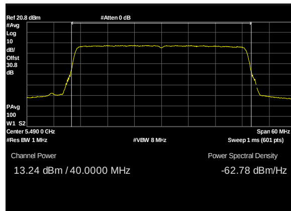
Plot 140. Conducted Transmitter Output Power, UNII 2C, BW 40M, CF 5490M, c1, 13dBi
