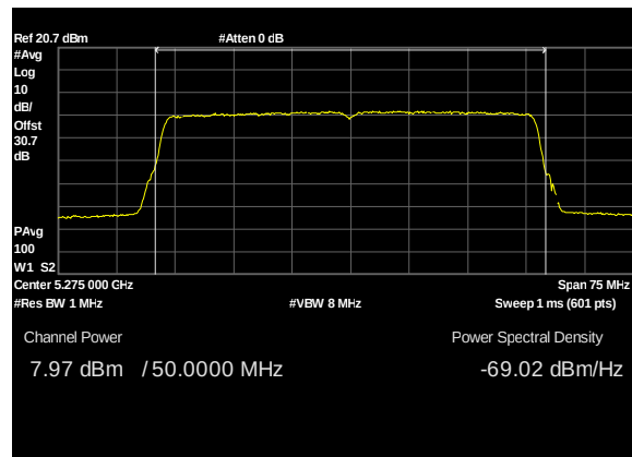
Plot 85. Conducted Transmitter Output Power, UNII 2A, BW 50M, CF 5275M, c0, 19dBi
