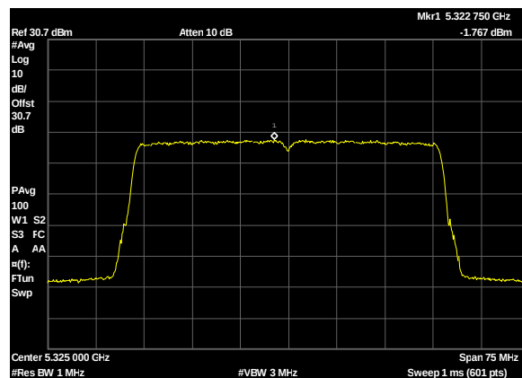
Plot 239. Power Spectral Density, UNII 2A, BW 50M, CF 5325M, c0, 13dBi
