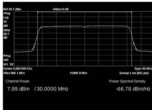
Plot 73. Conducted Transmitter Output Power, UNII 2A, BW 30M, CF 5265M, c0, 19dBi
