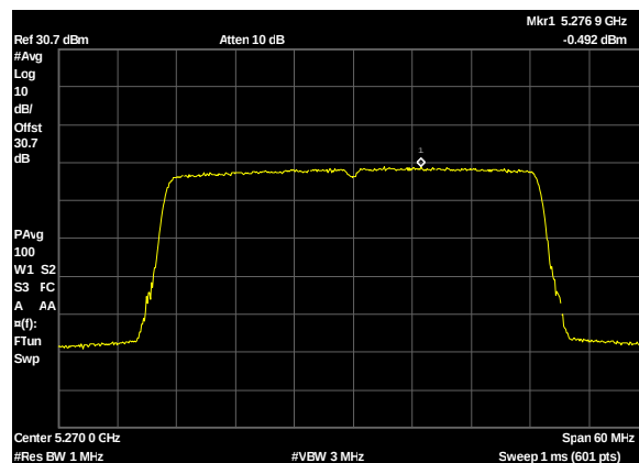
Plot 230. Power Spectral Density, UNII 2A, BW 40M, CF 5270M, c1, 13dBi
