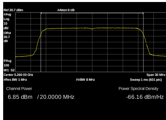
Plot 67. Conducted Transmitter Output Power, UNII 2A, BW 20M, CF 5260M, c0, 19dBi
