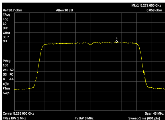
Plot 223. Power Spectral Density, UNII 2A, BW 30M, CF 5265M, c0, 13dBi
