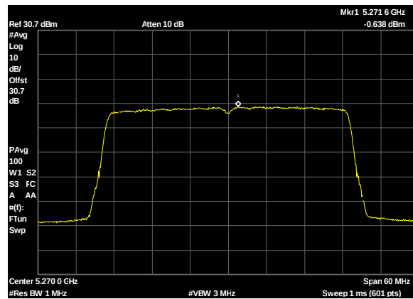
Plot 229. Power Spectral Density, UNII 2A, BW 40M, CF 5270M, c0, 13dBi
