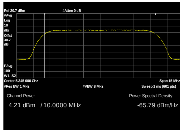
Plot 65. Conducted Transmitter Output Power, UNII 2A, BW 10M, CF 5345M, c0, 19dBi
