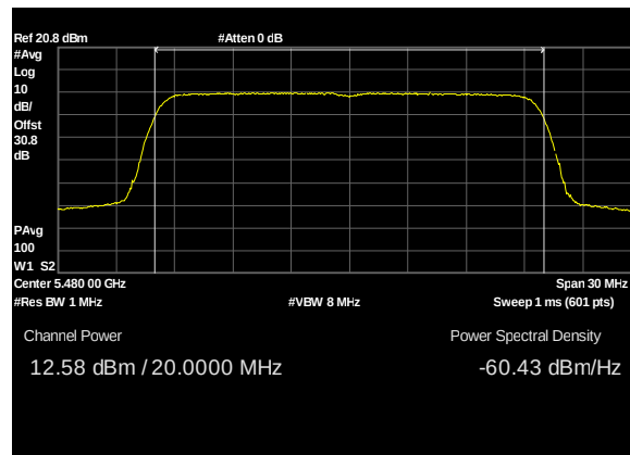
Plot 127. Conducted Transmitter Output Power, UNII 2C, BW 20M, CF 5480M, c0, 13dBi
