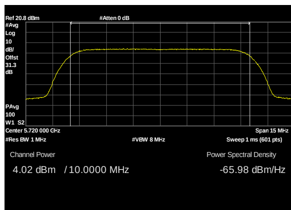
Plot 156. Conducted Transmitter Output Power, UNII 2C, BW 10M, CF 5720M, c1, 19dBi
