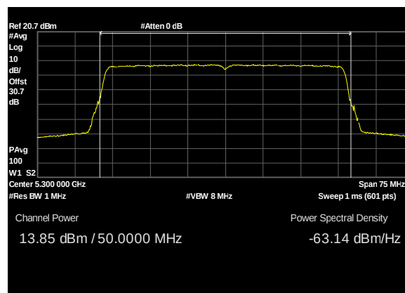
Plot 57. Conducted Transmitter Output Power, UNII 2A, BW 50M, CF 5300M, c0, 13dBi
