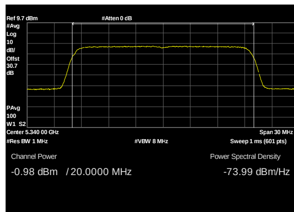
Plot 101. Conducted Transmitter Output Power, UNII 2A, BW 20M, CF 5340M, c0, 27dBi
