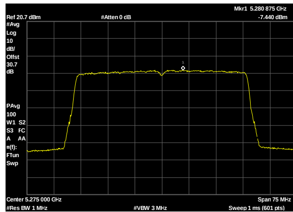
Plot 265. Power Spectral Density, UNII 2A, BW 50M, CF 5275M, c0, 19dBi
