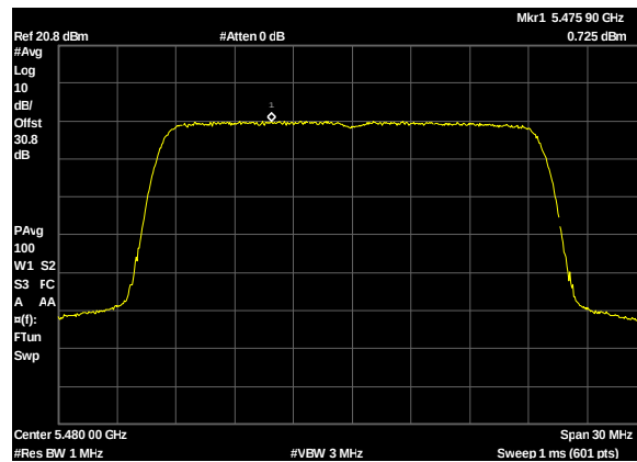
Plot 306. Power Spectral Density, UNII 2C, BW 20M, CF 5480M, c0, 13dBi
