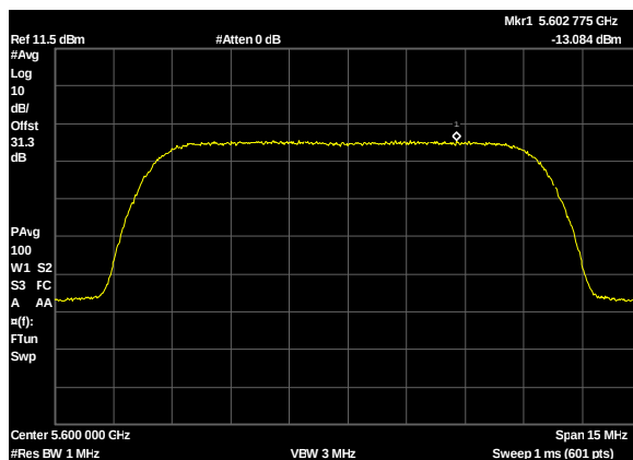
Plot 363. Power Spectral Density, UNII 2C, BW 10W, CF 5600M, c1, 27dBi
