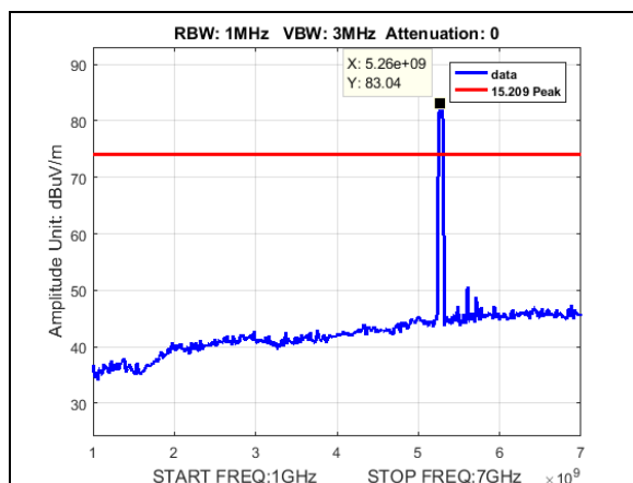
Plot 556. Radiated Spurious Emissions, Peak, BW 50M, CF 5275M, 27dB, 1-7GHz
