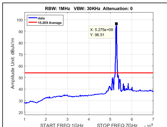
Plot 537. Radiated Spurious Emissions, Average, BW 40M, CF 5270M, 27dBi, 1-7GHz
