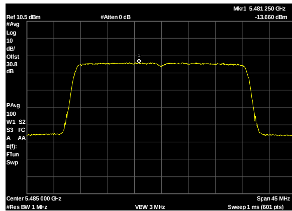
Plot 372. Power Spectral Density, UNII 2C, BW 30W, CF 5485M, c0, 27dBi
