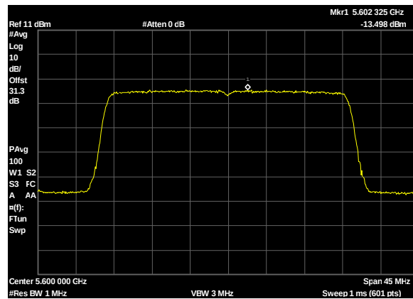
Plot 375. Power Spectral Density, UNII 2C, BW 30W, CF 5600M, c1, 27dBi
