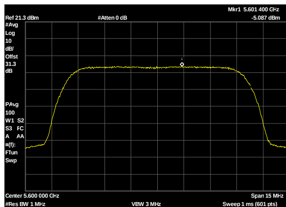
Plot 333. Power Spectral Density, UNII 2C, BW 10M, CF 5600M, c1, 19dBi
