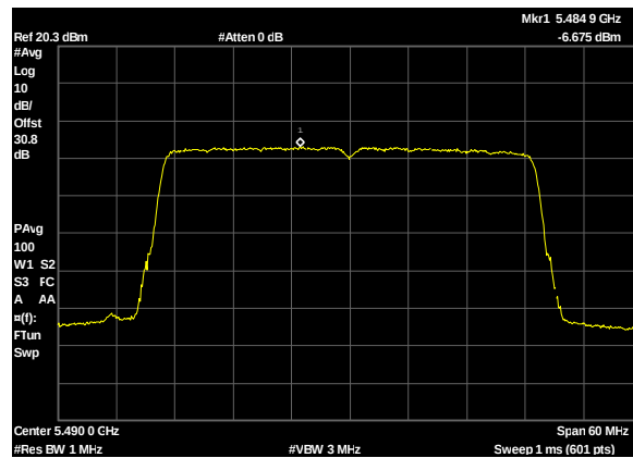
Plot 348. Power Spectral Density, UNII 2C, BW 40M, CF 5490M, c0, 19dBi
