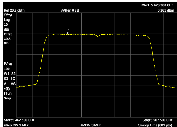
Plot 312. Power Spectral Density, UNII 2C, BW 30M, CF 5485M, c0, 13dBi
