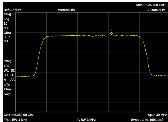
Plot 277. Power Spectral Density, UNII 2A, BW 20M, CF 5260M, c0, 27dBi
