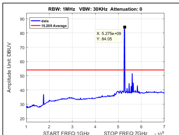
Plot 501. Radiated Spurious Emissions, Average, BW 20M, CF 5260M, 19dBi
