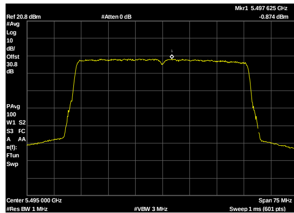
Plot 324. Power Spectral Density, UNII 2C, BW 50M, CF 5495M, c0, 13dBi
