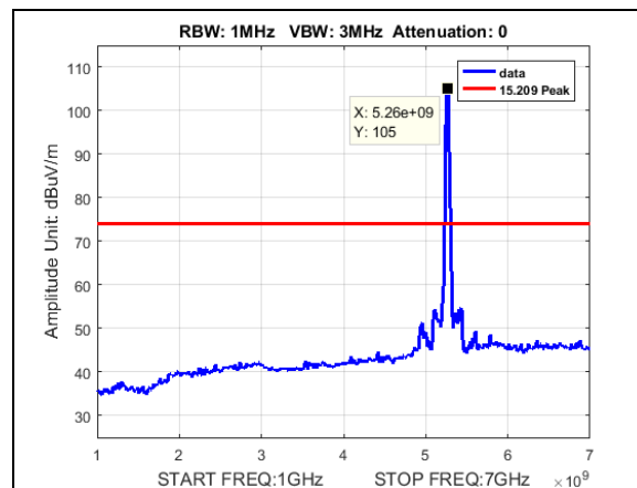
Plot 550. Radiated Spurious Emissions, Peak, BW 30M, CF 5265M, 27dB, 1-7GHz
