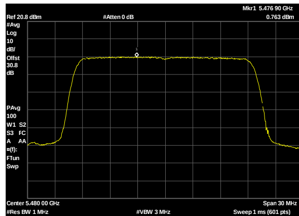
Plot 307. Power Spectral Density, UNII 2C, BW 20M, CF 5480M, c1, 13dBi
