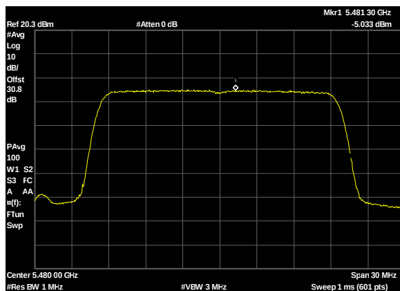
Plot 337. Power Spectral Density, UNII 2C, BW 20M, CF 5480M, c1, 19dBi
