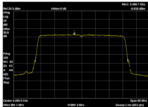
Plot 349. Power Spectral Density, UNII 2C, BW 40M, CF 5490M, c1, 19dBi
