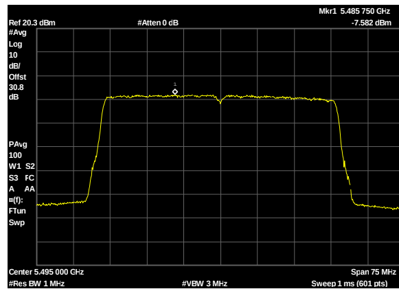
Plot 354. Power Spectral Density, UNII 2C, BW 50M, CF 5495M, c0, 19dBi
