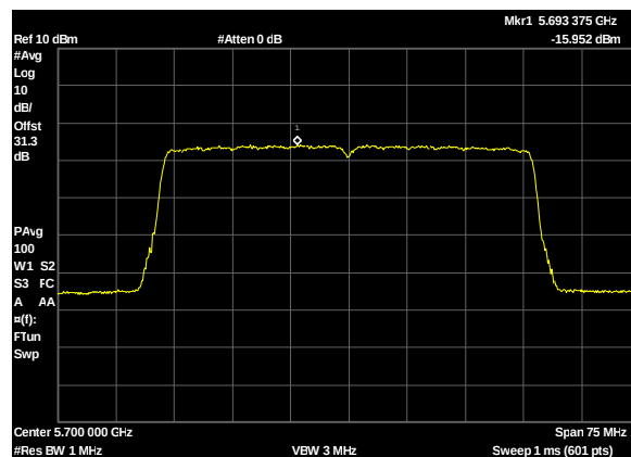
Plot 388. Power Spectral Density, UNII 2C, BW 50W, CF 5700M, c0, 27dBi
