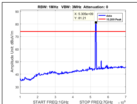
Plot 557. Radiated Spurious Emissions, Peak, BW 50M, CF 5300M, 27dB, 1-7GHz
