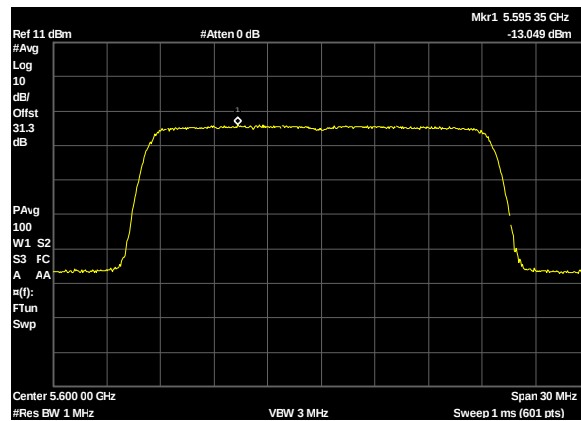
Plot 369. Power Spectral Density, UNII 2C, BW 20W, CF 5600M, c1, 27dBi
