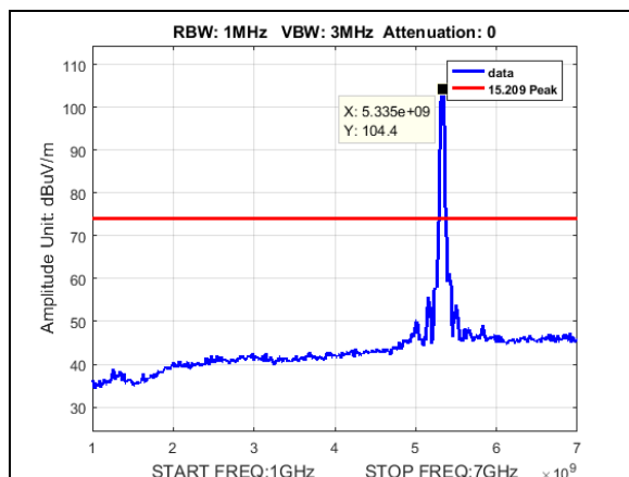
Plot 555. Radiated Spurious Emissions, Peak, BW 40M, CF 5330M, 27dB, 1-7GHz
