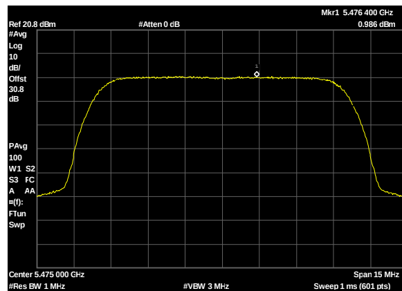
Plot 301. Power Spectral Density, UNII 2C, BW 10M, CF 5475M, c1, 13dBi
