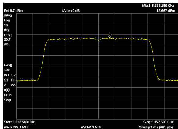
Plot 287. Power Spectral Density, UNII 2A, BW 30M, CF 5335M, c0, 27dBi
