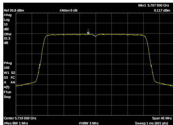
Plot 316. Power Spectral Density, UNII 2C, BW 30M, CF 5710M, c0, 13dBi
