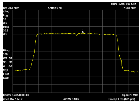
Plot 355. Power Spectral Density, UNII 2C, BW 50M, CF 5495M, c1, 19dBi
