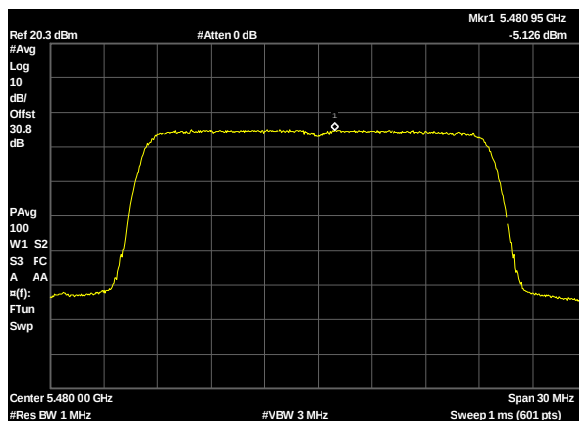
Plot 336. Power Spectral Density, UNII 2C, BW 20M, CF 5480M, c0, 19dBi
