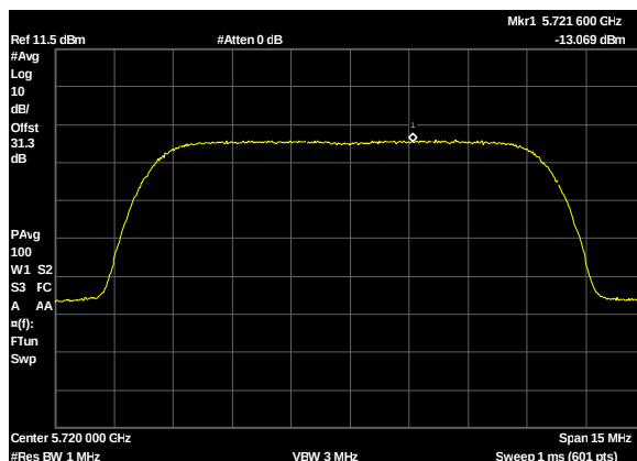
Plot 364. Power Spectral Density, UNII 2C, BW 10W, CF 5720M, c0, 27dBi
