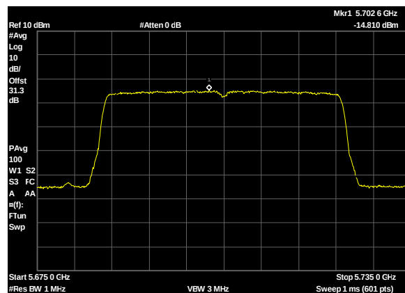
Plot 382. Power Spectral Density, UNII 2C, BW 40W, CF 5705M, c0, 27dBi
