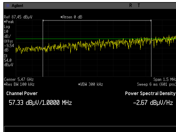
Plot 489. Undesirable Emissions, Peak, Radiated Bandedge 5470M, BW 50M, CF 5495M, 27dB
