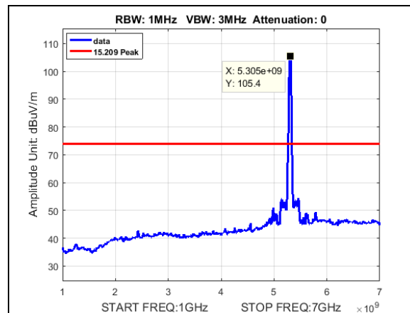
Plot 551. Radiated Spurious Emissions, Peak, BW 30M, CF 5300M, 27dB, 1-7GHz
