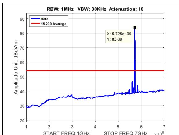
Plot 594. Radiated Spurious Emissions, Average, BW 10M, CF 5720M, 27dBi
