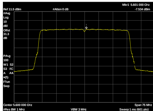
Plot 357. Power Spectral Density, UNII 2C, BW 50M, CF 5600M, c1, 19dBi
