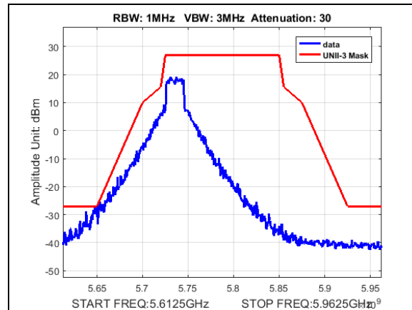
Plot 178. Undesirable Emissions, UNII3, emission mask, BW 20M, CF 5735M, 19dB
