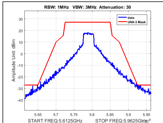
Plot 189. Undesirable Emissions, UNII3, emission mask, BW 30M, CF 5790M, 13dBm
