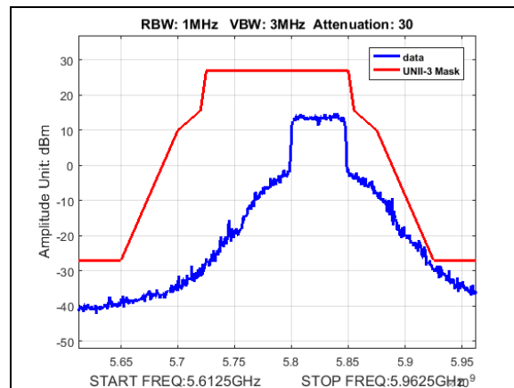
Plot 210. Undesirable Emissions, UNII3, emission mask, BW 50M, CF 5825M, 13dBm
