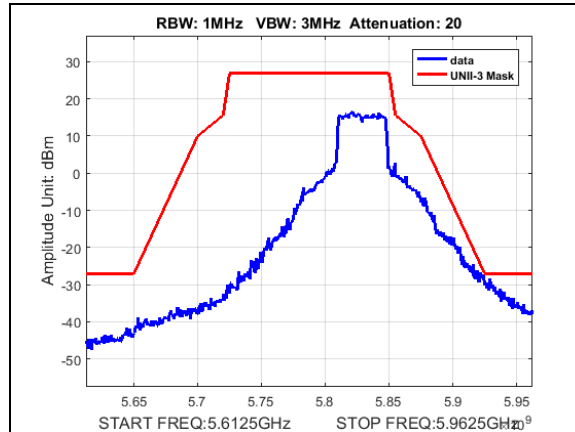
Plot 202. Undesirable Emissions, UNII3, emission mask, BW 40M, CF 5830M, 19dBi
