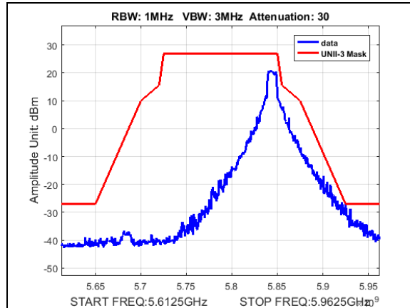
Plot 175. Undesirable Emissions, UNII3, emission mask, BW 10M, CF 5845M, 19dBi
