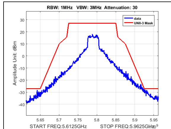
Plot 190. Undesirable Emissions, UNII3, emission mask, BW 30M, CF 5790M, 19dBi
