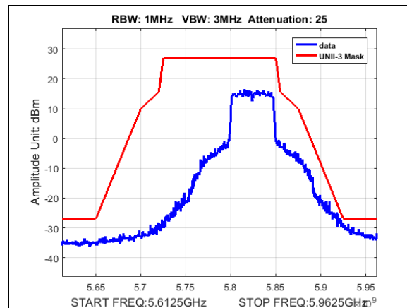
Plot 212. Undesirable Emissions, UNII3, emission mask, BW 50M, CF 5825M, 27dBm
