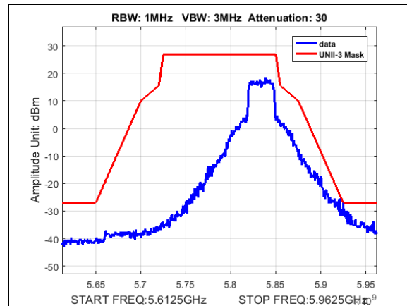
Plot 193. Undesirable Emissions, UNII3, emission mask, BW 30M, CF 5835M, 19dBi
