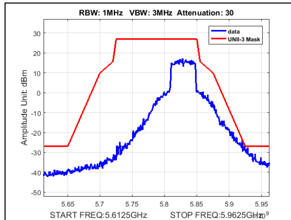
Plot 201. Undesirable Emissions, UNII3, emission mask, BW 40M, CF 5830M, 13dBi
