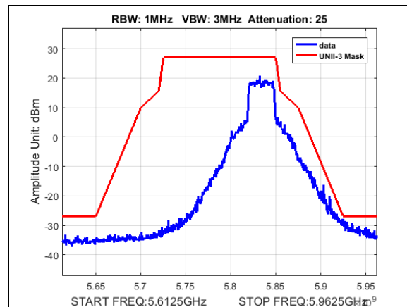
Plot 194. Undesirable Emissions, UNII3, emission mask, BW 30M, CF 5835M, 27dBi
