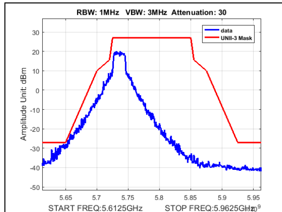
Plot 177. Undesirable Emissions, UNII3, emission mask, BW 20M, CF 5735M, 13dBi
