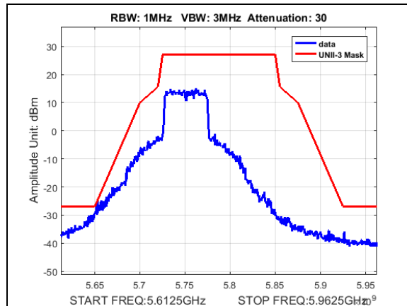
Plot 204. Undesirable Emissions, UNII3, emission mask, BW 50M, CF 5750M, 13dBi
