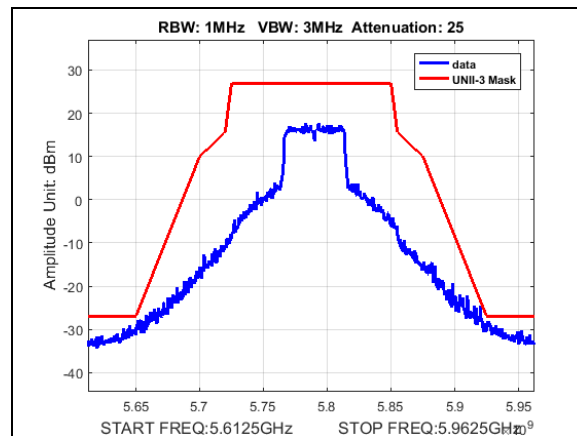
Plot 209. Undesirable Emissions, UNII3, emission mask, BW 50M, CF 5790M, 27dBm
