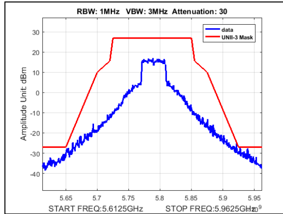
Plot 199. Undesirable Emissions, UNII3, emission mask, BW 40M, CF 5790M, 19dBi
