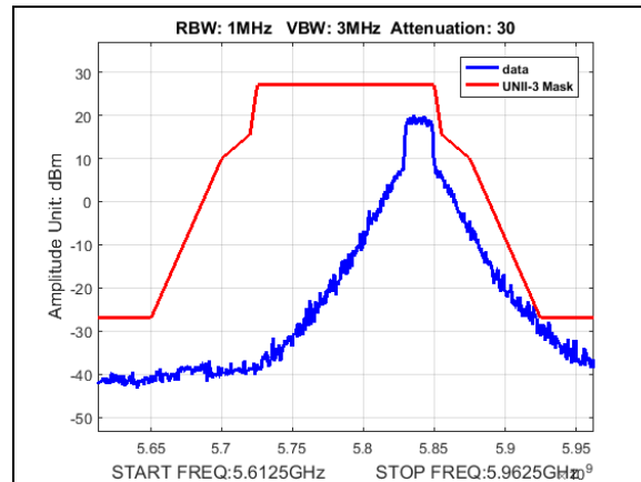
Plot 184. Undesirable Emissions, UNII3, emission mask, BW 20M, CF 5840M, 19dBi
