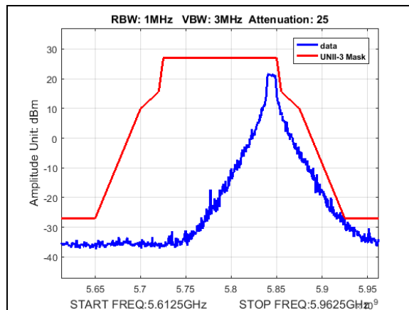
Plot 176. Undesirable Emissions, UNII3, emission mask, BW 10M, CF 5845M, 27dBi
