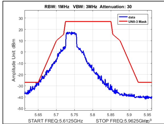
Plot 187. Undesirable Emissions, UNII3, emission mask, BW 30M, CF 5740M, 19dBm
