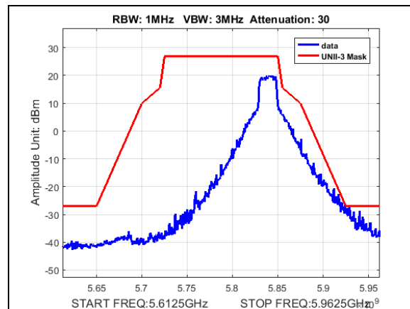
Plot 183. Undesirable Emissions, UNII3, emission mask, BW 20M, CF 5840M, 13dBi
