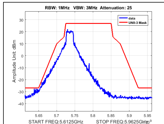
Plot 179. Undesirable Emissions, UNII3, emission mask, BW 20M, CF 5735M, 27dB
