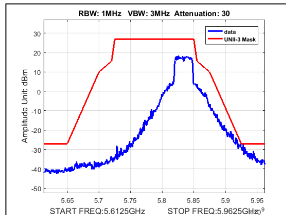
Plot 192. Undesirable Emissions, UNII3, emission mask, BW 30M, CF 5835M, 13dBi
