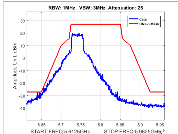
Plot 188. Undesirable Emissions, UNII3, emission mask, BW 30M, CF 5740M, 27dBm
