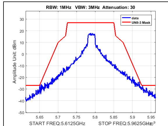
Plot 181. Undesirable Emissions, UNII3, emission mask, BW 20M, CF 5790M, 19dBi
