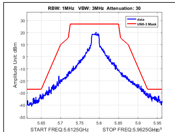
Plot 180. Undesirable Emissions, UNII3, emission mask, BW 20M, CF 5790M, 13dB
