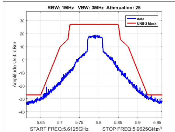
Plot 200. Undesirable Emissions, UNII3, emission mask, BW 40M, CF 5790M, 27dBi
