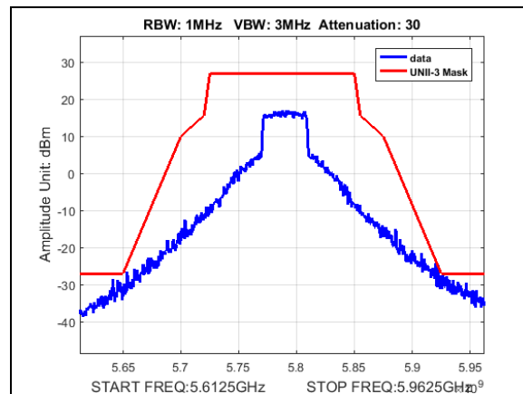
Plot 198. Undesirable Emissions, UNII3, emission mask, BW 40M, CF 5790M, 13dB
