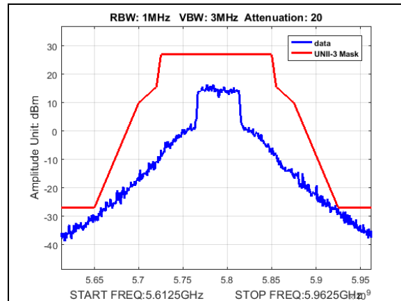
Plot 208. Undesirable Emissions, UNII3, emission mask, BW 50M, CF 5790M, 19dBm
