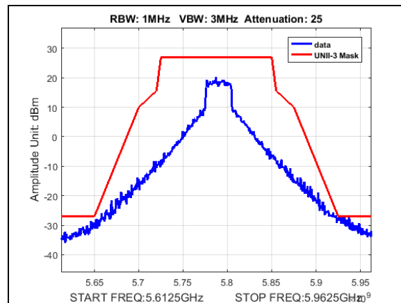
Plot 191. Undesirable Emissions, UNII3, emission mask, BW 30M, CF 5790M, 27dBi
