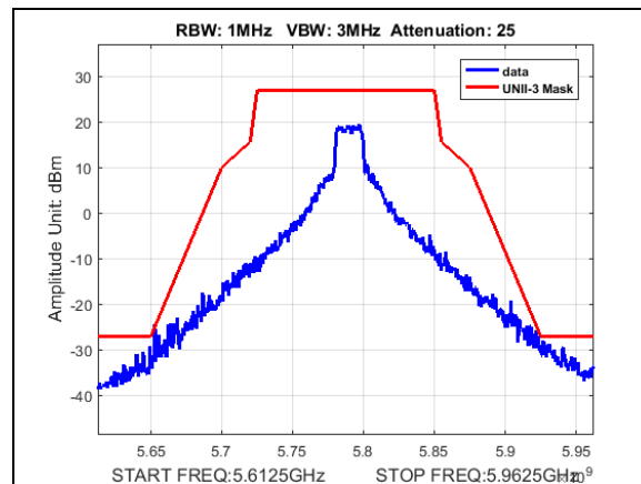
Plot 182. Undesirable Emissions, UNII3, emission mask, BW 20M, CF 5790M, 27dBi
