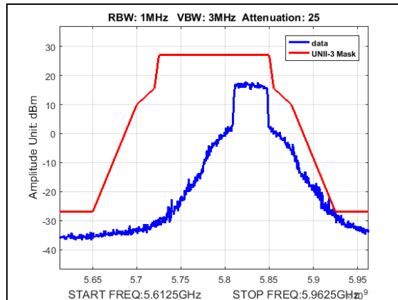
Plot 203. Undesirable Emissions, UNII3, emission mask, BW 40M, CF 5830M, 27dBi
