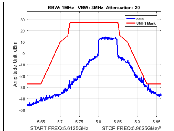
Plot 211. Undesirable Emissions, UNII3, emission mask, BW 50M, CF 5825M, 19dBm
