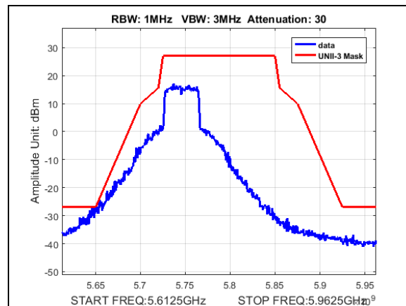
Plot 195. Undesirable Emissions, UNII3, emission mask, BW 40M, CF 5745M, 13dBi
