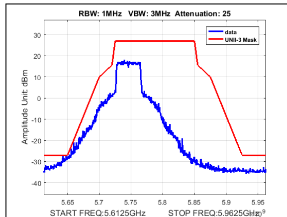
Plot 197. Undesirable Emissions, UNII3, emission mask, BW 40M, CF 5745M, 27dB
