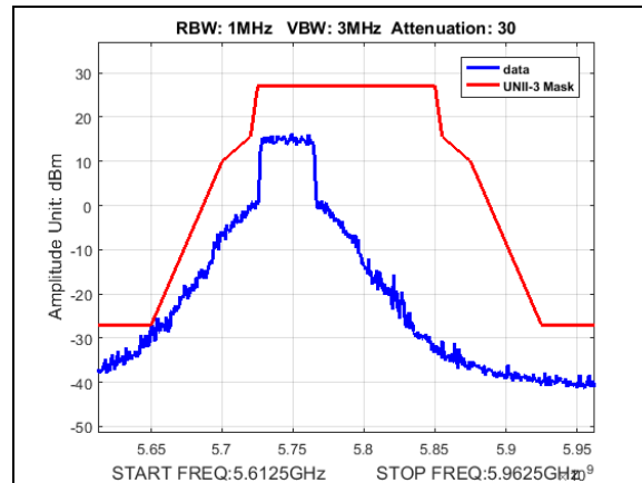
Plot 196. Undesirable Emissions, UNII3, emission mask, BW 40M, CF 5745M, 19dB
