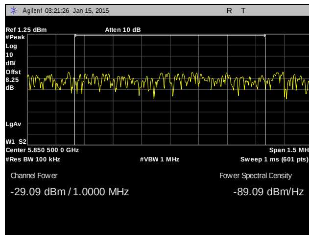
Plot 606. Radiated Emissions, 20 MHz, Channel 5840 MHz, Band Edge 5850, -17 dBm, 34 dBi Antenna
