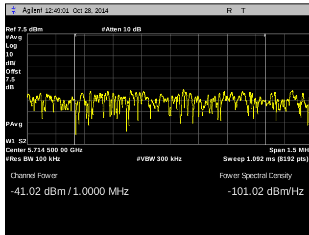
Plot 473. Radiated Band Edge, 5735 MHz, 5715 Band Edge, -27 dBm, 20 MHz, 23 dBi Antenna
