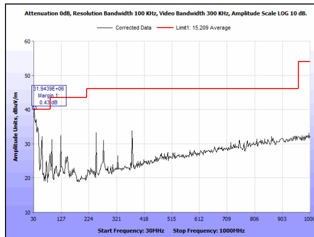
Plot 331. Radiated Spurious Emissions, High Channel, 40 MHz, 30 MHz – 1 GHz
