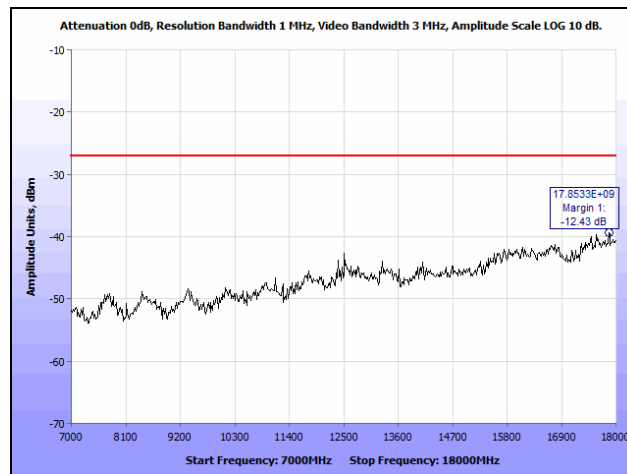
Plot 443. Radiated Band Edge, 5835 MHz, 30 MHz, 7 GHz – 18 GHz
