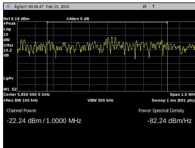
Plot 532. Radiated Band Edge, 5805 MHz, 5850 Band Edge, -17 dBm, 50 MHz, 23 dBi Antenna
