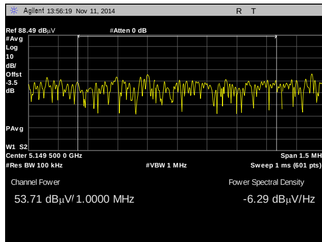
Plot 554. Radiated Restricted Band Emissions, 5178 MHz, Low Edge, 30 MHz, Average
