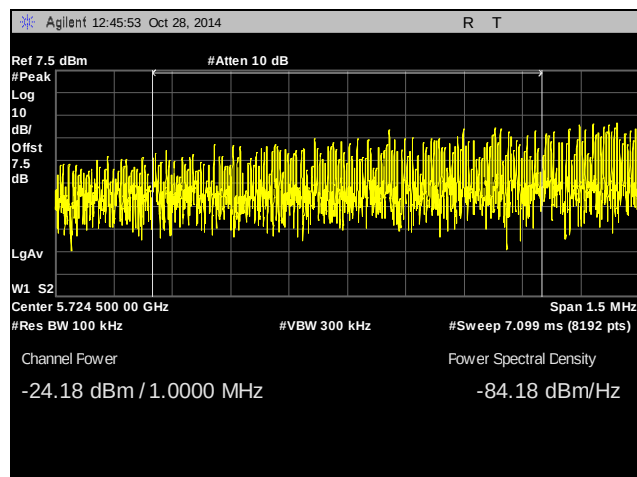
Plot 491. Radiated Band Edge, 5740 MHz, 5725 Band Edge, -17 dBm, 30 MHz, 23 dBi Antenna
