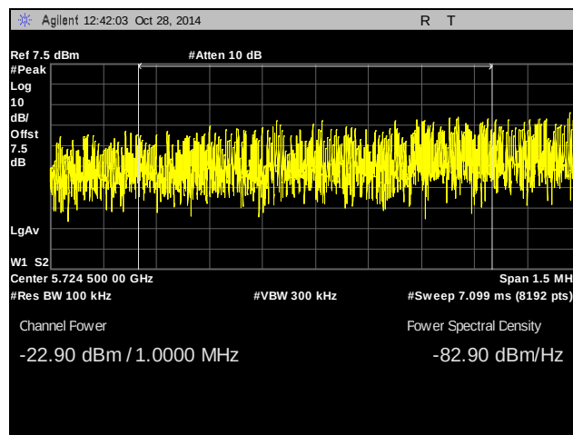
Plot 507. Radiated Band Edge, 5745 MHz, 5725 Band Edge, -17 dBm, 40 MHz, 23 dBi Antenna
