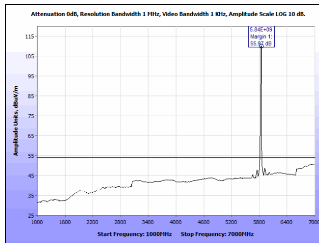
Plot 340. Radiated Spurious Emissions, 10 MHz, 5833 MHz, 1 GHz – 7 GHz, Average, UNII 3, 23 dBi Antenna
