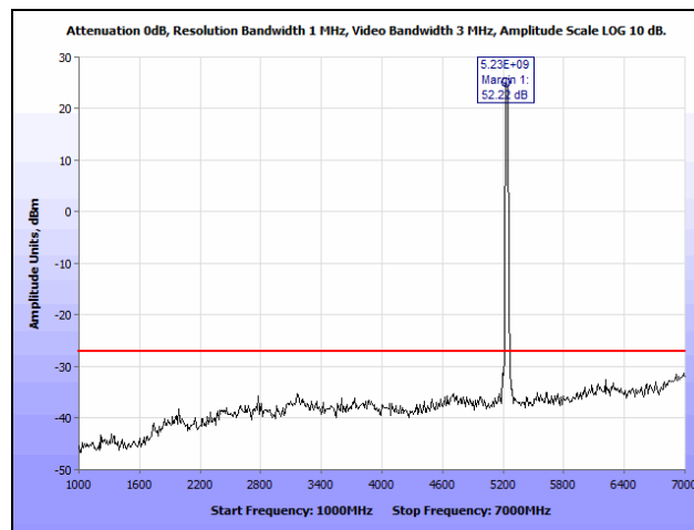
Plot 406. Radiated Band Edge, 5240 MHz, 20 MHz, 1 GHz – 7 GHz
