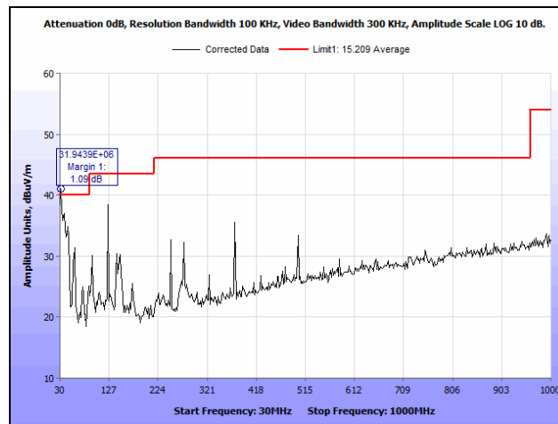
Plot 322. Radiated Spurious Emissions, High Channel, 10 MHz, 30 MHz – 1 GHz
