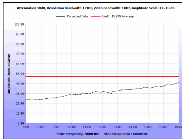
Plot 382. Radiated Spurious Emissions, 40 MHz, 5815 MHz, 7 GHz – 18 GHz, Average, UNII 3, 23 dBi Antenna
