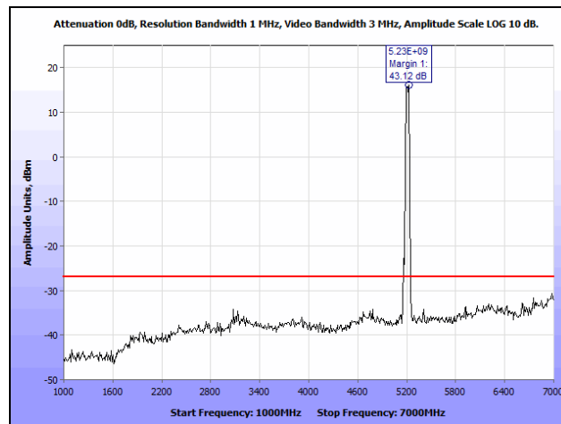
Plot 422. Radiated Band Edge, 5209 MHz, 50 MHz, 1 GHz – 7 GHz
