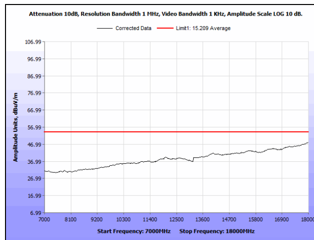
Plot 394. Radiated Spurious Emissions, 50 MHz, 5810 MHz, 7 GHz – 18 GHz, Average, UNII 3, 23 dBi Antenna
