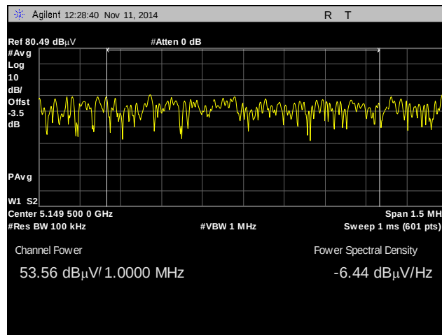
Plot 568. Radiated Restricted Band Emissions, 5180 MHz, Low Edge, 50 MHz, Average
