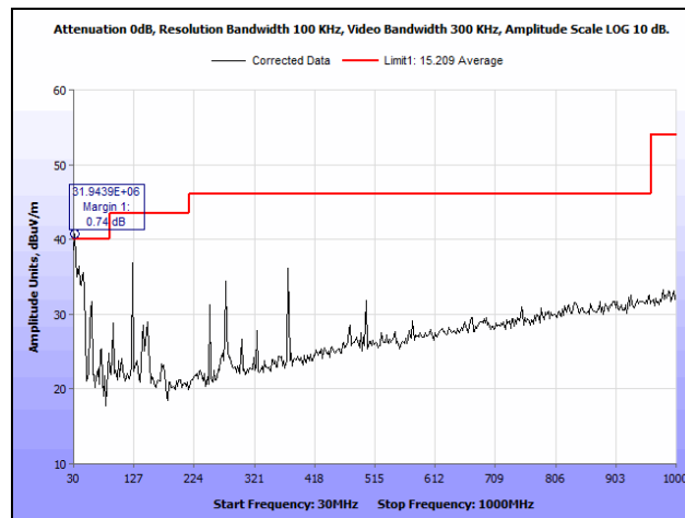
Plot 325. Radiated Spurious Emissions, High Channel, 20 MHz, 30 MHz – 1 GHz
