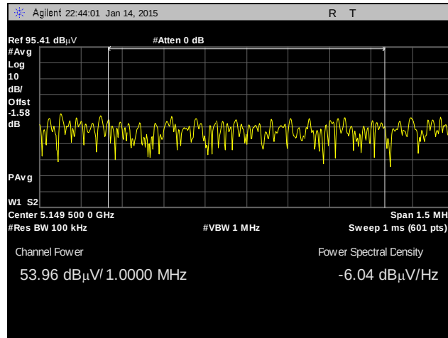
Plot 596. Radiated Emissions, 10 MHz, Channel 5160 MHz, Band Edge 5150, Average 54 Limit, 34 dBi Antenna
