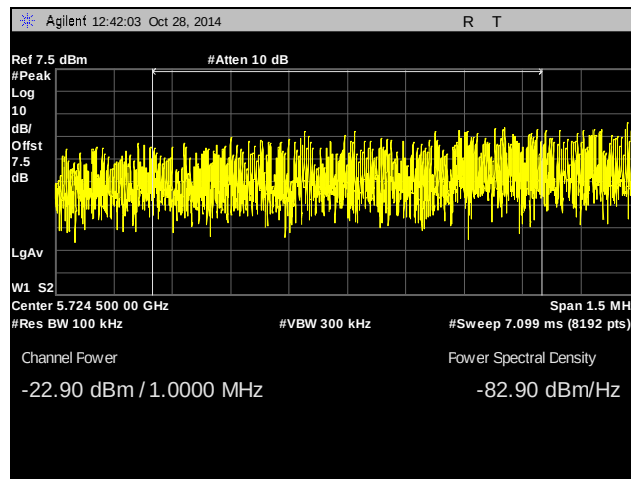
Plot 588. Radiated Restricted Band Emissions, 5745 MHz, Limit: Minus 17, 1 M Integration, 40 MHz
