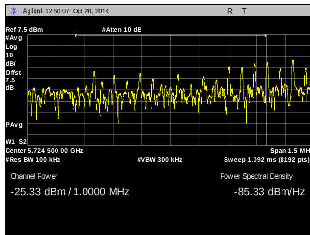
Plot 474. Radiated Band Edge, 5735 MHz, 5725 Band Edge, -17 dBm, 20 MHz, 23 dBi Antenna
