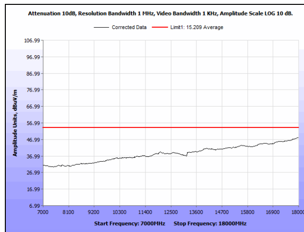
Plot 370. Radiated Spurious Emissions, 30 MHz, 5830 MHz, 7 GHz – 18 GHz, Average, UNII 3, 23 dBi Antenna
