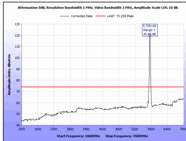
Plot 349. Radiated Spurious Emissions, 20 MHz, 5750 MHz, 1 GHz – 7 GHz, Peak, UNII 3, 23 dBi Antenna
