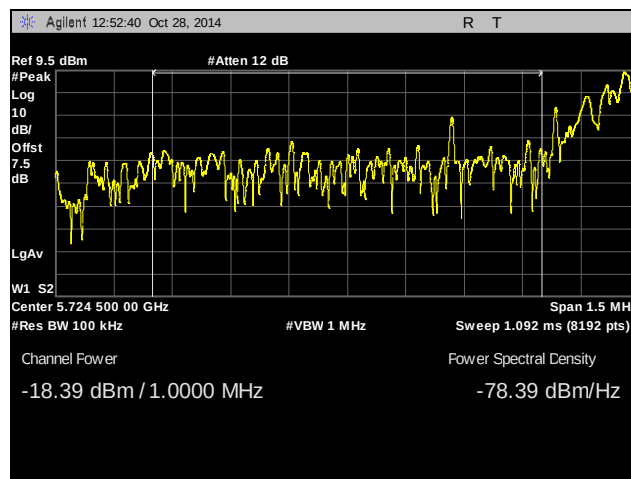
Plot 457. Radiated Band Edge, 5730 MHz, 5725 Band Edge, -17 dBm, 10 MHz, 23 dBi Antenna
