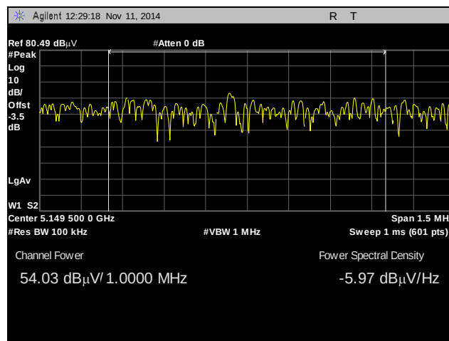
Plot 569. Radiated Restricted Band Emissions, 5180 MHz, Low Edge, 50 MHz, Peak
