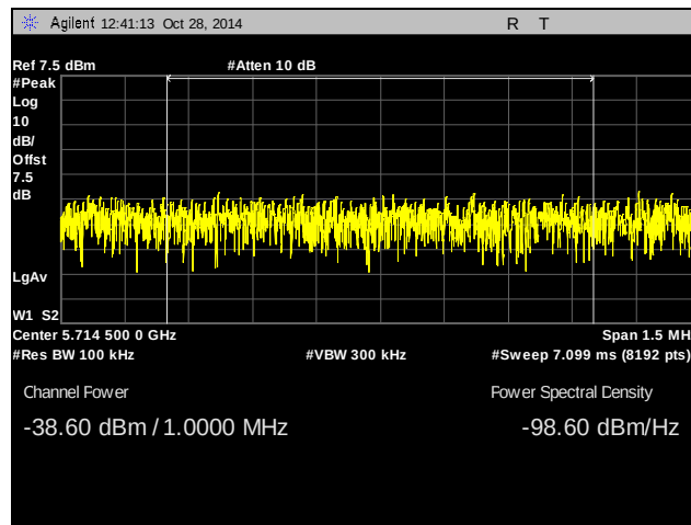
Plot 506. Radiated Band Edge, 5745 MHz, 5715 Band Edge, -27 dBm, 40 MHz, 23 dBi Antenna
