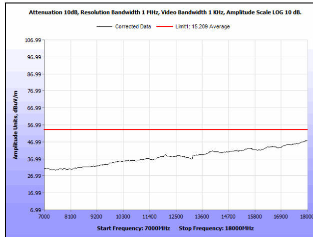
Plot 358. Radiated Spurious Emissions, 20 MHz, 5830 MHz, 7 GHz – 18 GHz, Average, UNII 3, 23 dBi Antenna
