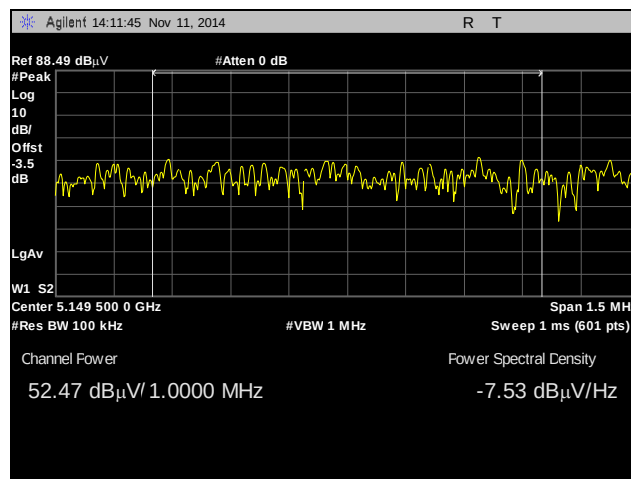
Plot 539. Radiated Restricted Band Emissions, 5160 MHz, Low Edge, 10 MHz, Peak
