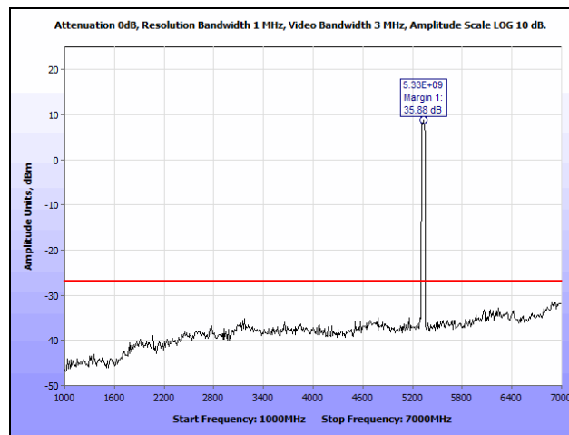
Plot 220. Radiated Spurious Emissions, 40 MHz, High Channel, 1 GHz – 7 GHz, Lower Band
