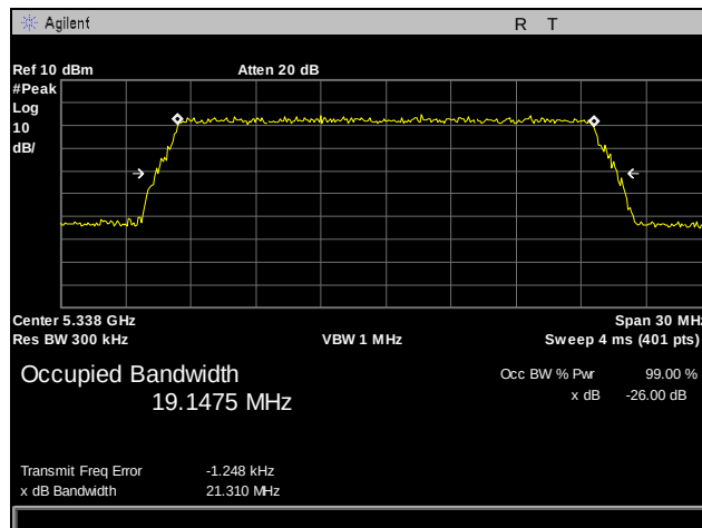
Plot 17. 26 dB Occupied Bandwidth, 5338 MHz, Antenna 1, 20 MHz
