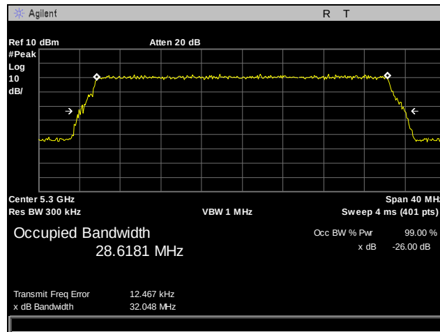
Plot 22. 26 dB Occupied Bandwidth, 5300 MHz, Antenna 1, 30 MHz
