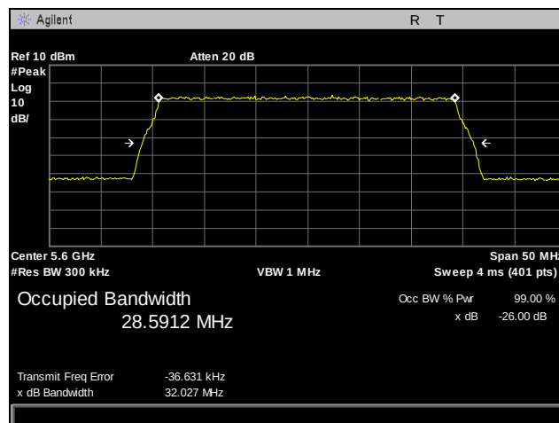
Plot 49. 26 dB Occupied Bandwidth, 5600 MHz, Antenna 0, 30 MHz
