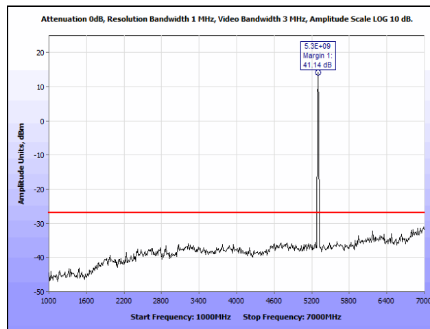
Plot 190. Radiated Spurious Emissions, 10 MHz, Mid Channel, 1 GHz – 7 GHz, Lower Band
