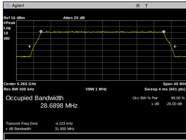
Plot 21. 26 dB Occupied Bandwidth, 5265 MHz, Antenna 1, 30 MHz
