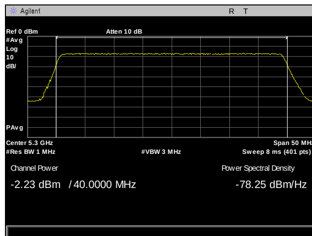
Plot 88. Output Power, 5300 MHz, Antenna 1, 40 MHz
