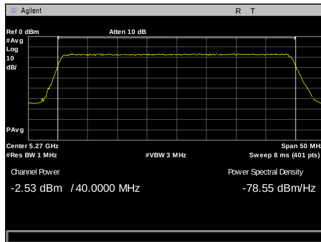
Plot 87. Output Power, 5270 MHz, Antenna 1, 40 MHz
