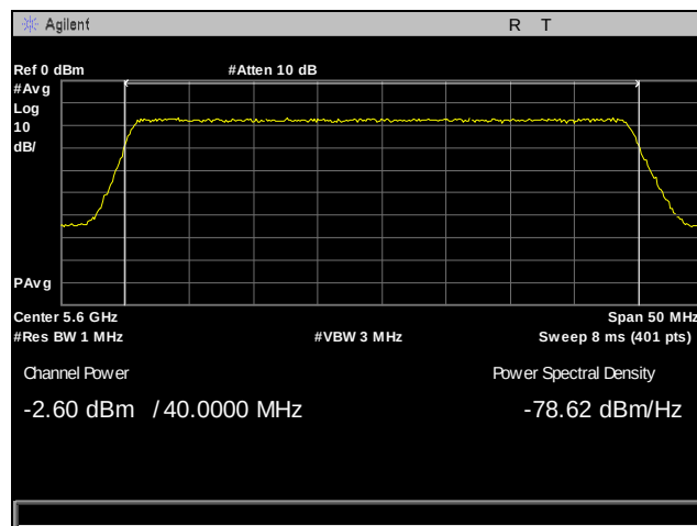
Plot 115. Output Power, 5600 MHz, Antenna 0, 40 MHz
