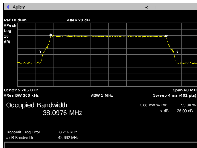
Plot 56. 26 dB Occupied Bandwidth, 5705 MHz, Antenna 0, 40 MHz
