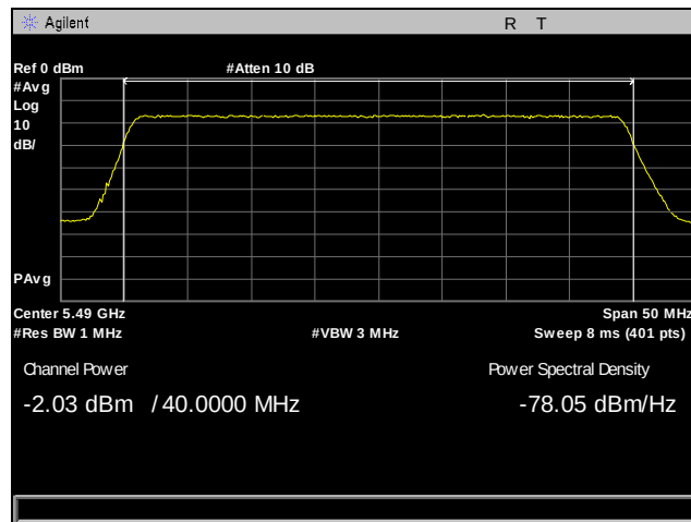
Plot 114. Output Power, 5490 MHz, Antenna 0, 40 MHz
