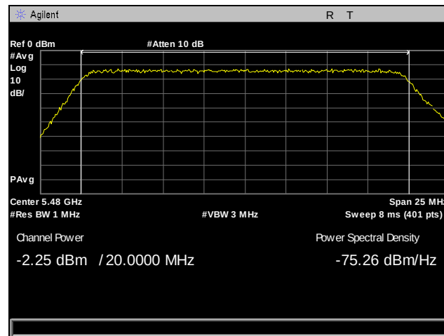
Plot 102. Output Power, 5480 MHz, Antenna 0, 20 MHz
