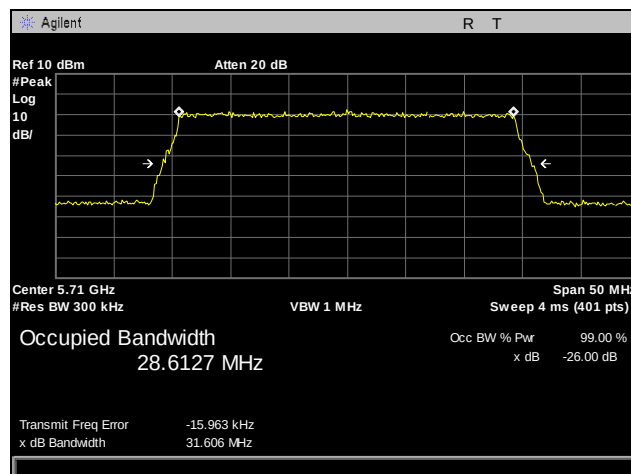
Plot 50. 26 dB Occupied Bandwidth, 5710 MHz, Antenna 0, 30 MHz
