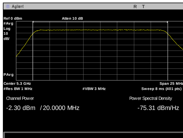
Plot 76. Output Power, 5300 MHz, Antenna 1, 20 MHz
