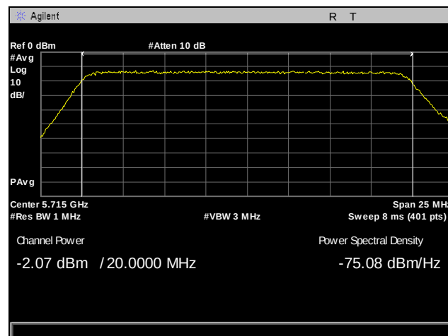
Plot 104. Output Power, 5715 MHz, Antenna 0, 20 MHz
