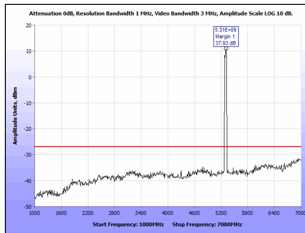
Plot 217. Radiated Spurious Emissions, 40 MHz, Mid Channel, 1 GHz – 7 GHz, Lower Band
