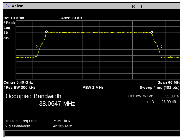
Plot 54. 26 dB Occupied Bandwidth, 5490 MHz, Antenna 0, 40 MHz
