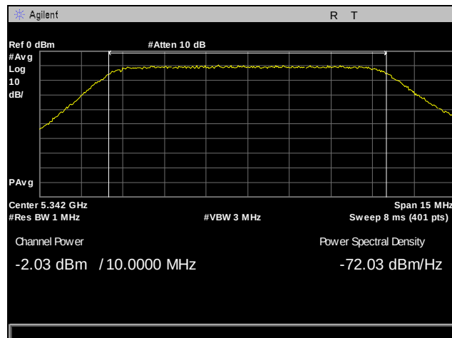
Plot 68. Output Power, 5342 MHz, Antenna 0, 10 MHz
