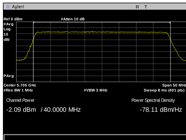
Plot 116. Output Power, 5705 MHz, Antenna 0, 40 MHz
