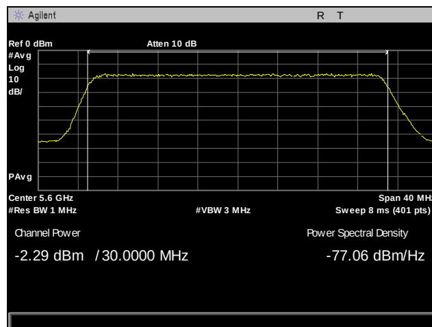
Plot 112. Output Power, 5600 MHz, Antenna 1, 30 MHz
