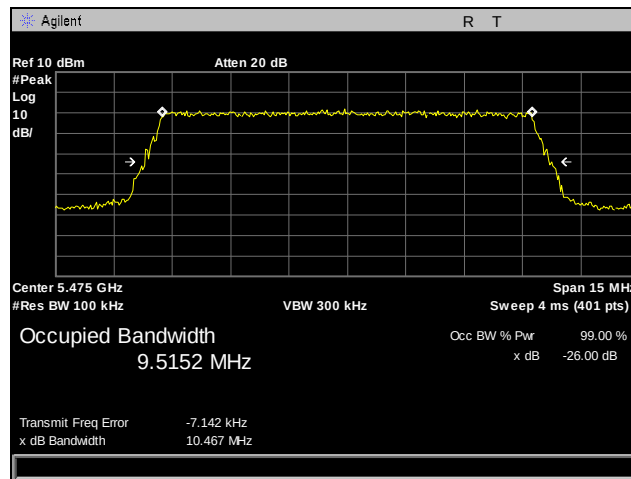
Plot 36. 26 dB Occupied Bandwidth, 5475 MHz, Antenna 0, 10 MHz
