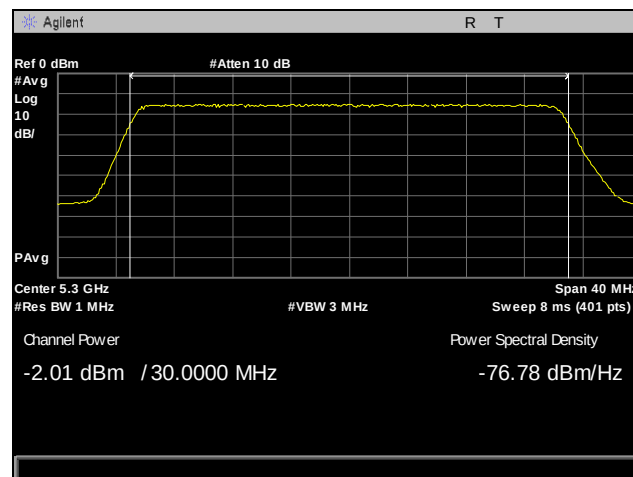
Plot 79. Output Power, 5300 MHz, Antenna 0, 30 MHz
