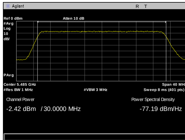
Plot 111. Output Power, 5485 MHz, Antenna 1, 30 MHz
