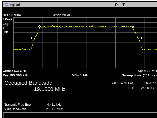
Plot 16. 26 dB Occupied Bandwidth, 5300 MHz, Antenna 1, 20 MHz
