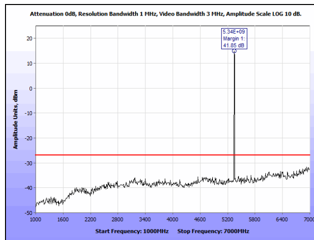
Plot 193. Radiated Spurious Emissions, 10 MHz, High Channel, 1 GHz – 7 GHz, Lower Band
