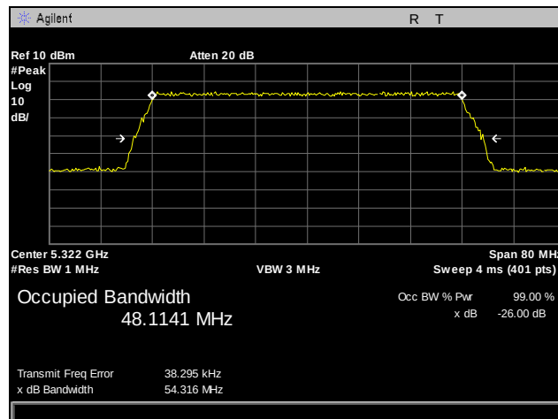
Plot 35. 26 dB Occupied Bandwidth, 5322 MHz, Antenna 1, 50 MHz
