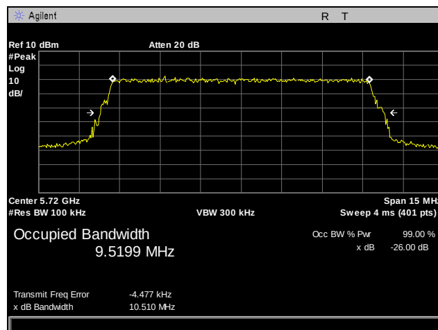
Plot 38. 26 dB Occupied Bandwidth, 5720 MHz, Antenna 0, 10 MHz
