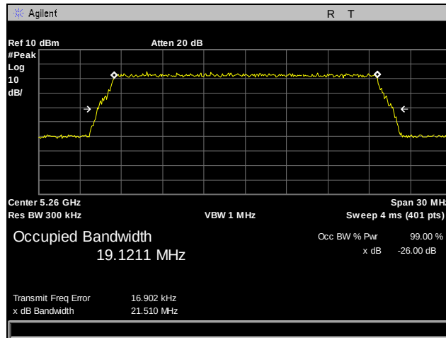
Plot 15. 26 dB Occupied Bandwidth, 5260 MHz, Antenna 1, 20 MHz
