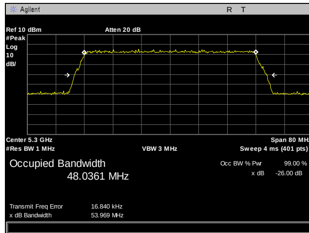
Plot 34. 26 dB Occupied Bandwidth, 5300 MHz, Antenna 1, 50 MHz
