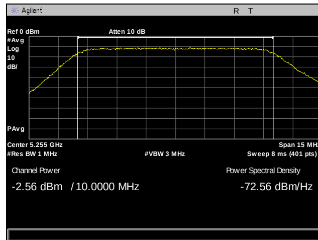
Plot 69. Output Power, 5255 MHz, Antenna 1, 10 MHz
