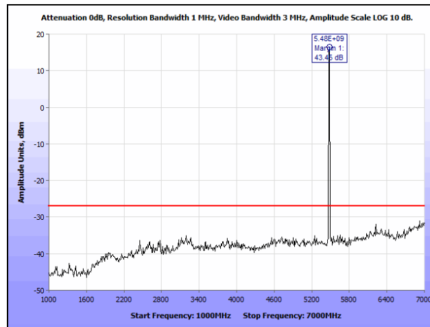
Plot 232. Radiated Spurious Emissions, 10 MHz, Low Channel, 1 GHz – 7 GHz, Upper Band
