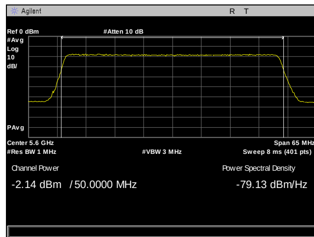
Plot 121. Output Power, 5600 MHz, Antenna 0, 50 MHz
