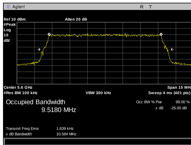
Plot 37. 26 dB Occupied Bandwidth, 5600 MHz, Antenna 0, 10 MHz
