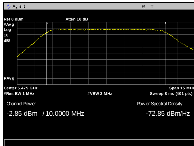
Plot 99. Output Power, 5475 MHz, Antenna 1, 10 MHz
