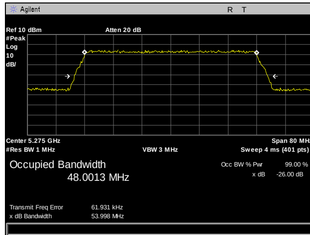
Plot 33. 26 dB Occupied Bandwidth, 5275 MHz, Antenna 1, 50 MHz
