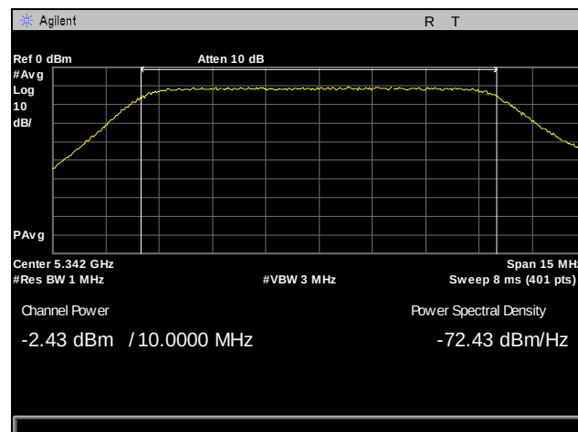
Plot 71. Output Power, 5342 MHz, Antenna 1, 10 MHz
