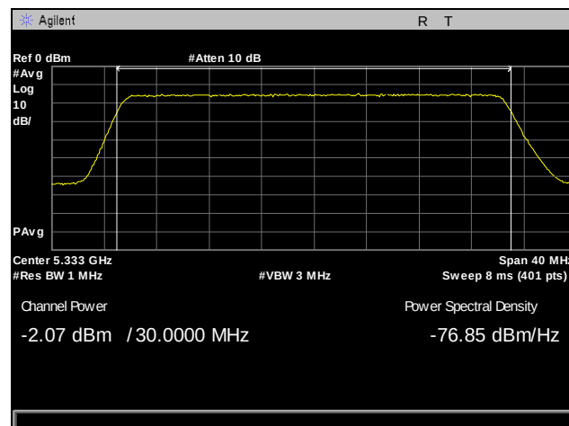
Plot 80. Output Power, 5333 MHz, Antenna 0, 30 MHz
