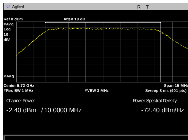
Plot 101. Output Power, 5720 MHz, Antenna 1, 10 MHz
