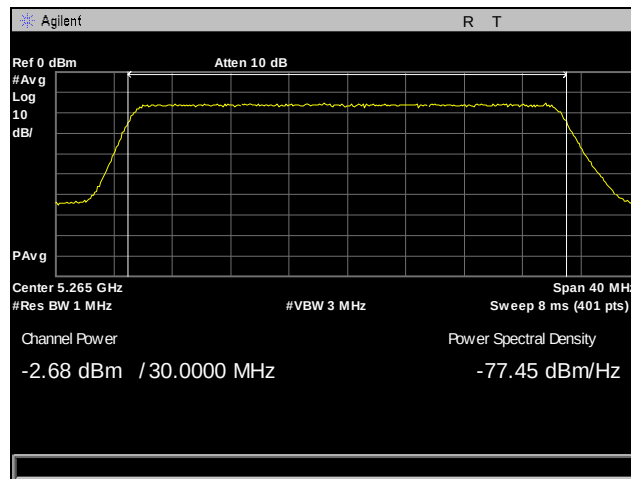
Plot 81. Output Power, 5265 MHz, Antenna 1, 30 MHz
