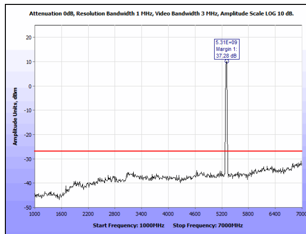
Plot 208. Radiated Spurious Emissions, 30 MHz, Mid Channel, 1 GHz – 7 GHz, Lower Band
