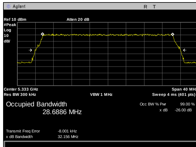
Plot 23. 26 dB Occupied Bandwidth, 5333 MHz, Antenna 1, 30 MHz
