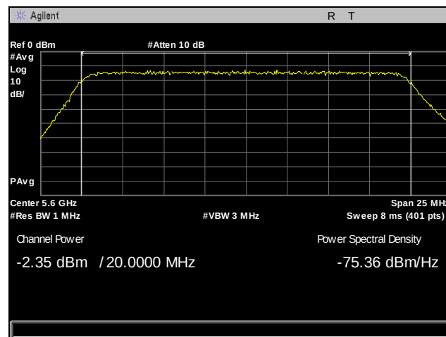
Plot 103. Output Power, 5600 MHz, Antenna 0, 20 MHz
