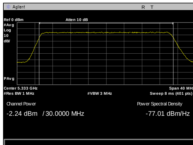
Plot 83. Output Power, 5333 MHz, Antenna 1, 30 MHz
