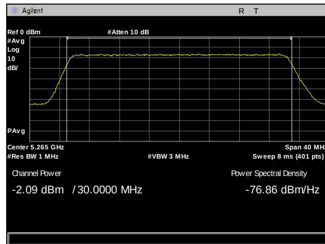
Plot 78. Output Power, 5265 MHz, Antenna 0, 30 MHz
