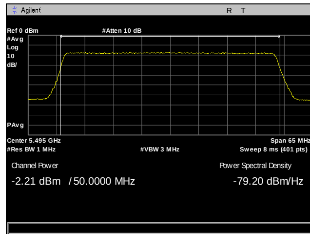
Plot 120. Output Power, 5495 MHz, Antenna 0, 50 MHz
