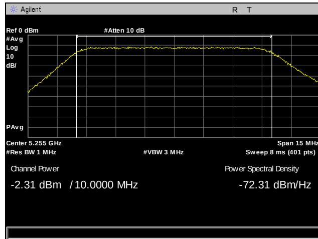
Plot 66. Output Power, 5255 MHz, Antenna 0, 10 MHz
