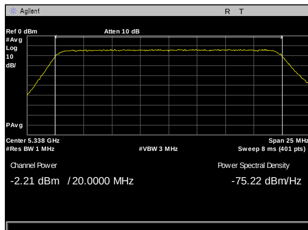
Plot 77. Output Power, 5338 MHz, Antenna 1, 20 MHz
