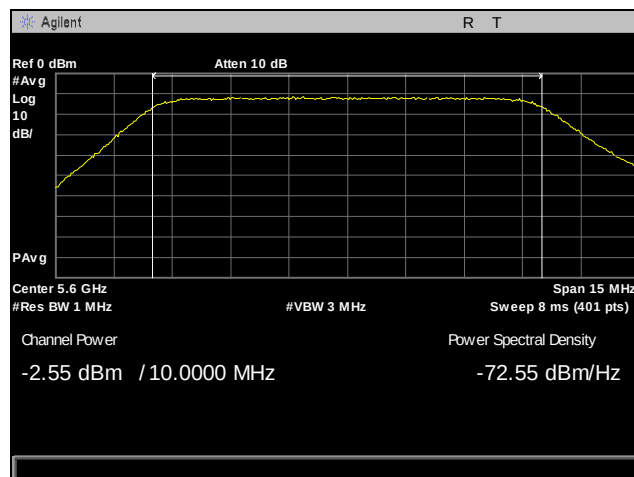
Plot 100. Output Power, 5600 MHz, Antenna 1, 10 MHz
