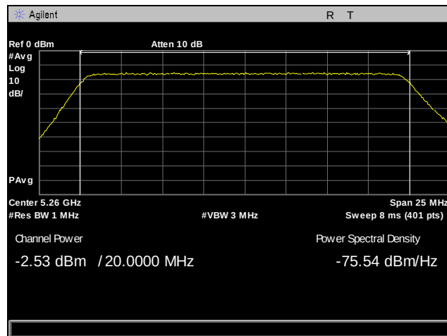
Plot 75. Output Power, 5260 MHz, Antenna 1, 20 MHz
