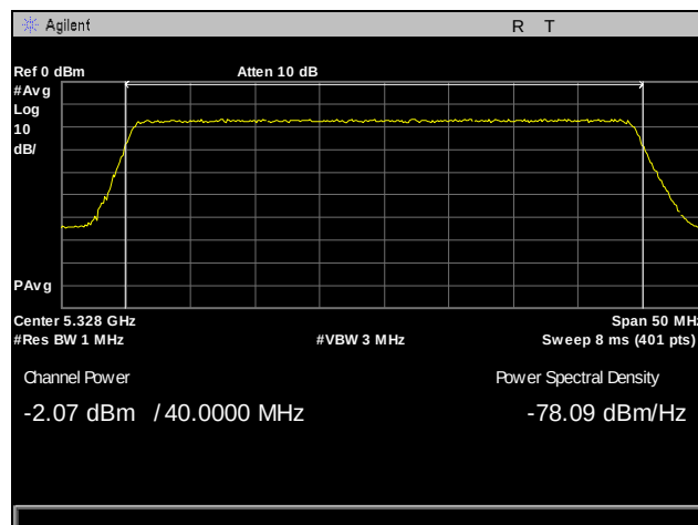
Plot 89. Output Power, 5328 MHz, Antenna 1, 40 MHz
