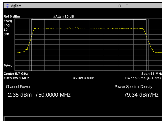
Plot 122. Output Power, 5700 MHz, Antenna 0, 50 MHz
