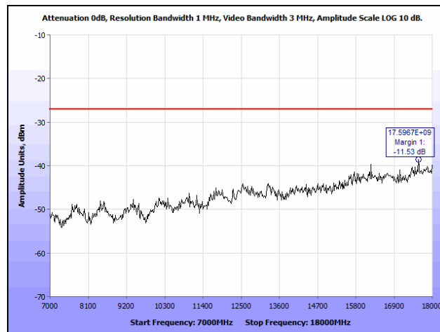
Plot 230. Radiated Spurious Emissions, 50 MHz, High Channel, 7 GHz – 18 GHz, Lower Band
