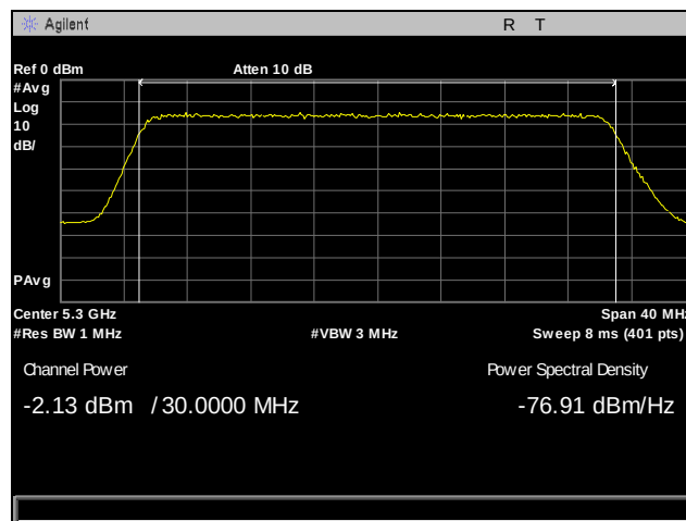
Plot 82. Output Power, 5300 MHz, Antenna 1, 30 MHz
