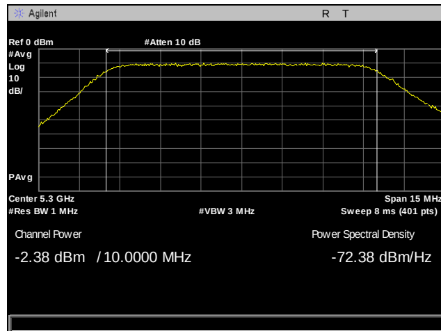
Plot 67. Output Power, 5300 MHz, Antenna 0, 10 MHz
