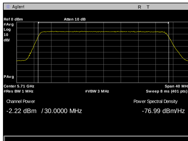
Plot 113. Output Power, 5710 MHz, Antenna 1, 30 MHz
