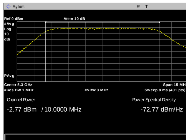
Plot 70. Output Power, 5300 MHz, Antenna 1, 10 MHz
