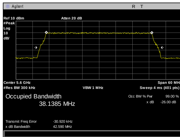
Plot 55. 26 dB Occupied Bandwidth, 5600 MHz, Antenna 0, 40 MHz
