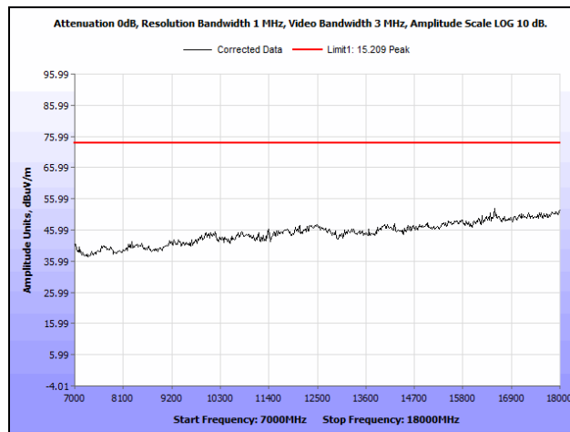
Plot 350. Radiated Spurious Emissions, 50 MHz, High Channel, 7 GHz – 18 GHz, Peak, Lower Band, 23 dBi Antenna
