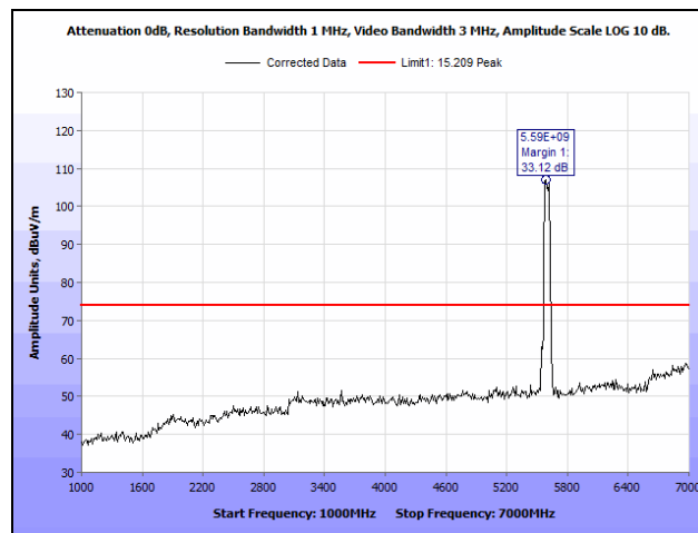
Plot 418. Radiated Spurious Emissions, 50 MHz, Mid Channel, 1 GHz – 7 GHz, Peak, Upper Band, 23 dBi Antenna
