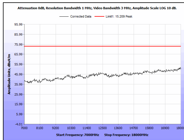
Plot 400. Radiated Spurious Emissions, 40 MHz, Low Channel, 7 GHz – 18 GHz, Peak, Upper Band, 23 dBi Antenna
