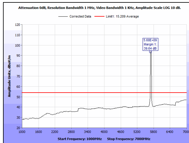
Plot 422. Radiated Spurious Emissions, 50 MHz, High Channel, 1 GHz – 7 GHz, Average, Upper Band, 23 dBi Antenna
