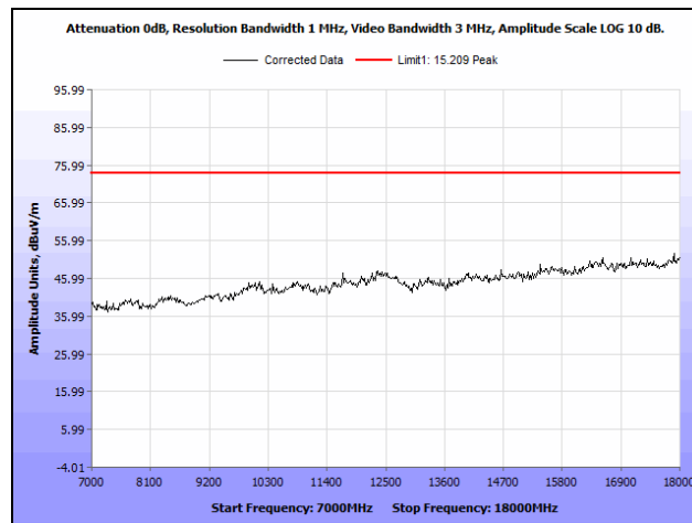
Plot 380. Radiated Spurious Emissions, 20 MHz, High Channel, 7 GHz – 18 GHz, Peak, Upper Band, 23 dBi Antenna
