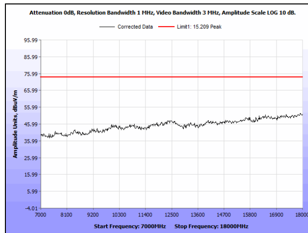
Plot 410. Radiated Spurious Emissions, 40 MHz, High Channel, 7 GHz – 18 GHz, Peak, Upper Band, 23 dBi Antenna
