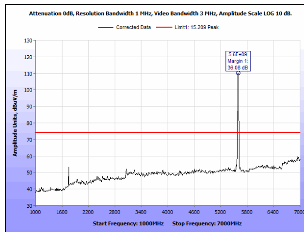
Plot 373. Radiated Spurious Emissions, 20 MHz, Mid Channel, 1 GHz – 7 GHz, Peak, Upper Band, 23 dBi Antenna
