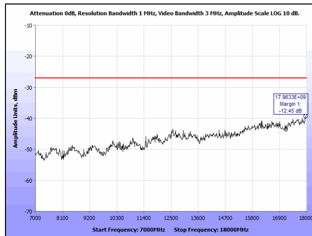
Plot 242. Radiated Spurious Emissions, 20 MHz, Low Channel, 7 GHz – 18 GHz, Upper Band
