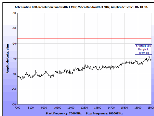
Plot 260. Radiated Spurious Emissions, 40 MHz, Low Channel, 7 GHz – 18 GHz, Upper Band
