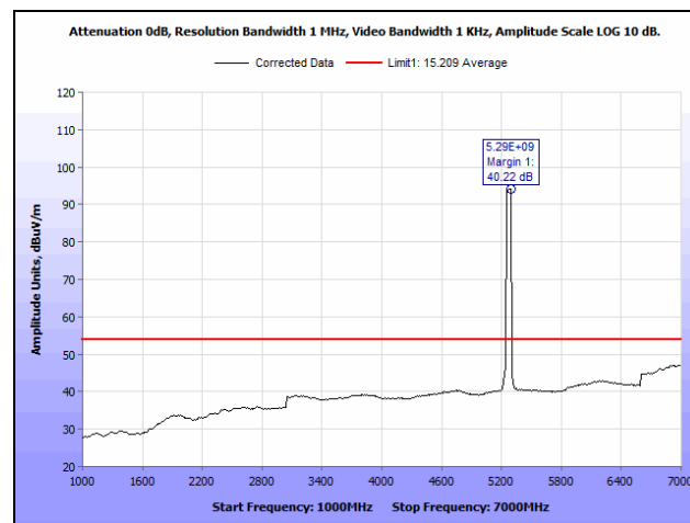
Plot 337. Radiated Spurious Emissions, 50 MHz, Low Channel, 1 GHz – 7 GHz, Average, Lower Band, 23 dBi Antenna
