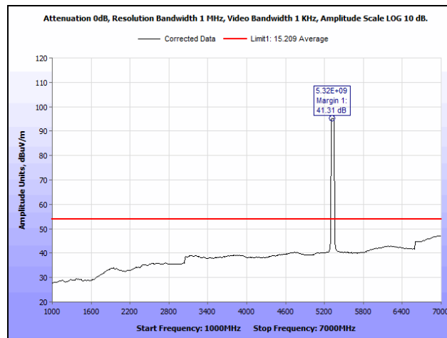
Plot 332. Radiated Spurious Emissions, 40 MHz, High Channel, 1 GHz – 7 GHz, Average, Lower Band, 23 dBi Antenna
