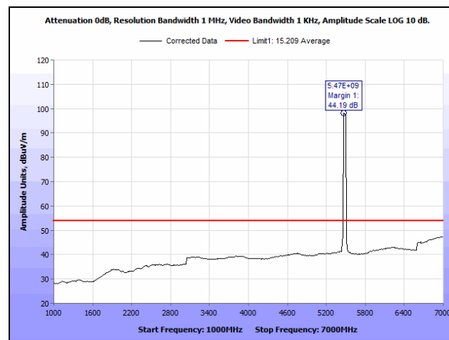
Plot 382. Radiated Spurious Emissions, 30 MHz, Low Channel, 1 GHz – 7 GHz, Average, Upper Band, 23 dBi Antenna
