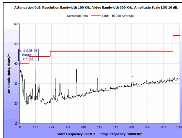
Plot 281. Radiated Spurious Emissions, 10 MHz, Mid Channel, 30 MHz – 1 GHz, Lower Band, 23 dBi Antenna
