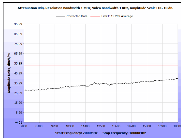
Plot 394. Radiated Spurious Emissions, 30 MHz, High Channel, 7 GHz – 18 GHz, Average, Upper Band, 23 dBi Antenna
