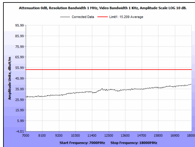
Plot 359. Radiated Spurious Emissions, 10 MHz, Mid Channel, 7 GHz – 18 GHz, Average, Upper Band, 23 dBi Antenna
