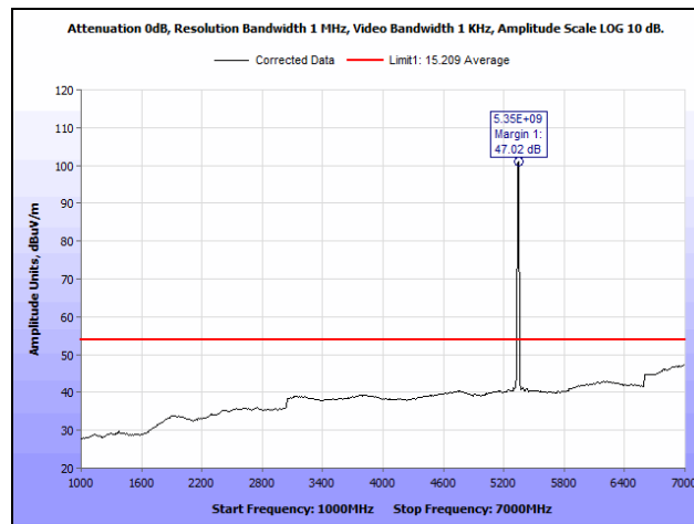
Plot 287. Radiated Spurious Emissions, 10 MHz, High Channel, 1 GHz – 7 GHz, Average, Lower Band, 23 dBi Antenna
