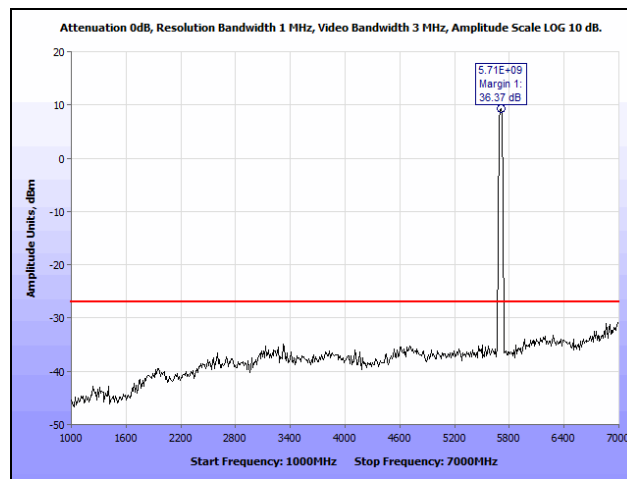
Plot 265. Radiated Spurious Emissions, 40 MHz, High Channel, 1 GHz – 7 GHz, Upper Band
