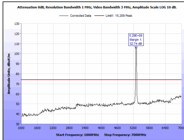
Plot 328. Radiated Spurious Emissions, 40 MHz, Mid Channel, 1 GHz – 7 GHz, Peak, Lower Band, 23 dBi Antenna
