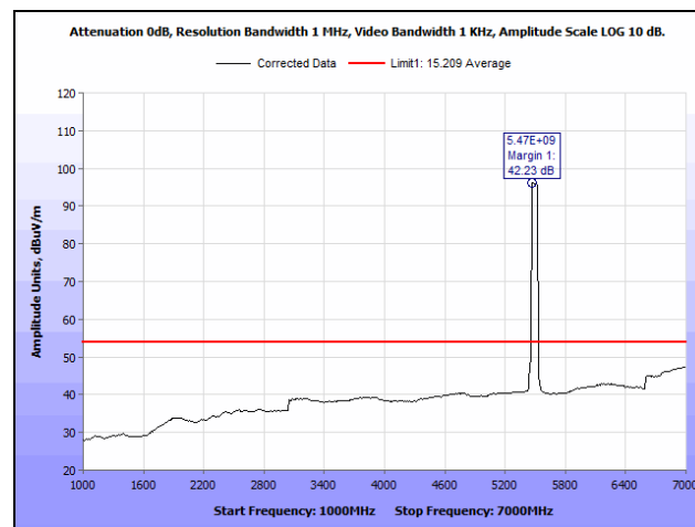
Plot 412. Radiated Spurious Emissions, 50 MHz, Low Channel, 1 GHz – 7 GHz, Average, Upper Band, 23 dBi Antenna
