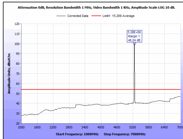
Plot 277. Radiated Spurious Emissions, 10 MHz, Low Channel, 1 GHz – 7 GHz, Average, Lower Band, 23 dBi Antenna
