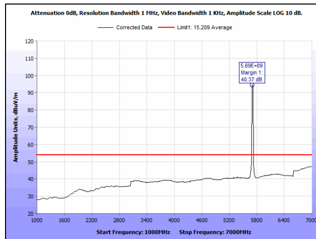
Plot 407. Radiated Spurious Emissions, 40 MHz, High Channel, 1 GHz – 7 GHz, Average, Upper Band, 23 dBi Antenna
