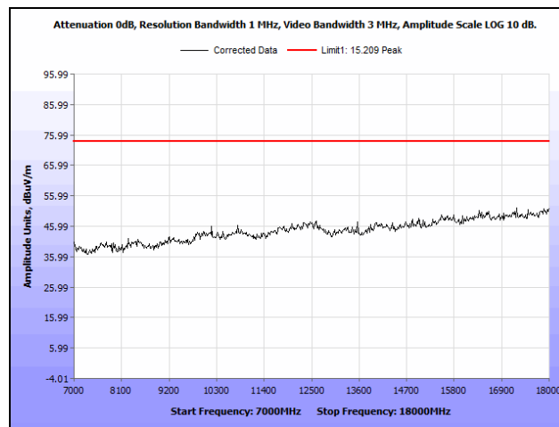
Plot 355. Radiated Spurious Emissions, 10 MHz, Low Channel, 7 GHz – 18 GHz, Peak, Upper Band, 23 dBi Antenna
