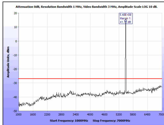
Plot 241. Radiated Spurious Emissions, 20 MHz, Low Channel, 1 GHz – 7 GHz, Upper Band
