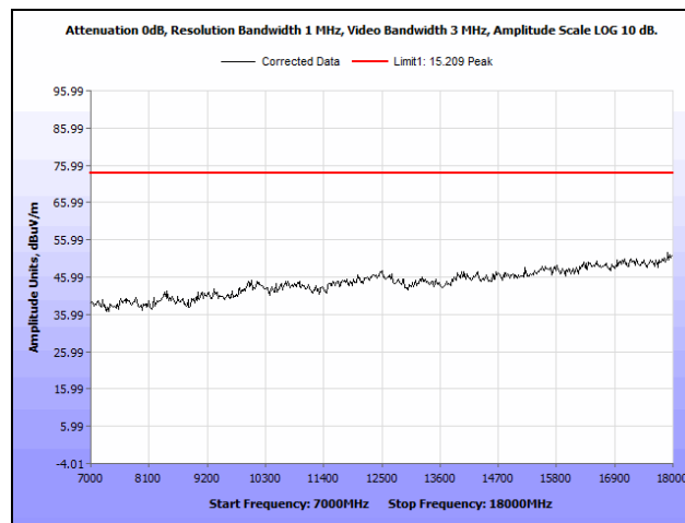
Plot 310. Radiated Spurious Emissions, 30 MHz, Low Channel, 7 GHz – 18 GHz, Peak, Lower Band, 23 dBi Antenna
