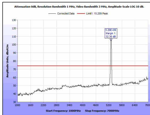
Plot 343. Radiated Spurious Emissions, 50 MHz, Mid Channel, 1 GHz – 7 GHz, Peak, Lower Band, 23 dBi Antenna
