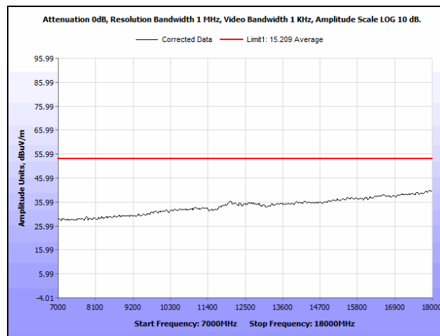
Plot 424. Radiated Spurious Emissions, 50 MHz, High Channel, 7 GHz – 18 GHz, Average, Upper Band, 23 dBi Antenna
