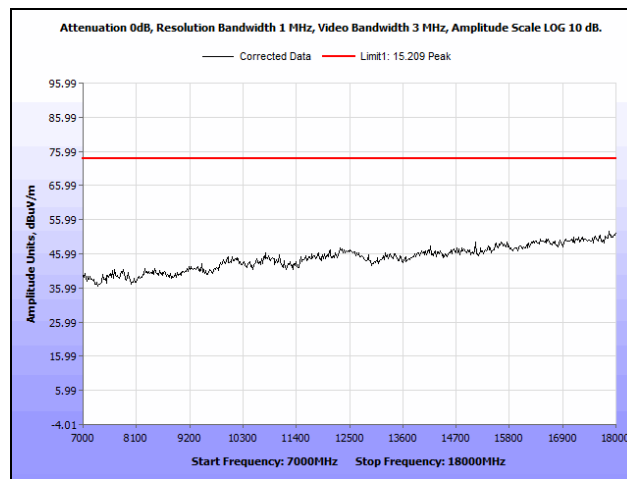
Plot 385. Radiated Spurious Emissions, 30 MHz, Low Channel, 7 GHz – 18 GHz, Peak, Upper Band, 23 dBi Antenna
