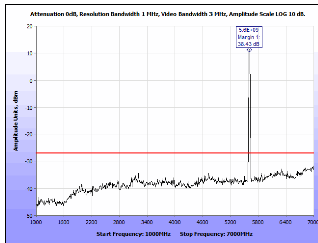
Plot 253. Radiated Spurious Emissions, 30 MHz, Mid Channel, 1 GHz – 7 GHz, Upper Band
