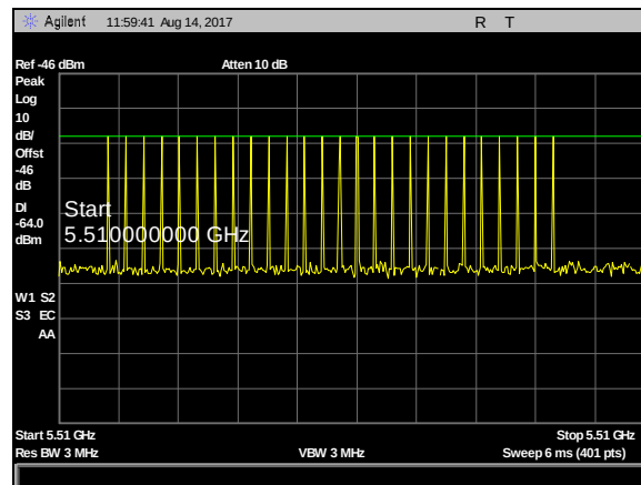
Plot 40. DFS Calibration Plots, Type 2 Calibration 5510 MHz, Sig Gen Level -23 dBm
