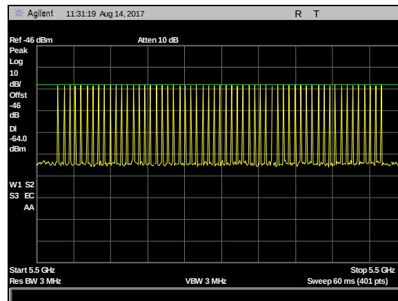
Plot 43. DFS Calibration Plots, Type 1 Calibration 5500 MHz, Sig Gen Level -23 dBm
