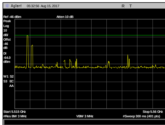
Plot 5. DFS Calibration Plots, Type 6 Calibration 5515 MHz, Sig Gen Level -23 dBm
