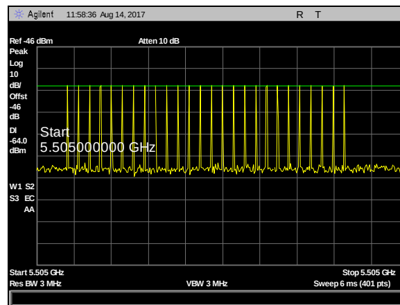
Plot 41. DFS Calibration Plots, Type 2 Calibration 5505 MHz, Sig Gen Level -23 dBm
