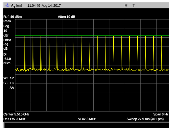
Plot 53. DFS Calibration Plots, Type 0 Calibration 5515 MHz, Sig Gen Level -23 dBm
