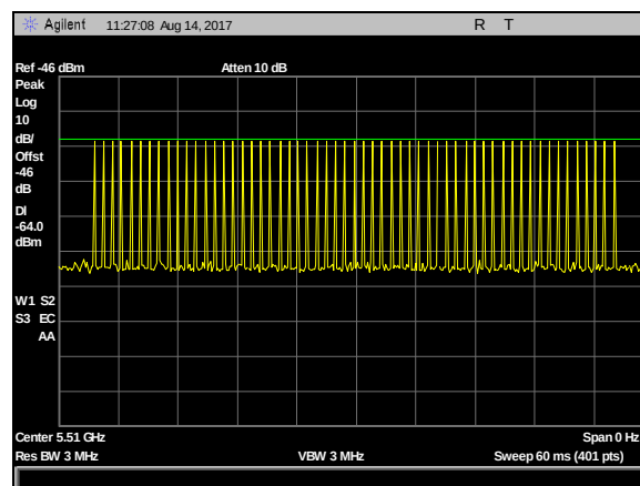
Plot 45. DFS Calibration Plots, Type 1 Calibration 5510 MHz, Sig Gen Level -23 dBm
