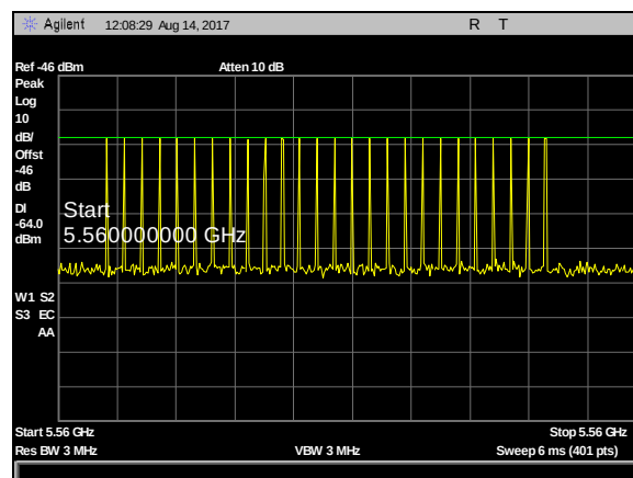
Plot 36. DFS Calibration Plots, Type 2 Calibration 5560 MHz, Sig Gen Level -23 dBm
