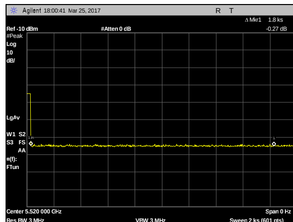
Plot 62. Non-Occupancy Period,
