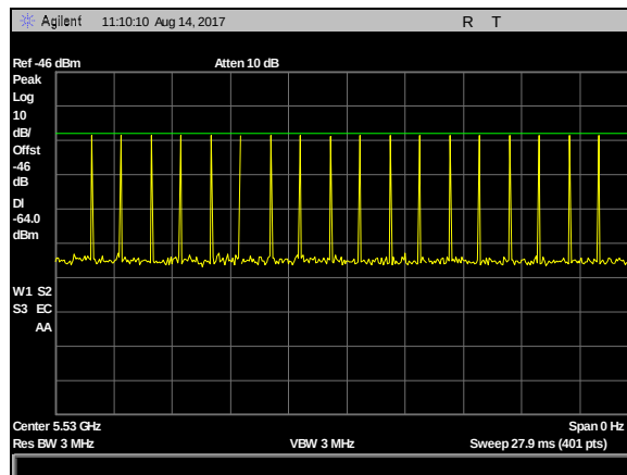
Plot 52. DFS Calibration Plots, Type 0 Calibration 5530 MHz, Sig Gen Level -23 dBm
