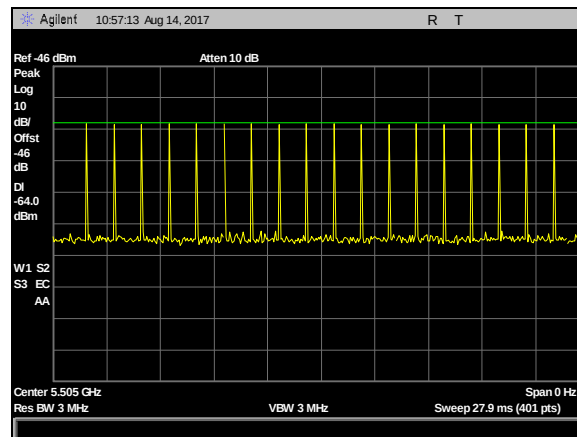
Plot 55. DFS Calibration Plots, Type 0 Calibration 5505 MHz, Sig Gen Level -23 dBm
