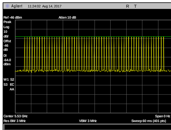
Plot 47. DFS Calibration Plots, Type 1 Calibration 5530 MHz, Sig Gen Level -23 dBm
