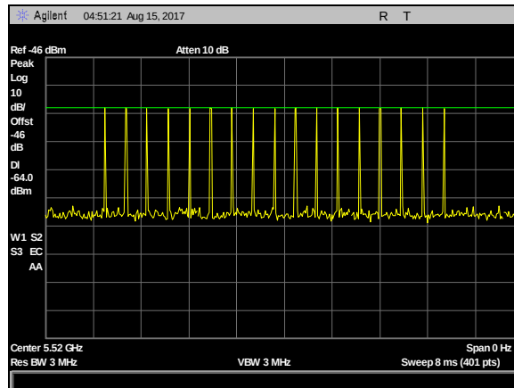
Plot 28. DFS Calibration Plots, Type 3 Calibration 5520 MHz, Sig Gen Level -23 dBm
