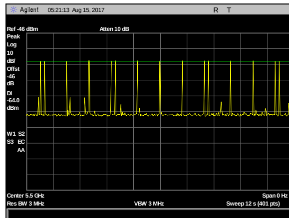
Plot 16. DFS Calibration Plots, Type 5 Calibration 5500 MHz, Sig Gen Level -23 dBm
