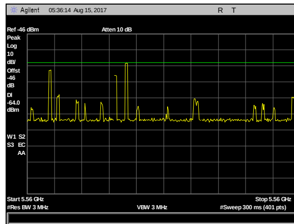
Plot 1. DFS Calibration Plots, Type 6 Calibration 5560 MHz, Sig Gen Level -23 dBm
