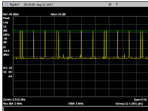
Plot 13. DFS Calibration Plots, Type 5 Calibration 5515 MHz, Sig Gen Level -23 dBm
