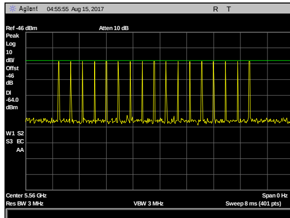
Plot 25. DFS Calibration Plots, Type 3 Calibration 5560 MHz, Sig Gen Level -23 dBm
