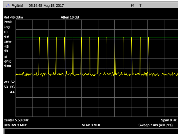
Plot 19. DFS Calibration Plots, Type 4 Calibration 5530 MHz, Sig Gen Level -23 dBm
