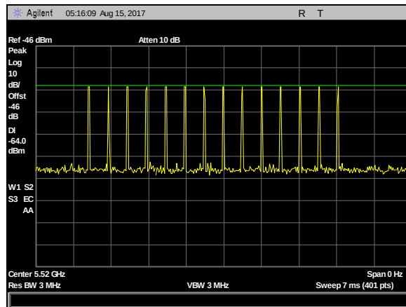
Plot 20. DFS Calibration Plots, Type 4 Calibration 5520 MHz, Sig Gen Level -23 dBm
