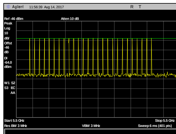
Plot 42. DFS Calibration Plots, Type 2 Calibration 5500 MHz, Sig Gen Level -23 dBm
