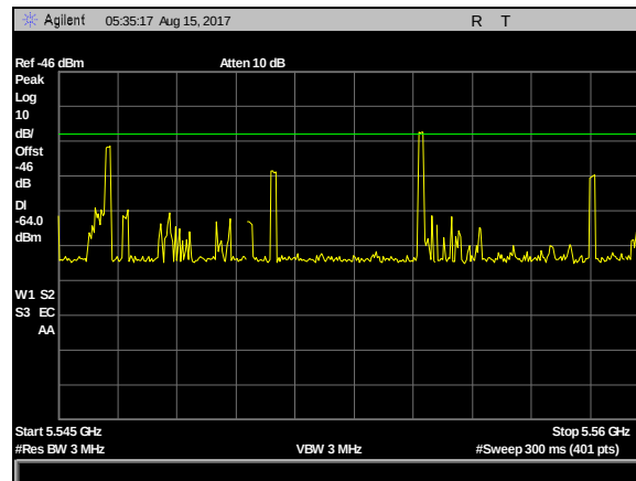
Plot 2. DFS Calibration Plots, Type 6 Calibration 5545 MHz, Sig Gen Level -23 dBm
