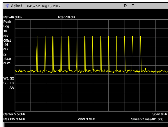
Plot 24. DFS Calibration Plots, Type 4 Calibration 5500 MHz, Sig Gen Level -23 dBm
