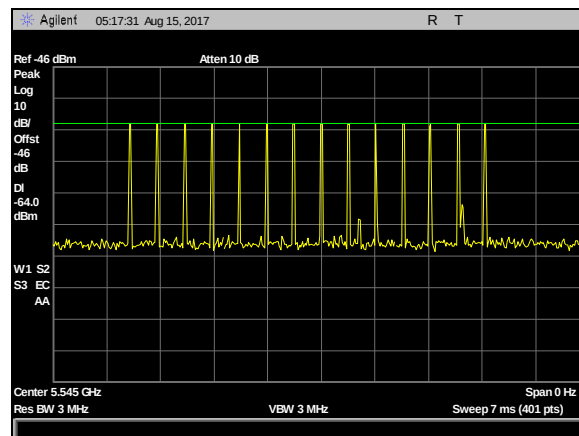
Plot 18. DFS Calibration Plots, Type 4 Calibration 5545 MHz, Sig Gen Level -23 dBm
