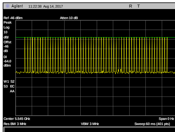
Plot 48. DFS Calibration Plots, Type 1 Calibration 5545 MHz, Sig Gen Level -23 dBm
