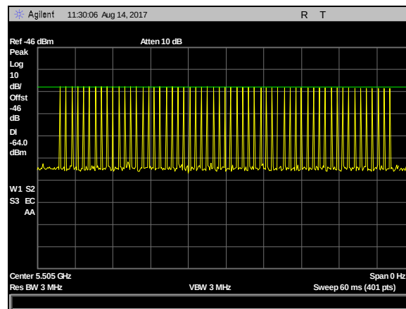
Plot 44. DFS Calibration Plots, Type 1 Calibration 5505 MHz, Sig Gen Level -23 dBm
