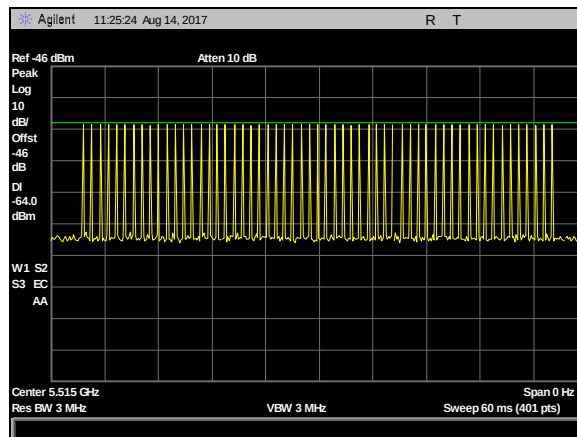
Plot 46. DFS Calibration Plots, Type 1 Calibration 5515 MHz, Sig Gen Level -23 dBm
