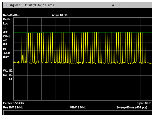
Plot 49. DFS Calibration Plots, Type 1 Calibration 5560 MHz, Sig Gen Level -23 dBm
