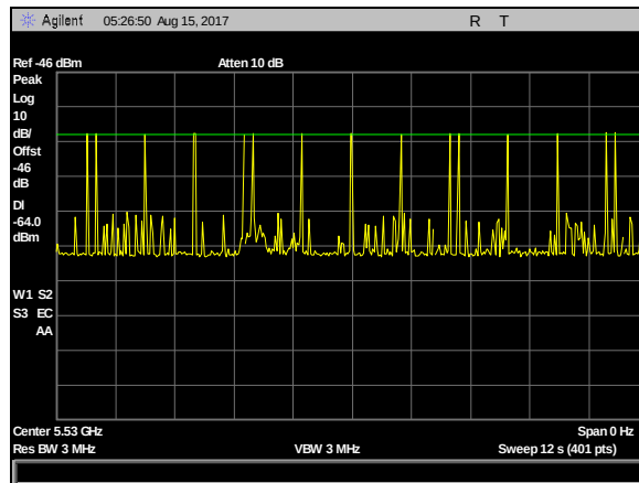
Plot 11. DFS Calibration Plots, Type 5 Calibration 5530 MHz, Sig Gen Level -23 dBm
