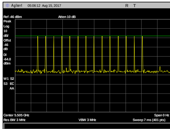
Plot 23. DFS Calibration Plots, Type 4 Calibration 5505 MHz, Sig Gen Level -23 dBm
