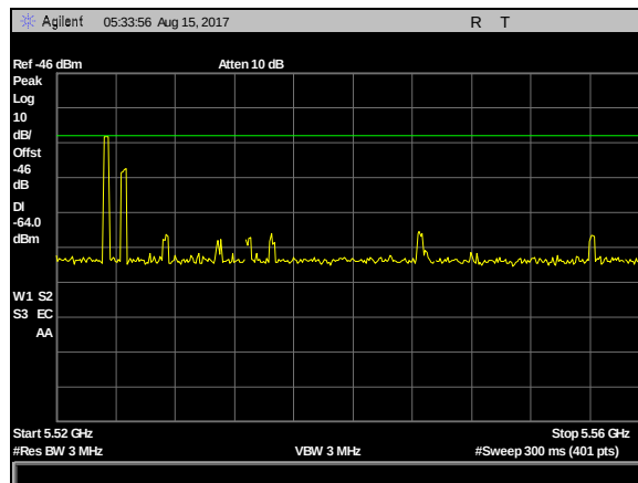
Plot 4. DFS Calibration Plots, Type 6 Calibration 5520 MHz, Sig Gen Level -23 dBm
