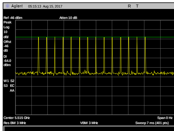
Plot 21. DFS Calibration Plots, Type 4 Calibration 5515 MHz, Sig Gen Level -23 dBm
