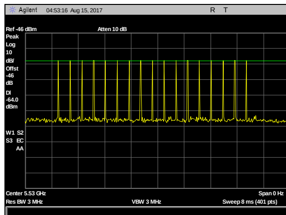
Plot 27. DFS Calibration Plots, Type 3 Calibration 5530 MHz, Sig Gen Level -23 dBm
