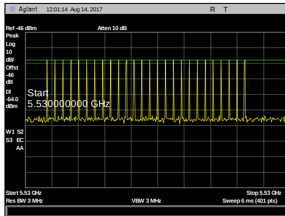
Plot 38. DFS Calibration Plots, Type 2 Calibration 5530 MHz, Sig Gen Level -23 dBm
