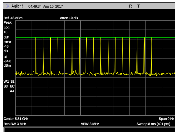
Plot 30. DFS Calibration Plots, Type 3 Calibration 5510 MHz, Sig Gen Level -23 dBm
