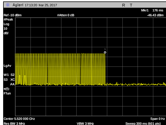
Plot 60. Channel Close Time
