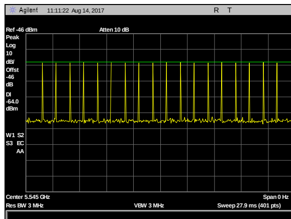
Plot 51. DFS Calibration Plots, Type 0 Calibration 5545 MHz, Sig Gen Level -23 dBm
