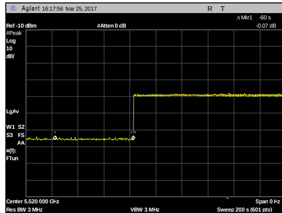
Plot 57. Initial Channel Availability Check Time, 5520 MHz, 100 MHz Bw Channel
