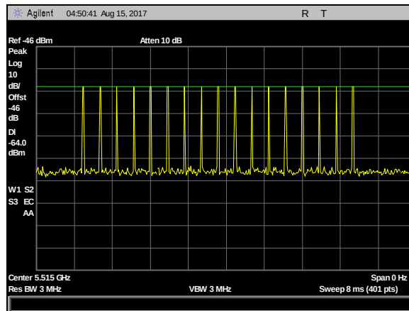
Plot 29. DFS Calibration Plots, Type 3 Calibration 5515 MHz, Sig Gen Level -23 dBm
