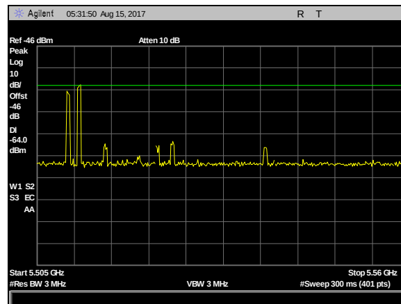
Plot 7. DFS Calibration Plots, Type 6 Calibration 5505 MHz, Sig Gen Level -23 dBm
