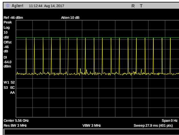
Plot 50. DFS Calibration Plots, Type 0 Calibration 5560 MHz, Sig Gen Level -23 dBm
