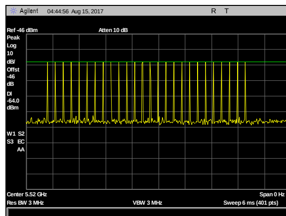
Plot 33. DFS Calibration Plots, Type 2 Calibration 5520 MHz, Sig Gen Level -23 dBm
