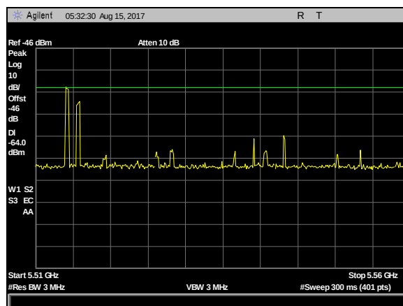
Plot 6. DFS Calibration Plots, Type 6 Calibration 5510 MHz, Sig Gen Level -23 dBm
