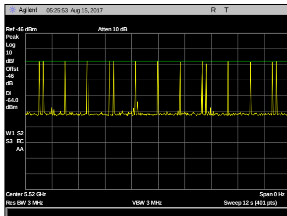
Plot 12. DFS Calibration Plots, Type 5 Calibration 5520 MHz, Sig Gen Level -23 dBm
