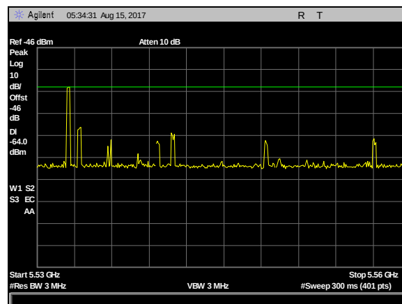
Plot 3. DFS Calibration Plots, Type 6 Calibration 5530 MHz, Sig Gen Level -23 dBm
