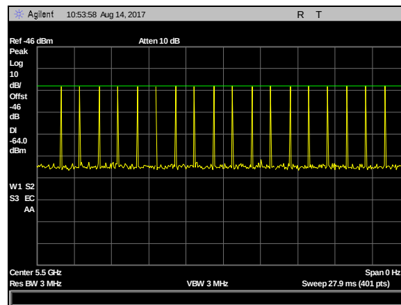
Plot 56. DFS Calibration Plots, Type 0 Calibration 5500 MHz, Sig Gen Level -23 dBm
