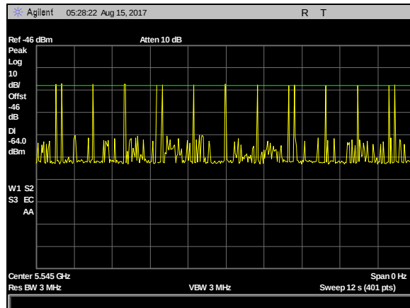
Plot 10. DFS Calibration Plots, Type 5 Calibration 5545 MHz, Sig Gen Level -23 dBm
