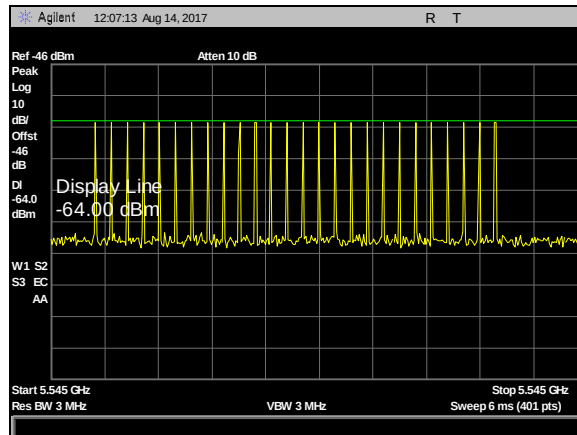
Plot 37. DFS Calibration Plots, Type 2 Calibration 5545 MHz, Sig Gen Level -21 dBm
