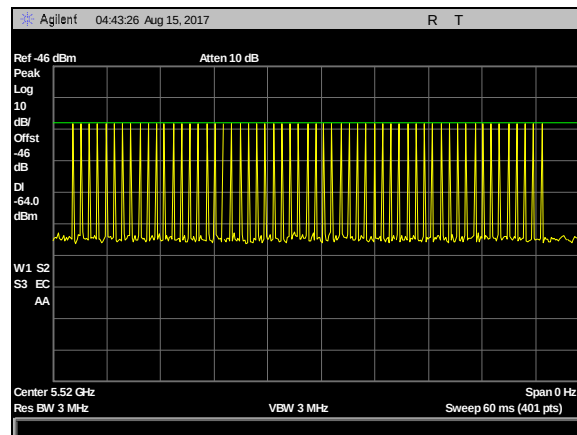
Plot 34. DFS Calibration Plots, Type 1 Calibration 5520 MHz, Sig Gen Level -23 dBm
