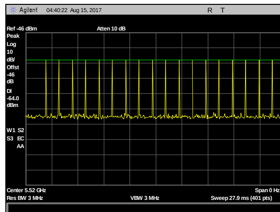
Plot 35. DFS Calibration Plots, Type 0 Calibration 5520 MHz, Sig Gen Level -23 dBm
