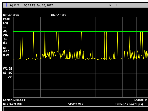
Plot 15. DFS Calibration Plots, Type 5 Calibration 5505 MHz, Sig Gen Level -23 dBm
