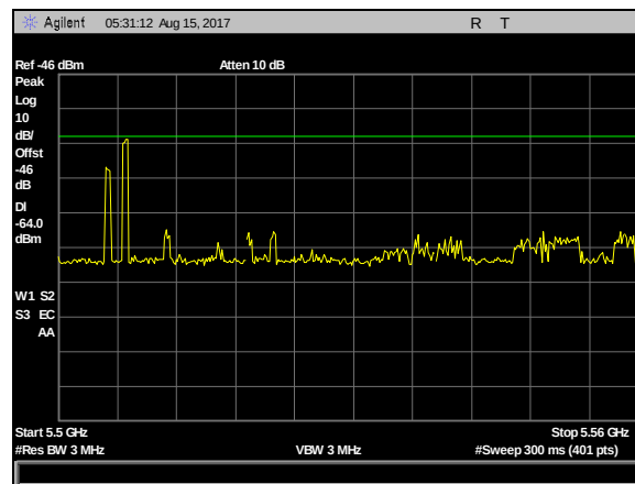
Plot 8. DFS Calibration Plots, Type 6 Calibration 5500 MHz, Sig Gen Level -23 dBm
