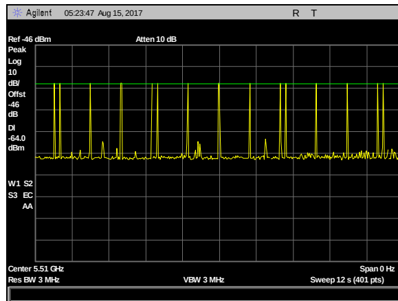
Plot 14. DFS Calibration Plots, Type 5 Calibration 5510 MHz, Sig Gen Level -23 dBm
