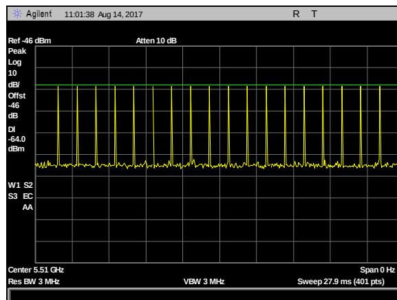
Plot 54. DFS Calibration Plots, Type 0 Calibration 5510 MHz, Sig Gen Level -23 dBm
