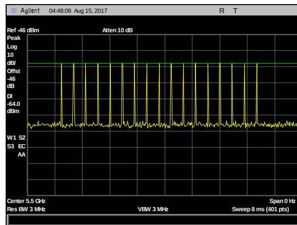
Plot 32. DFS Calibration Plots, Type 3 Calibration 5500 MHz, Sig Gen Level -23 dBm
