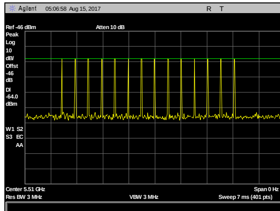
Plot 22. DFS Calibration Plots, Type 4 Calibration 5510 MHz, Sig Gen Level -23 dBm
