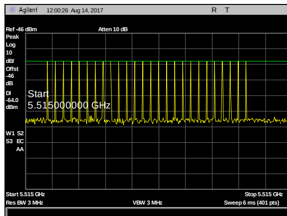
Plot 39. DFS Calibration Plots, Type 2 Calibration 5515 MHz, Sig Gen Level -23 dBm
