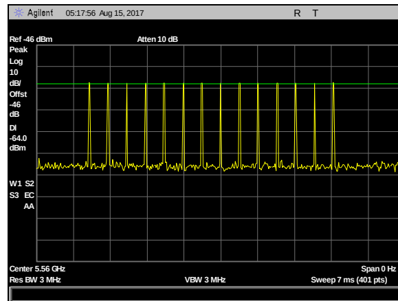
Plot 17. DFS Calibration Plots, Type 4 Calibration 5560 MHz, Sig Gen Level -23 dBm
