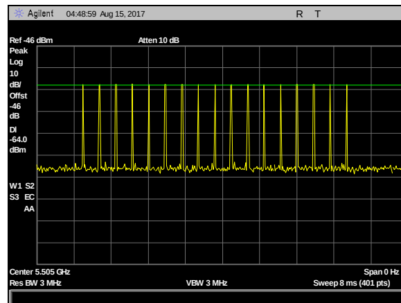
Plot 31. DFS Calibration Plots, Type 3 Calibration 5505 MHz, Sig Gen Level -23 dBm
