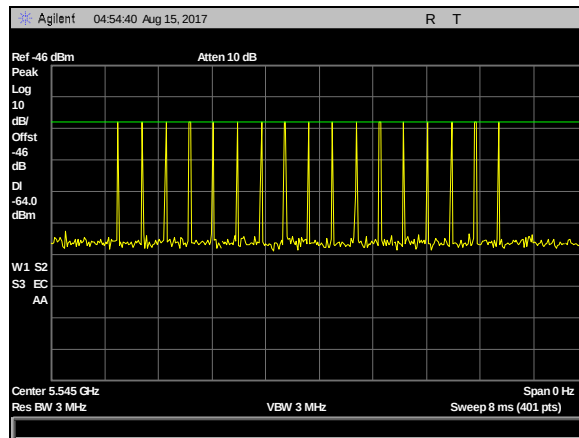
Plot 26. DFS Calibration Plots, Type 3 Calibration 5545 MHz, Sig Gen Level -23 dBm
