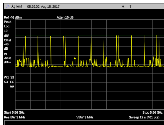
Plot 9. DFS Calibration Plots, Type 5 Calibration 5560 MHz, Sig Gen Level -23 dBm
