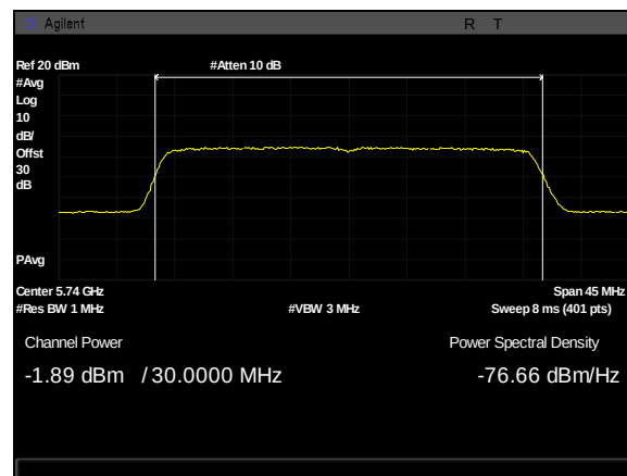
Plot 168. Conducted Transmitter Output Power, Point-to-Multipoint, 34 dBi, chain0, 5740M, 30M
