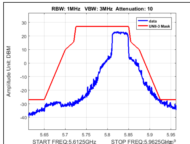
Plot 420. Undesirable Emissions, Fixed Point-to-Point, UNII-3, emission mask, 34dBi, 40M, 5830
