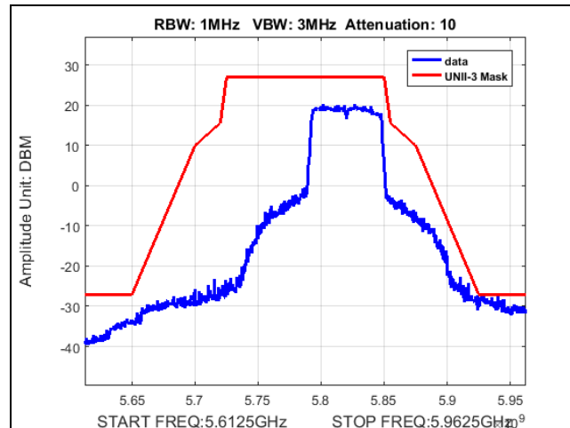
Plot 426. Undesirable Emissions, Fixed Point-to-Point, UNII-3, emission mask, 34dBi, 60M, 5820
