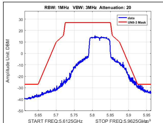
Plot 450. Undesirable Emissions, Fixed Point-to-Point, UNII-3, emission mask, 22dBi, 60M, 5820
