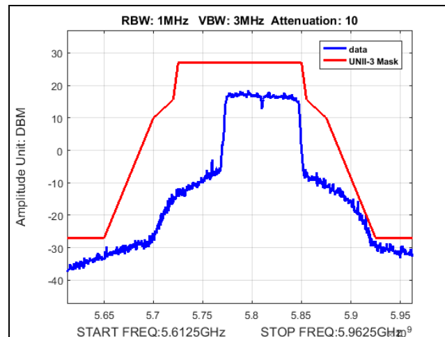
Plot 429. Undesirable Emissions, Fixed Point-to-Point, UNII-3, emission mask, 34dBi, 80M, 5810
