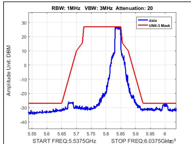
Plot 414. Undesirable Emissions, Fixed Point-to-Point, UNII-3, emission mask, 34dBi, 20M, 5840
