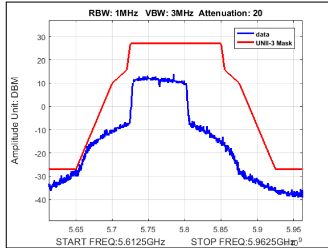
Plot 451. Undesirable Emissions, Fixed Point-to-Point, UNII-3, emission mask, 22dBi, 80M, 5765
