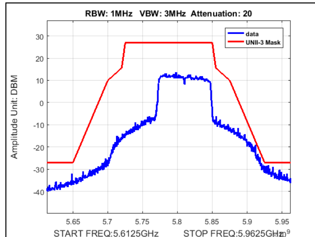
Plot 453. Undesirable Emissions, Fixed Point-to-Point, UNII-3, emission mask, 22dBi, 80M, 5810
