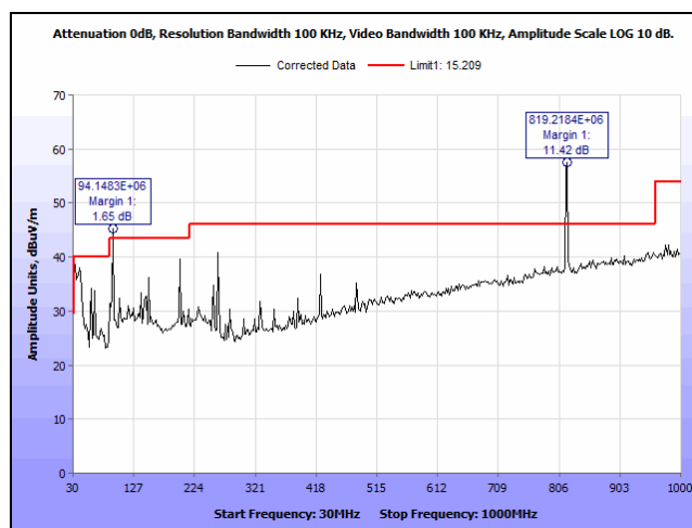
Plot 407. Undesirable Emissions, Radiated Emissions below 1GHz, 22dBi, worst case
