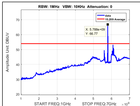
Plot 511. Undesirable Emissions, Fixed Point-to-Point, AVG, 34dBi, radiated spurious emissions, 10M, 5790, 1-7GHz
