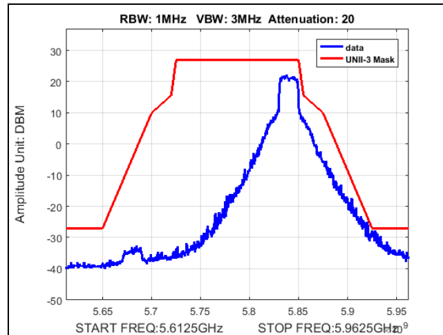
Plot 438. Undesirable Emissions, Fixed Point-to-Point, UNII-3, emission mask, 22dBi, 20M, 5840
