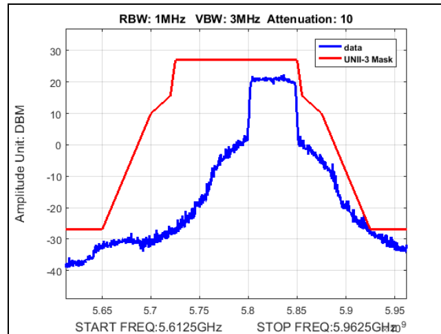
Plot 423. Undesirable Emissions, Fixed Point-to-Point, UNII-3, emission mask, 34dBi, 50M, 5825
