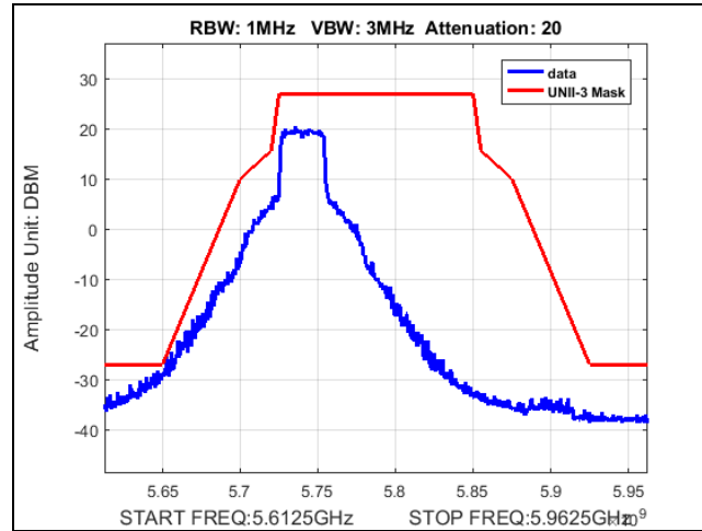
Plot 439. Undesirable Emissions, Fixed Point-to-Point, UNII-3, emission mask, 22dBi, 30M, 5740
