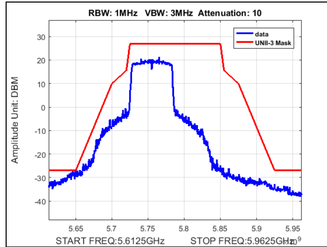
Plot 424. Undesirable Emissions, Fixed Point-to-Point, UNII-3, emission mask, 34dBi, 60M, 5755
