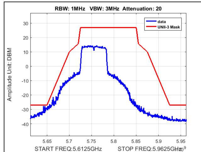
Plot 448. Undesirable Emissions, Fixed Point-to-Point, UNII-3, emission mask, 22dBi, 60M, 5755
