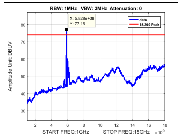
Plot 494. Undesirable Emissions, Fixed Point-to-Point, PK, 22dBi, radiated spurious emissions, 30M, 5835, 1-18GHz
