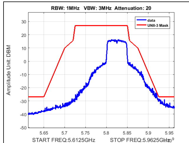
Plot 447. Undesirable Emissions, Fixed Point-to-Point, UNII-3, emission mask, 22dBi, 50M, 5825
