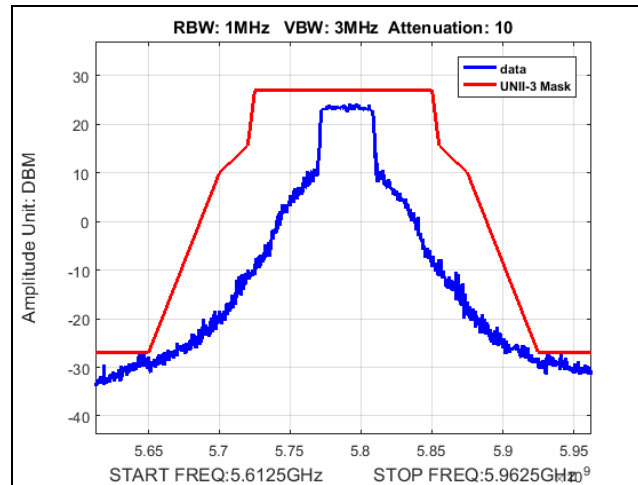
Plot 419. Undesirable Emissions, Fixed Point-to-Point, UNII-3, emission mask, 34dBi, 40M, 5790
