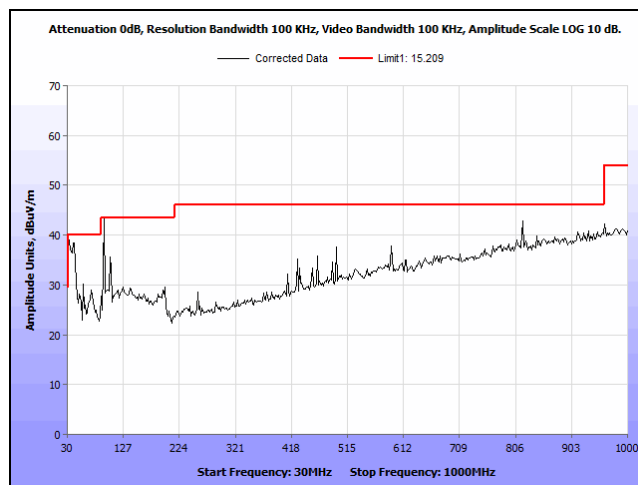
Plot 406. Undesirable Emissions, Radiated Emissions below 1GHz, 13dBi, worst case
