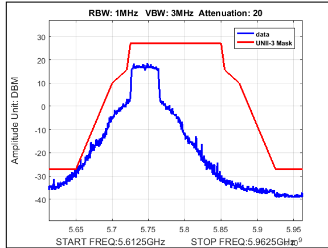
Plot 442. Undesirable Emissions, Fixed Point-to-Point, UNII-3, emission mask, 22dBi, 40M, 5745
