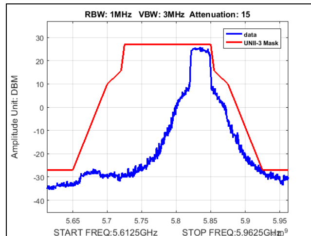
Plot 417. Undesirable Emissions, Fixed Point-to-Point, UNII-3, emission mask, 34dBi, 30M, 5835
