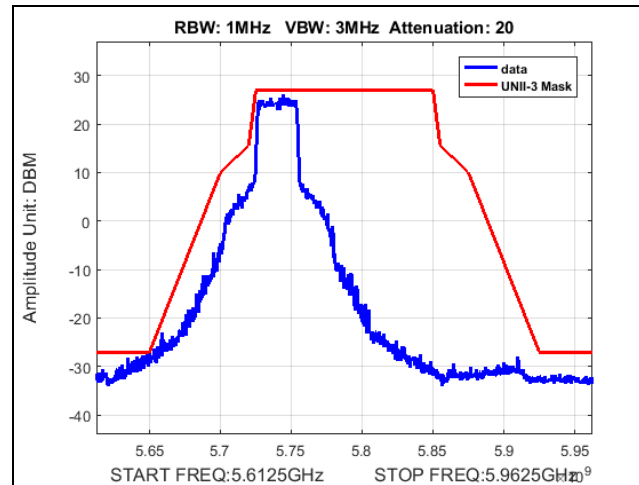
Plot 415. Undesirable Emissions, Fixed Point-to-Point, UNII-3, emission mask, 34dBi, 30M, 5740
