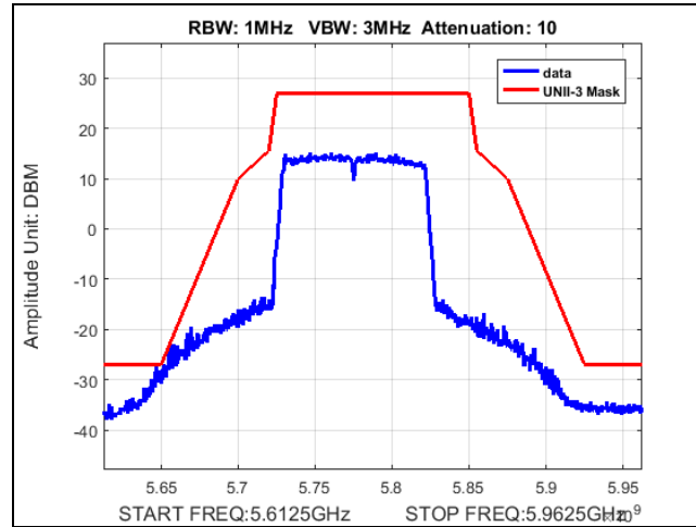
Plot 430. Undesirable Emissions, Fixed Point-to-Point, UNII-3, emission mask, 34dBi, 100M, 5775
