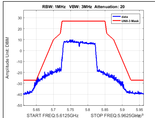
Plot 454. Undesirable Emissions, Fixed Point-to-Point, UNII-3, emission mask, 22dBi, 100M, 5775
