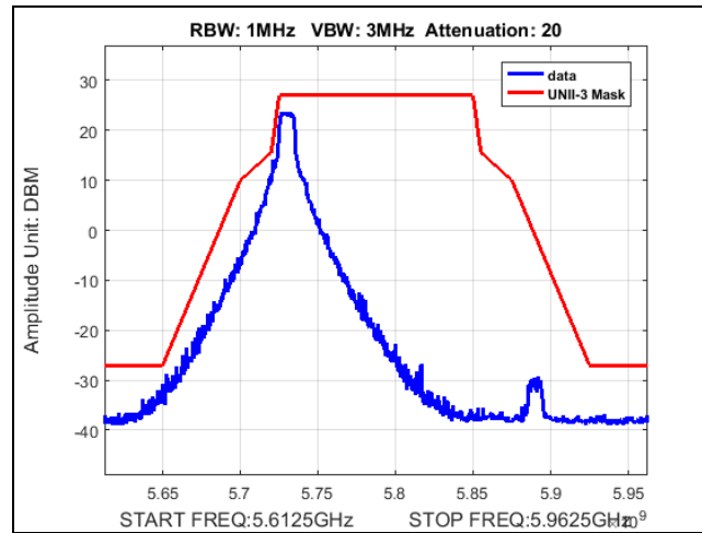
Plot 433. Undesirable Emissions, Fixed Point-to-Point, UNII-3, emission mask, 22dBi, 10M, 5730
