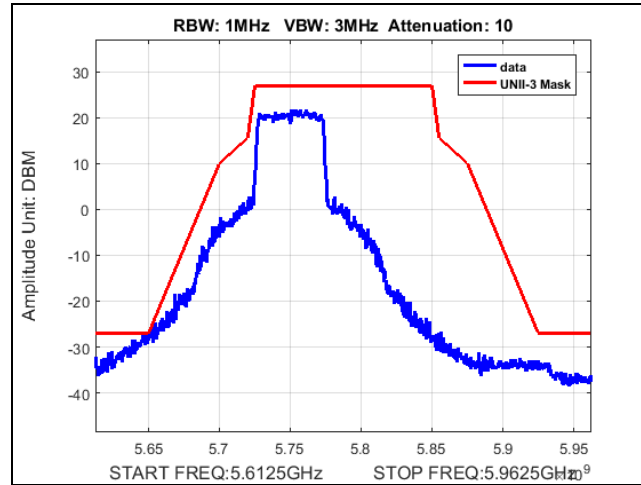
Plot 421. Undesirable Emissions, Fixed Point-to-Point, UNII-3, emission mask, 34dBi, 50M, 5750
