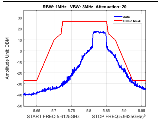
Plot 444. Undesirable Emissions, Fixed Point-to-Point, UNII-3, emission mask, 22dBi, 40M, 5830
