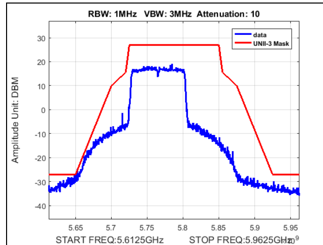
Plot 427. Undesirable Emissions, Fixed Point-to-Point, UNII-3, emission mask, 34dBi, 80M, 5765
