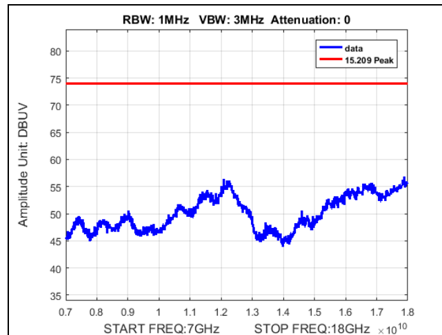
Plot 668. Undesirable Emissions, Point-to-Multipoint, PK, 13dBi, radiated spurious emissions, worst case, 7-18GHz
