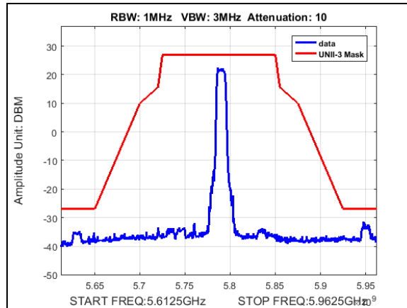
Plot 569. Undesirable Emissions, Point-to-Multipoint, UNII-3, emission mask, 34dBi, 10M, 5790
