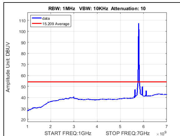
Plot 641. Undesirable Emissions, Point-to-Multipoint, AVG, 13dBi, radiated spurious emissions, 10M, 5790M, 1-7GHz
