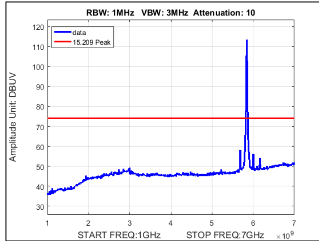
Plot 667. Undesirable Emissions, Point-to-Multipoint, PK, 13dBi, radiated spurious emissions, 10M, 5845M, 1-7GHz
