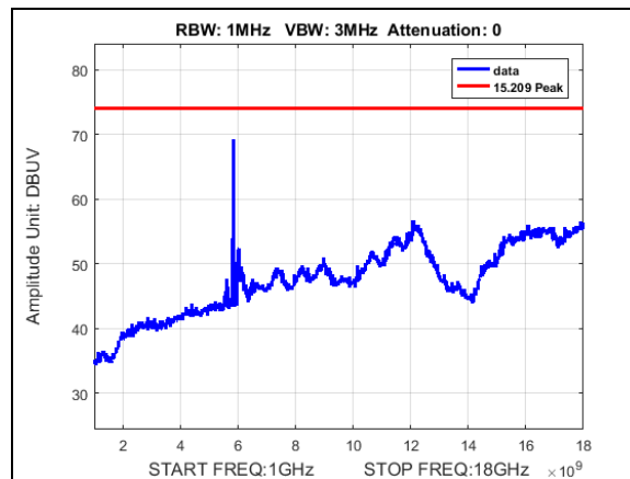
Plot 722. Undesirable Emissions, Point-to-Multipoint, PK, 22dBi, radiated spurious emissions, 30M, 5835M, 1-18GHz
