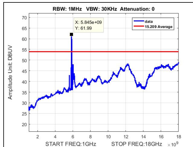
Plot 695. Undesirable Emissions, Point-to-Multipoint, AVG, 22dBi, radiated spurious emissions, 20M, 5840M, 1-18GHz
