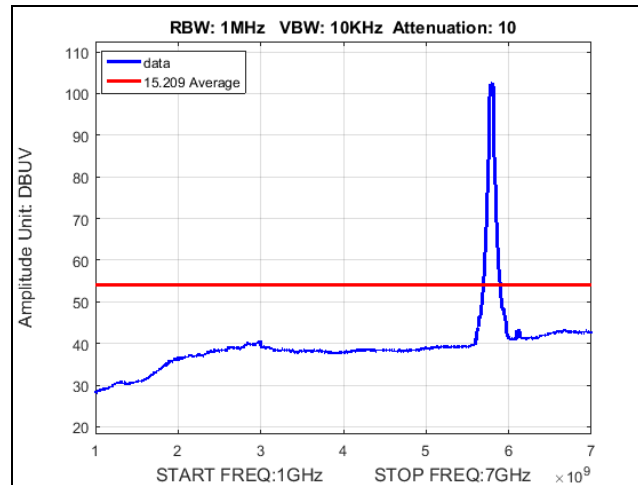
Plot 651. Undesirable Emissions, Point-to-Multipoint, AVG, 13dBi, radiated spurious emissions, 40M, 5790M, 1-7GHz
