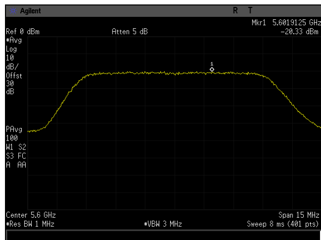
Plot 553. Power Spectral Density, UNII 2C, BW 10M, Ch 5600M, 2x2 34dB c0
