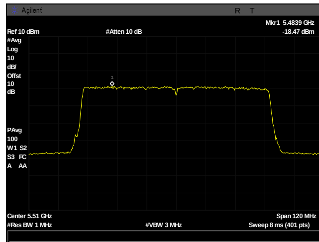
Plot 492. Power Spectral Density, UNII 2C, BW 80M, Ch 5510M, 2x2 13dBi c1
