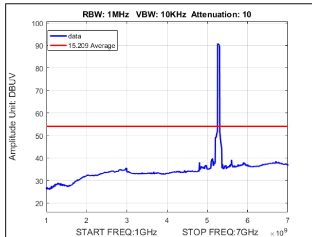
Plot 705. Undesirable Emissions, UNII 2A, AVG, radiated spurious, 22dBi sector, 50M, 5275M, 1-7GHz
