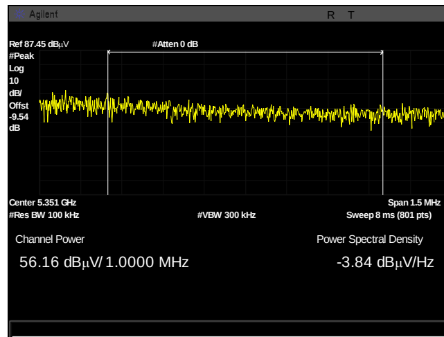
Plot 611. Undesirable Emissions, UNII 2A, PK, bandedge 5350, 13dBi, 50M, 5325M, pwr integration
