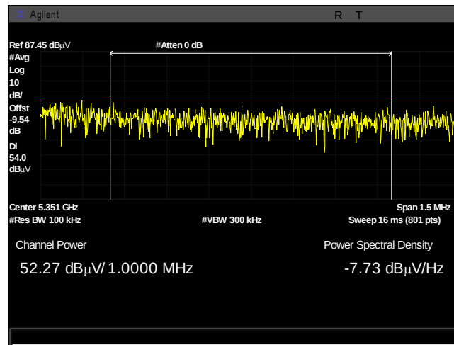
Plot 602. Undesirable Emissions, UNII 2A, AVG, bandedge 5350, 13dBi, 40M, 5330M, pwr integration
