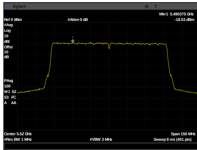
Plot 498. Power Spectral Density, UNII 2C, BW 100M, Ch 5520M, 2x2 13dBi c1
