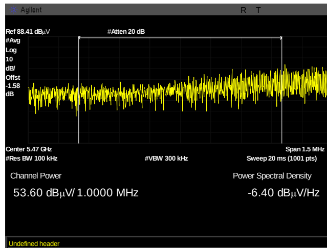
Plot 996. Undesirable Emissions, UNII 2C, AVG, bandedge 5470, 34dBi, 30M, 5485M, pwr integration
