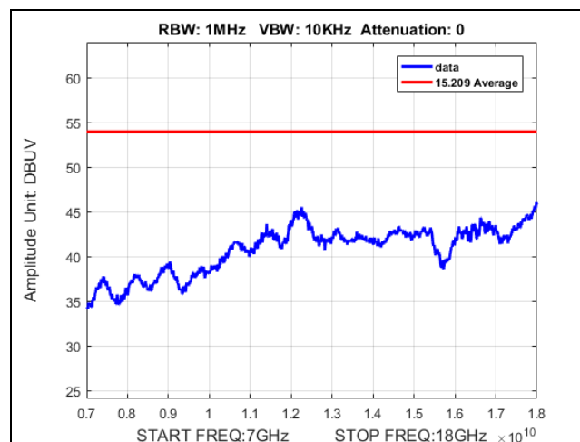
Plot 715. Undesirable Emissions, UNII 2A, AVG, radiated spurious, 22dBi sector, worst case, 7-18GHz
