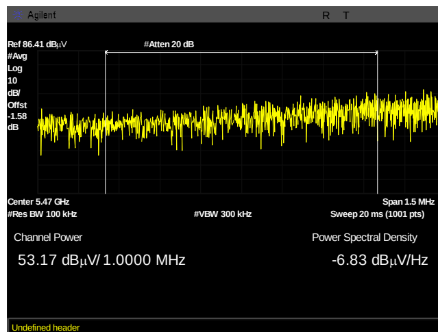
Plot 997. Undesirable Emissions, UNII 2C, AVG, bandedge 5470, 34dBi, 40M, 5490M, pwr integration
