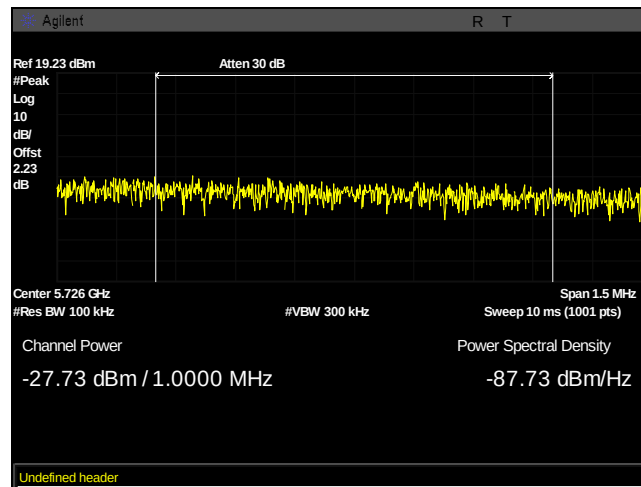
Plot 952. Undesirable Emissions, UNII 2C, -27dBm, bandedge 5725, 22dBiM, 80M, 5685M, pwr integration
