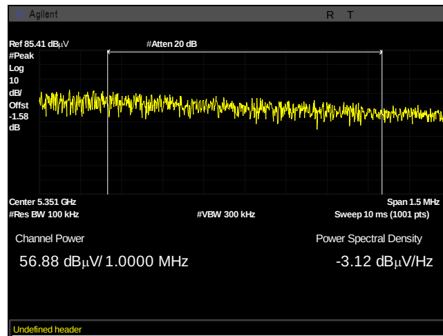
Plot 644. Undesirable Emissions, UNII 2A, PK, bandedge 5350, 34dBi, 60M, 5320M, pwr integration
