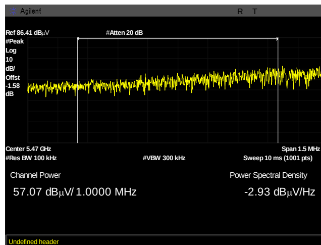
Plot 1006. Undesirable Emissions, UNII 2C, PK, bandedge 5470, 34dBi, 50M, 5495M, pwr integration
