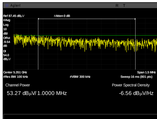
Plot 604. Undesirable Emissions, UNII 2A, AVG, bandedge 5350, 13dBi, 60M, 5320M, pwr integration
