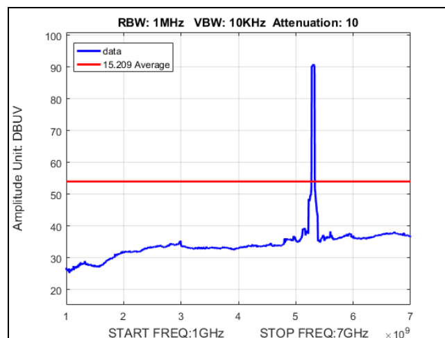
Plot 706. Undesirable Emissions, UNII 2A, AVG, radiated spurious, 22dBi sector, 50M, 5300M, 1-7GHz
