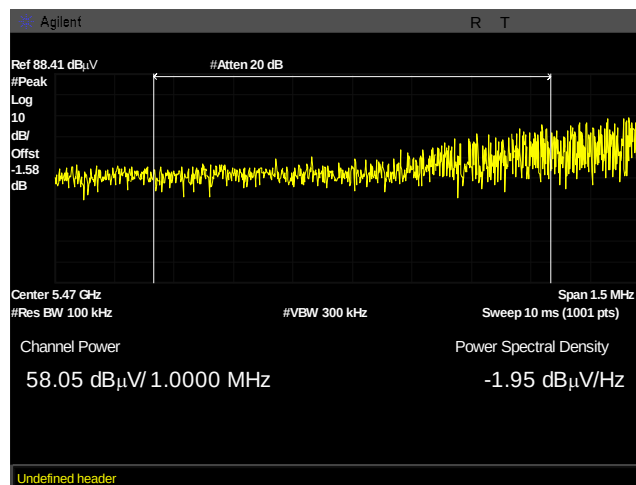
Plot 1003. Undesirable Emissions, UNII 2C, PK, bandedge 5470, 34dBi, 20M, 5480M, pwr integration
