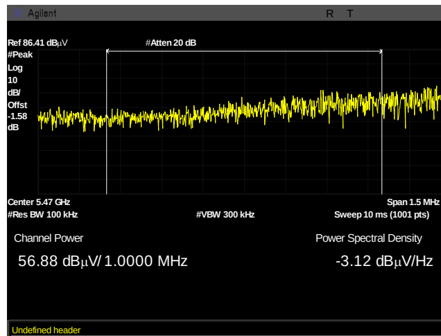
Plot 1005. Undesirable Emissions, UNII 2C, PK, bandedge 5470, 34dBi, 40M, 5490M, pwr integration
