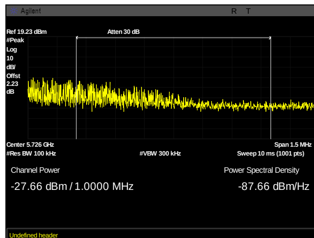
Plot 947. Undesirable Emissions, UNII 2C, -27dBm, bandedge 5725, 22dBiM, 20M, 5715M, pwr integration
