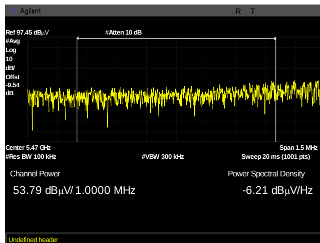
Plot 982. Undesirable Emissions, UNII 2C, AVG, bandedge 5470, 22dBi, sector, 50M, 5495, pwr integration
