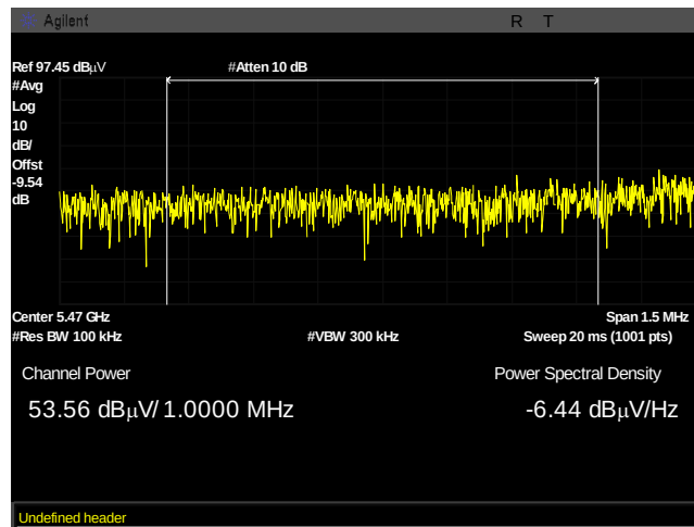
Plot 981. Undesirable Emissions, UNII 2C, AVG, bandedge 5470, 22dBi, sector, 40M, 5490, pwr integration
