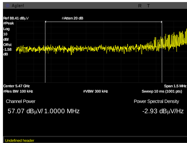
Plot 1002. Undesirable Emissions, UNII 2C, PK, bandedge 5470, 34dBi, 10M, 5475M, pwr integration
