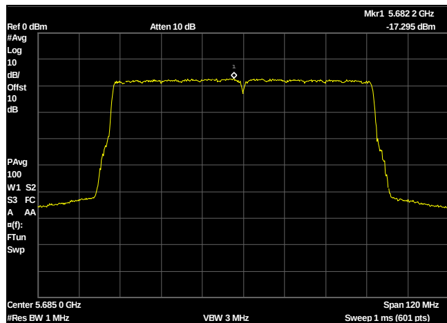
Plot 543. Power Spectral Density, UNII 2C, BW 80M, Ch 5685M, 2x2 22dBi c0
