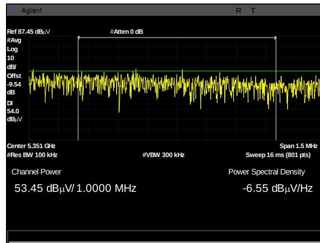
Plot 599. Undesirable Emissions, UNII 2A, AVG, bandedge 5350, 13dBi, 10M, 5345M, pwr integration
