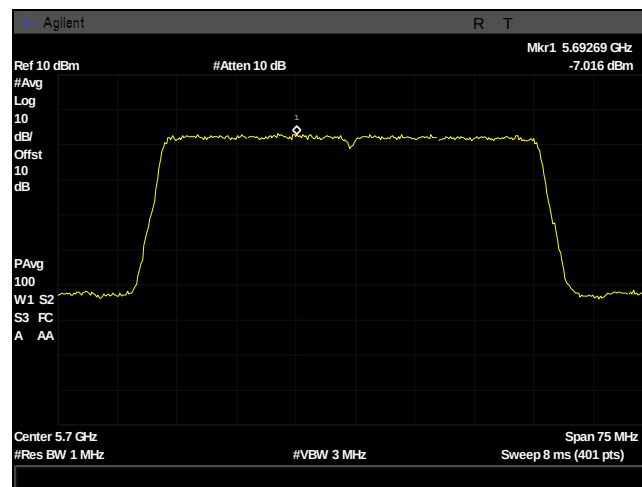
Plot 483. Power Spectral Density, UNII 2C, BW 50M, Ch 5700M, 2x2 13dBi c0
