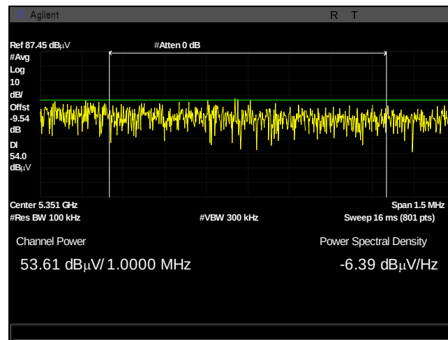
Plot 600. Undesirable Emissions, UNII 2A, AVG, bandedge 5350, 13dBi, 20M, 5340M, pwr integration
