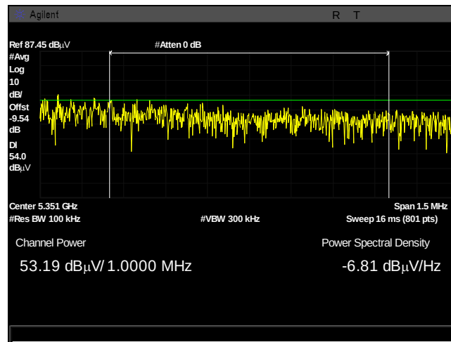
Plot 603. Undesirable Emissions, UNII 2A, AVG, bandedge 5350, 13dBi, 50M, 5325M, pwr integration
