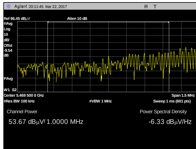
Plot 964. Undesirable Emissions, UNII 2C, AVG, bandedge 5470, 13dBi, 30M, 5485M, pwr integration
