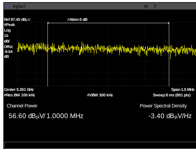
Plot 608. Undesirable Emissions, UNII 2A, PK, bandedge 5350, 13dBi, 20M, 5340M, pwr integration
