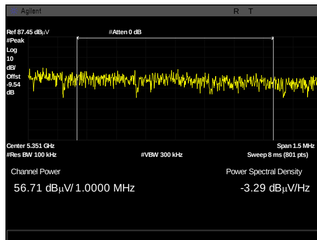
Plot 607. Undesirable Emissions, UNII 2A, PK, bandedge 5350, 13dBi, 10M, 5345M, pwr integration
