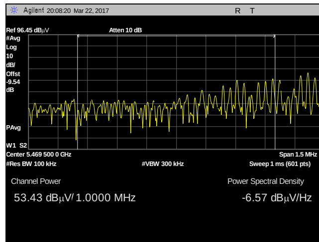
Plot 963. Undesirable Emissions, UNII 2C, AVG, bandedge 5470, 13dBi, 20M, 5480M, pwr integration
