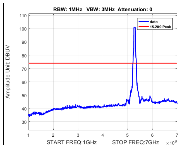
Plot 685. Undesirable Emissions, UNII 2A, PK, radiated spurious, 13dBi, 60M, 5280M
