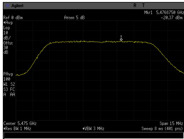
Plot 552. Power Spectral Density, UNII 2C, BW 10M, Ch 5475M, 2x2 34dB c1
