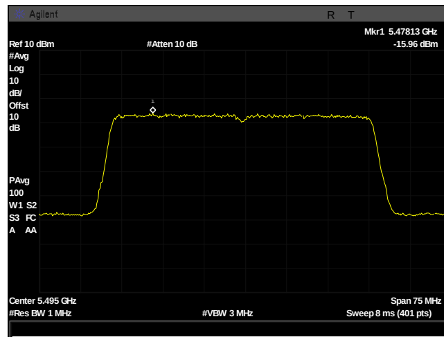
Plot 479. Power Spectral Density, UNII 2C, BW 50M, Ch 5495M, 2x2 13dBi c0
