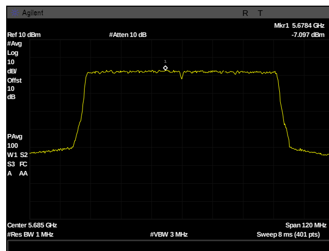
Plot 496. Power Spectral Density, UNII 2C, BW 80M, Ch 5685M, 2x2 13dBi c1
