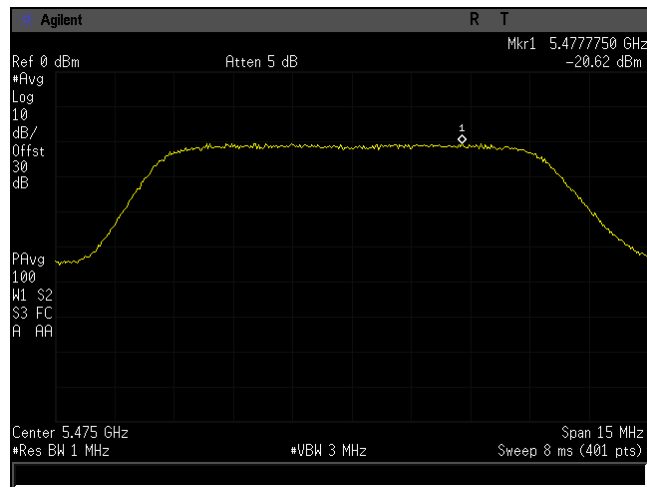
Plot 551. Power Spectral Density, UNII 2C, BW 10M, Ch 5475M, 2x2 34dB c0
