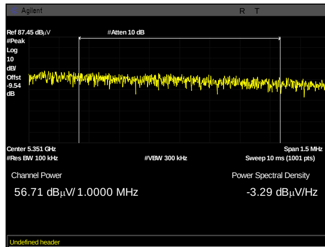
Plot 630. Undesirable Emissions, UNII 2A, PK, bandedge 5350, 22dB, sector, 100M, 5300M, pwr integration
