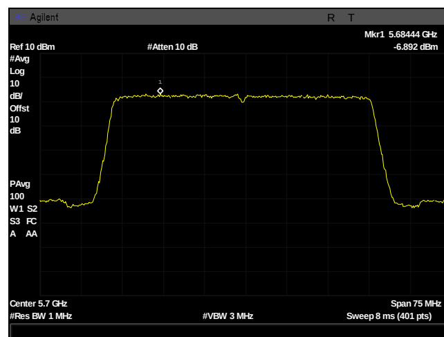
Plot 484. Power Spectral Density, UNII 2C, BW 50M, Ch 5700M, 2x2 13dBi c1
