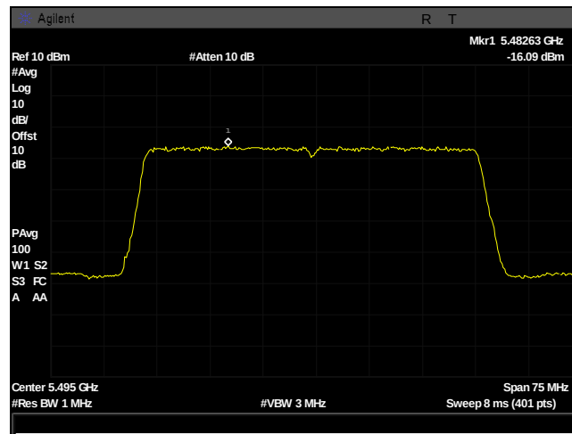
Plot 480. Power Spectral Density, UNII 2C, BW 50M, Ch 5495M, 2x2 13dBi c1
