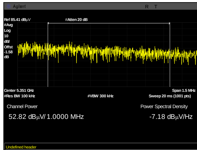
Plot 636. Undesirable Emissions, UNII 2A, AVG, bandedge 5350, 34dBi, 60M, 5320M, pwr integration
