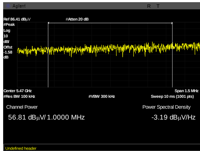
Plot 1008. Undesirable Emissions, UNII 2C, PK, bandedge 5470, 34dBi, 80M, 5510M, pwr integration
