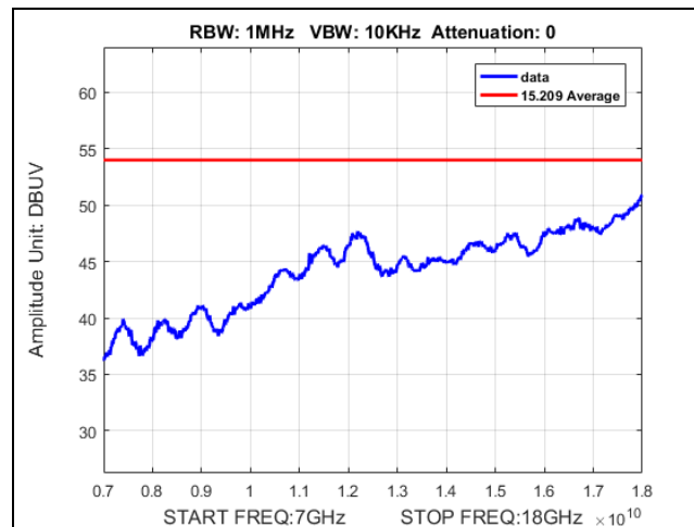
Plot 841. Undesirable Emissions, UNII 2C, AVG, radiated spurious, 22dBi sector, worst case, 7-18GHz
