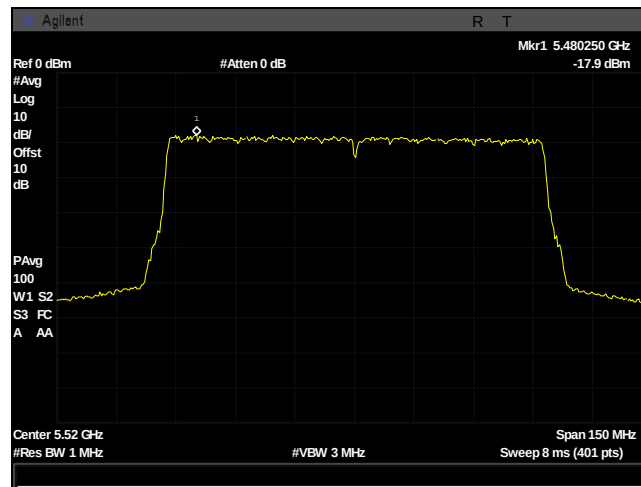
Plot 497. Power Spectral Density, UNII 2C, BW 100M, Ch 5520M, 2x2 13dBi c0
