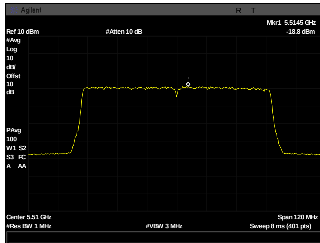
Plot 491. Power Spectral Density, UNII 2C, BW 80M, Ch 5510M, 2x2 13dBi c0
