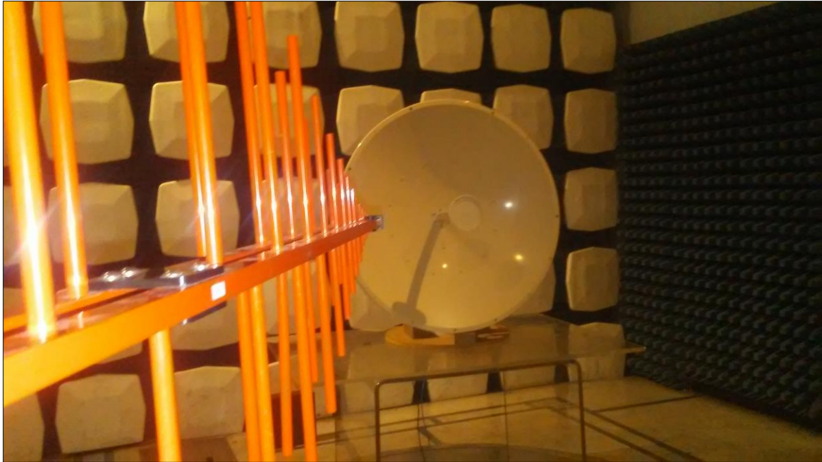
Photograph 1. Test Setup, Radiated Emissions Below 1GHz, 34dBi antenna
