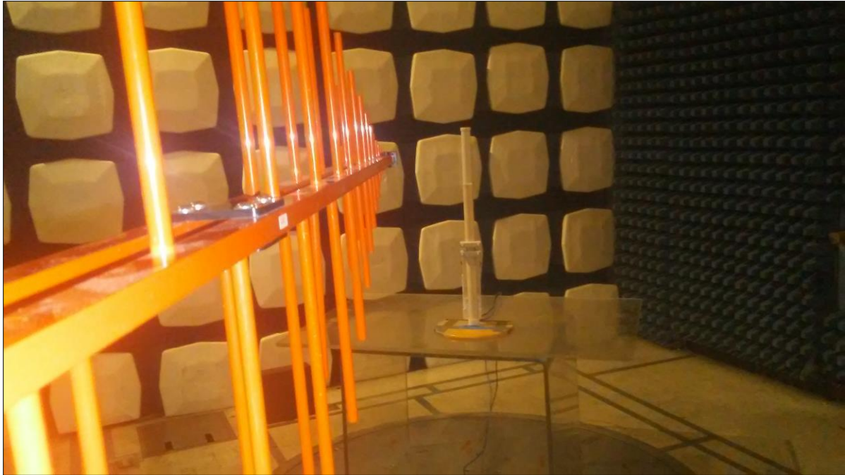
Photograph 5. Test Setup, Radiated Emissions Below 1GHz, 13dBi antenna
