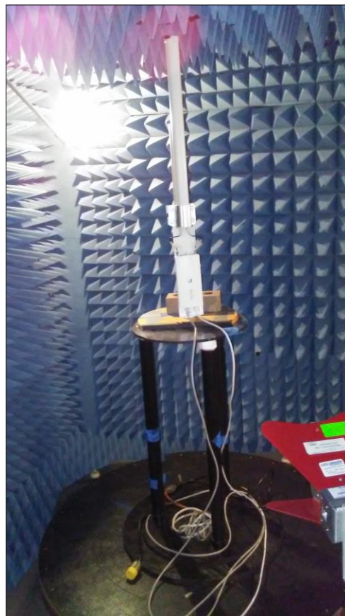
Photograph 6. Test Setup, Radiated Emissions Above 1GHz, 13dBi antenna
