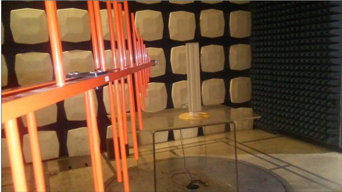
Photograph 3. Test Setup, Radiated Emissions Below 1GHz, 22dBi antenna
