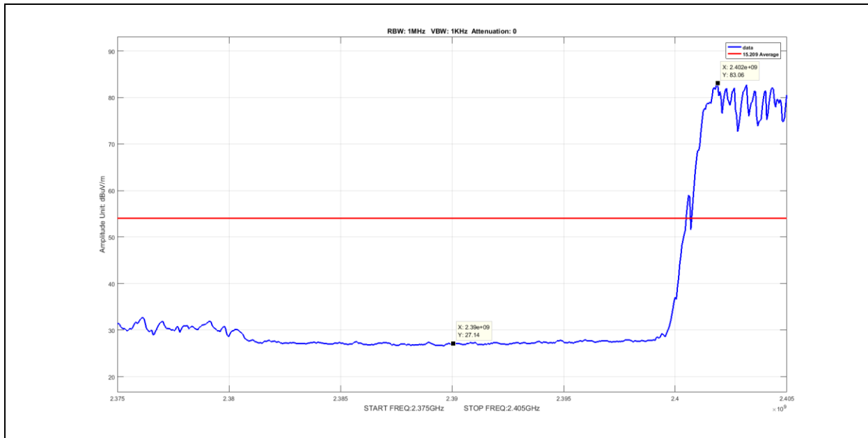
Plot 79. Radiated Restricted Band Edge, Average, Hopping, 2390MHz, DH1
