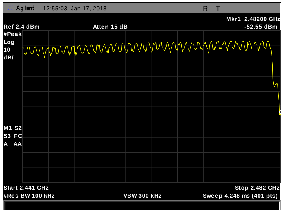
Plot 28. Number of Channels, 3-DH1.2
