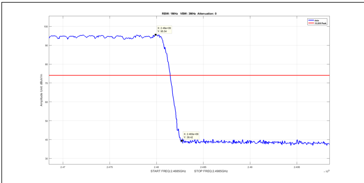
Plot 92. Radiated Restricted Band Edge, Peak, Hopping, 2483.5MHz, DH5
