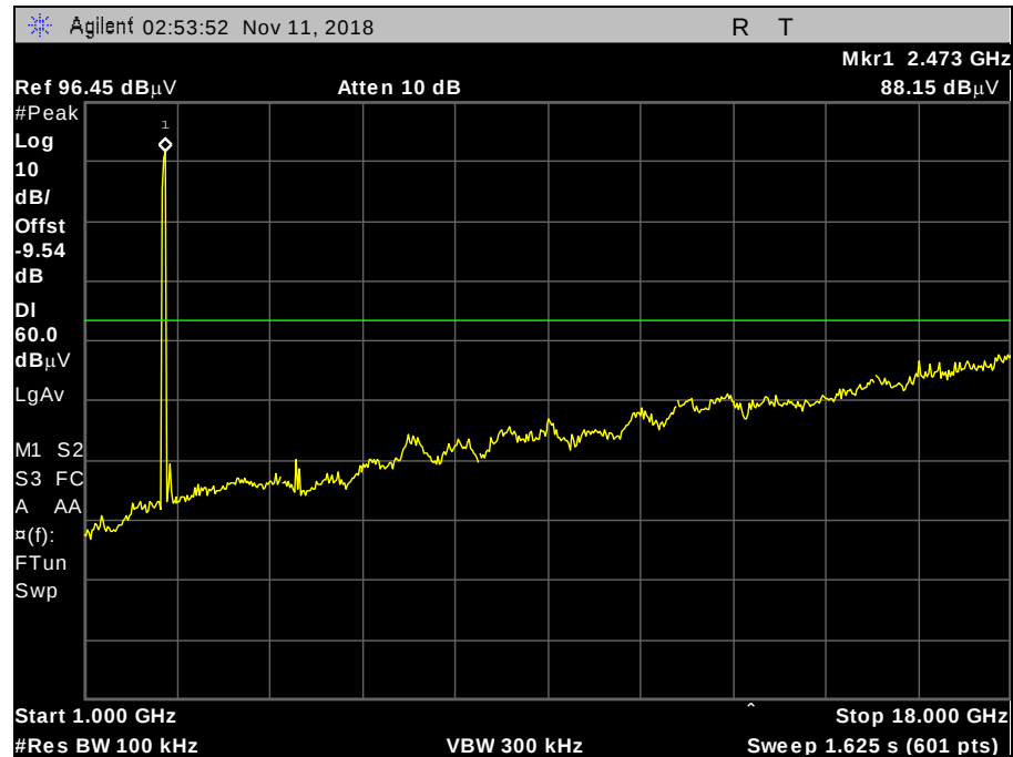
Plot 105. Conducted Spurious Emissions, Hopping, 3-DH1, 1 GHz – 18 GHz
