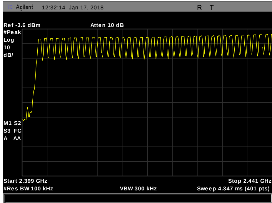
Plot 23. Number of Channels, DH1.1
