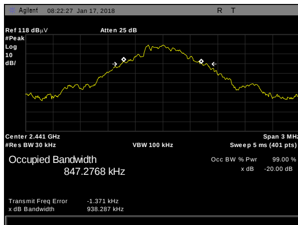
Plot 4. 20 dB Occupied Bandwidth, DH1, 2441 MHz
