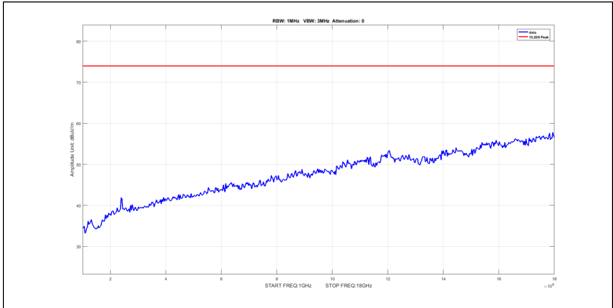
Plot 68. Radiated Spurious Emissions, Peak, Nonhopping, 1G – 18G, 3-DH5, 2402MHz
