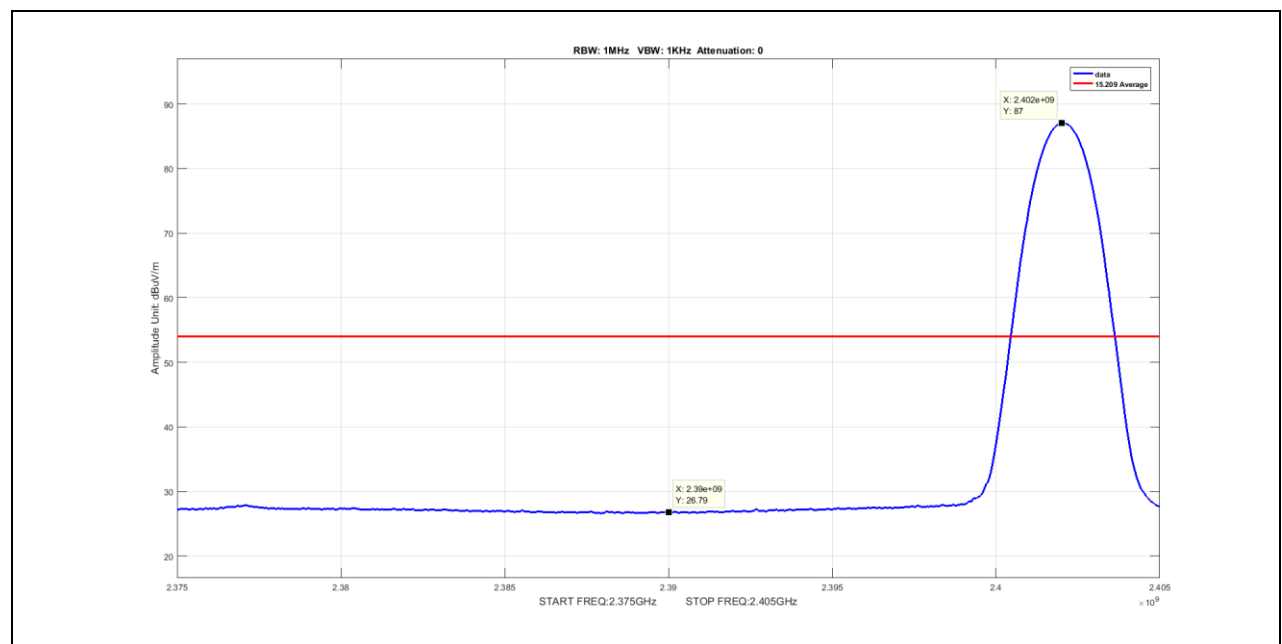
Plot 72. Radiated Restricted Band Edge, Average, 2390MHz, DH5
