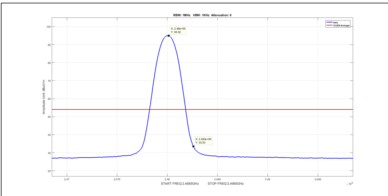
Plot 76. Radiated Restricted Band Edge, Average, 2483.5MHz, DH5
