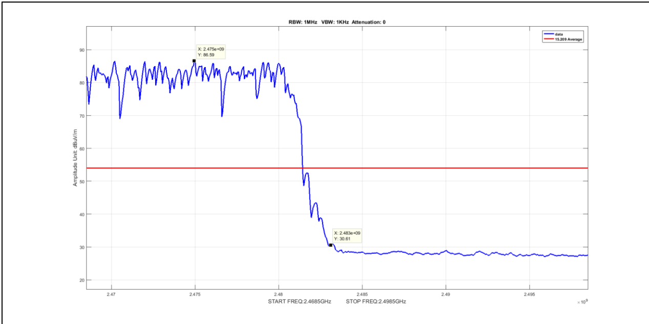
Plot 85. Radiated Restricted Band Edge, Average, Hopping, 2483.5MHz, 3-DH1
