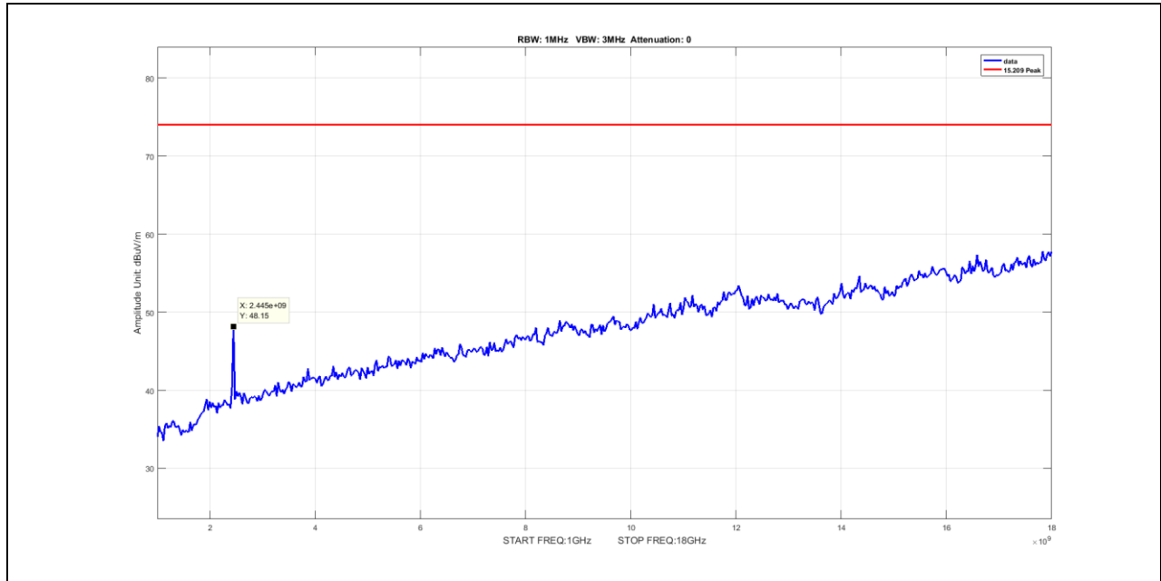
Plot 60. Radiated Spurious Emissions, Peak, Nonhopping, 1G – 18G, DH1, 2441MHz
