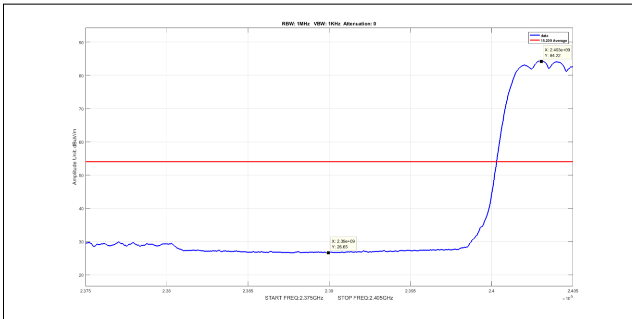
Plot 82. Radiated Restricted Band Edge, Average, Hopping, 2390MHz, 3-DH5
