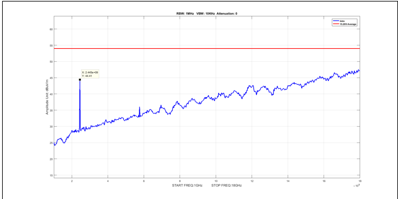
Plot 54. Radiated Spurious Emissions, Average, Nonhopping, 1G – 18G, 3-DH1, 2441MHz
