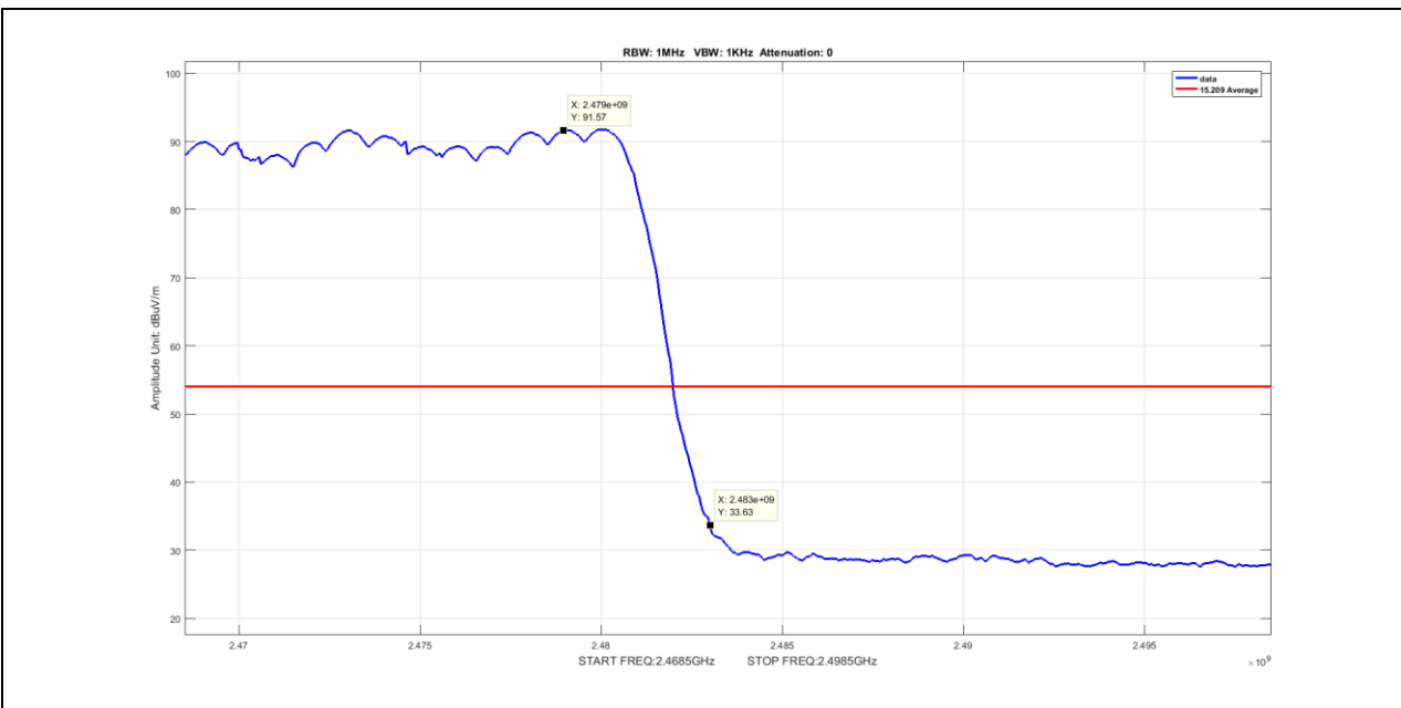
Plot 86. Radiated Restricted Band Edge, Average, Hopping, 2483.5MHz, 3-DH5
