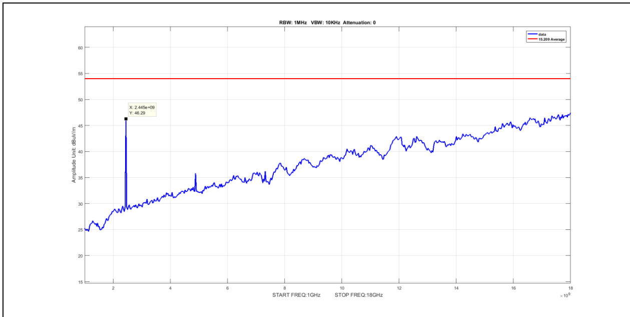
Plot 48. Radiated Spurious Emissions, Average, Nonhopping, 1G – 18G, DH1, 2441MHz
