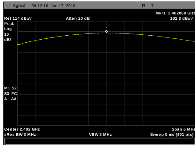
Plot 44. Peak Power Output, 3-DH5, 2402MHz
