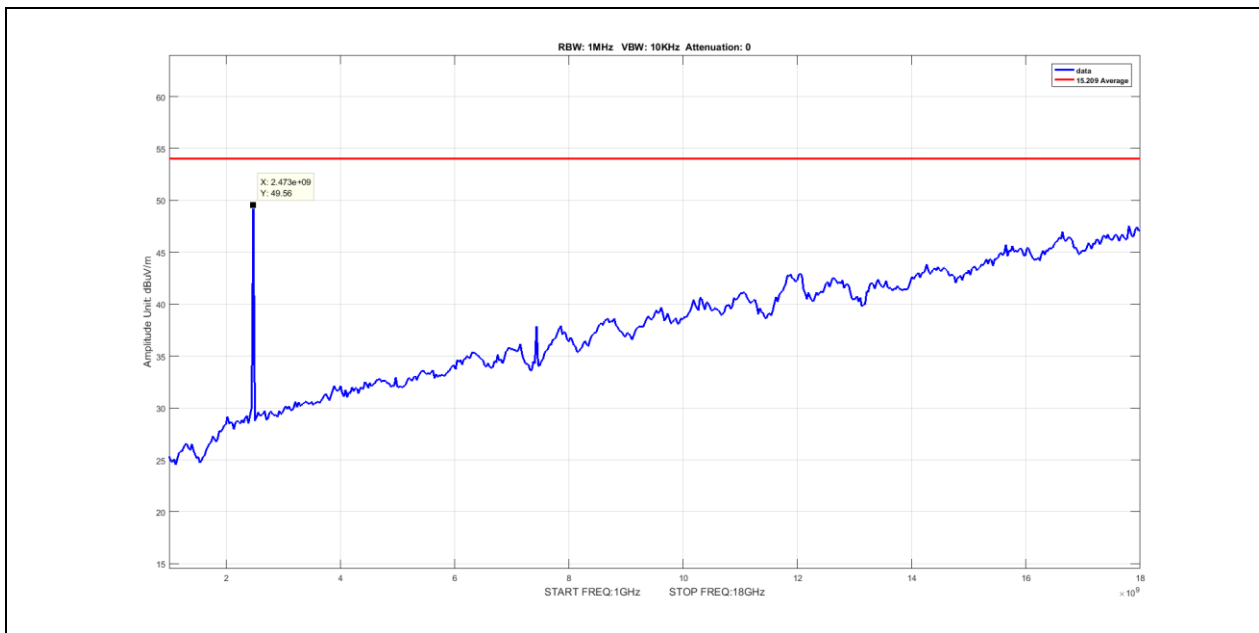
Plot 49. Radiated Spurious Emissions, Average, Nonhopping, 1G – 18G, DH1, 2480MHz
