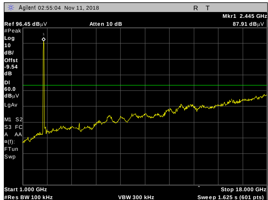
Plot 106. Conducted Spurious Emissions, Hopping, 3-DH5, 1 GHz – 18 GHz
