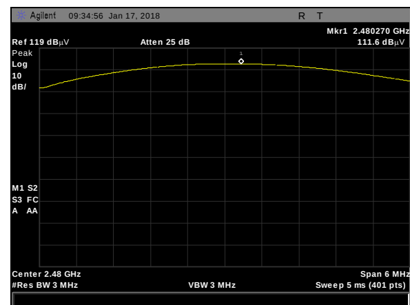
Plot 37. Peak Power Output, DH1, 2480MHz
