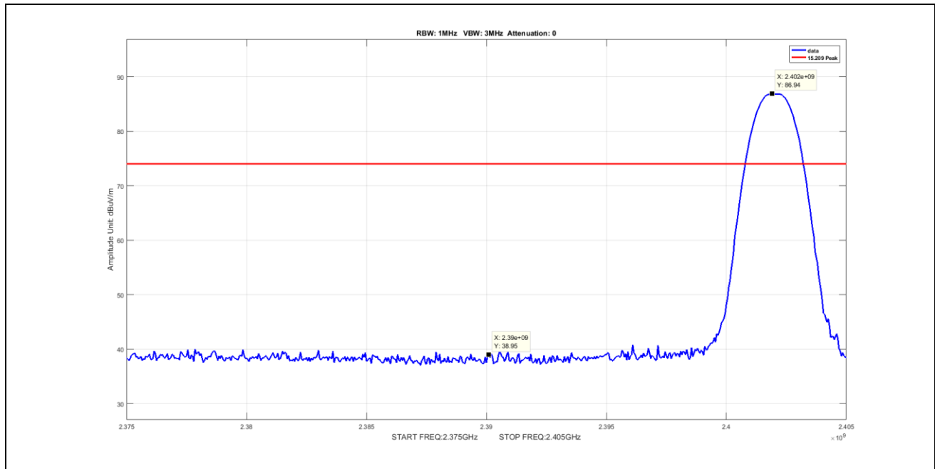
Plot 95. Radiated Restricted Band Edge, Peak, 2402MHz, DH1
