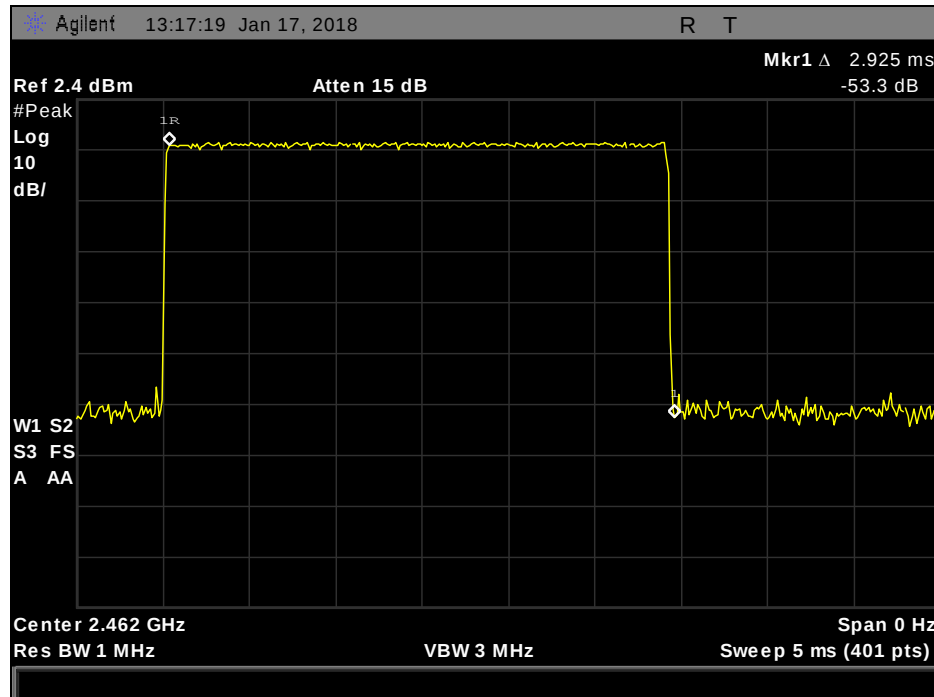
Plot 22. 3-DH5 Pulse Width
