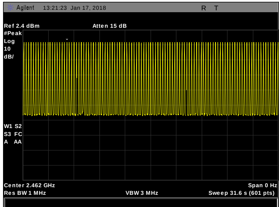
Plot 18. Dwell Time, 3-DH5 Burst
