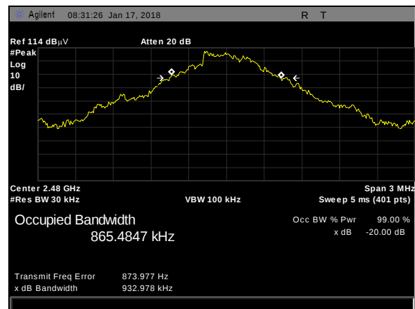
Plot 5. 20 dB Occupied Bandwidth, DH1, 2480 MHz
