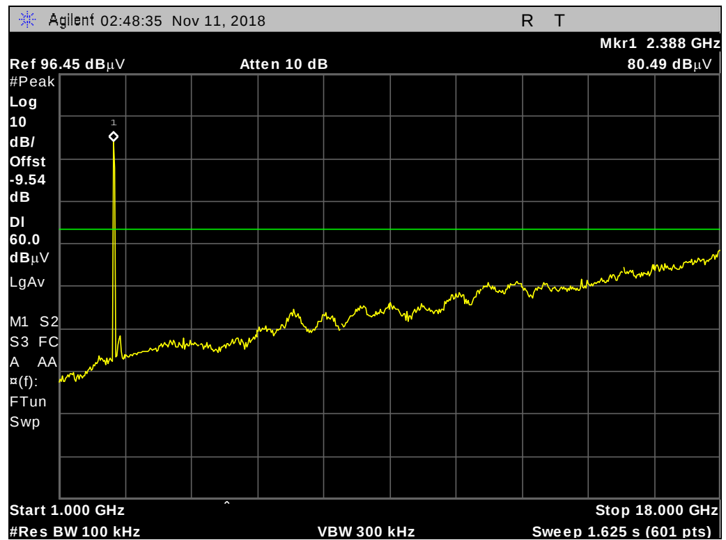
Plot 110. Conducted Spurious Emissions, Nonhopping, 2402MHz, 3-DH5, 1 GHz – 18 GHz
