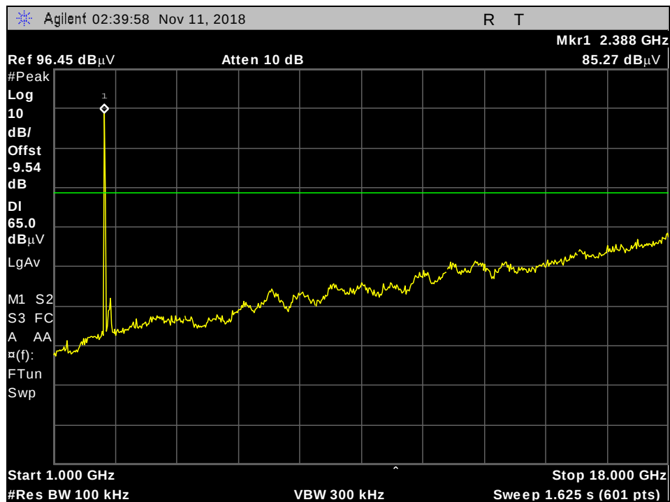
Plot 108. Conducted Spurious Emissions, Nonhopping, 2402MHz, DH5, 1 GHz – 18 GHz
