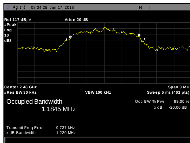
Plot 11. 20 dB Occupied Bandwidth, 3-DH1, 2480 MHz
