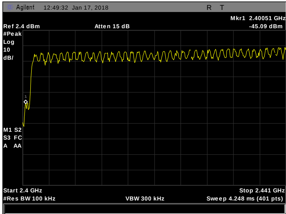
Plot 27. Number of Channels, 3-DH1.1
