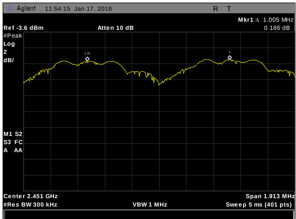
Plot 33. Channel Separation, 3-DH1
