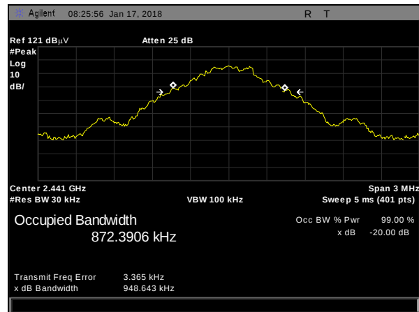
Plot 7. 20 dB Occupied Bandwidth, DH5, 2441 MHz
