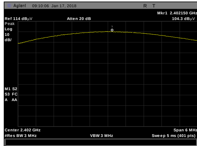
Plot 41. Peak Power Output, 3-DH1, 2402MHz
