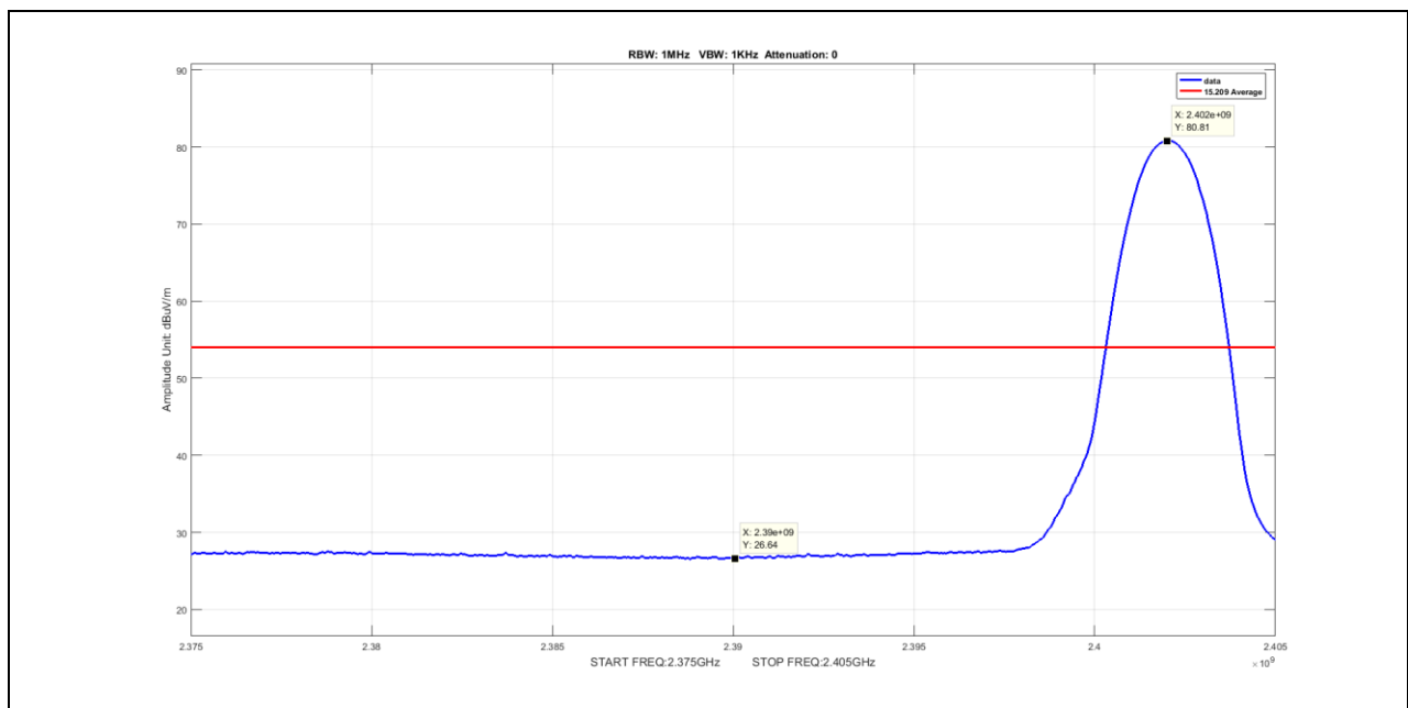
Plot 74. Radiated Restricted Band Edge, Average, 2390MHz, 3-DH5
