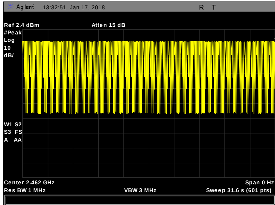
Plot 17. Dwell Time, 3-DH1 Burst
