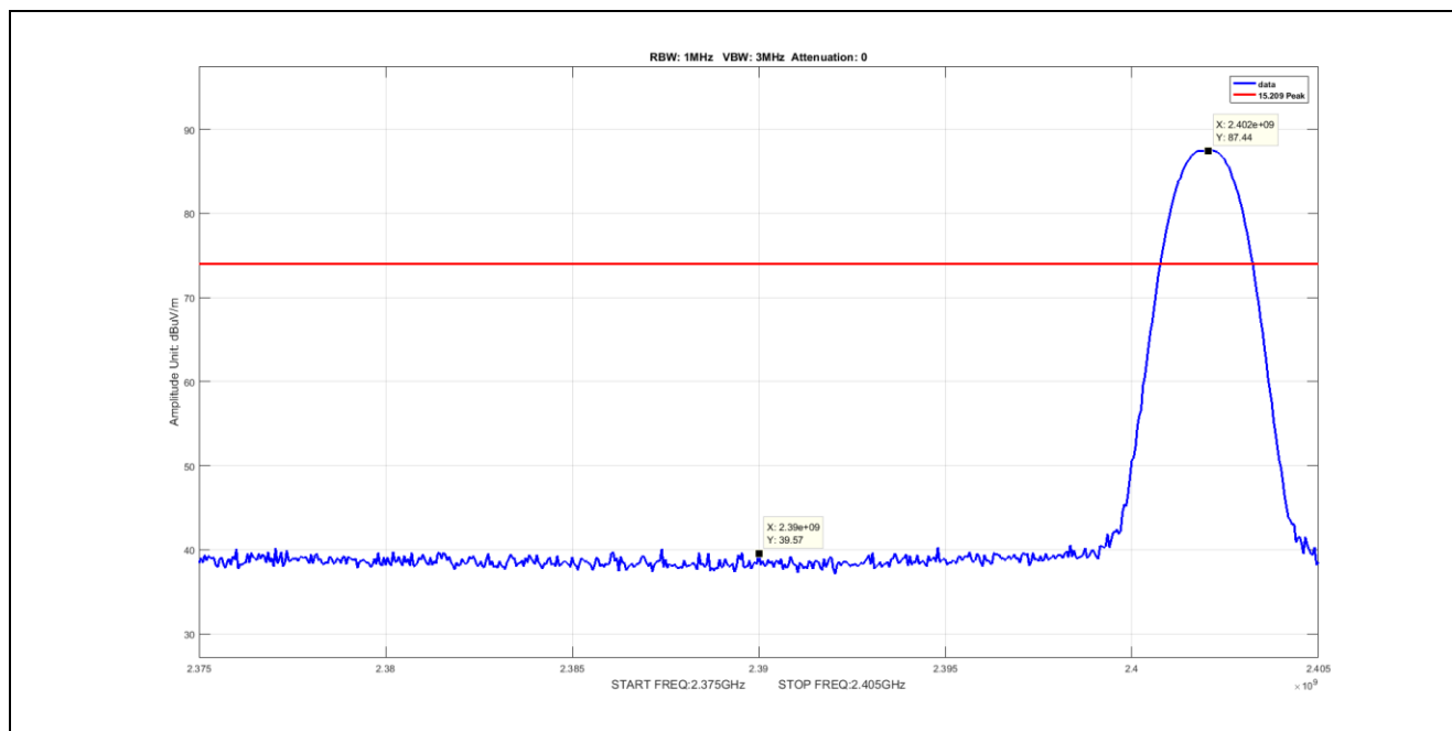
Plot 96. Radiated Restricted Band Edge, Peak, 2402MHz, DH5
