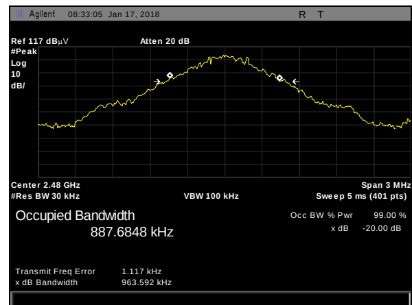
Plot 8. 20 dB Occupied Bandwidth, DH5, 2480 MHz
