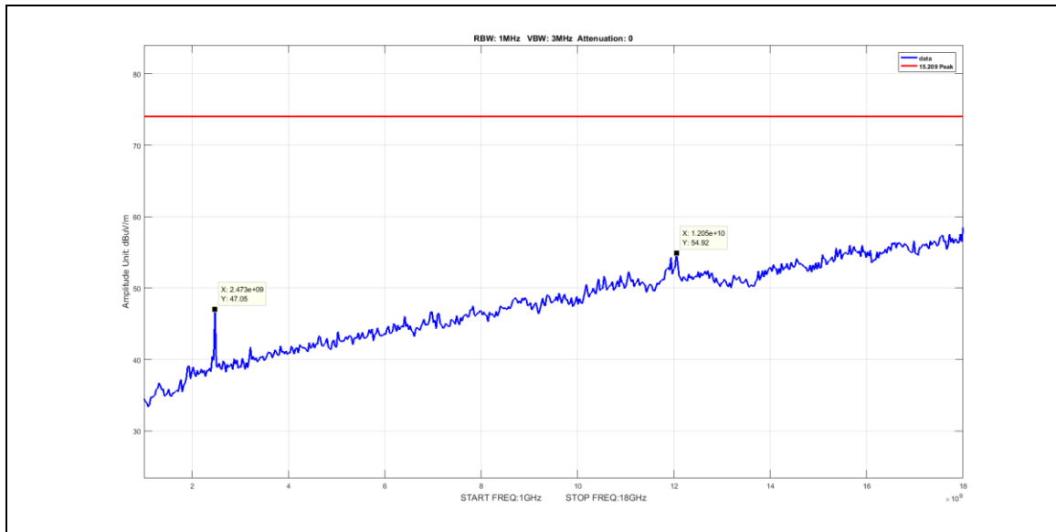
Plot 70. Radiated Spurious Emissions, Peak, Nonhopping, 1G – 18G, 3-DH5, 2480MHz
