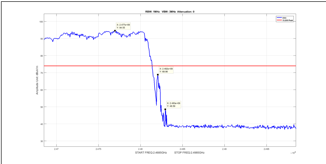
Plot 93. Radiated Restricted Band Edge, Peak, Hopping, 2483.5MHz, 3-DH1
