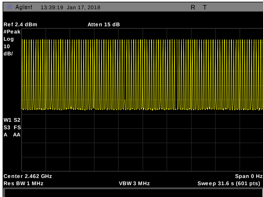
Plot 16. Dwell Time, DH5 Burst
