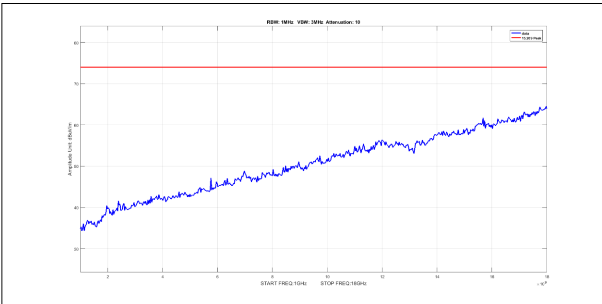
Plot 65. Radiated Spurious Emissions, Peak, Nonhopping, 1G – 18G, 3-DH1, 2402MHz
