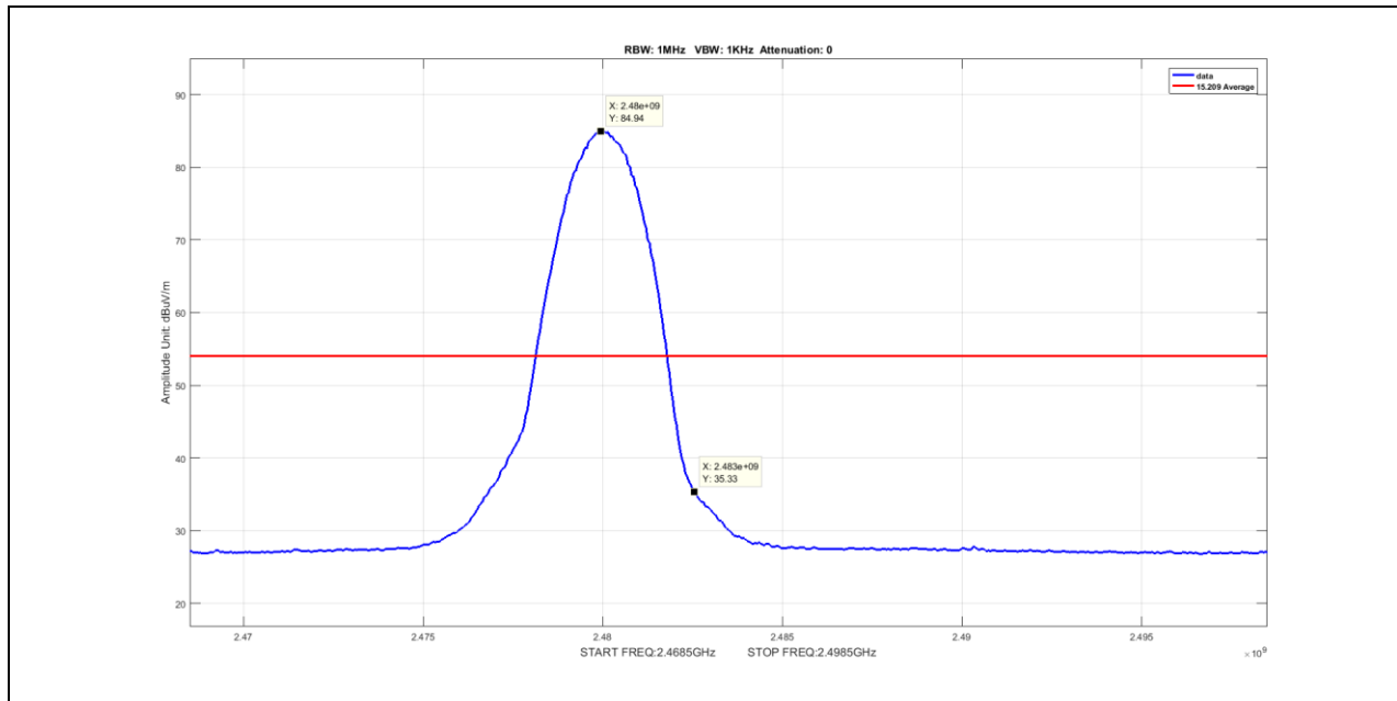
Plot 77. Radiated Restricted Band Edge, Average, 2483.5MHz, 3-DH1
