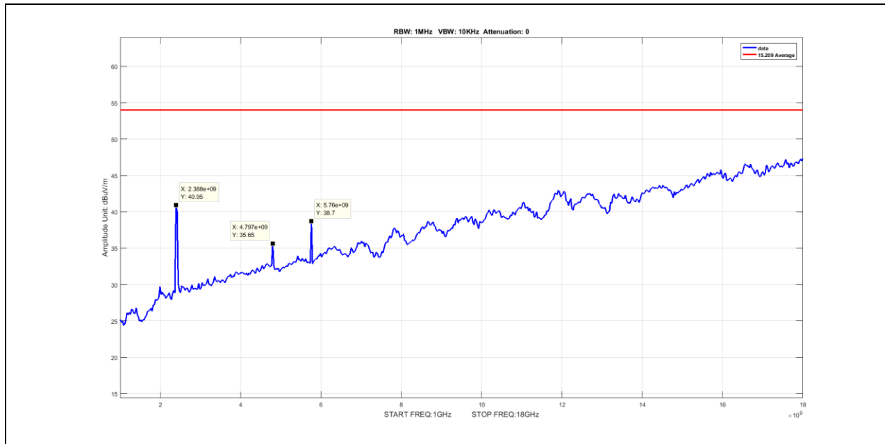
Plot 50. Radiated Spurious Emissions, Average, Nonhopping, 1G – 18G, DH5, 2402MHz
