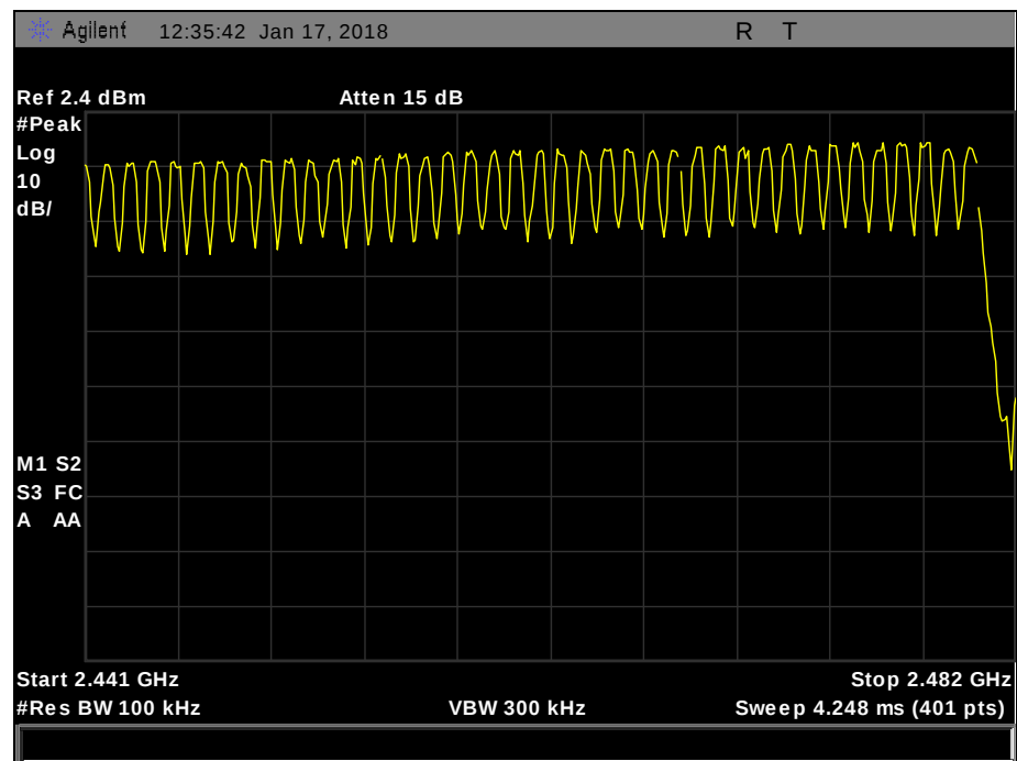
Plot 24. Number of Channels, DH1.2
