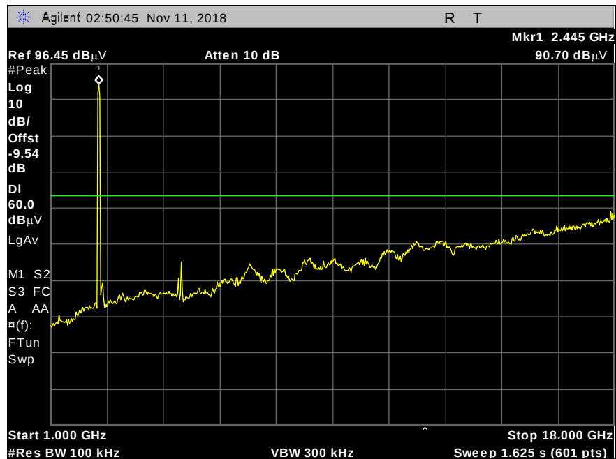
Plot 103. Conducted Spurious Emissions, Hopping, DH1, 1 GHz – 18 GHz
