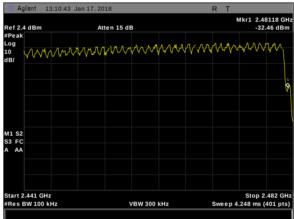
Plot 30. Number of Channels, 3-DH5.5
