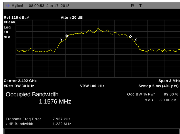
Plot 9. 20 dB Occupied Bandwidth, 3-DH1, 2402 MHz
