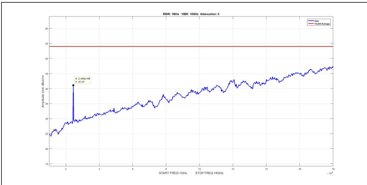
Plot 57. Radiated Spurious Emissions, Average, Nonhopping, 1G – 18G, 3-DH5, 2441MHz
