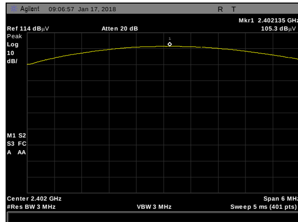
Plot 38. Peak Power Output, DH5, 2402MHz
