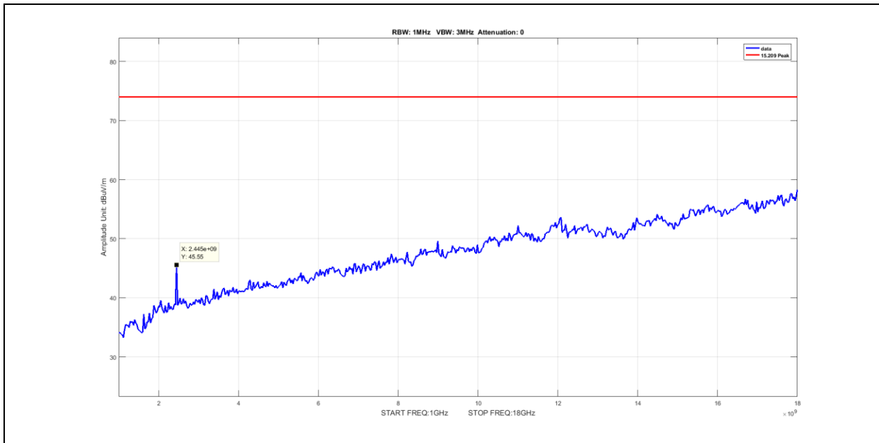
Plot 69. Radiated Spurious Emissions, Peak, Nonhopping, 1G – 18G, 3-DH5, 2441MHz
