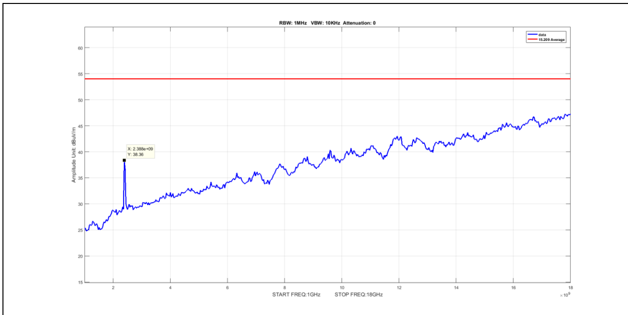
Plot 53. Radiated Spurious Emissions, Average, Nonhopping, 1G – 18G, 3-DH1, 2402MHz
