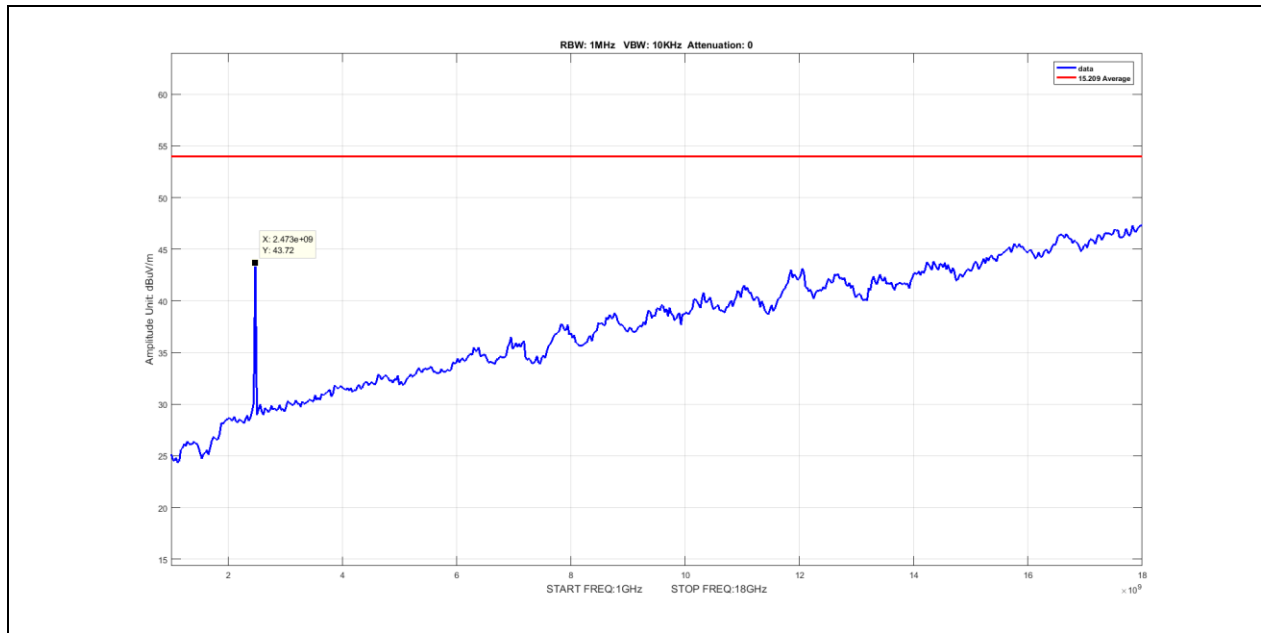
Plot 58. Radiated Spurious Emissions, Average, Nonhopping, 1G – 18G, 3-DH5, 2480MHz
