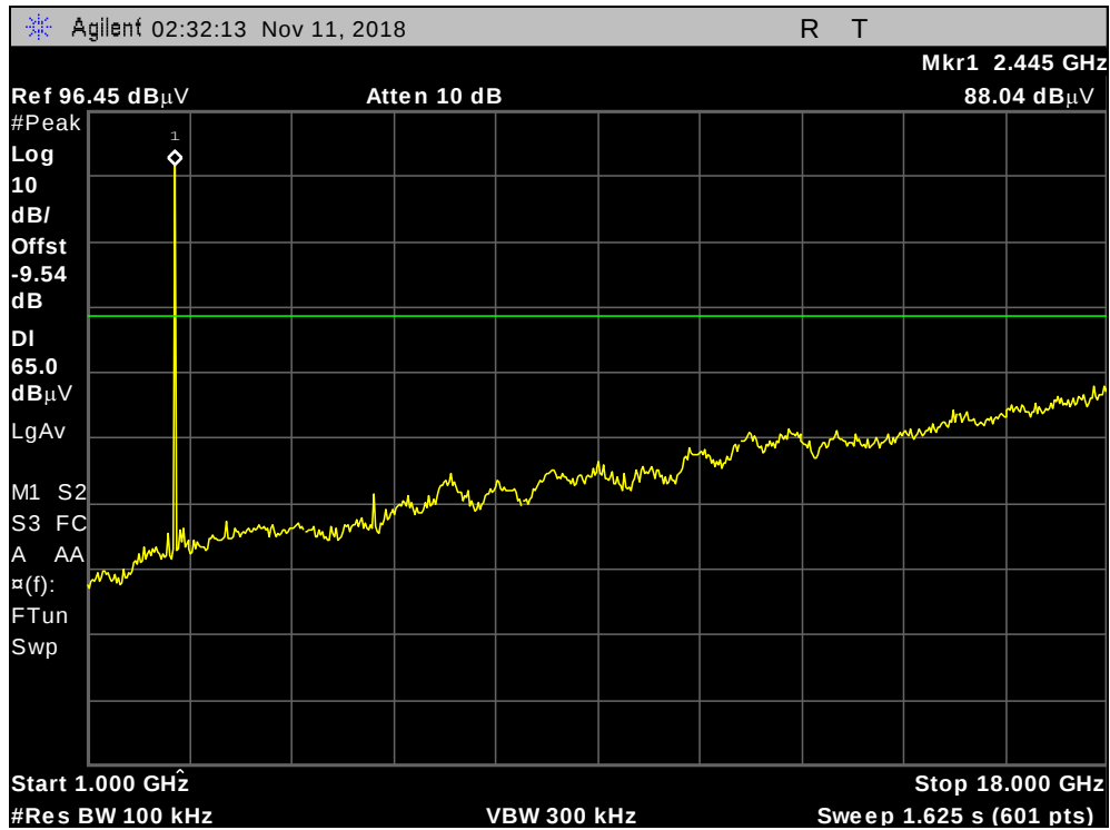
Plot 111. Conducted Spurious Emissions, Nonhopping, 2441MHz, DH1, 1 GHz – 18 GHz
