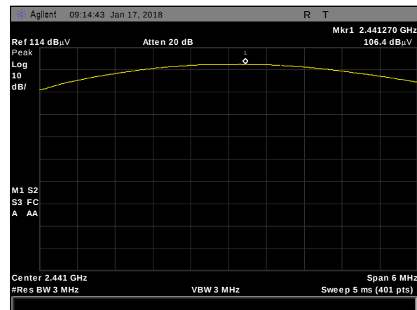
Plot 36. Peak Power Output, DH1, 2441MHz
