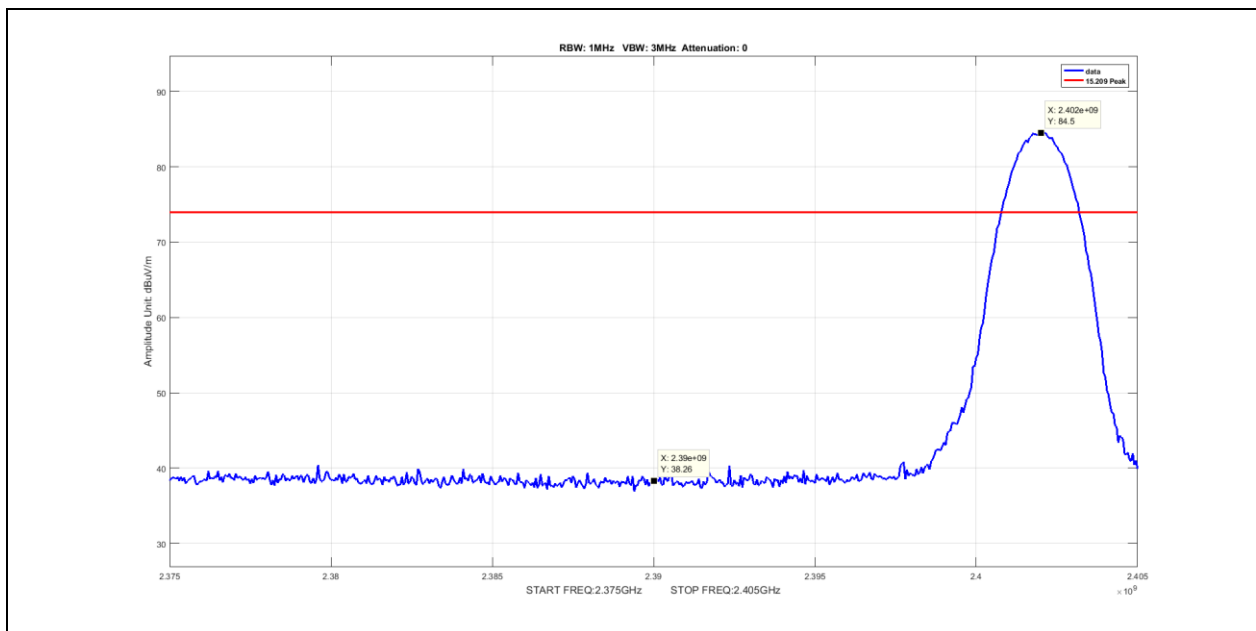
Plot 98. Radiated Restricted Band Edge, Peak, 2402MHz, 3-DH5
