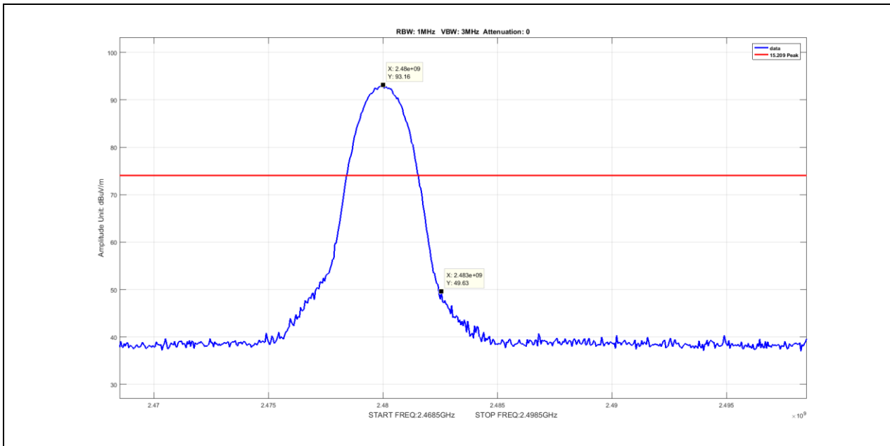
Plot 101. Radiated Restricted Band Edge, Peak, Nonhopping, 2480MHz, 3-DH1
