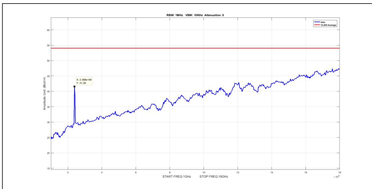
Plot 47. Radiated Spurious Emissions, Average, Nonhopping, 1G – 18G, DH1, 2402MHz
