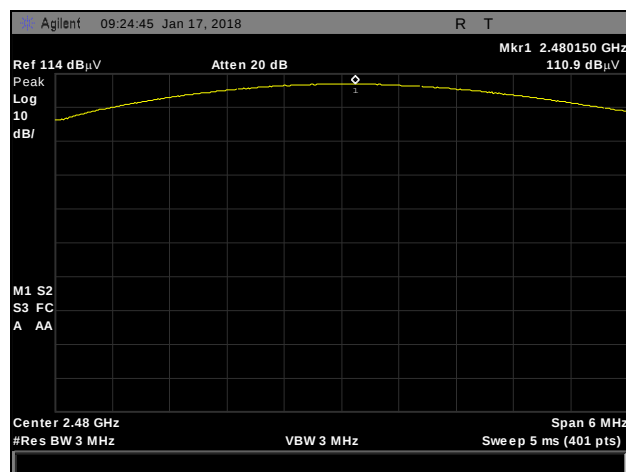
Plot 46. Peak Power Output, 3-DH5, 2480MHz
