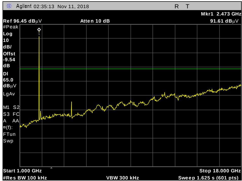
Plot 115. Conducted Spurious Emissions, Nonhopping, 2480MHz, DH1, 1 GHz – 18 GHz
