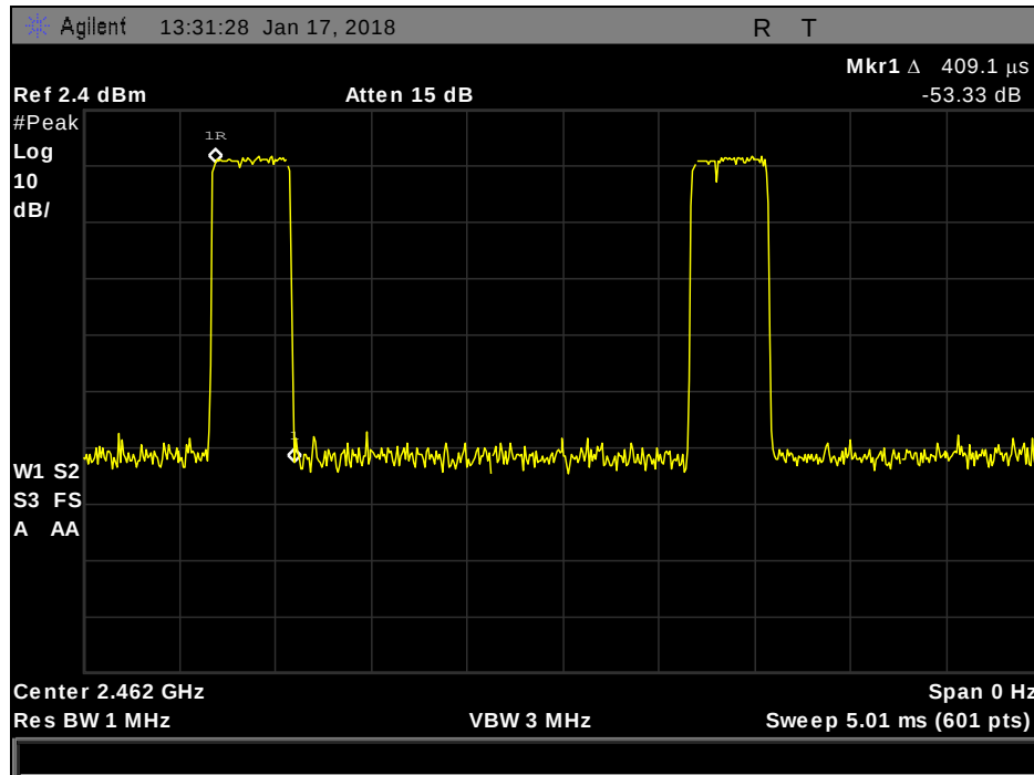
Plot 21. 3-DH1 Pulse Width
