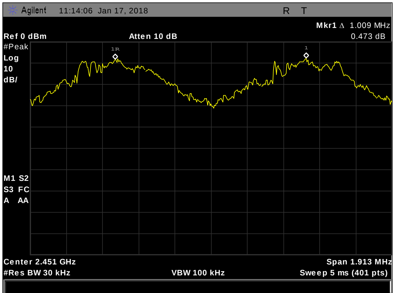
Plot 31. Channel Separation, DH1
