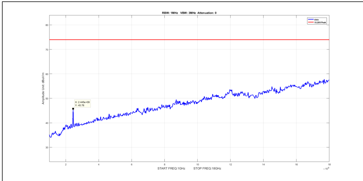
Plot 66. Radiated Spurious Emissions, Peak, Nonhopping, 1G – 18G, 3-DH1, 2441MHz
