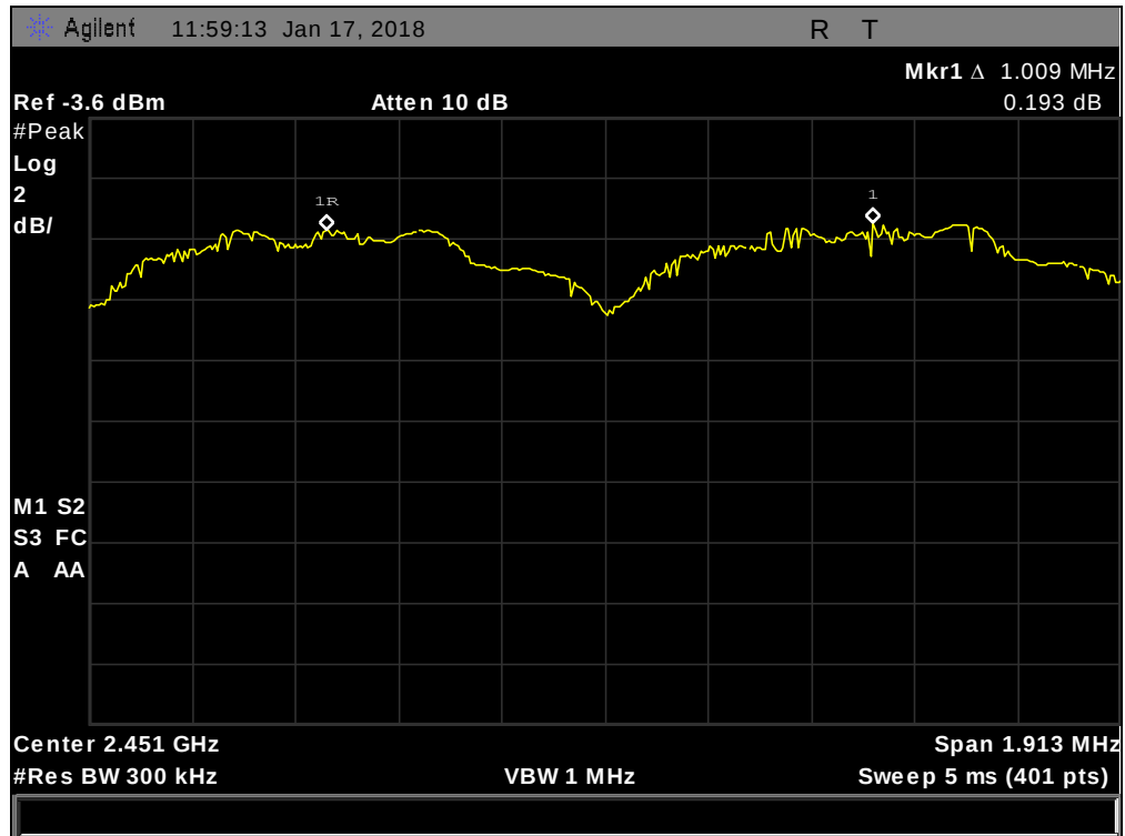
Plot 34. Channel Separation, 3-DH5
