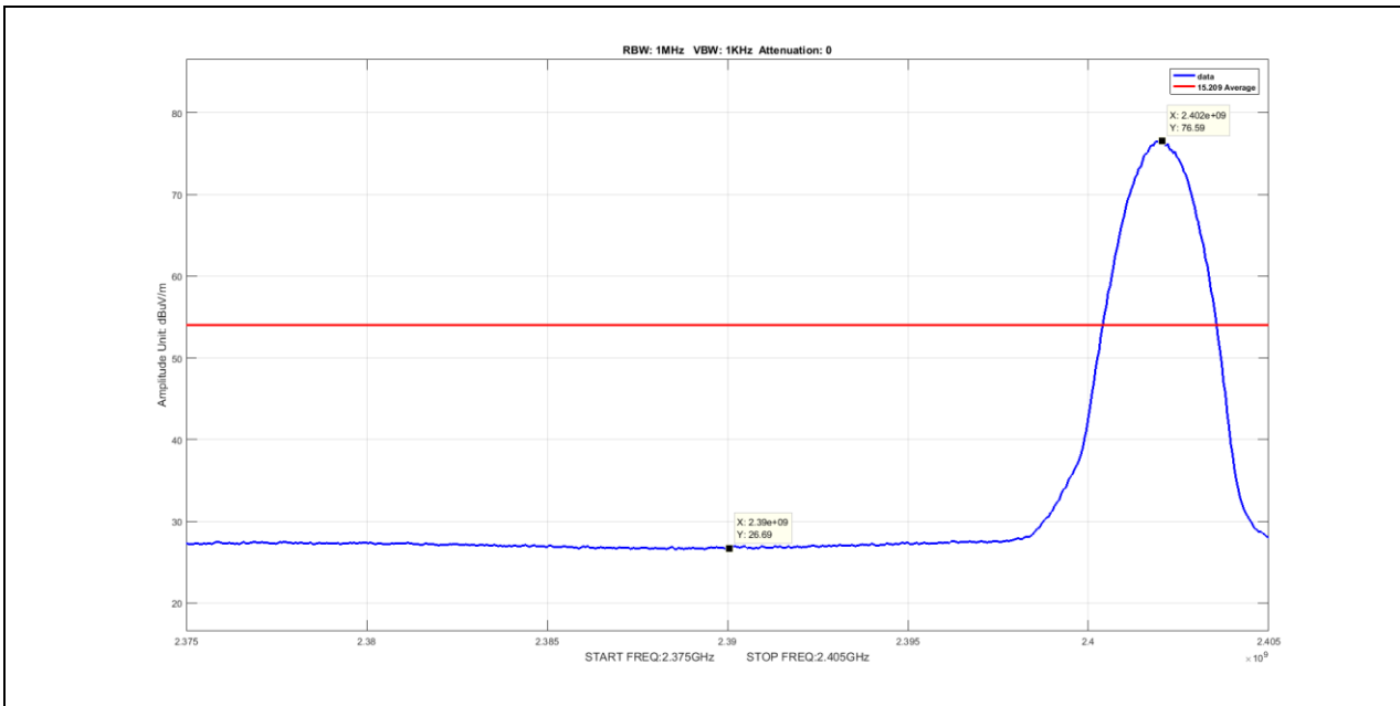
Plot 73. Radiated Restricted Band Edge, Average, 2390MHz, 3-DH1
