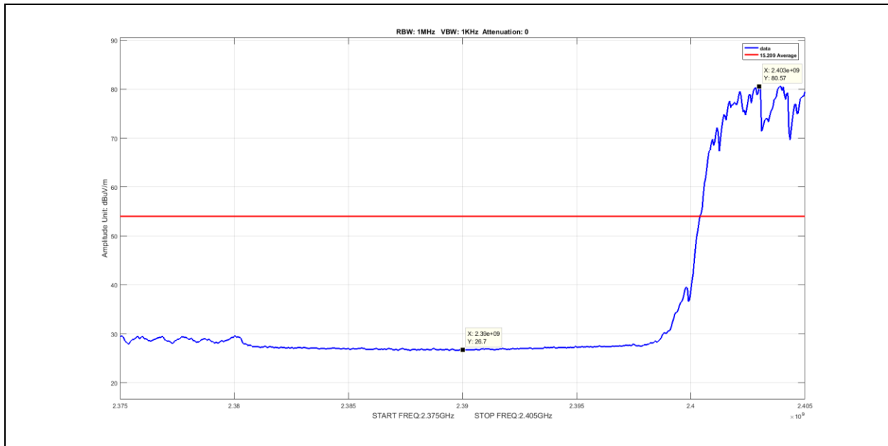
Plot 81. Radiated Restricted Band Edge, Average, Hopping, 2390MHz, 3-DH1
