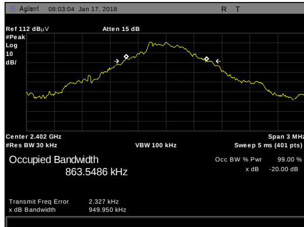
Plot 3. 20 dB Occupied Bandwidth, DH1, 2402 MHz
