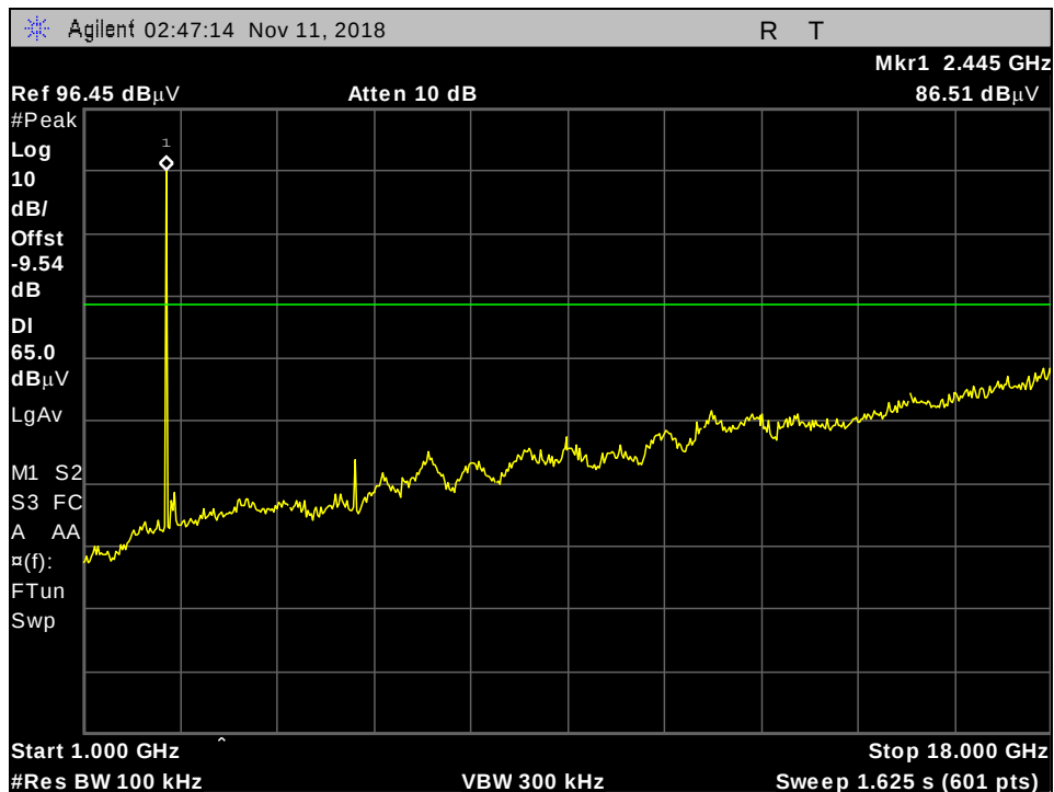
Plot 114. Conducted Spurious Emissions, Nonhopping, 2441MHz, 3-DH5, 1 GHz – 18 GHz
