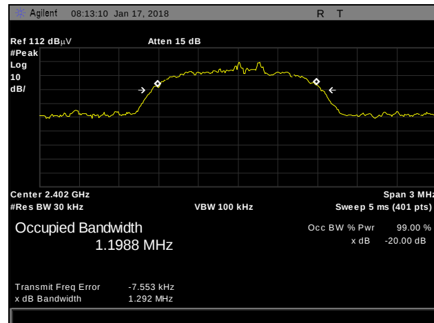
Plot 12. 20 dB Occupied Bandwidth, 3-DH5, 2402 MHz
