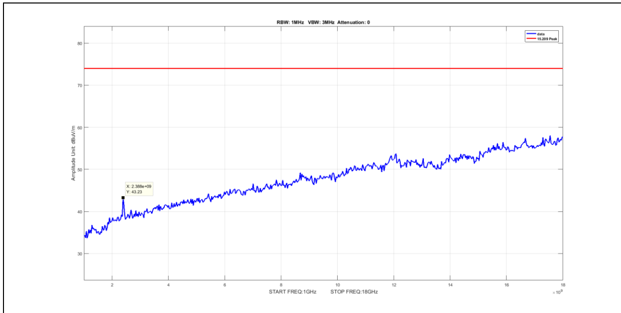
Plot 62. Radiated Spurious Emissions, Peak, Nonhopping, 1G – 18G, DH5, 2402MHz
