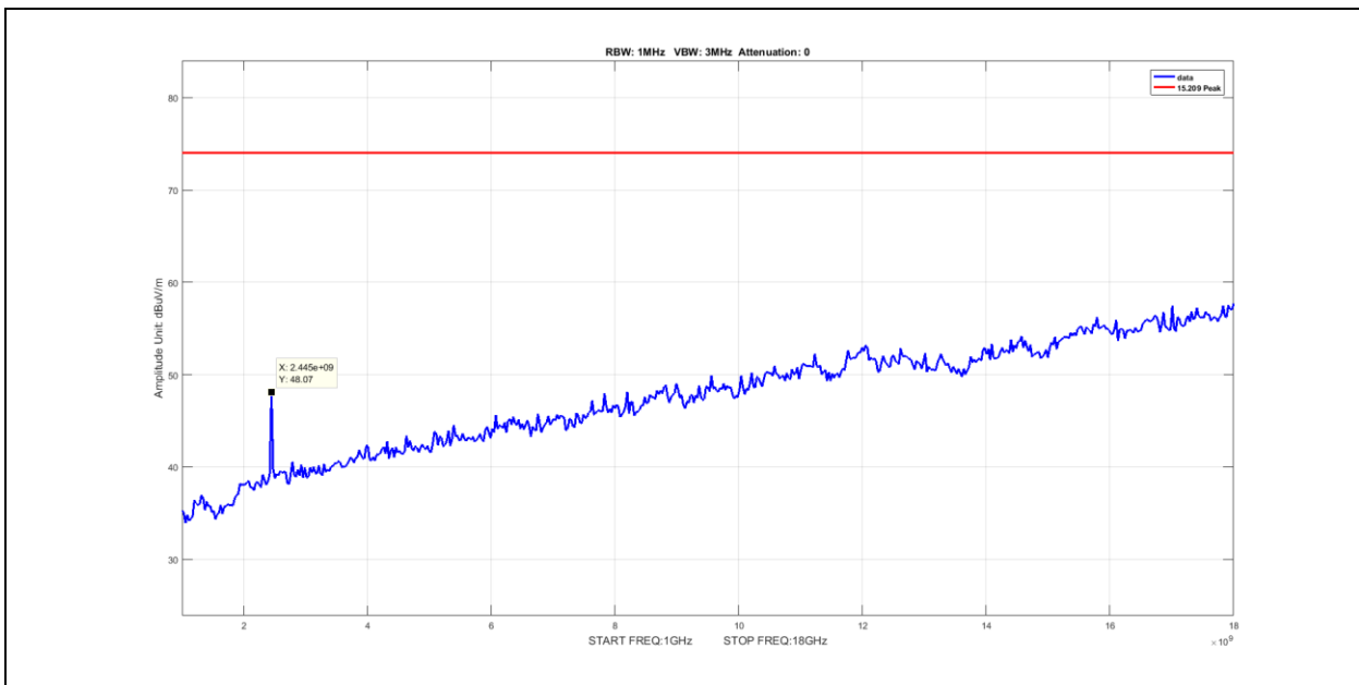
Plot 63. Radiated Spurious Emissions, Peak, Nonhopping, 1G – 18G, DH5, 2441MHz
