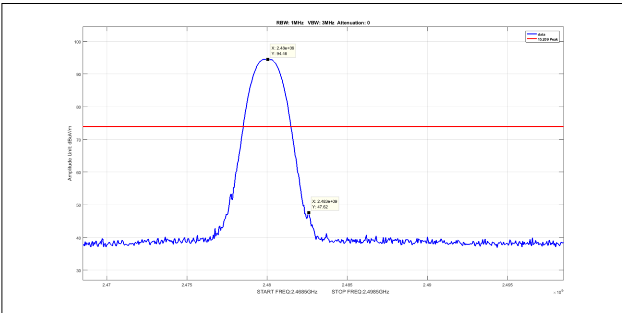
Plot 100. Radiated Restricted Band Edge, Peak, 2480MHz, DH5
