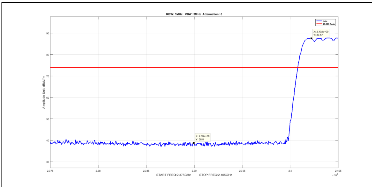
Plot 88. Radiated Restricted Band Edge, Peak, Hopping, 2390MHz, DH5
