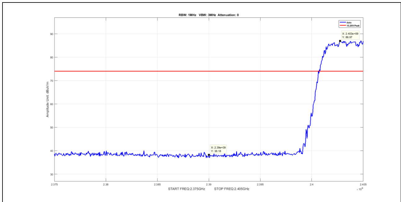
Plot 90. Radiated Restricted Band Edge, Peak, Hopping, 2390MHz, 3-DH5
