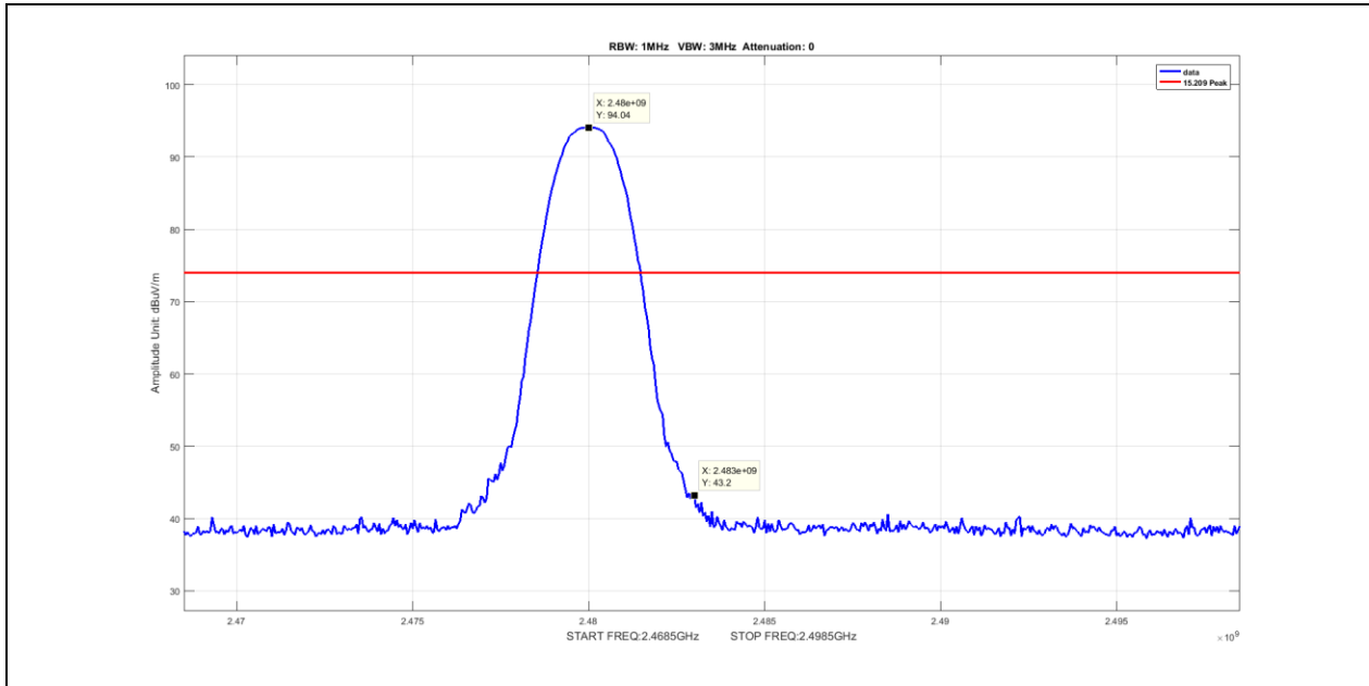
Plot 99. Radiated Restricted Band Edge, Peak, 2480MHz, DH1
