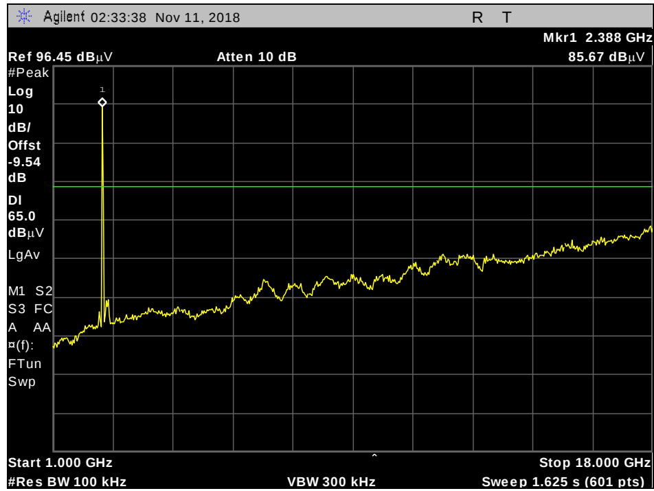
Plot 107. Conducted Spurious Emissions, Nonhopping, 2402MHz, DH1, 1 GHz – 18 GHz
