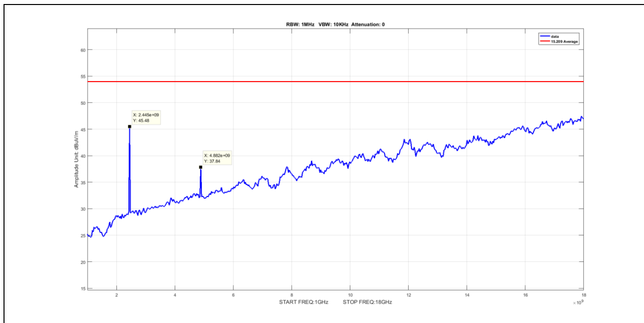
Plot 51. Radiated Spurious Emissions, Average, Nonhopping, 1G – 18G, DH5, 2441MHz
