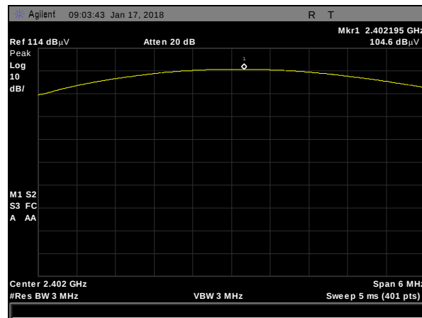
Plot 35. Peak Power Output, DH1, 2402MHz
