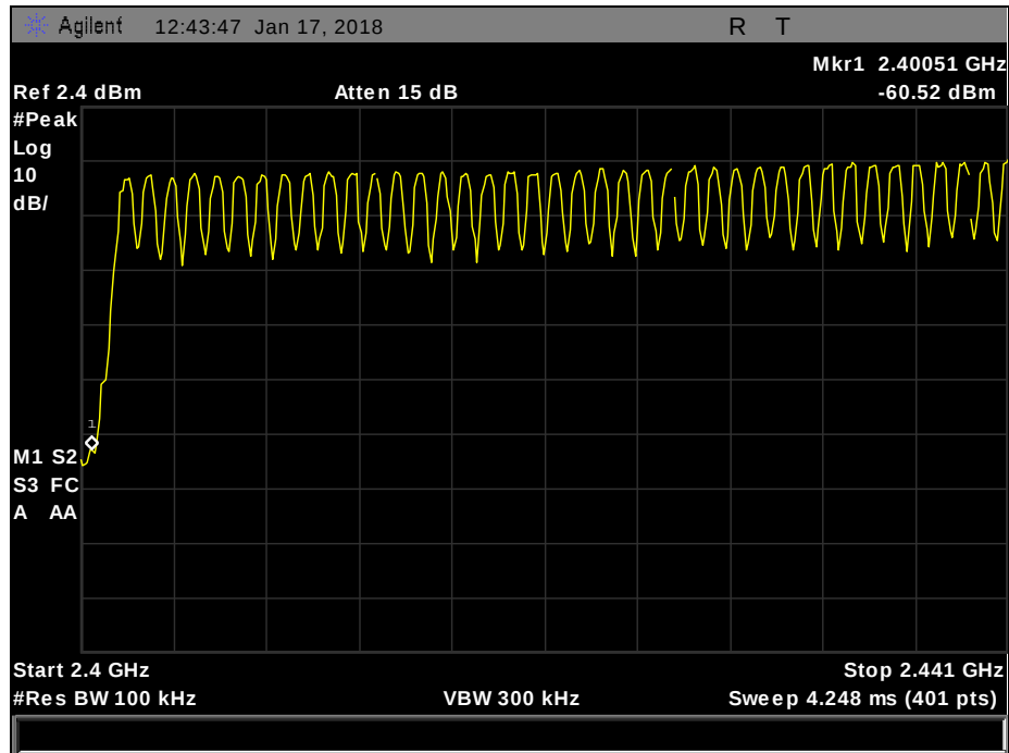
Plot 25. Number of Channels, DH5.1
