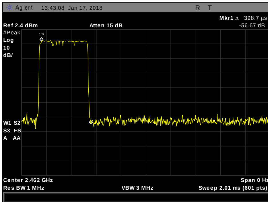
Plot 19. DH1 Pulse Width
