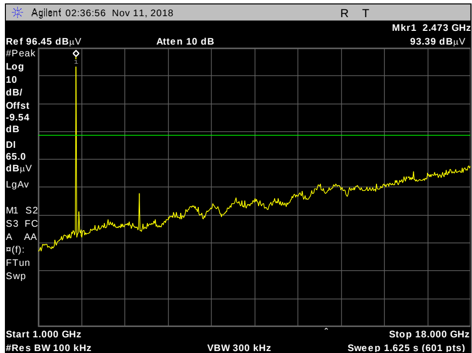
Plot 116. Conducted Spurious Emissions, Nonhopping, 2480MHz, DH5, 1 GHz – 18 GHz
