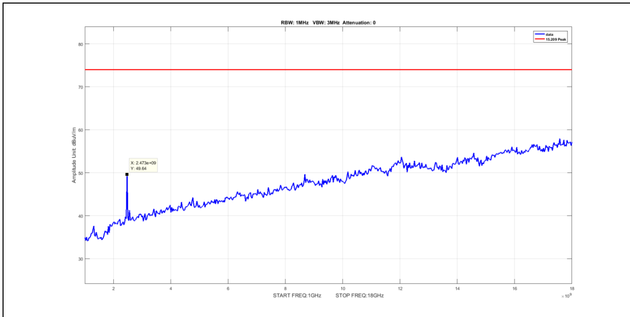
Plot 64. Radiated Spurious Emissions, Peak, Nonhopping, 1G – 18G, DH5, 2480MHz
