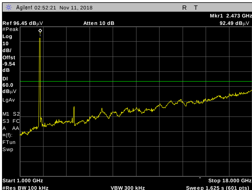
Plot 104. Conducted Spurious Emissions, Hopping, DH5, 1 GHz – 18 GHz
