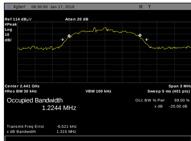
Plot 13. 20 dB Occupied Bandwidth, 3-DH5, 2441 MHz
