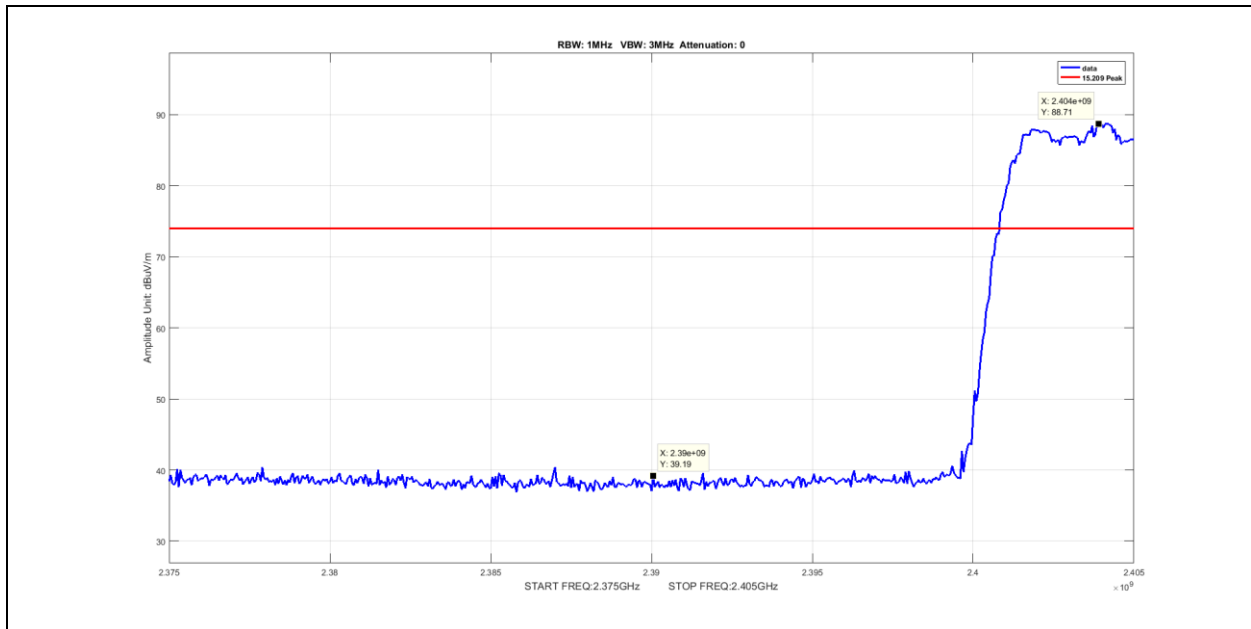
Plot 87. Radiated Restricted Band Edge, Peak, Hopping, 2390MHz, DH1
