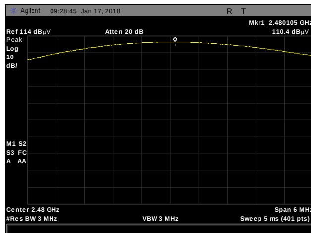
Plot 43. Peak Power Output, 3-DH1, 2480MHz
