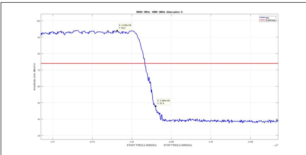
Plot 94. Radiated Restricted Band Edge, Peak, Hopping, 2483.5MHz, 3-DH5
