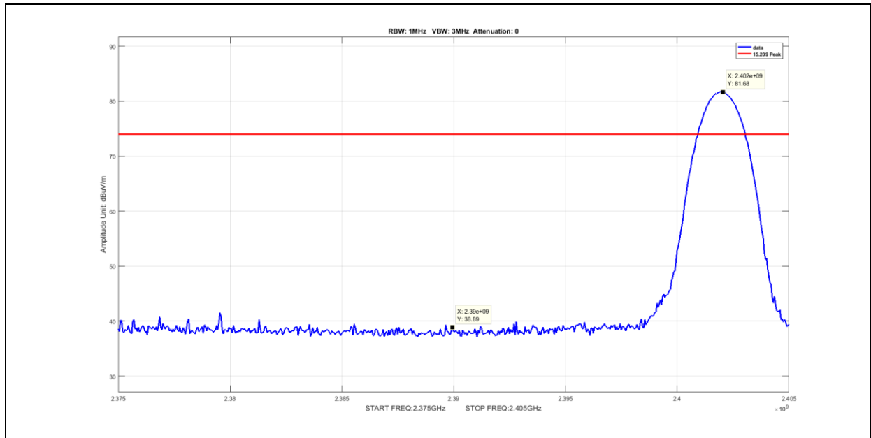
Plot 97. Radiated Restricted Band Edge, Peak, 2402MHz, 3-DH1
