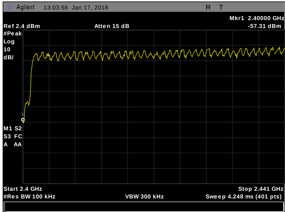
Plot 29. Number of Channels, 3-DH5.1
