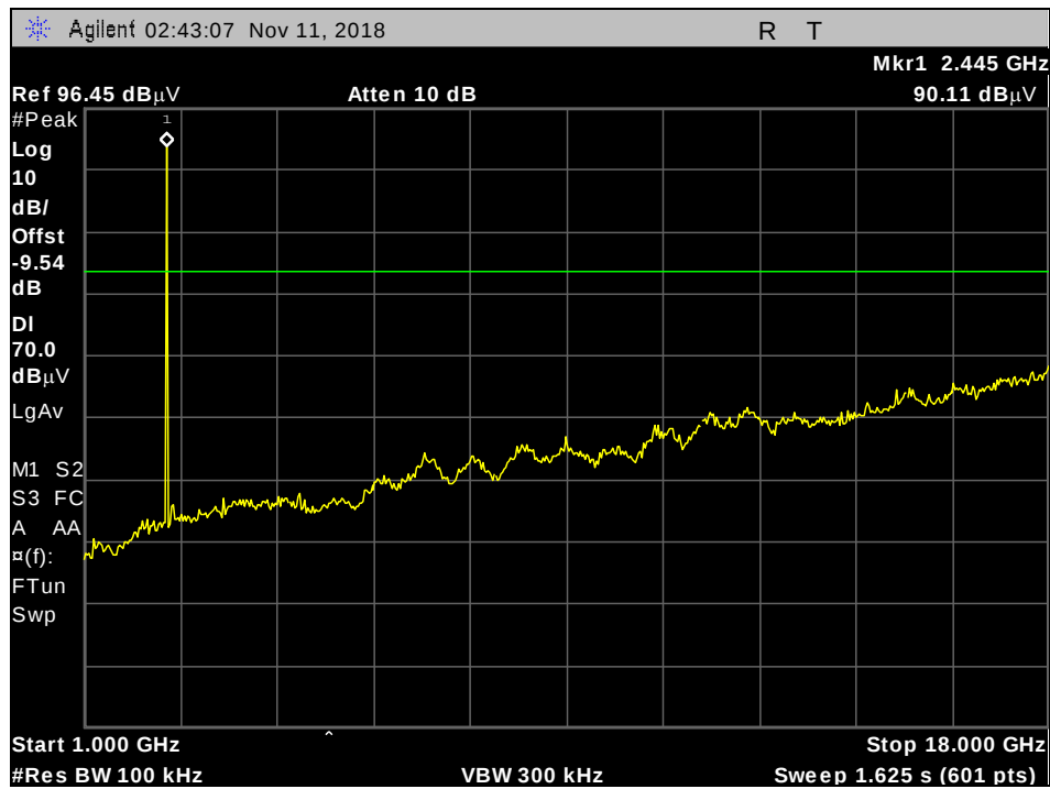
Plot 113. Conducted Spurious Emissions, Nonhopping, 2441MHz, 3-DH1, 1 GHz – 18 GHz
