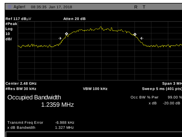
Plot 14. 20 dB Occupied Bandwidth, 3-DH5, 2480 MHz
