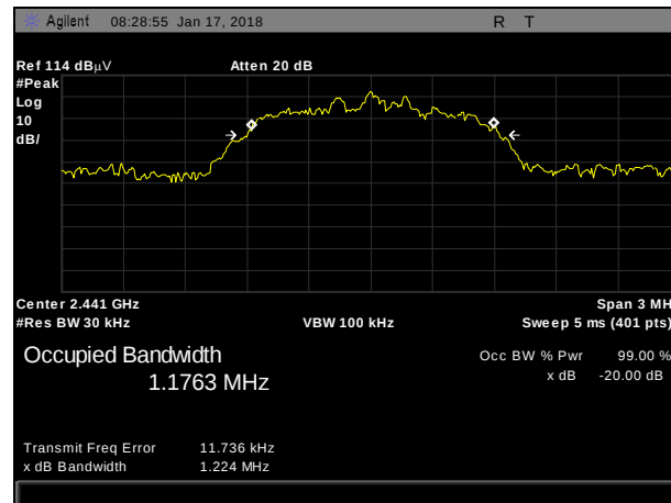
Plot 10. 20 dB Occupied Bandwidth, 3-DH1, 2441 MHz
