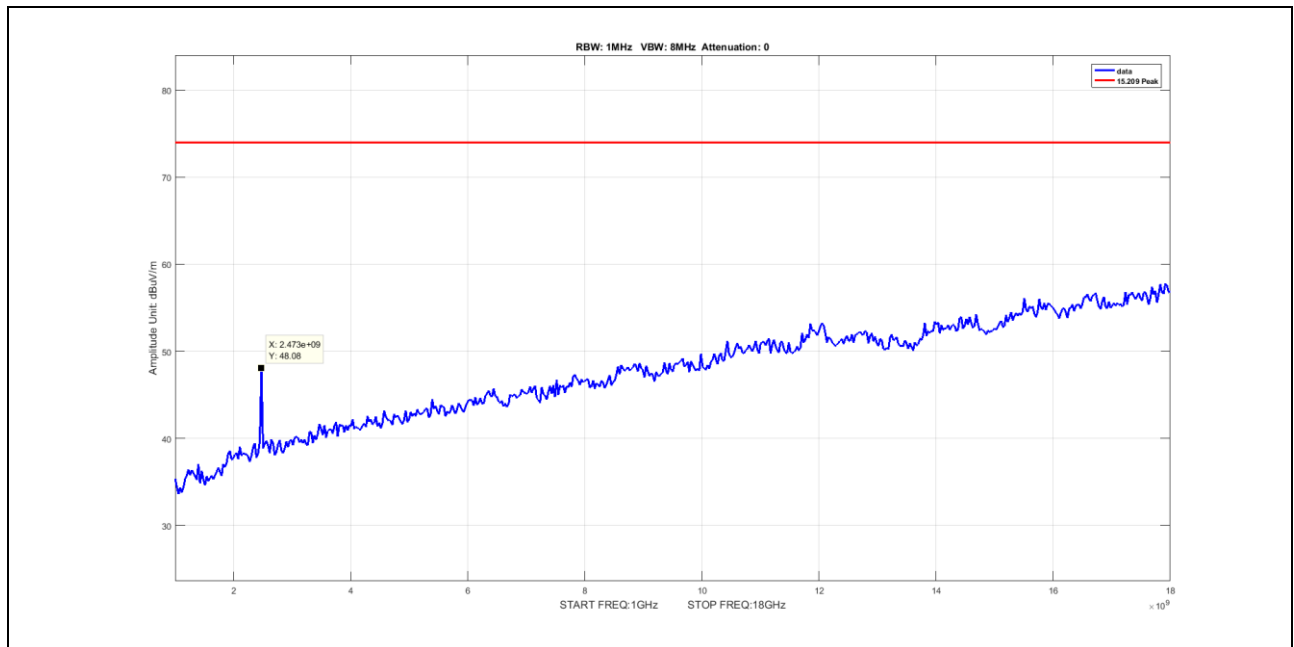
Plot 61. Radiated Spurious Emissions, Peak, Nonhopping, 1G – 18G, DH1, 2480MHz
