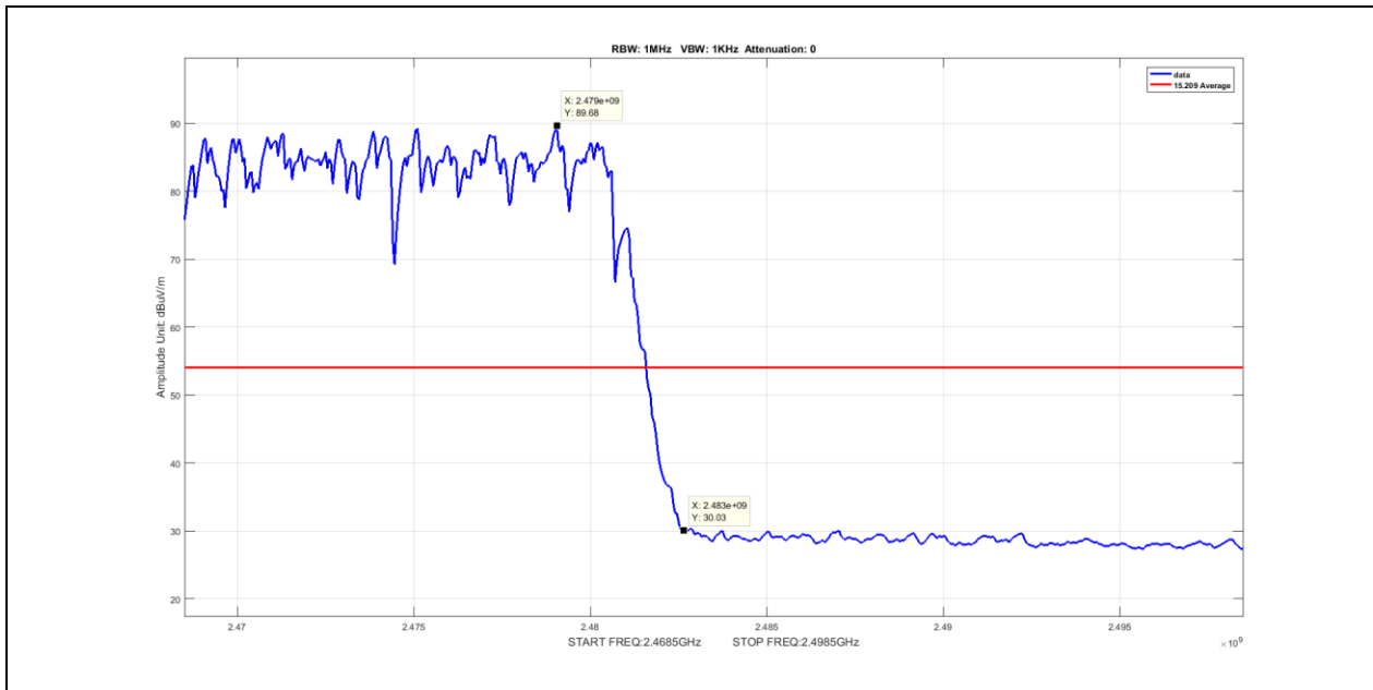
Plot 83. Radiated Restricted Band Edge, Average, Hopping, 2483.5MHz, DH1
