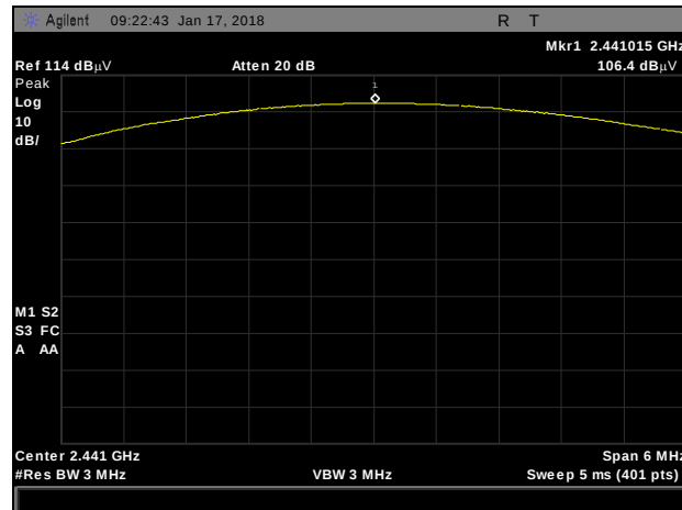
Plot 45. Peak Power Output, 3-DH5, 2441MHz
