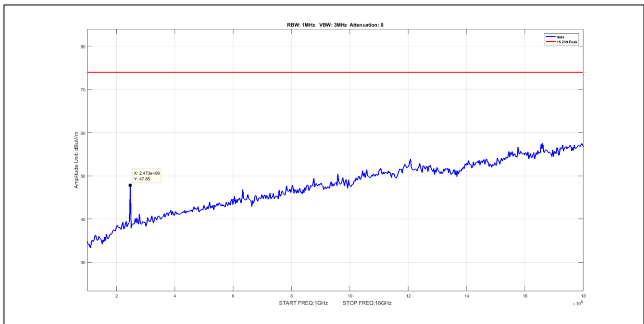
Plot 67. Radiated Spurious Emissions, Peak, Nonhopping, 1G – 18G, 3-DH1, 2480MHz
