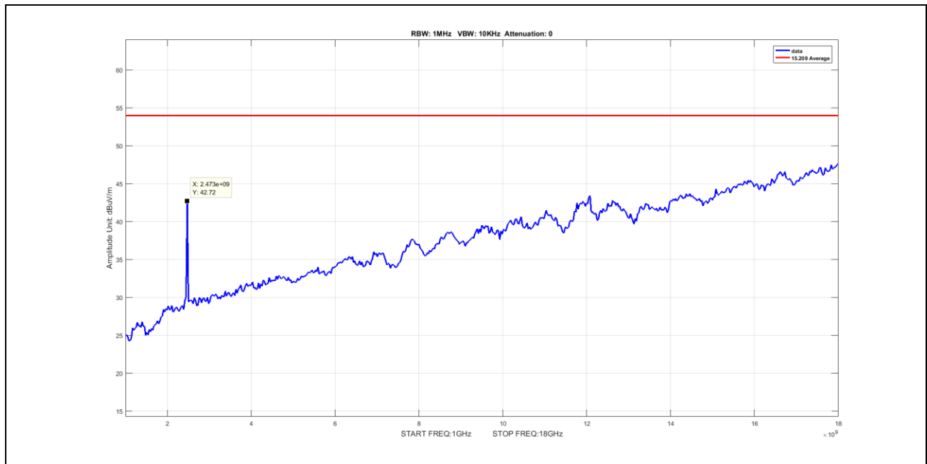
Plot 55. Radiated Spurious Emissions, Average, Nonhopping, 1G – 18G, 3-DH1, 2480MHz
