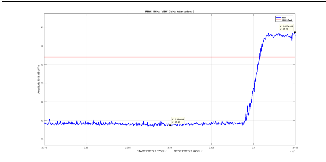
Plot 89. Radiated Restricted Band Edge, Peak, Hopping, 2390MHz, 3-DH1
