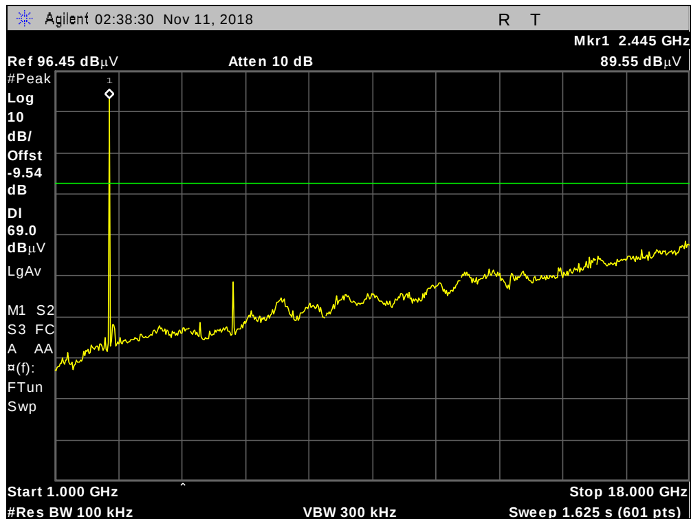
Plot 112. Conducted Spurious Emissions, Nonhopping, 2441MHz, DH5, 1 GHz – 18 GHz
