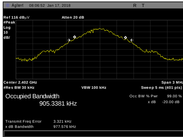
Plot 6. 20 dB Occupied Bandwidth, DH5, 2402 MHz
