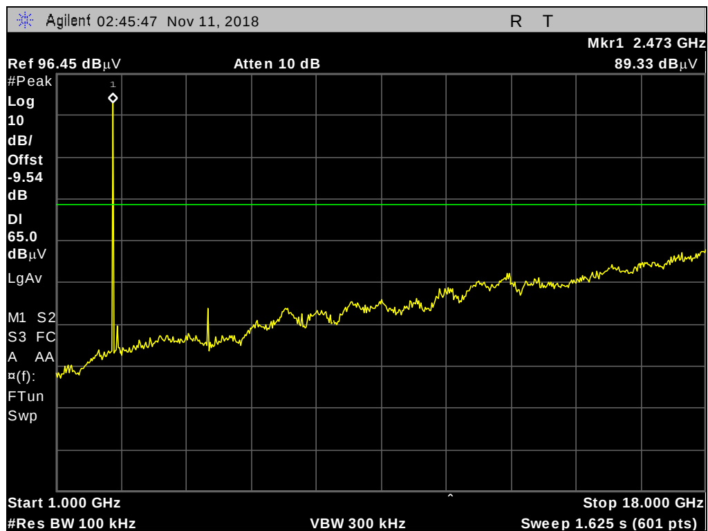
Plot 118. Conducted Spurious Emissions, Nonhopping, 2480MHz, 3-DH5, 1 GHz – 18 GHz
