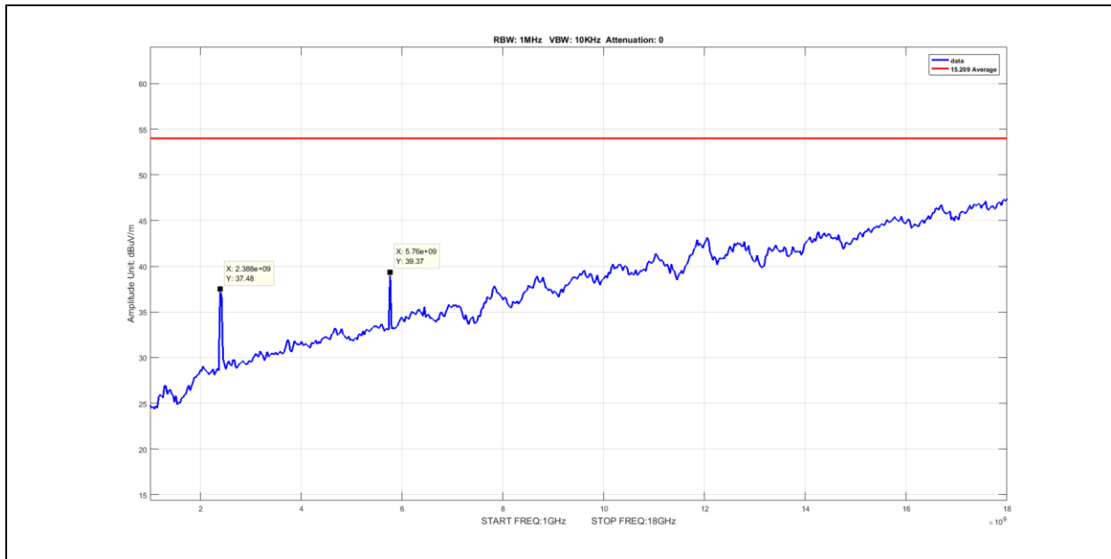
Plot 56. Radiated Spurious Emissions, Average, Nonhopping, 1G – 18G, 3-DH5, 2402MHz
