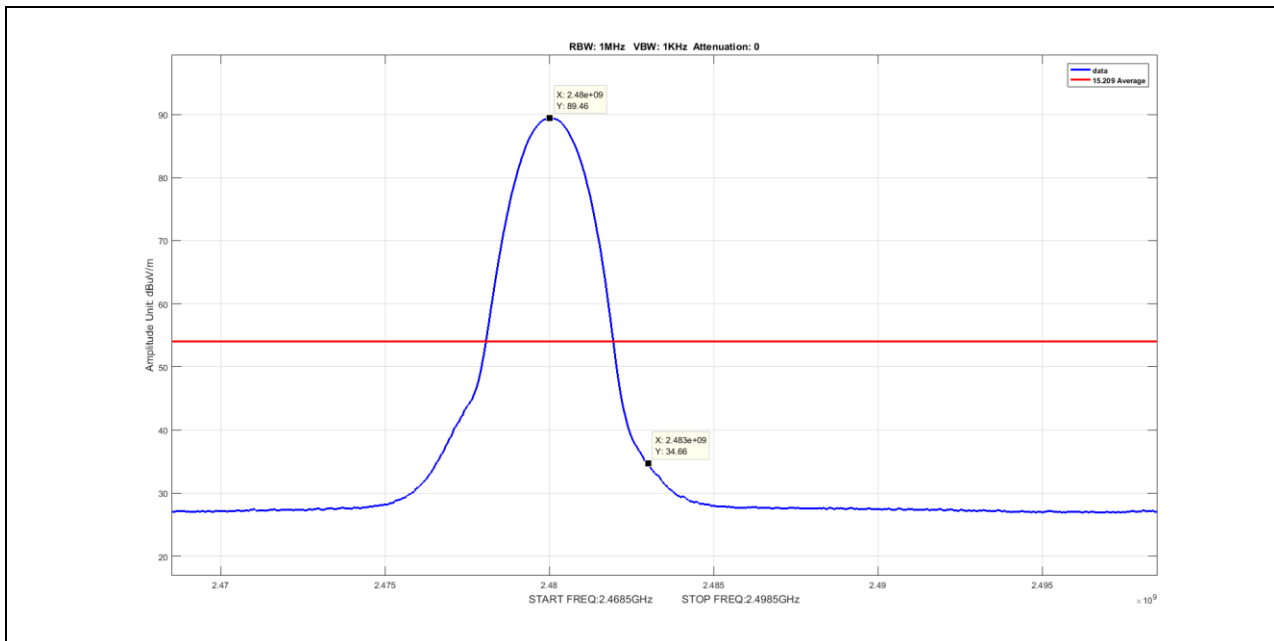
Plot 78. Radiated Restricted Band Edge, Average, 2483.5MHz, 3-DH5
