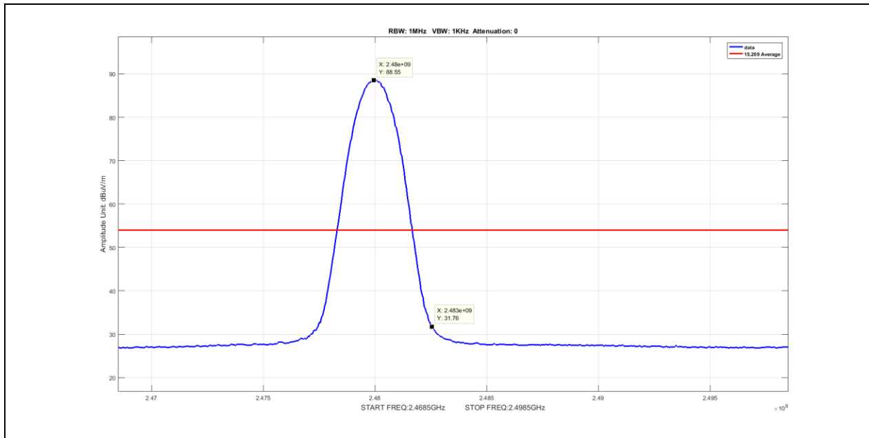
Plot 75. Radiated Restricted Band Edge, Average, 2483.5MHz, DH1
