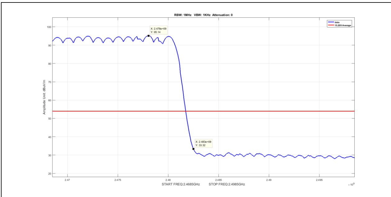
Plot 84. Radiated Restricted Band Edge, Average, Hopping, 2483.5MHz, DH5
