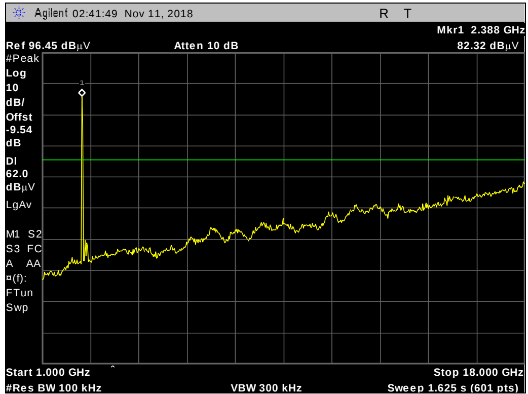
Plot 109. Conducted Spurious Emissions, Nonhopping, 2402MHz, 3-DH1, 1 GHz – 18 GHz
