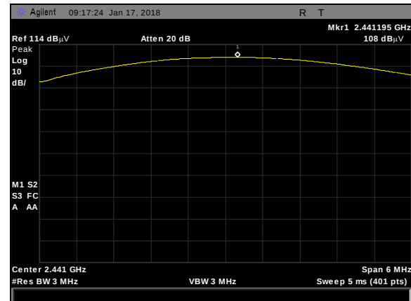
Plot 39. Peak Power Output, DH5, 2441MHz
