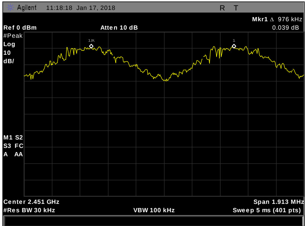
Plot 32. Channel Separation, DH5
