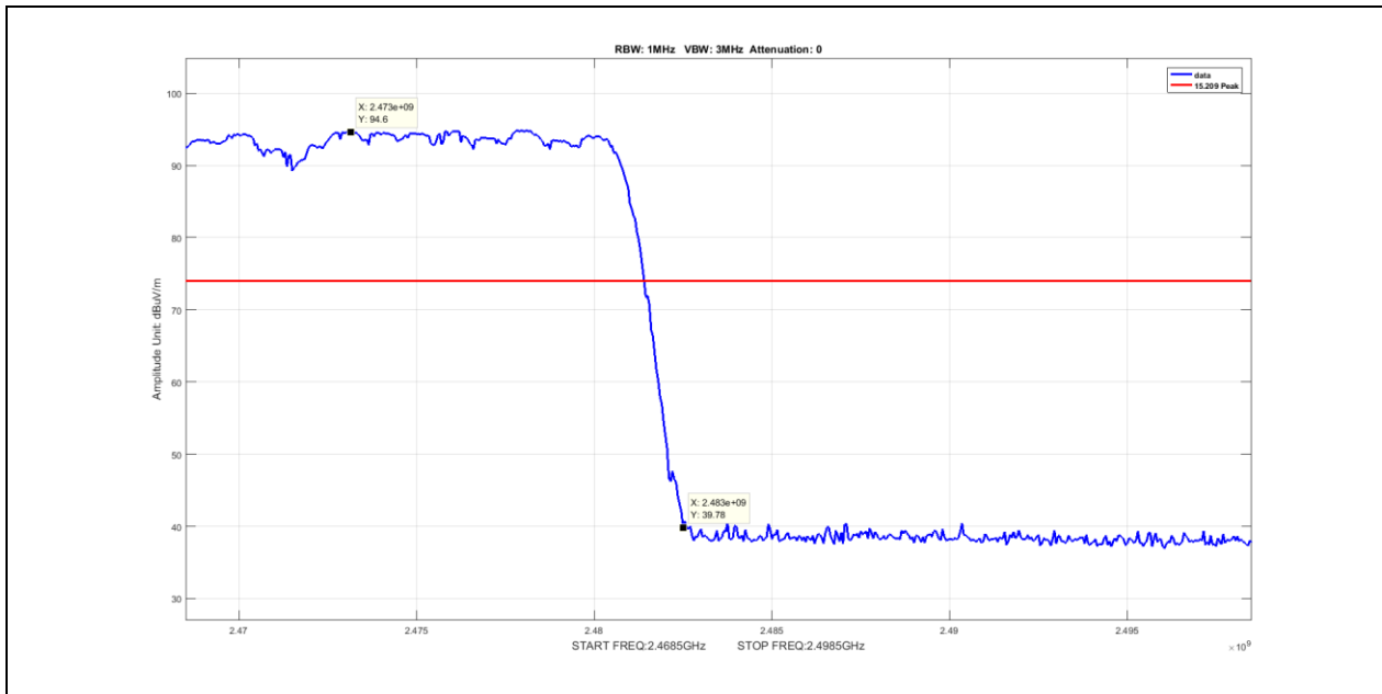
Plot 91. Radiated Restricted Band Edge, Peak, Hopping, 2483.5MHz, DH1
