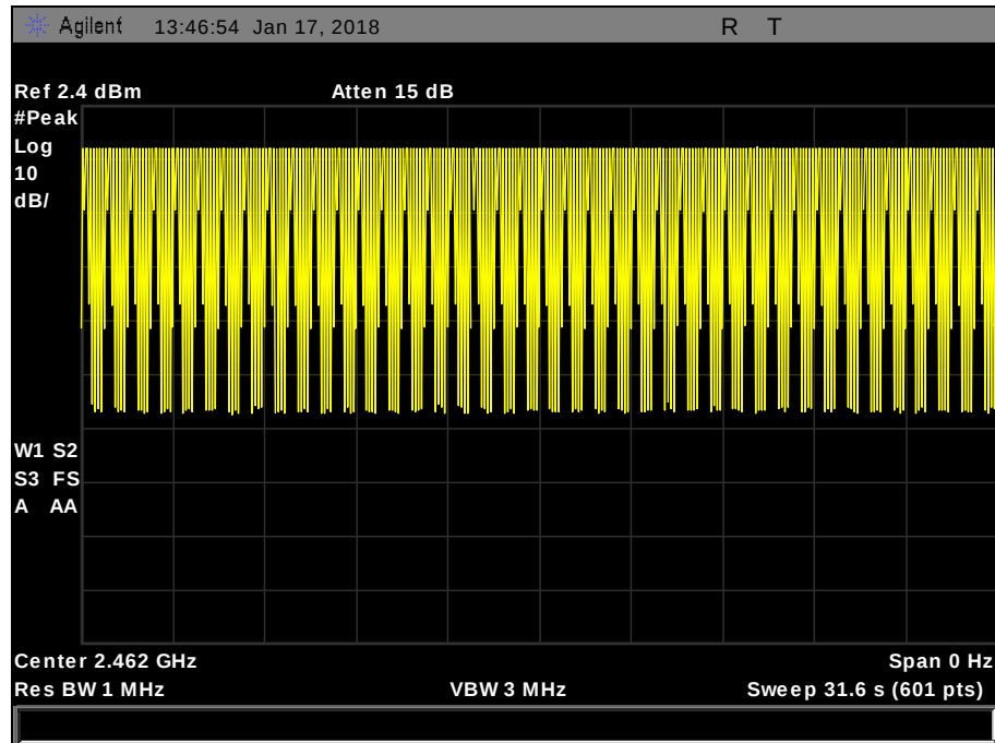
Plot 15. Dwell Time, DH1 Burst
