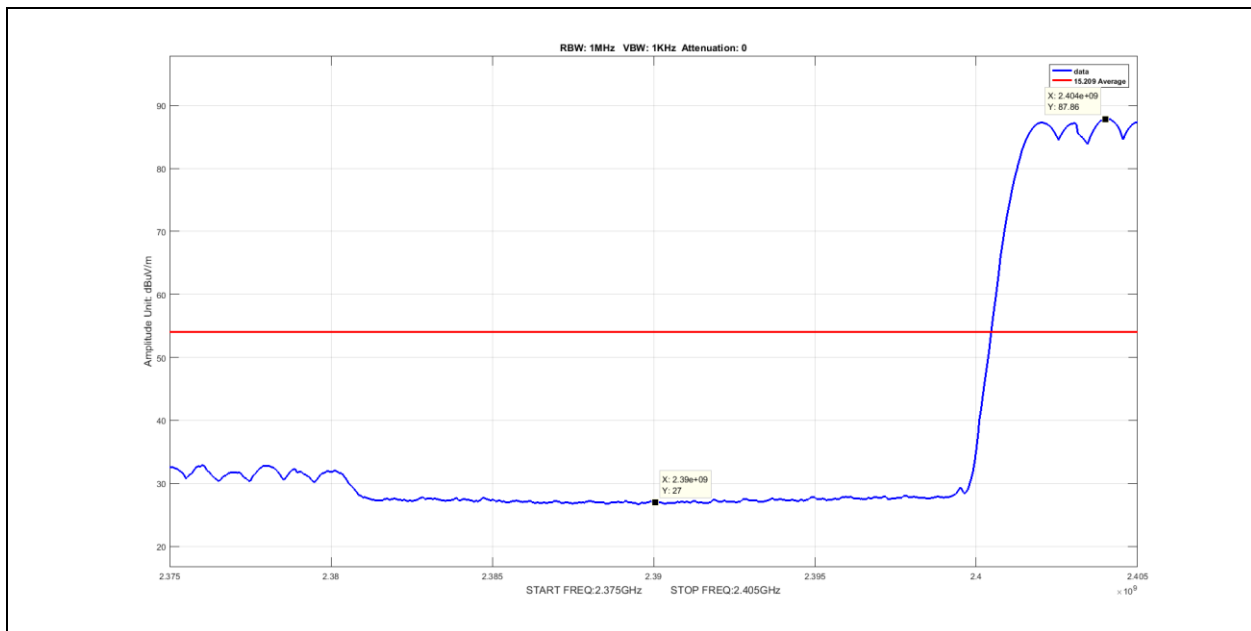
Plot 80. Radiated Restricted Band Edge, Average, Hopping, 2390MHz, DH5
