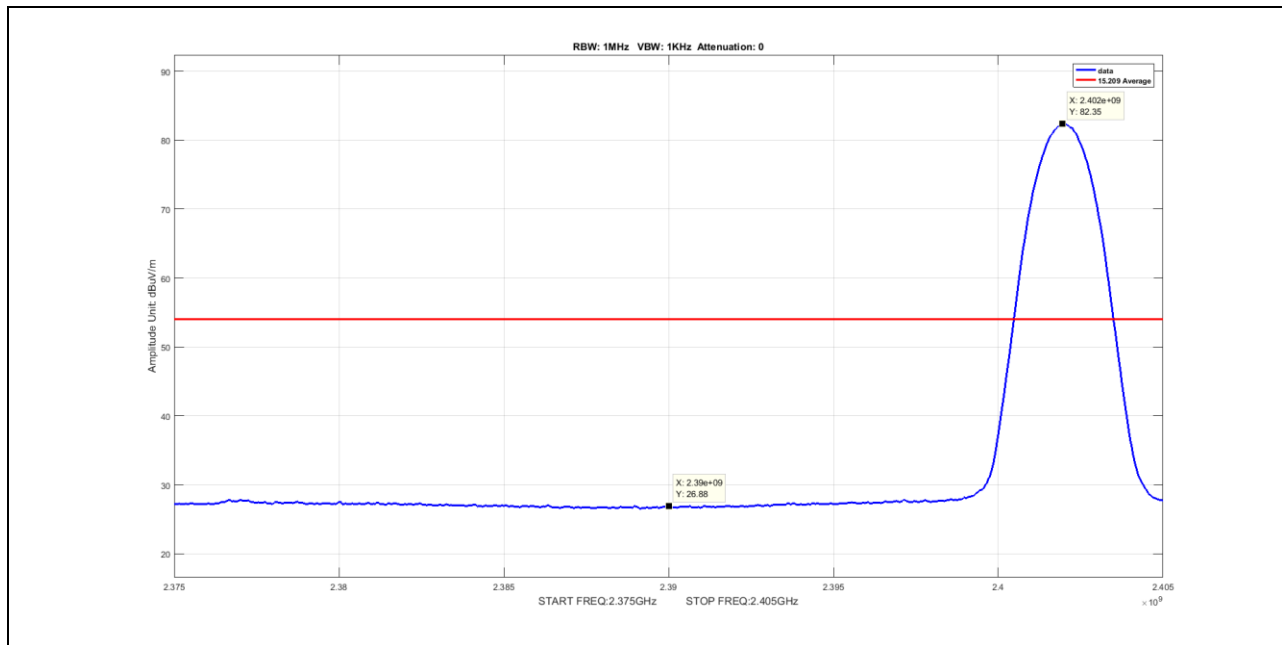
Plot 71. Radiated Restricted Band Edge, Average, 2390MHz, DH1
