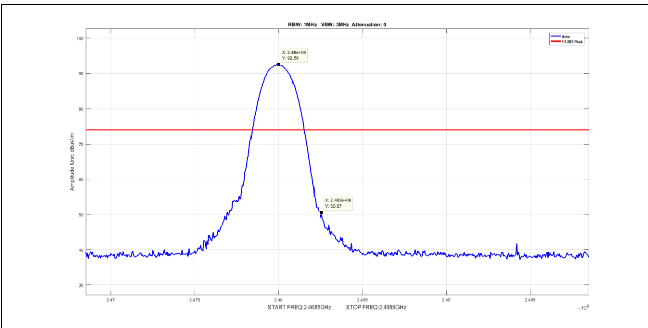
Plot 102. Radiated Restricted Band Edge, Peak, Nonhopping, 2480MHz, 3-DH5
