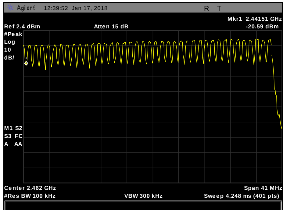
Plot 26. Number of Channels, DH5.2
