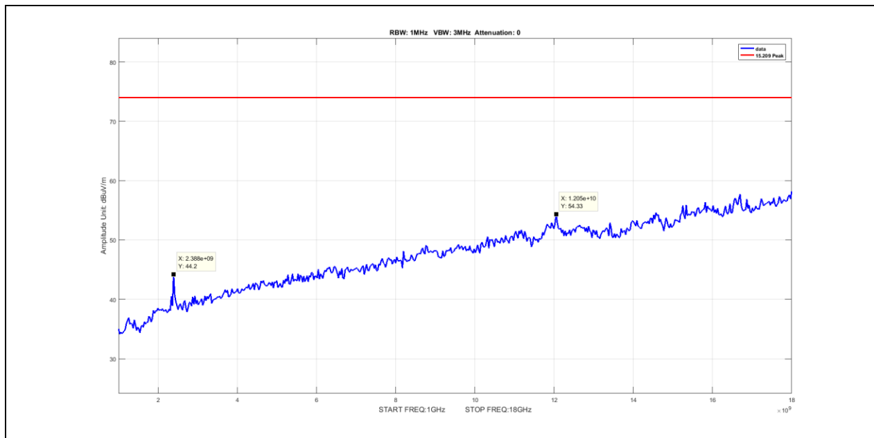
Plot 59. Radiated Spurious Emissions, Peak, Nonhopping, 1G – 18G, DH1, 2402MHz
