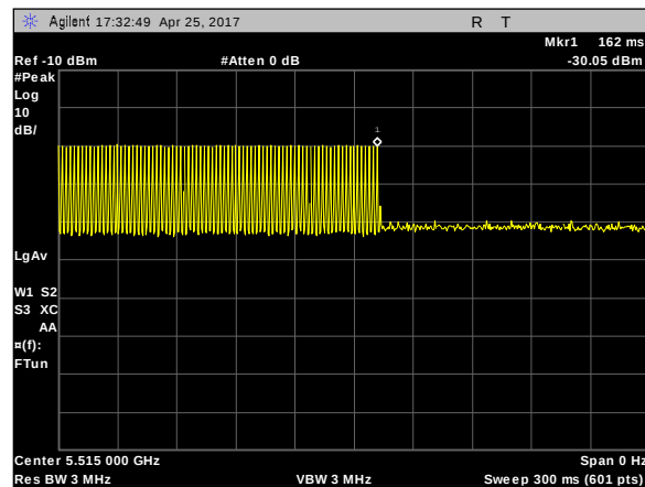
Plot 33. Channel Close Time, 5515MHz, BW 50MHz, 300ms
