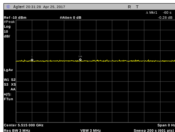
Plot 31. Radar Burst at the End of CACT, 5515MHz, BW 50MHz
