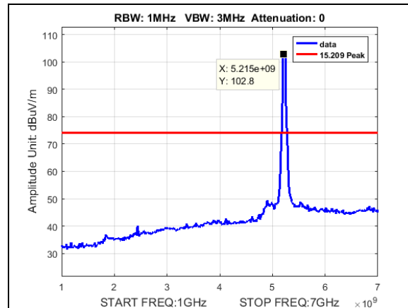
Plot 196. Undesirable Emissions, Peak radiated spurious BW 50M, CF 5225M, 19dB, 1-7GHz
