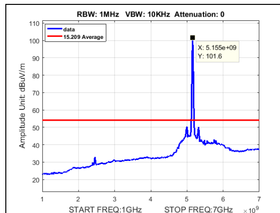
Plot 198. Undesirable Emissions, Average radiated spurious BW 10M, CF 5155M, 27dB, 1-7GHz
