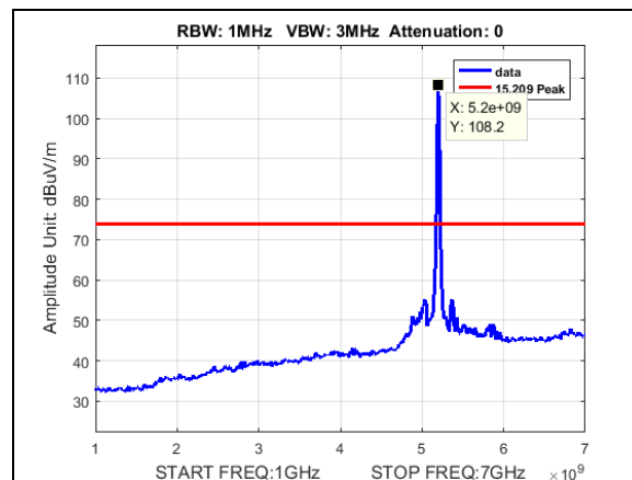
Plot 215. Undesirable Emissions, Peak radiated spurious BW 10M, CF 5200M, 27dBi, 1-7GHz
