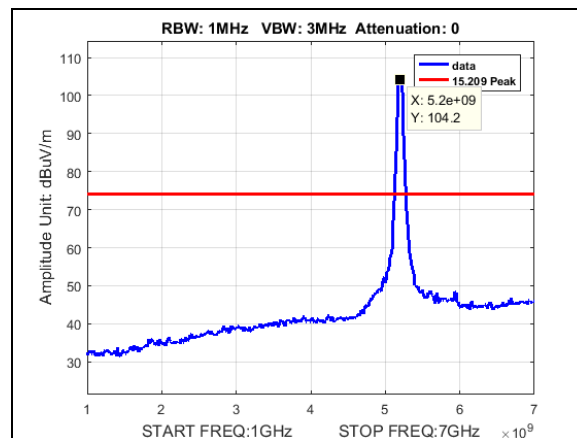
Plot 227. Undesirable Emissions, Peak radiated spurious BW 50M, CF 5200M, 27dBi, 1-7GHz
