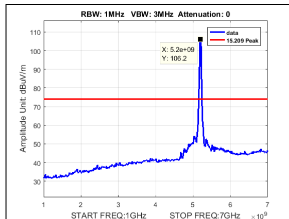
Plot 218. Undesirable Emissions, Peak radiated spurious BW 20M, CF 5200M, 27dBi, 1-7GHz
