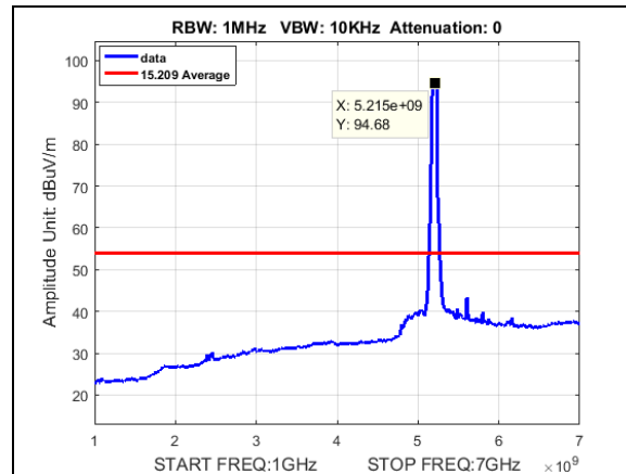
Plot 179. Undesirable Emissions, Average radiated spurious BW 50M, CF 5200M, 19dBi, 1-7GHz
