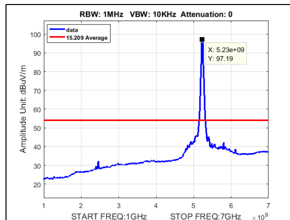
Plot 209. Undesirable Emissions, Average radiated spurious BW 40M, CF 5230M, 27dBi, 1-7GHz
