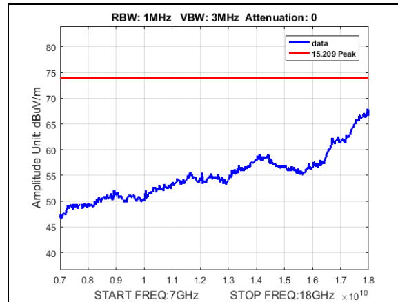
Plot 229. Undesirable Emissions, Peak radiated spurious worst case 27dBi, 7-18GHz
