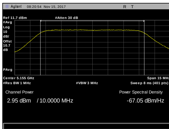
Plot 16. Conducted Transmitter Output Power, BW 10M, CF 5155M, 13dBi, c0
