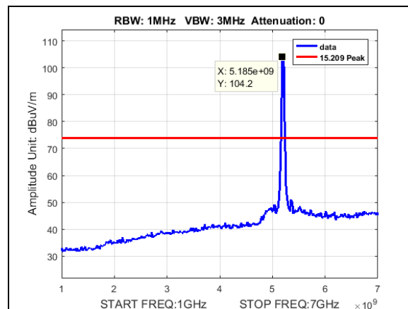
Plot 189. Undesirable Emissions, Peak radiated spurious BW 30M, CF 5200M, 19dB, 1-7GHz
