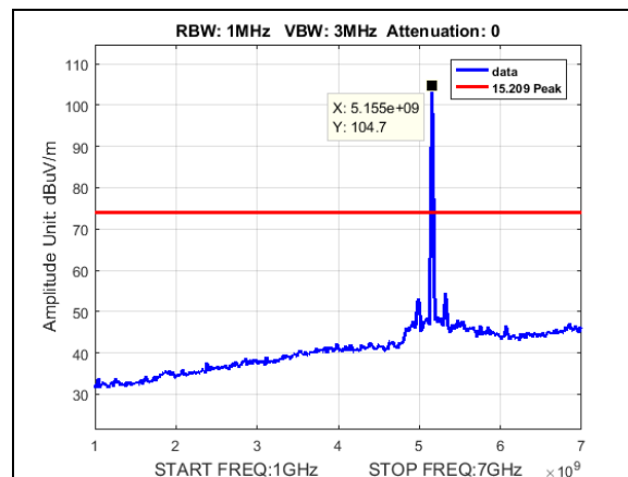
Plot 182. Undesirable Emissions, Peak radiated spurious BW 10M, CF 5155M, 19dB, 1-7GHz
