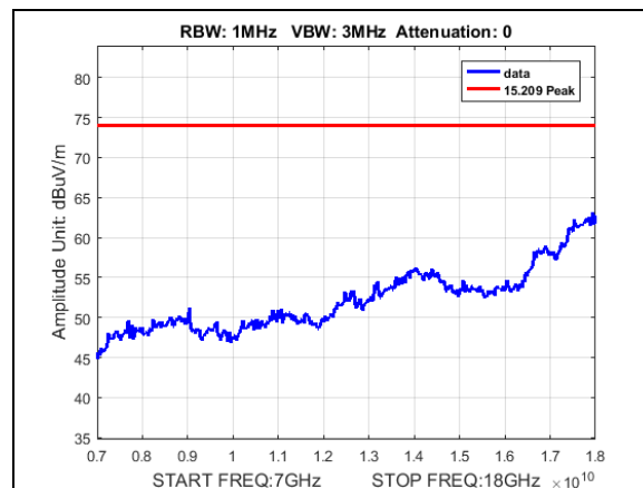
Plot 197. Undesirable Emissions, Peak radiated spurious Worst Case 19dB, 7-18GHz
