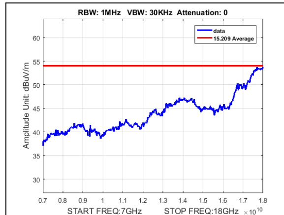
Plot 181. Undesirable Emissions, Average radiated spurious Worst Case 19dB, 7-18GHz
