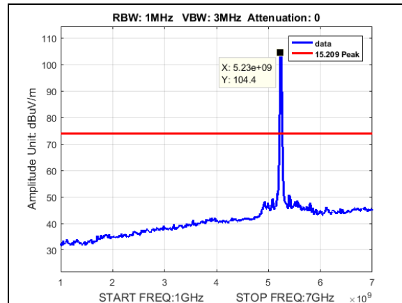
Plot 187. Undesirable Emissions, Peak radiated spurious BW 20M, CF 5240M, 19dB, 1-7GHz
