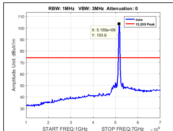
Plot 188. Undesirable Emissions, Peak radiated spurious BW 30M, CF 5165M, 19dB, 1-7GHz
