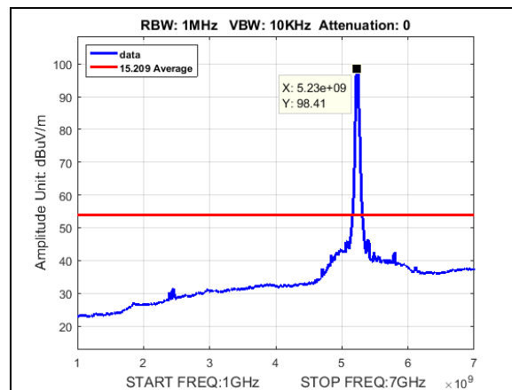
Plot 206. Undesirable Emissions, Average radiated spurious BW 30M, CF 5235M, 27dBi, 1-7GHz
