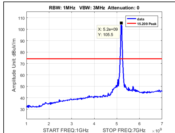
Plot 221. Undesirable Emissions, Peak radiated spurious BW 30M, CF 5200M, 27dBi, 1-7GHz
