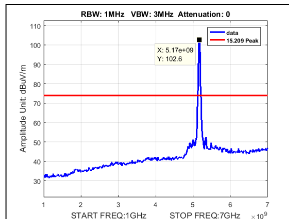
Plot 191. Undesirable Emissions, Peak radiated spurious BW 40M, CF 5170M, 19dBi, 1-7GHz
