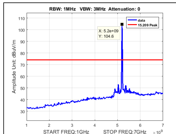
Plot 183. Undesirable Emissions, Peak radiated spurious BW 10M, CF 5200M, 19dB, 1-7GHz
