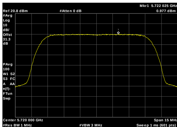
Plot 304. Power Spectral Density, UNII 2C, BW 10M, CF 5720M, c0, 13dBi
