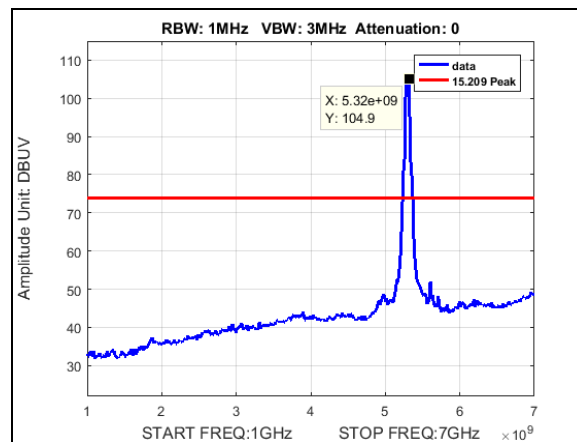
Plot 526. Radiated Spurious Emissions, Peak, BW 50M, CF 5300M, 19dB i
