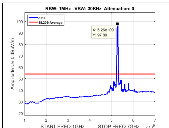
Plot 534. Radiated Spurious Emissions, Average, BW 30M, CF 5265M, 27dBi, 1-7GHz
