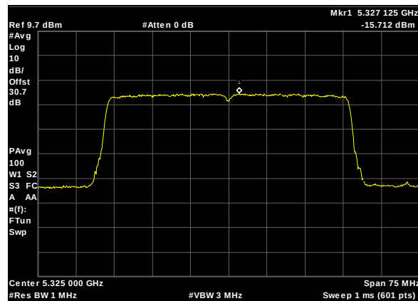
Plot 299. Power Spectral Density, UNII 2A, BW 50M, CF 5325M, c0, 27dBi
