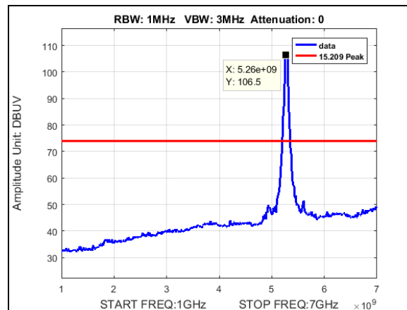
Plot 525. Radiated Spurious Emissions, Peak, BW 50M, CF 5275M, 19dB i
