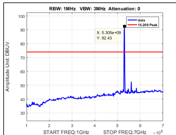
Plot 517. Radiated Spurious Emissions, Peak, BW 20M, CF 5300M, 19dBi
