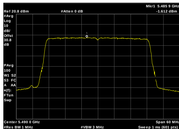
Plot 319. Power Spectral Density, UNII 2C, BW 40M, CF 5490M, c1, 13dBi
