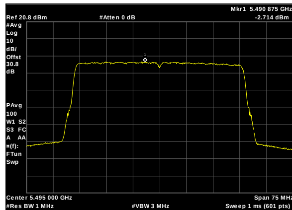
Plot 325. Power Spectral Density, UNII 2C, BW 50M, CF 5495M, c1, 13dBi
