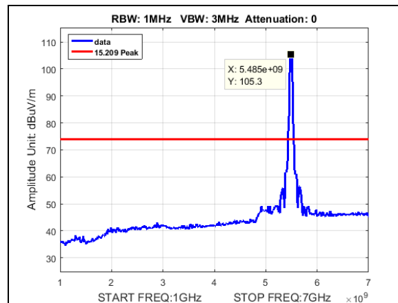
Plot 585. Radiated Spurious Emissions, Peak, BW 40M, CF 5490M, 19dBi
