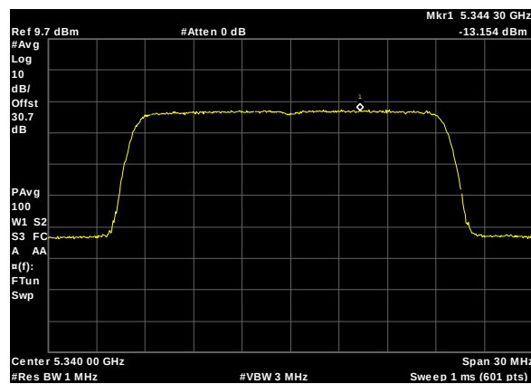
Plot 282. Power Spectral Density, UNII 2A, BW 20M, CF 5340M, c1, 27dBi
