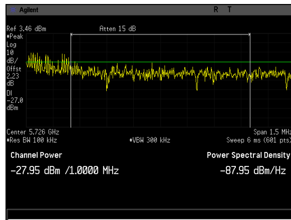
Plot 490. Undesirable Emissions, -27dBm, Radiated Bandedge 5725M, BW 10M, CF 5720M, 27dBi
