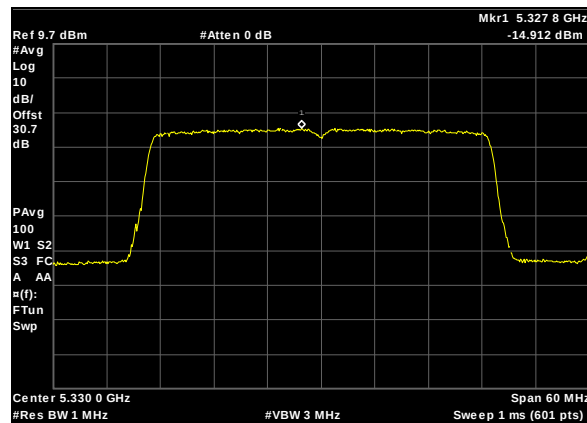
Plot 293. Power Spectral Density, UNII 2A, BW 40M, CF 5330M, c0, 27dBi
