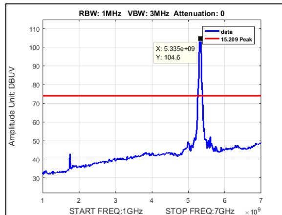
Plot 527. Radiated Spurious Emissions, Peak, BW 50M, CF 5325M, 19dB i
