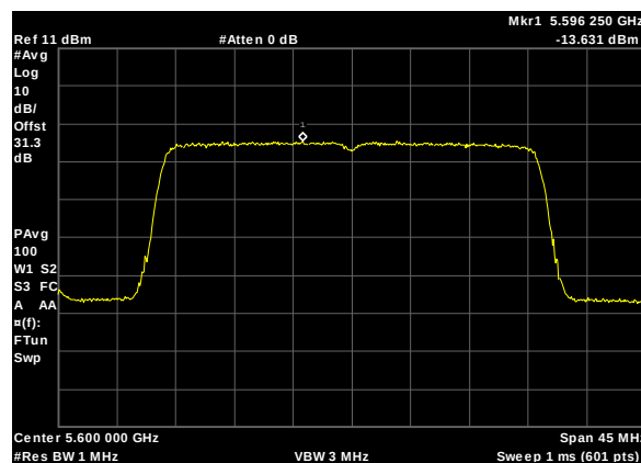
Plot 374. Power Spectral Density, UNII 2C, BW 30W, CF 5600M, c0, 27dBi
