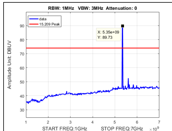
Plot 518. Radiated Spurious Emissions, Peak, BW 20M, CF 5340M, 19dBi
