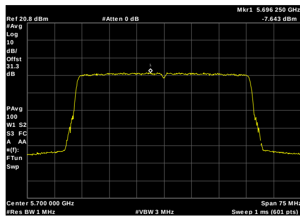
Plot 359. Power Spectral Density, UNII 2C, BW 50M, CF 5700M, c1, 19dBi
