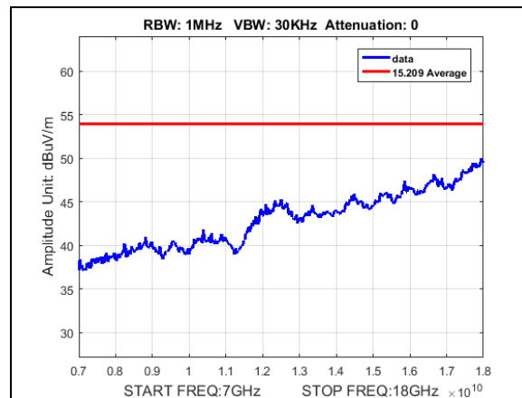
Plot 543. Radiated Spurious Emissions, Average, Worst Case, 27dBi, 7-18GHz
