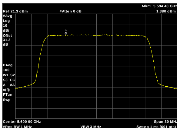
Plot 309. Power Spectral Density, UNII 2C, BW 20M, CF 5600M, c1, 13dBi
