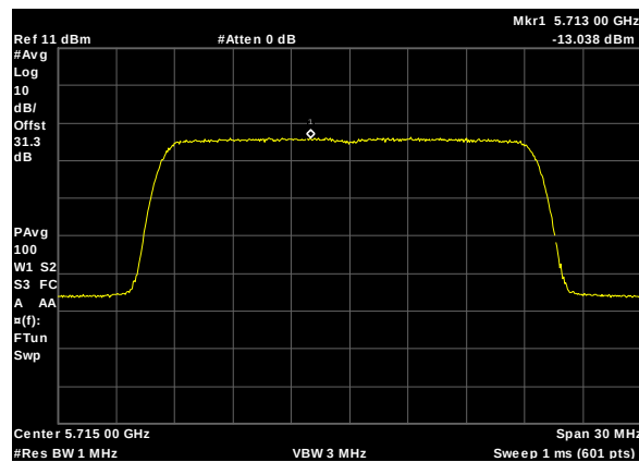
Plot 371. Power Spectral Density, UNII 2C, BW 20W, CF 5715M, c1, 27dBi
