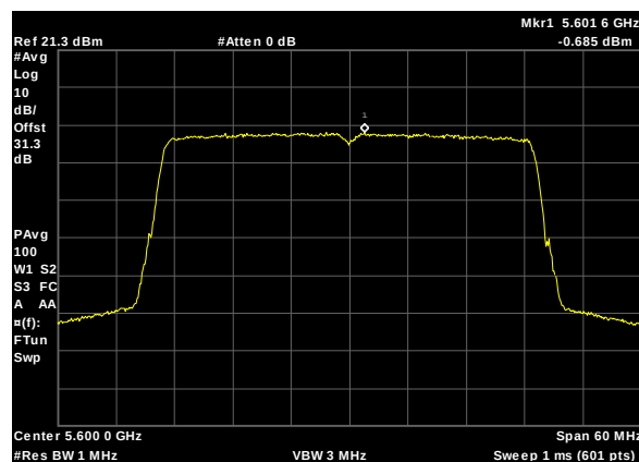
Plot 320. Power Spectral Density, UNII 2C, BW 40M, CF 5600M, c0, 13dBi
