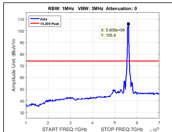
Plot 586. Radiated Spurious Emissions, Peak, BW 40M, CF 5600M, 19dBi
