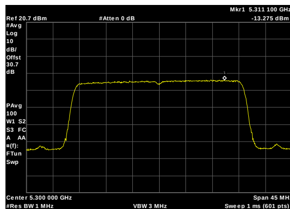
Plot 285. Power Spectral Density, UNII 2A, BW 30M, CF 5300M, c0, 27dBi
