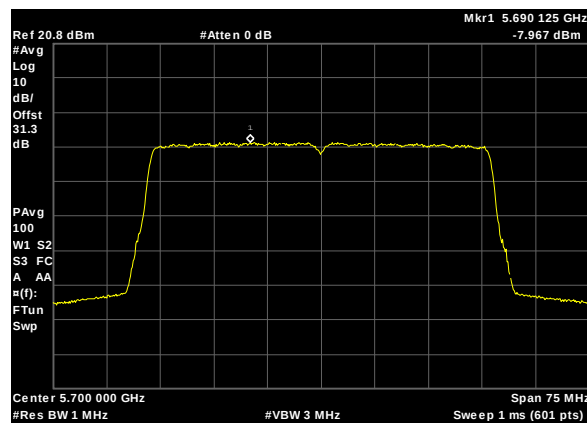
Plot 358. Power Spectral Density, UNII 2C, BW 50M, CF 5700M, c0, 19dBi
