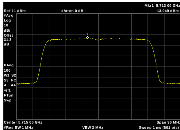
Plot 370. Power Spectral Density, UNII 2C, BW 20W, CF 5715M, c0, 27dBi
