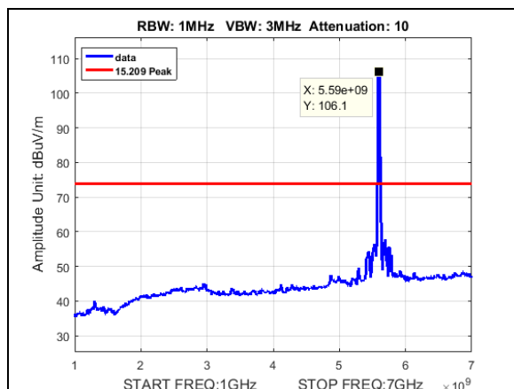
Plot 612. Radiated Spurious Emissions, Peak, BW 20M, CF 5600M, 27dBi
