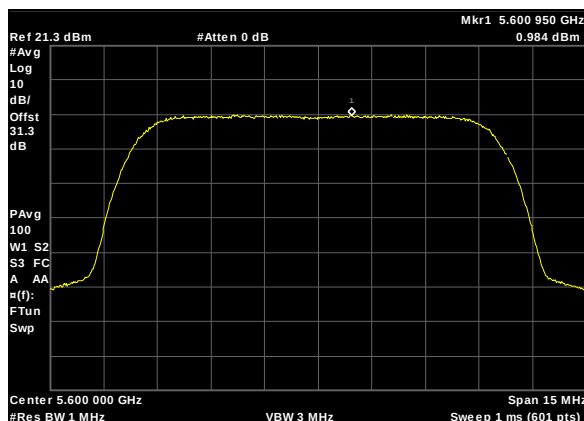
Plot 303. Power Spectral Density, UNII 2C, BW 10M, CF 5600M, c1, 13dBi
