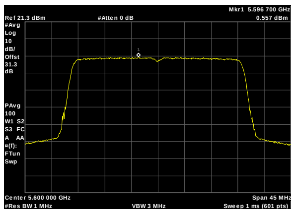
Plot 314. Power Spectral Density, UNII 2C, BW 30M, CF 5600M, c0, 13dBi
