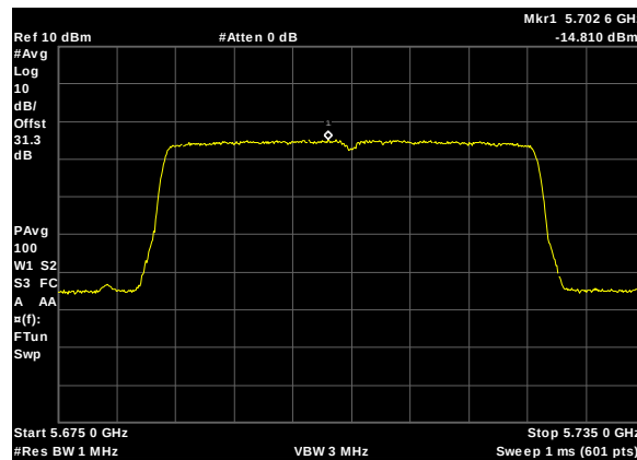
Plot 382. Power Spectral Density, UNII 2C, BW 40W, CF 5705M, c1, 27dBi
