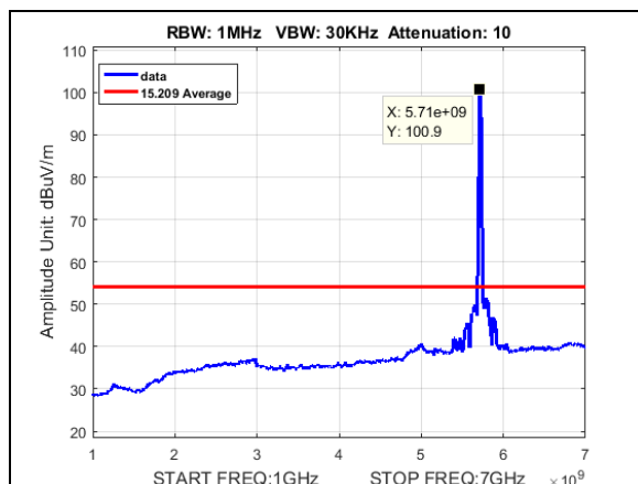
Plot 597. Radiated Spurious Emissions, Average, BW 20M, CF 5715M, 27dBi
