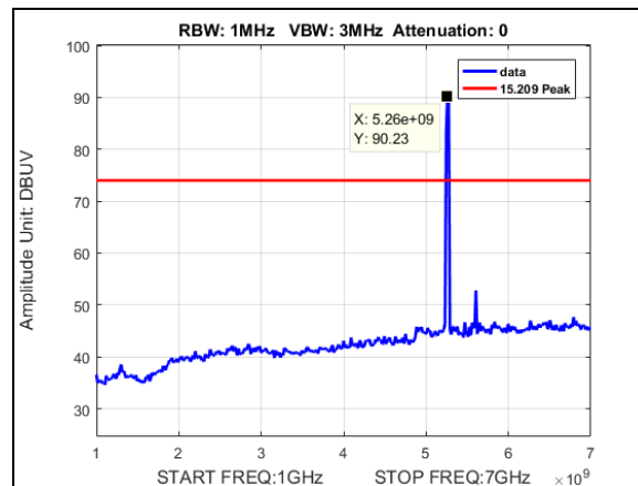
Plot 516. Radiated Spurious Emissions, Peak, BW 20M, CF 5260M, 19dBi
