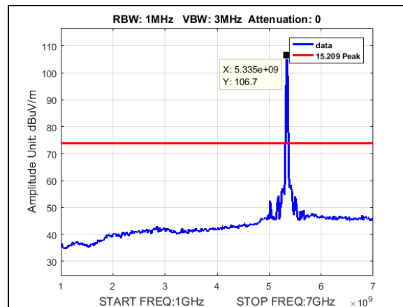
Plot 549. Radiated Spurious Emissions, Peak, BW 20M, CF 5340M, 27dB, 1-7GHz
