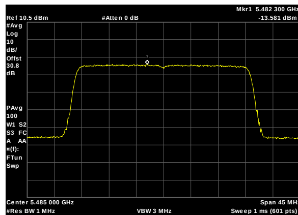
Plot 373. Power Spectral Density, UNII 2C, BW 30W, CF 5485M, c1, 27dBi
