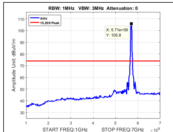
Plot 587. Radiated Spurious Emissions, Peak, BW 40M, CF 5705M, 19dBi
