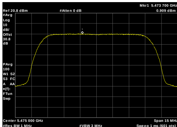
Plot 300. Power Spectral Density, UNII 2C, BW 10M, CF 5475M, c0, 13dBi
