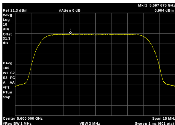
Plot 302. Power Spectral Density, UNII 2C, BW 10M, CF 5600M, c0, 13dBi
