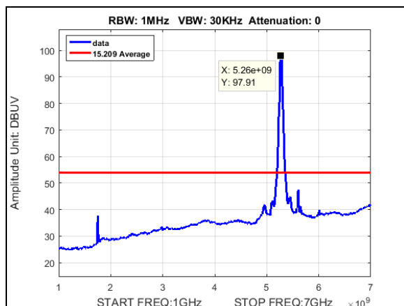
Plot 507. Radiated Spurious Emissions, Average, BW 40M, CF 5270M, 19dBi
