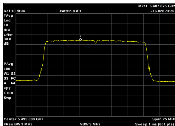
Plot 385. Power Spectral Density, UNII 2C, BW 50W, CF 5495M, c1, 27dBi
