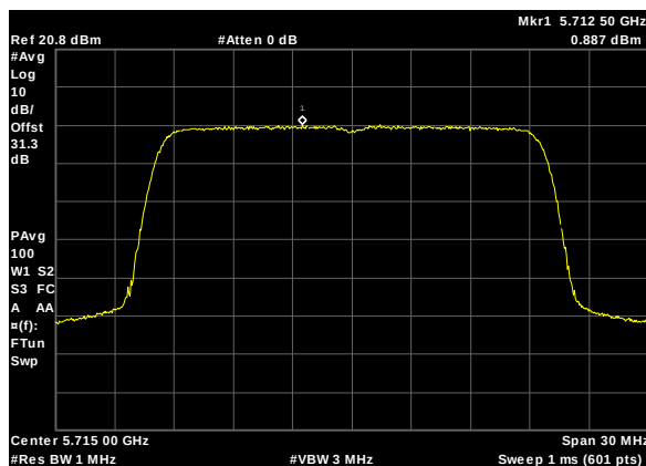
Plot 310. Power Spectral Density, UNII 2C, BW 20M, CF 5715M, c0, 13dBi
