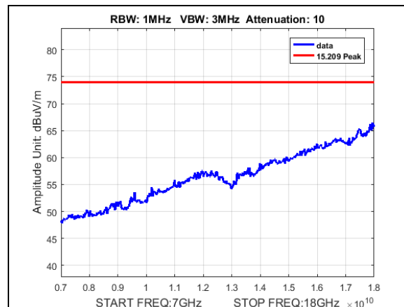
Plot 623. Radiated Spurious Emissions, Peak, worst case, 7-18GHz, 27dBi
