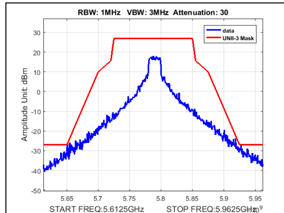
Plot 180. Undesirable Emissions, UNII3, emission mask, BW 20M, CF 5790M, 19dBi
