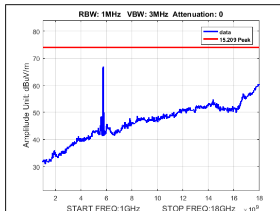
Plot 161. Undesirable Emissions, Peak, radiated spurious emissions, 40M, 5745, 1-18GHz
