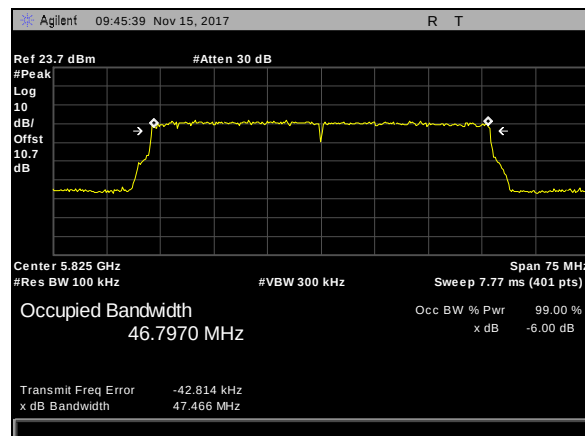
Plot 228. 6 dB Occupied Bandwidth, BW 50M, CF 5825M
