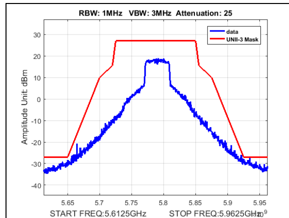
Plot 199. Undesirable Emissions, UNII3, emission mask, BW 40M, CF 5790M, 27dBi
