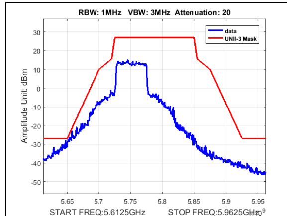
Plot 204. Undesirable Emissions, UNII3, emission mask, BW 50M, CF 5750M, 19dBm
