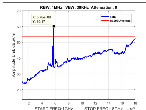
Plot 146. Undesirable Emissions, Average, radiated spurious emissions, 40M, 5745, 1-18GHz
