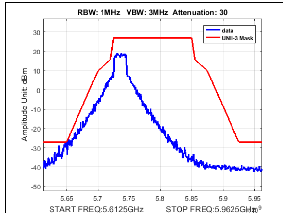
Plot 177. Undesirable Emissions, UNII3, emission mask, BW 20M, CF 5735M, 19dBi
