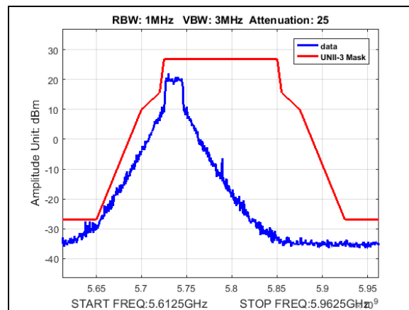
Plot 178. Undesirable Emissions, UNII3, emission mask, BW 20M, CF 5735M, 27dBi
