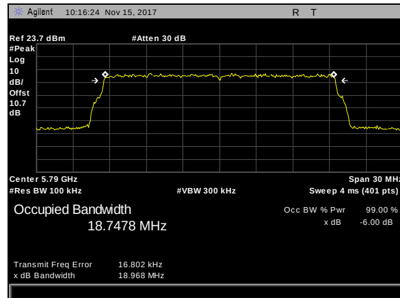
Plot 218. 6 dB Occupied Bandwidth, BW 20M, CF 5790M
