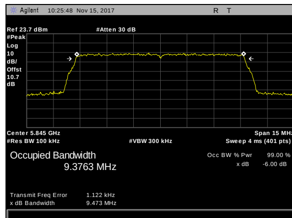
Plot 216. 6 dB Occupied Bandwidth, BW 10M, CF 5845M
