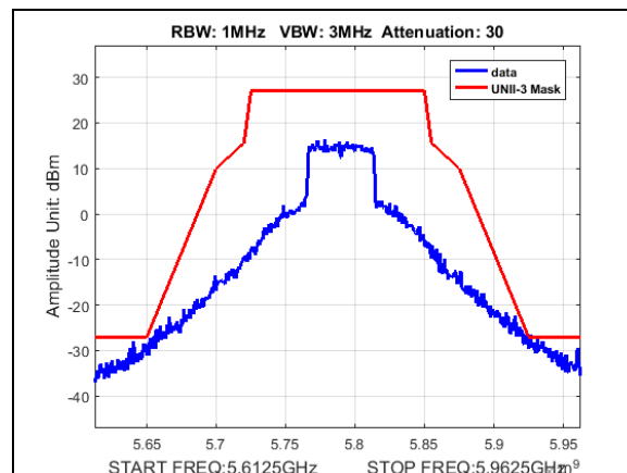
Plot 206. Undesirable Emissions, UNII3, emission mask, BW 50M, CF 5790M, 13dBm
