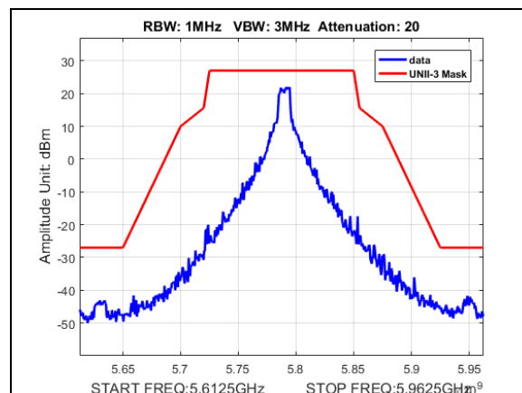
Plot 170. Undesirable Emissions, UNII3, emission mask, BW 10M, CF 5790M, 13dBi
