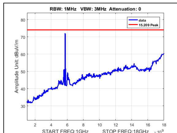
Plot 158. Undesirable Emissions, Peak, radiated spurious emissions, 30M, 5740, 1-18GHz
