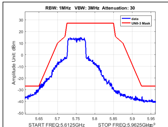
Plot 203. Undesirable Emissions, UNII3, emission mask, BW 50M, CF 5750M, 13dBi
