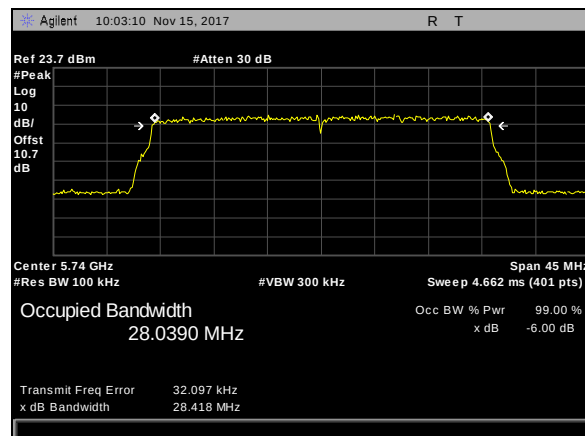
Plot 220. 6 dB Occupied Bandwidth, BW 30M, CF 5740M
