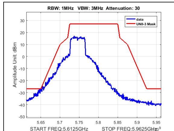
Plot 194. Undesirable Emissions, UNII3, emission mask, BW 40M, CF 5745M, 13dBi
