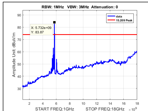
Plot 152. Undesirable Emissions, Peak, radiated spurious emissions, 10M, 5730, 1-18GHz
