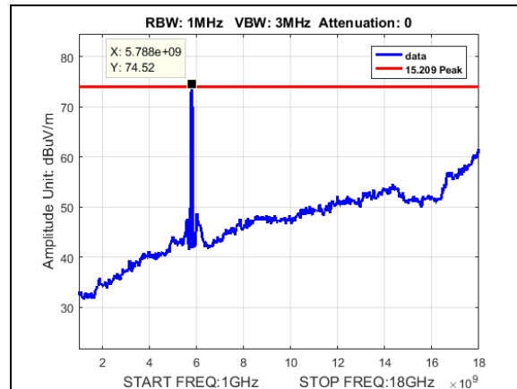
Plot 162. Undesirable Emissions, Peak, radiated spurious emissions, 40M, 5790, 1-18GHz
