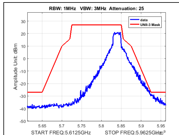
Plot 184. Undesirable Emissions, UNII3, emission mask, BW 20M, CF 5840M, 27dBi
