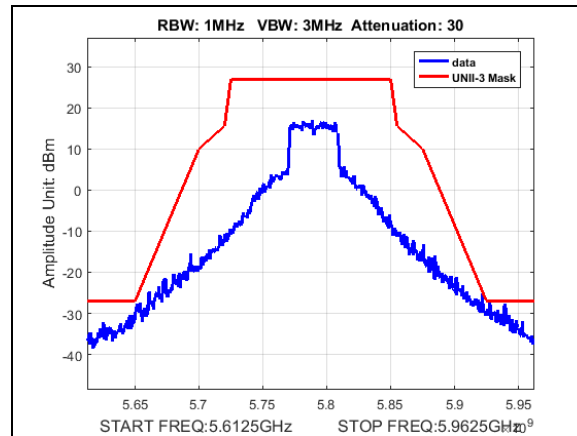
Plot 198. Undesirable Emissions, UNII3, emission mask, BW 40M, CF 5790M, 19dBi
