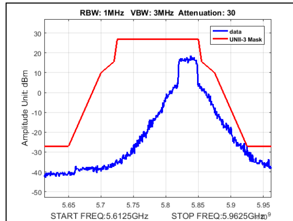
Plot 192. Undesirable Emissions, UNII3, emission mask, BW 30M, CF 5835M, 19dBi
