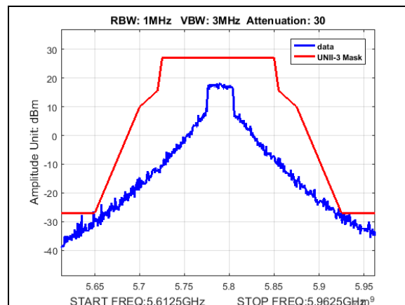
Plot 188. Undesirable Emissions, UNII3, emission mask, BW 30M, CF 5790M, 13dBi
