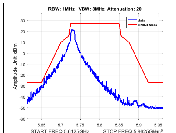
Plot 167. Undesirable Emissions, UNII3, emission mask, BW 10M, CF 5730M, 13dB
