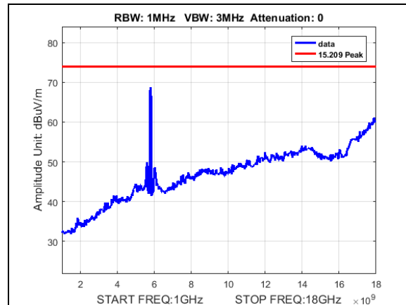
Plot 165. Undesirable Emissions, Peak, radiated spurious emissions, 50M, 5790, 1-18GHz
