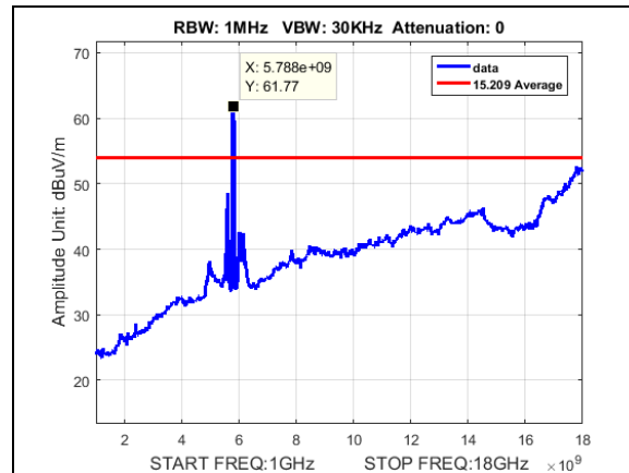
Plot 150. Undesirable Emissions, Average, radiated spurious emissions, 50M, 5790, 1-18GHz
