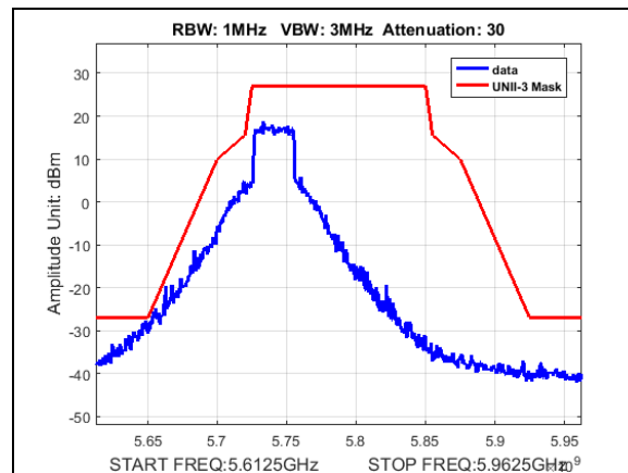
Plot 185. Undesirable Emissions, UNII3, emission mask, BW 30M, CF 5740M, 13dBi
