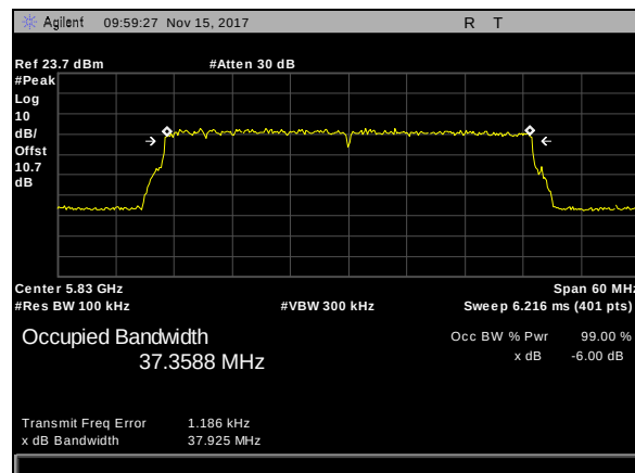
Plot 225. 6 dB Occupied Bandwidth, BW 40M, CF 5830M
