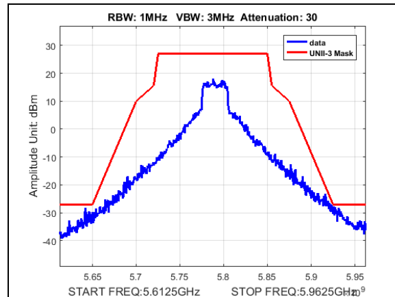
Plot 189. Undesirable Emissions, UNII3, emission mask, BW 30M, CF 5790M, 19dBi
