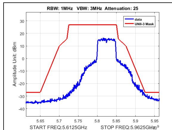
Plot 211. Undesirable Emissions, UNII3, emission mask, BW 50M, CF 5825M, 27dBm
