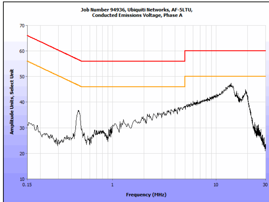
Plot 213. Conducted Emissions, Phase, no legend
