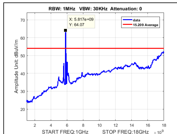
Plot 145. Undesirable Emissions, Average, radiated spurious emissions, 30M, 5835, 1-18GHz
