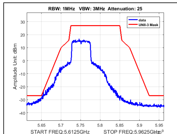
Plot 205. Undesirable Emissions, UNII3, emission mask, BW 50M, CF 5750M, 27dBm
