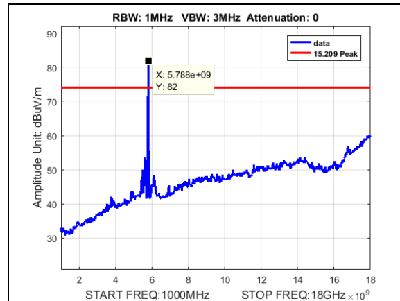
Plot 153. Undesirable Emissions, Peak, radiated spurious emissions, 10M, 5790, 1-18GHz
