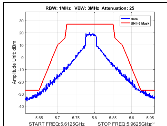
Plot 190. Undesirable Emissions, UNII3, emission mask, BW 30M, CF 5790M, 27dBi
