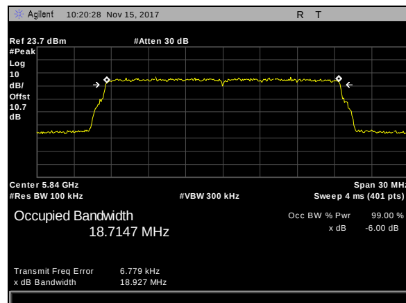
Plot 219. 6 dB Occupied Bandwidth, BW 20M, CF 5840M
