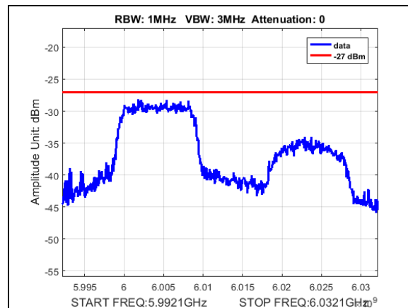
Plot 140. Undesirable Emissions, Average, radiated spurious emissions, 10M, 5845, 6015M spur
