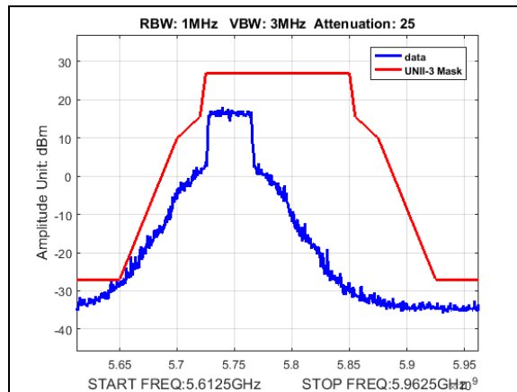
Plot 196. Undesirable Emissions, UNII3, emission mask, BW 40M, CF 5745M, 27dBm
