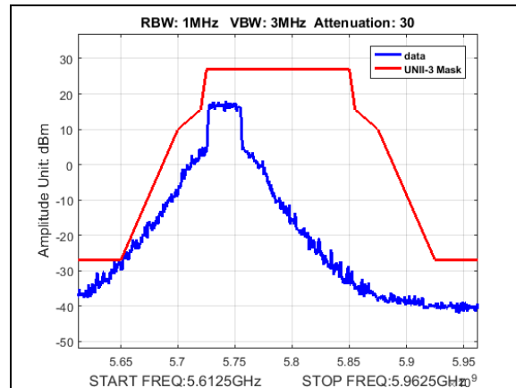
Plot 186. Undesirable Emissions, UNII3, emission mask, BW 30M, CF 5740M, 19dBi
