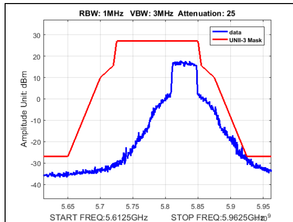
Plot 202. Undesirable Emissions, UNII3, emission mask, BW 40M, CF 5830M, 27dBi
