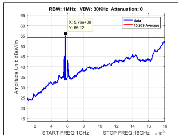
Plot 149. Undesirable Emissions, Average, radiated spurious emissions, 50M, 5750, 1-18GHz
