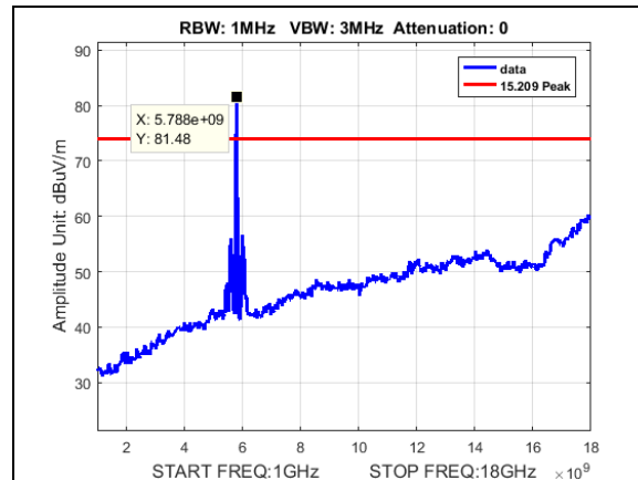
Plot 156. Undesirable Emissions, Peak, radiated spurious emissions, 20M, 5790, 1-18GHz
