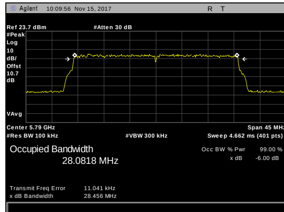
Plot 221. 6 dB Occupied Bandwidth, BW 30M, CF 5790M
