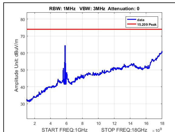
Plot 166. Undesirable Emissions, Peak, radiated spurious emissions, 50M, 5825, 1-18GHz
