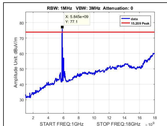
Plot 157. Undesirable Emissions, Peak, radiated spurious emissions, 20M, 5840, 1-18GHz
