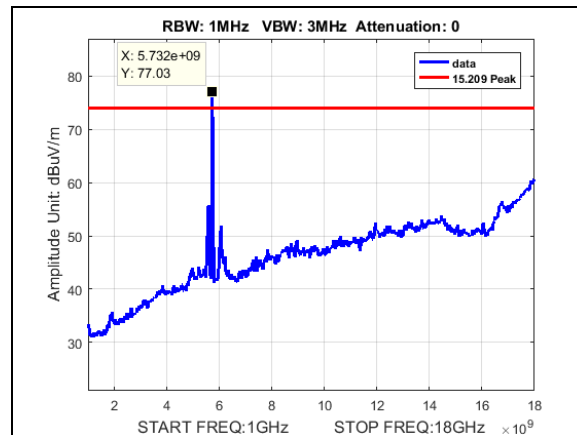
Plot 155. Undesirable Emissions, Peak, radiated spurious emissions, 20M, 5735, 1-18GHz
