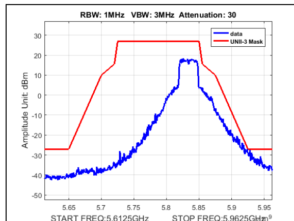
Plot 191. Undesirable Emissions, UNII3, emission mask, BW 30M, CF 5835M, 13dBi
