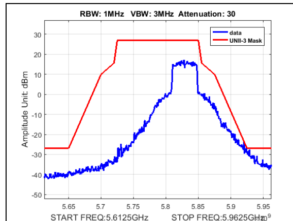
Plot 200. Undesirable Emissions, UNII3, emission mask, BW 40M, CF 5830M, 13dBi
