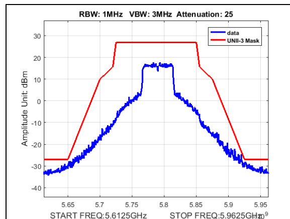
Plot 208. Undesirable Emissions, UNII3, emission mask, BW 50M, CF 5790M, 27dBi
