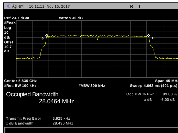
Plot 222. 6 dB Occupied Bandwidth, BW 30M, CF 5835M
