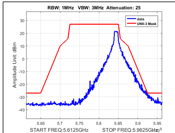
Plot 175. Undesirable Emissions, UNII3, emission mask, BW 10M, CF 5845M, 27dBi
