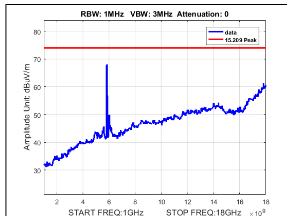
Plot 163. Undesirable Emissions, Peak, radiated spurious emissions, 40M, 5830, 1-18GHz
