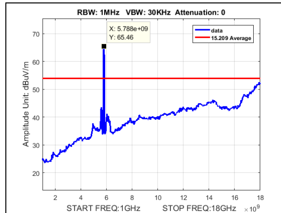
Plot 147. Undesirable Emissions, Average, radiated spurious emissions, 40M, 5790, 1-18GHz
