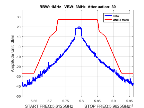
Plot 179. Undesirable Emissions, UNII3, emission mask, BW 20M, CF 5790M, 13dBi
