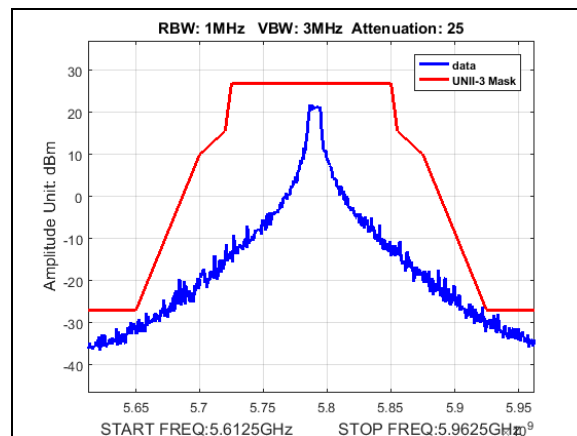
Plot 172. Undesirable Emissions, UNII3, emission mask, BW 10M, CF 5790M, 27dBi
