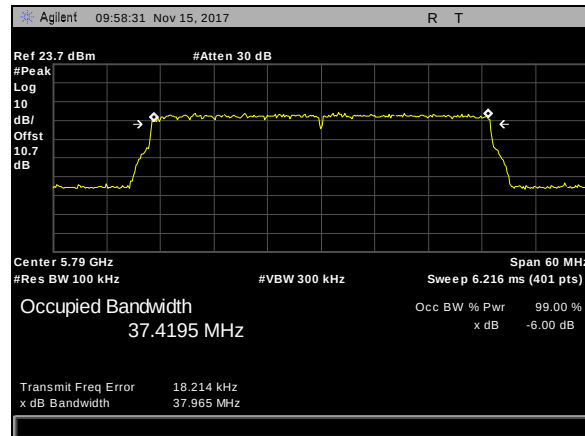
Plot 224. 6 dB Occupied Bandwidth, BW 40M, CF 5790M
