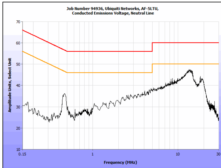
Plot 212. Conducted Emissions, Neutral, no legend
