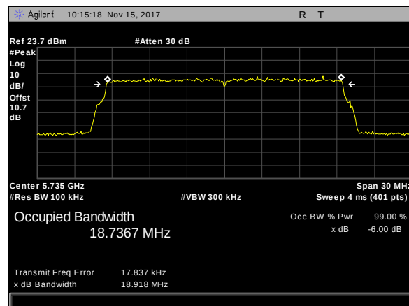
Plot 217. 6 dB Occupied Bandwidth, BW 20M, CF 5735M
