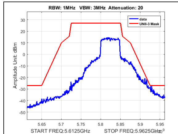
Plot 210. Undesirable Emissions, UNII3, emission mask, BW 50M, CF 5825M, 19dBm
