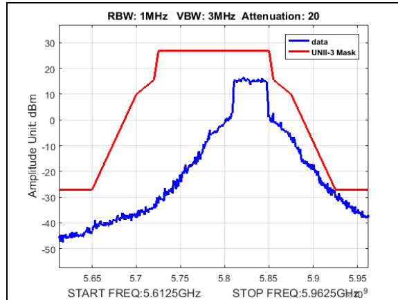
Plot 201. Undesirable Emissions, UNII3, emission mask, BW 40M, CF 5830M, 19dBi
