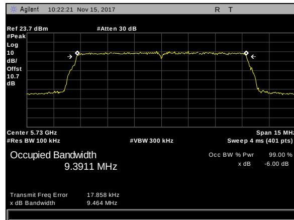
Plot 214. 6 dB Occupied Bandwidth, BW 10M, CF 5730M
