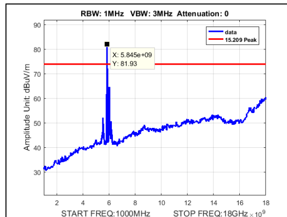
Plot 154. Undesirable Emissions, Peak, radiated spurious emissions, 10M, 5845, 1-18GHz
