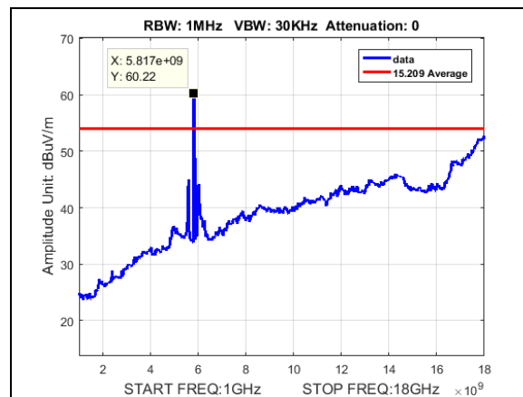
Plot 148. Undesirable Emissions, Average, radiated spurious emissions, 40M, 5830, 1-18GHz
