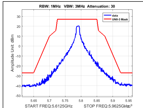
Plot 171. Undesirable Emissions, UNII3, emission mask, BW 10M, CF 5790M, 19dBi
