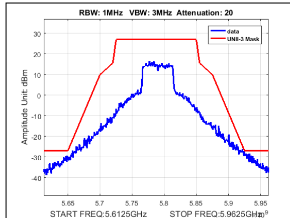
Plot 207. Undesirable Emissions, UNII3, emission mask, BW 50M, CF 5790M, 19dBi
