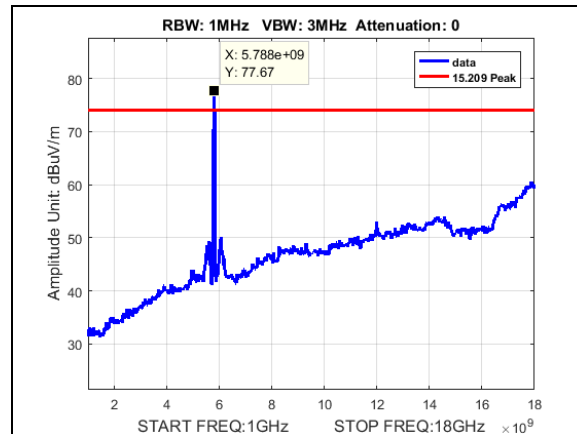
Plot 159. Undesirable Emissions, Peak, radiated spurious emissions, 30M, 5790, 1-18GHz
