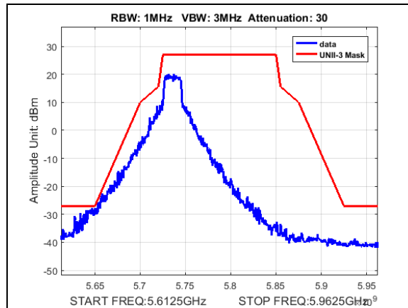
Plot 176. Undesirable Emissions, UNII3, emission mask, BW 20M, CF 5735M, 13dBi
