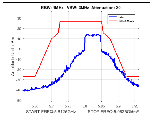
Plot 209. Undesirable Emissions, UNII3, emission mask, BW 50M, CF 5825M, 13dBi
