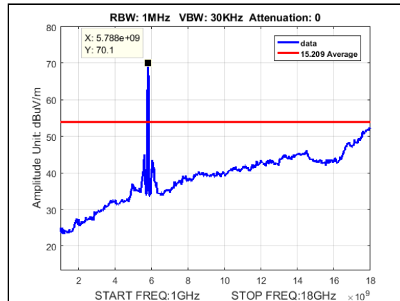
Photograph 1. Undesirable Emissions, Average, radiated spurious emissions, 30M, 5790, 1-18GHz
