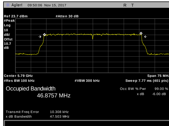
Plot 227. 6 dB Occupied Bandwidth, BW 50M, CF 5790M
