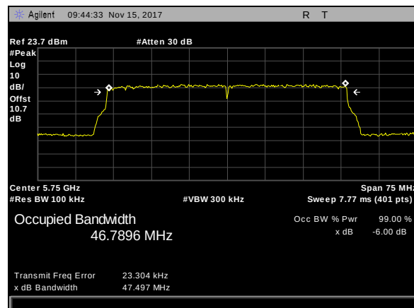
Plot 226. 6 dB Occupied Bandwidth, BW 50M, CF 5750M
