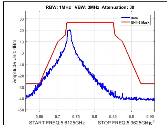
Plot 168. Undesirable Emissions, UNII3, emission mask, BW 10M, CF 5730M, 19dBi
