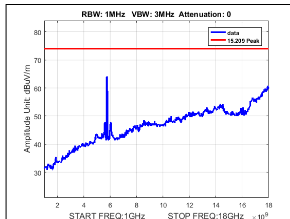
Plot 164. Undesirable Emissions, Peak, radiated spurious emissions, 50M, 5750, 1-18GHz
