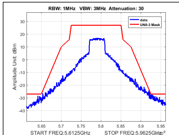
Plot 197. Undesirable Emissions, UNII3, emission mask, BW 40M, CF 5790M, 13dBm
