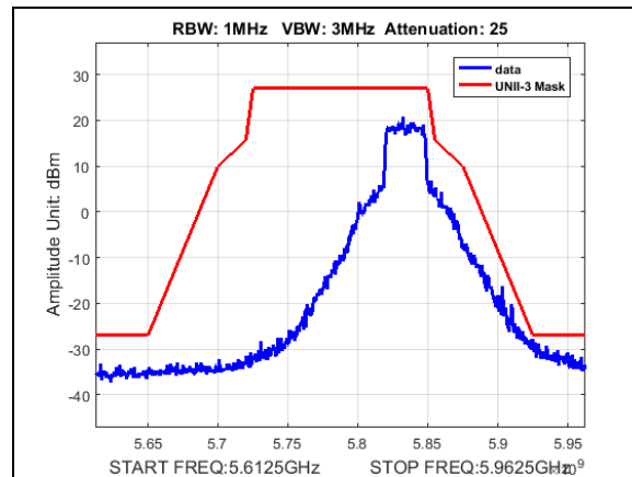
Plot 193. Undesirable Emissions, UNII3, emission mask, BW 30M, CF 5835M, 27dBi
