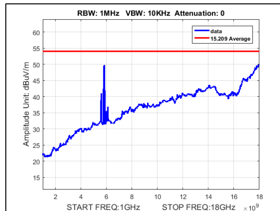
Plot 151. Undesirable Emissions, Average, radiated spurious emissions, 50M, 5825, 1-18GHz
