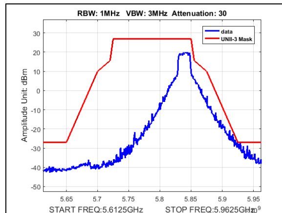
Plot 182. Undesirable Emissions, UNII3, emission mask, BW 20M, CF 5840M, 13dBi
