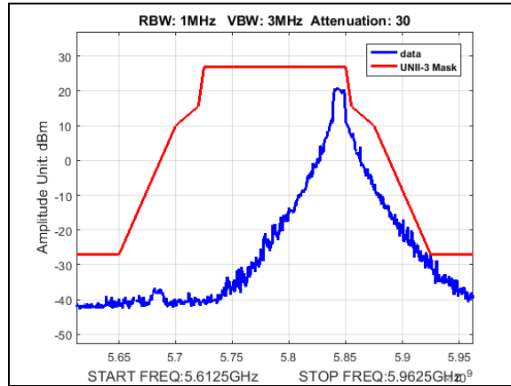
Plot 174. Undesirable Emissions, UNII3, emission mask, BW 10M, CF 5845M, 19dBi
