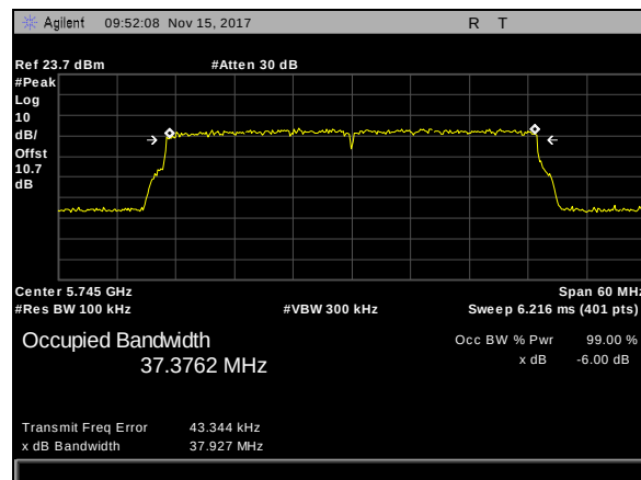
Plot 223. 6 dB Occupied Bandwidth, BW 40M, CF 5745M
