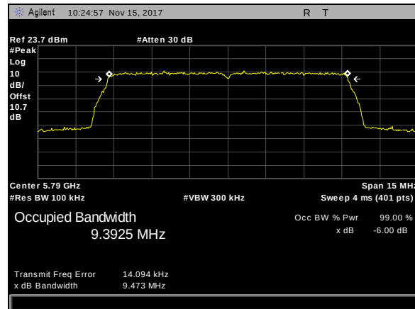
Plot 215. 6 dB Occupied Bandwidth, BW 10M, CF 5790M
