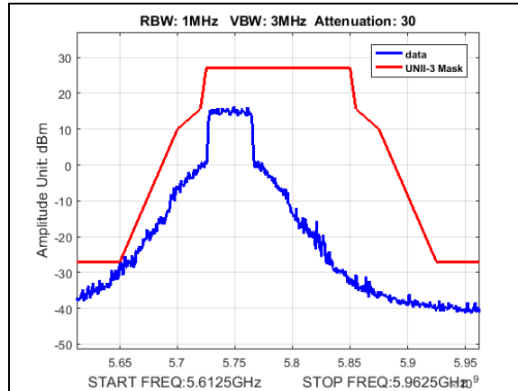
Plot 195. Undesirable Emissions, UNII3, emission mask, BW 40M, CF 5745M, 19dBm
