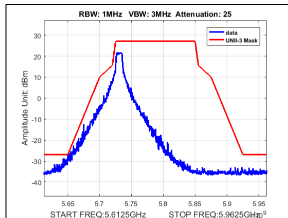
Plot 169. Undesirable Emissions, UNII3, emission mask, BW 10M, CF 5730M, 27dBi
