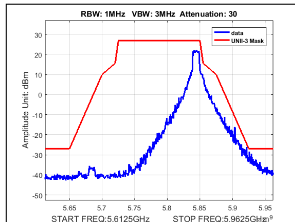
Plot 173. Undesirable Emissions, UNII3, emission mask, BW 10M, CF 5845M, 13dBi
