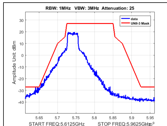
Plot 187. Undesirable Emissions, UNII3, emission mask, BW 30M, CF 5740M, 27dBi
