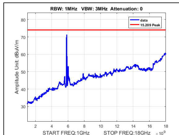
Plot 160. Undesirable Emissions, Peak, radiated spurious emissions, 30M, 5835, 1-18GHz
