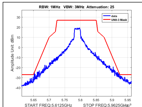
Plot 181. Undesirable Emissions, UNII3, emission mask, BW 20M, CF 5790M, 27dBi
