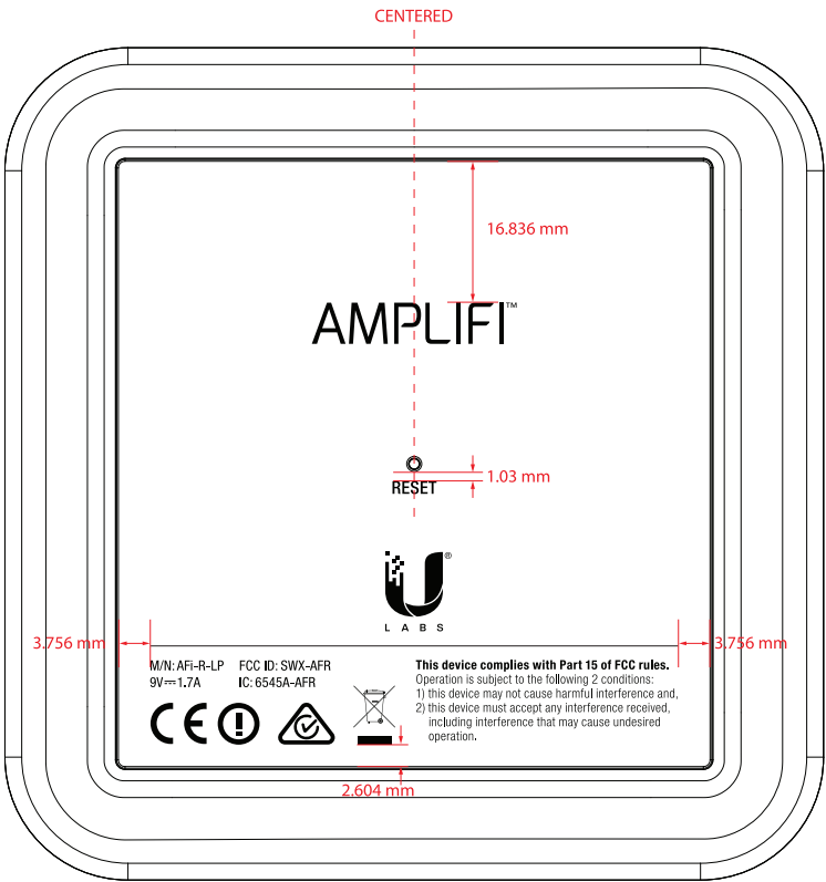
Bottom View
