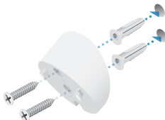
Angle Mount
