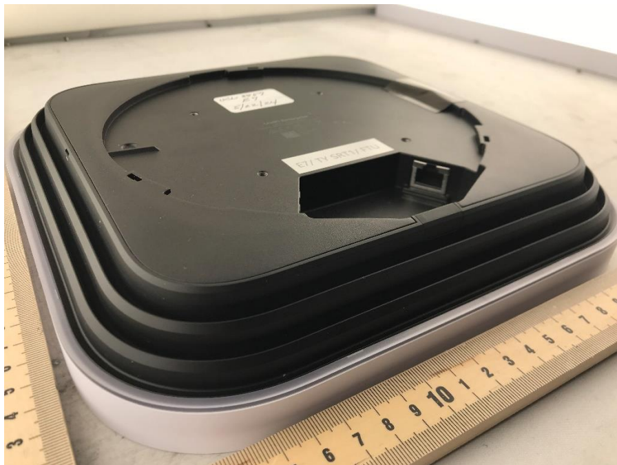
Photograph 9: POE In 10 G Port Connector
