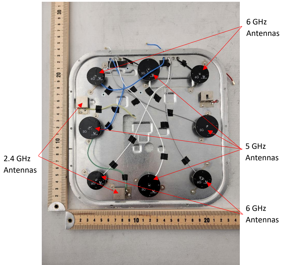
Photograph 3: Front Antenna Board
