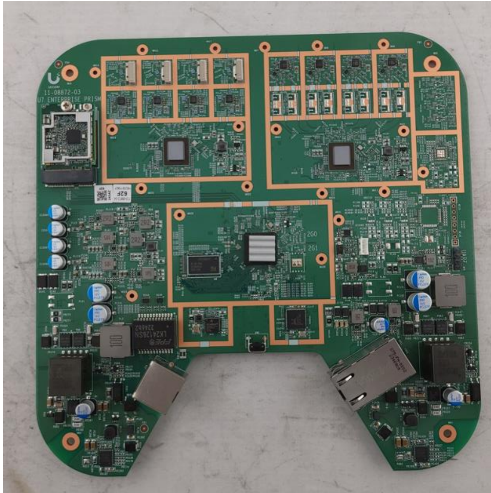
Photograph 6: Top Side Of PCB
