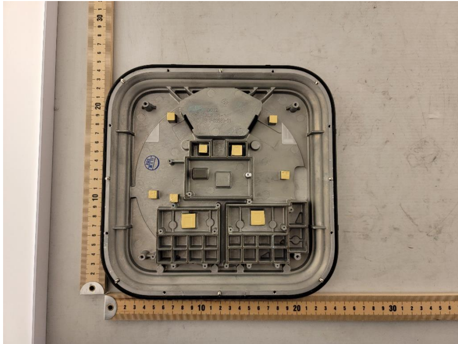
Photograph 5: Internal Back of DUT
