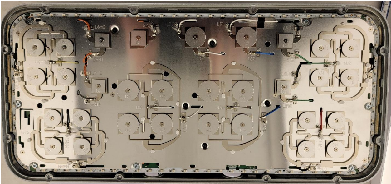
Photograph 6: Antenna Assembly
