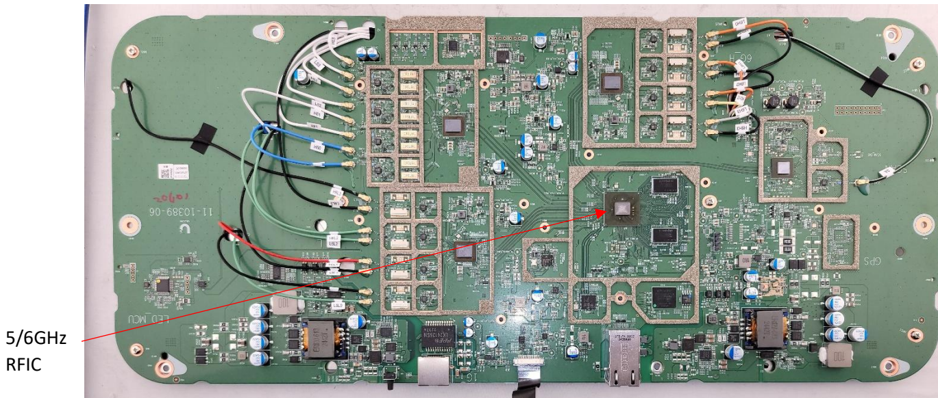
Photograph 3: Internal View of Main PCB 1
