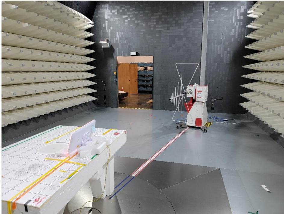
Photograph 1: View Test Set Up Radiated Emissions 30 – 1000 MHz
