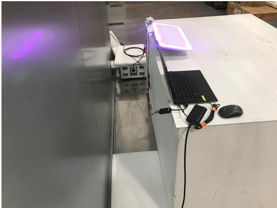
Photograph 7: View Test Set Up Back Conducted Emissions
