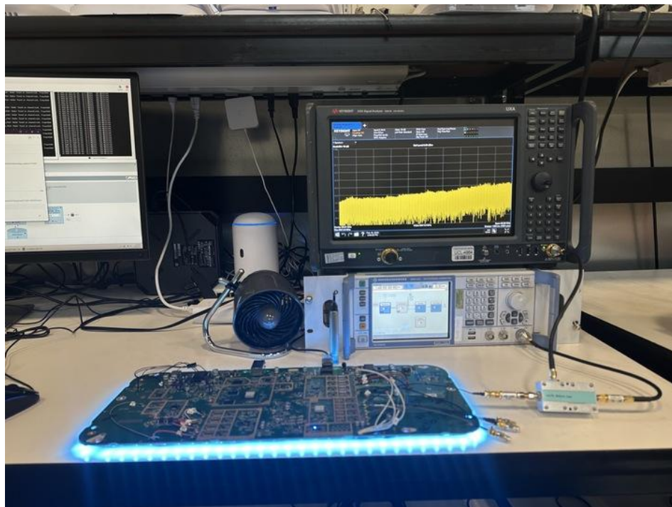
Photograph 8: View Test Set Up DFS
