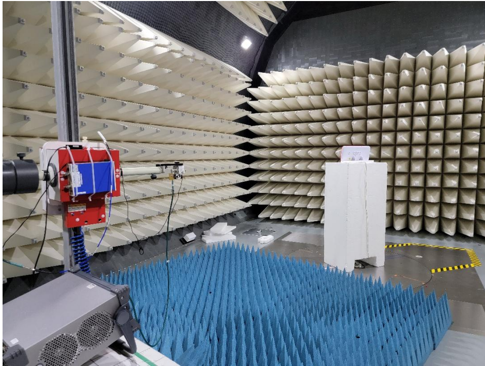
Photograph 3: View Test Set Up Radiated Emissions 17 – 40 GHz
