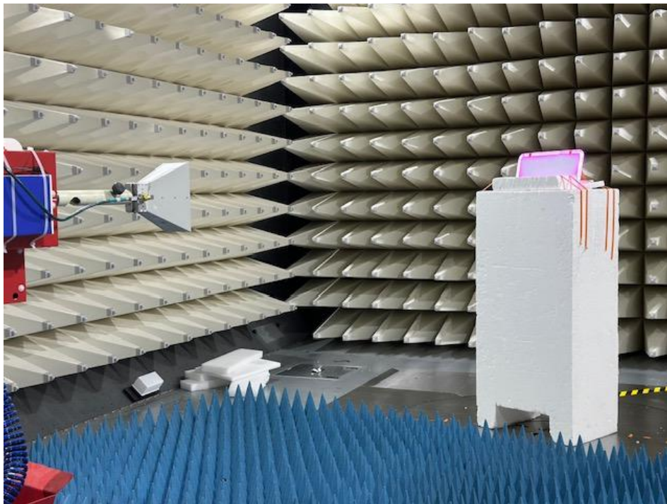
Photograph 2: View Test Set Up Radiated Emissions 1 – 17 GHz
