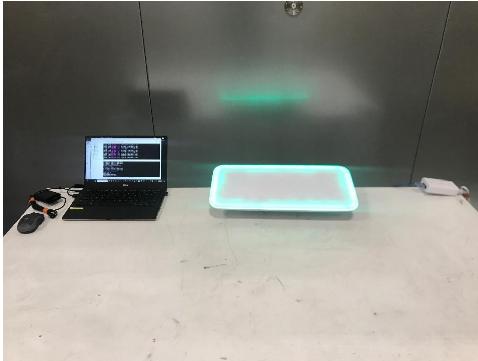
Photograph 6: View Test Set Up Front Conducted Emissions
