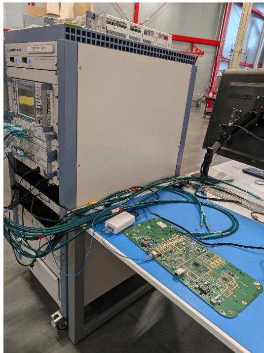
Photograph 4: View Test Set Up RF Conducted
