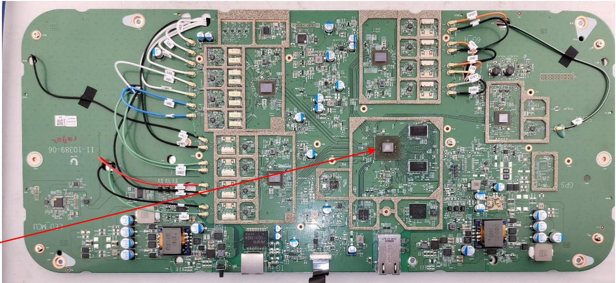
Photograph 3: Internal View of Main PCB Top
