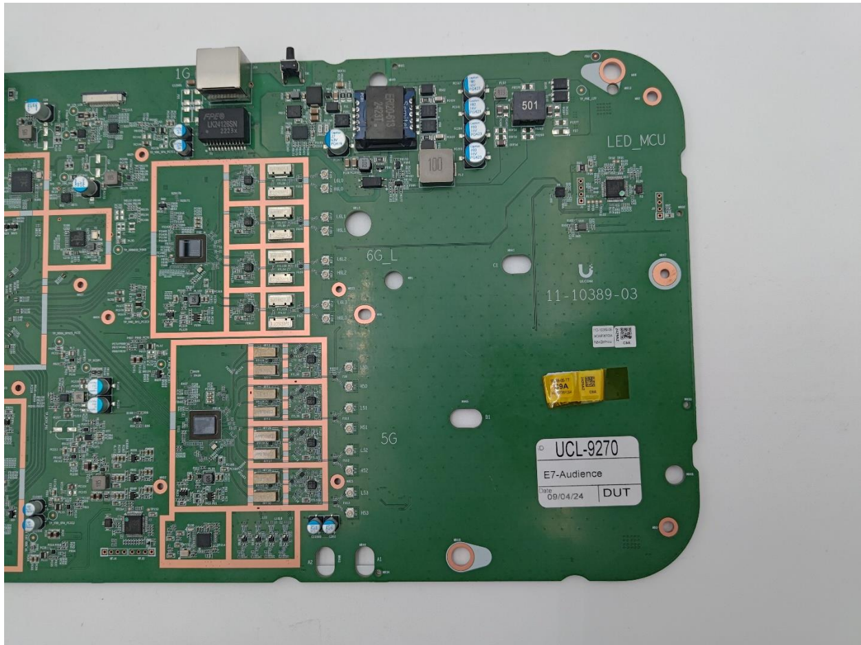
Photograph 7: Main PCB Top/Right
