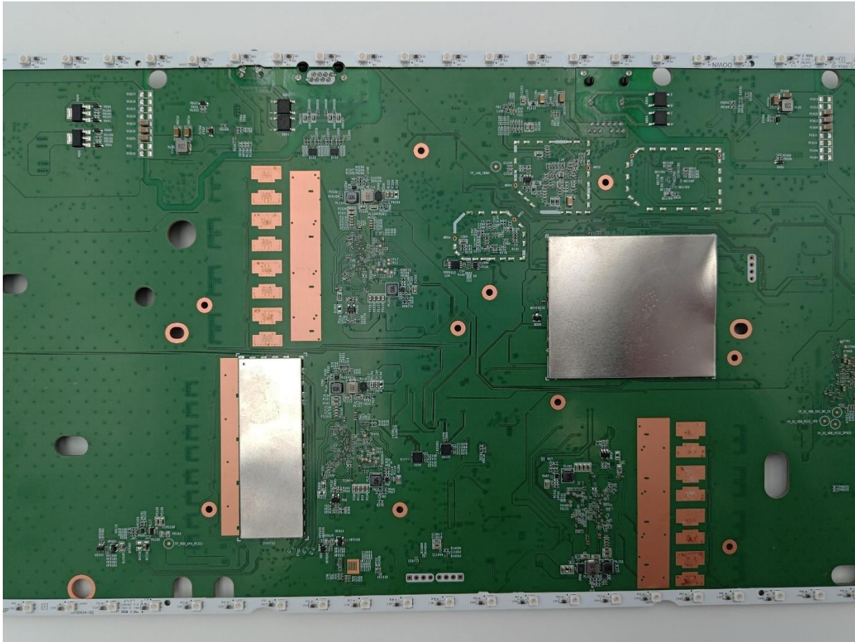
Photograph 10: Main PCB Bottom w/Cans/Middle
