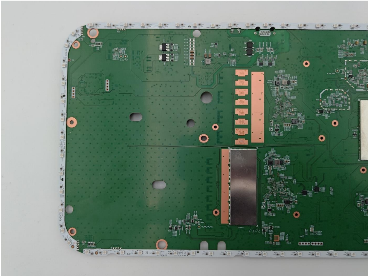
Photograph 9: Main PCB Bottom w/Cans/Left
