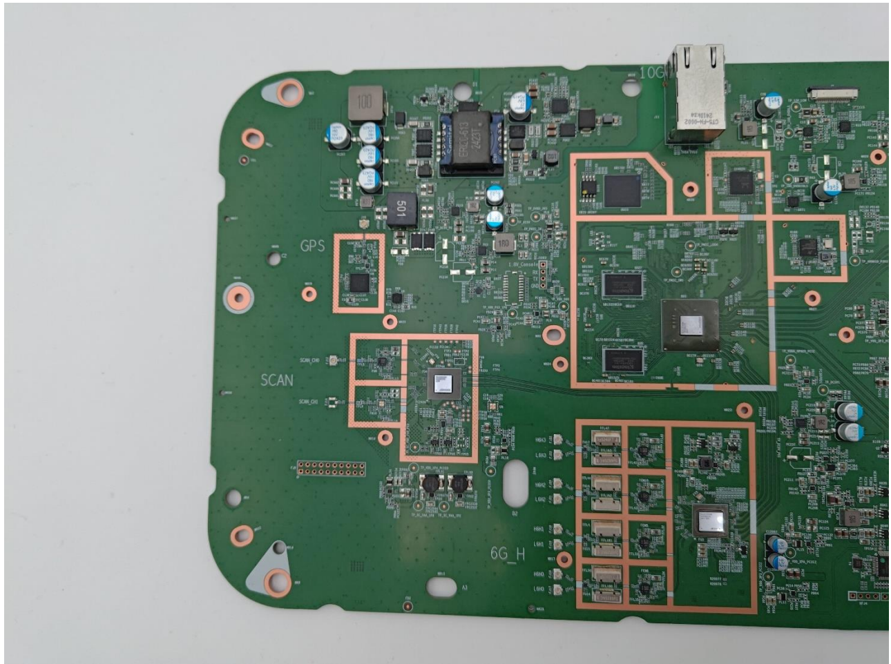
Photograph 5: Main PCB Top/Left
