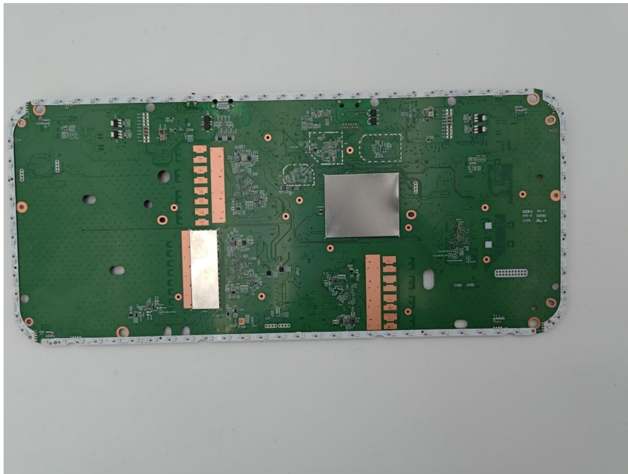
Photograph 8: Main PCB Bottom w/Cans
