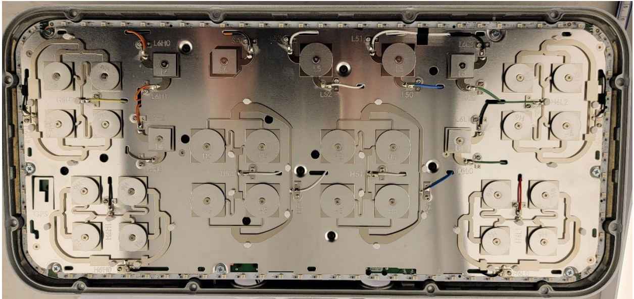
Photograph 16: Antenna Assembly
