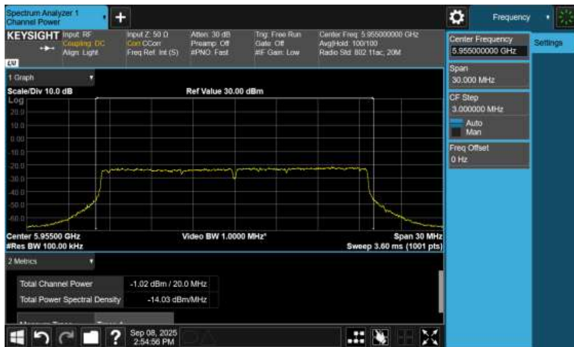
Plot 18: Power and PSD for Low-Power Indoor – 5955 MHz
