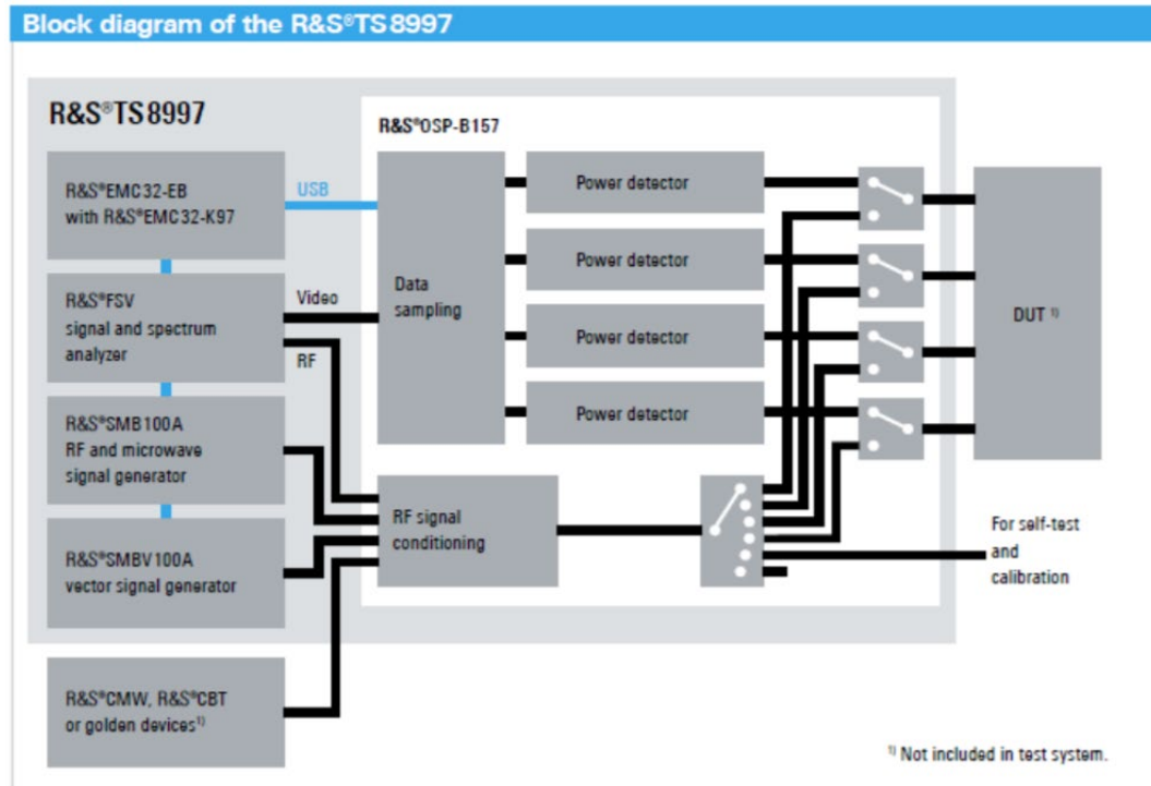
Diagram 1: Test Configuration Block Diagram
