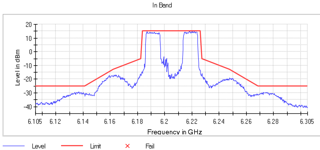
Figure 7: 6205 40MHz RU Vérification – Edge
