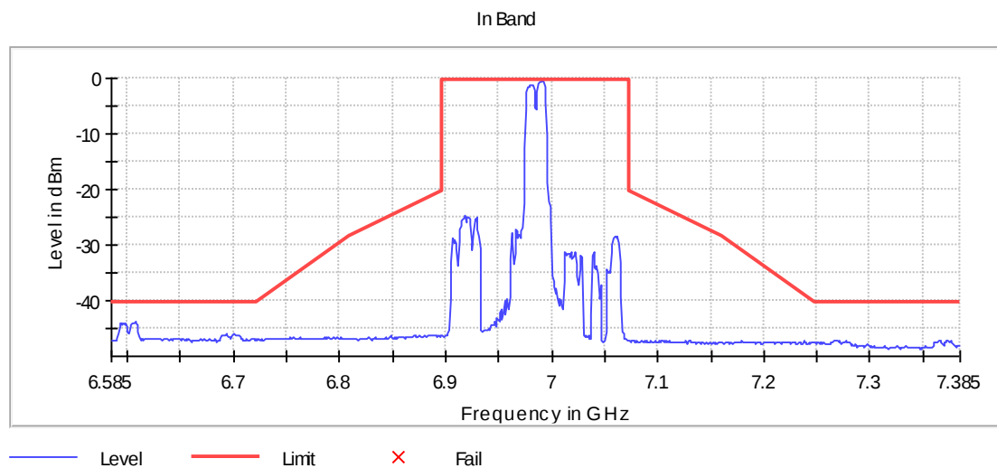
Figure 12: 6985 160MHz RU Vérification - Center
