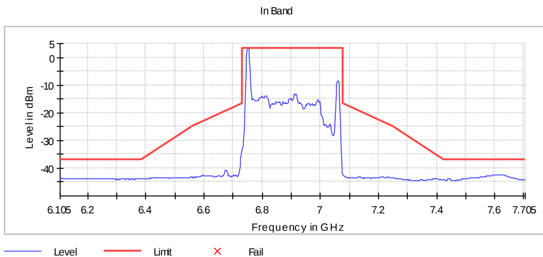
Figure 13: 6905 320MHz RU Vérification - Edge
