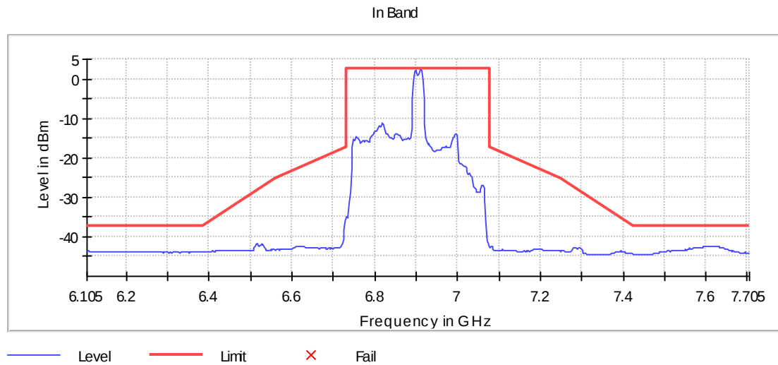
Figure 14: 6905 320MHz RU Vérification - Center
