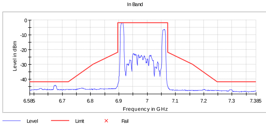
Figure 11: 6985 160MHz RU Vérification - Edge
