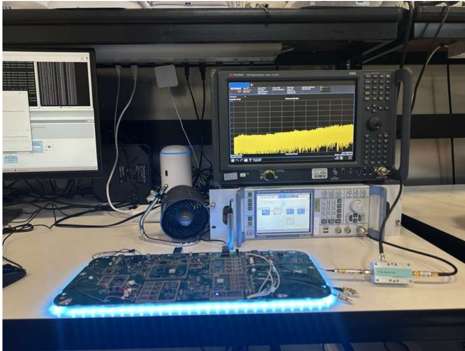
Photograph 5: View Test Set Up DFS
