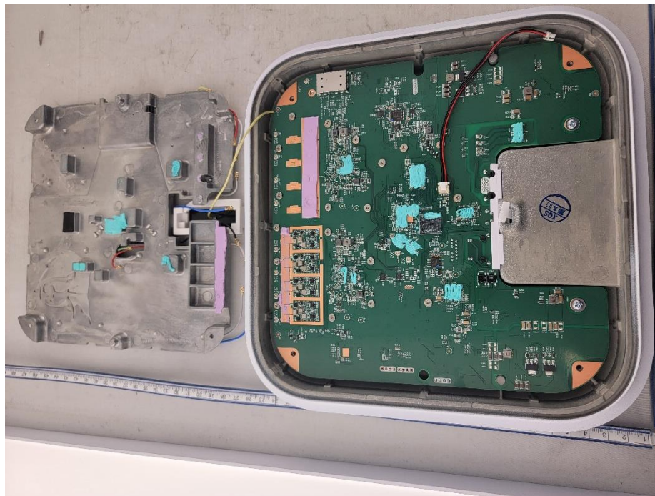
Photograph 2: Internal View of DUT
