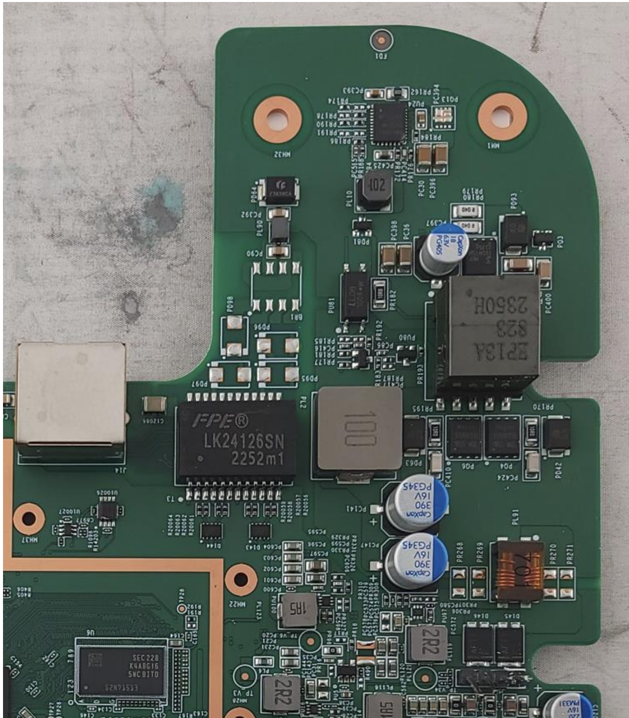
Photograph 6: Top Side Of PCB (Left/Top)
