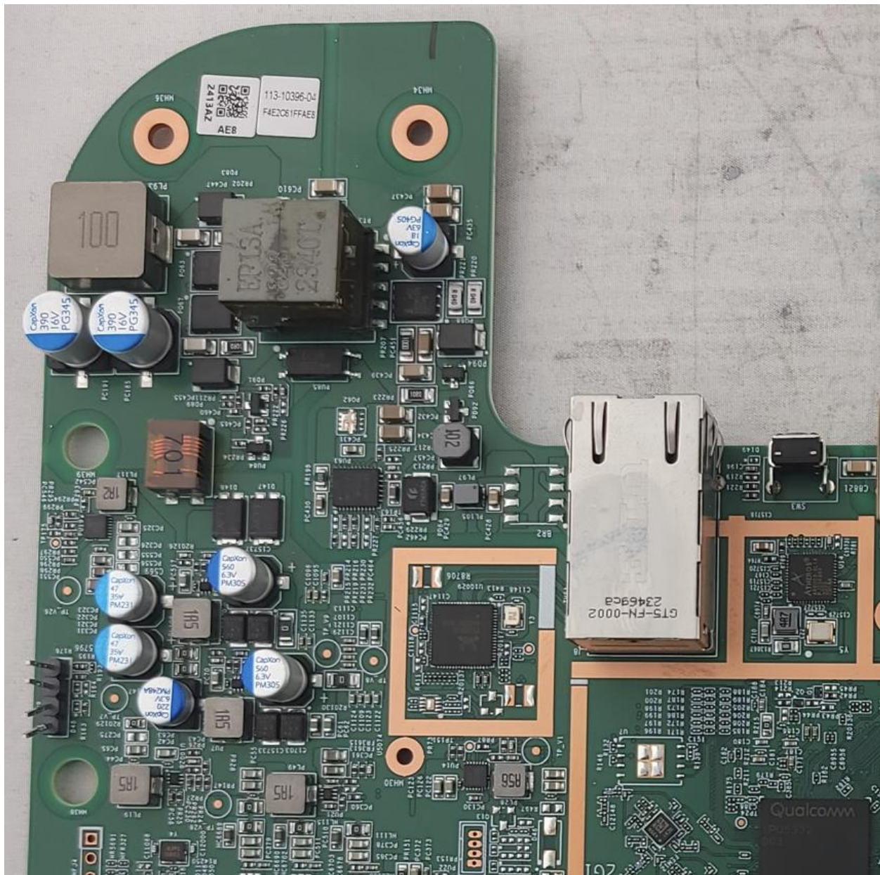
Photograph 5: Top Side Of PCB (Right/Top)
