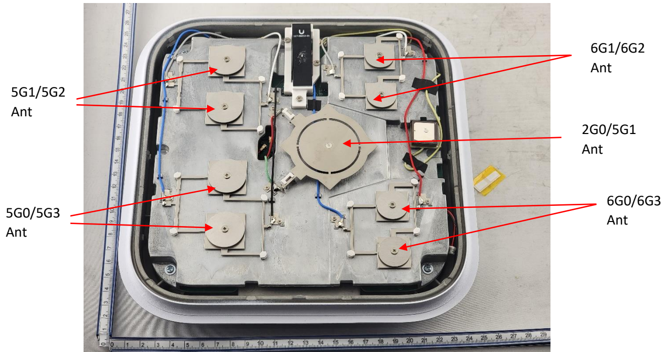
Photograph 1: Internal View of DUT
