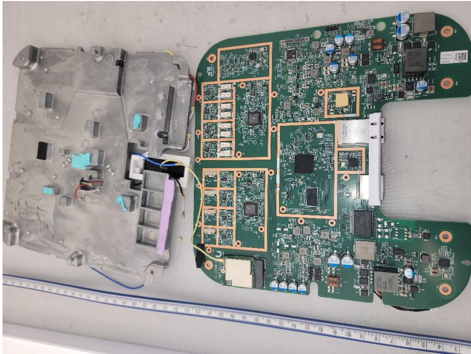
Photograph 3: Internal View of DUT
