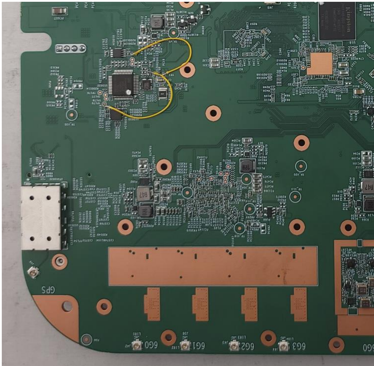
Photograph 5: Bottom Side Of PCB (Right/Bottom)
