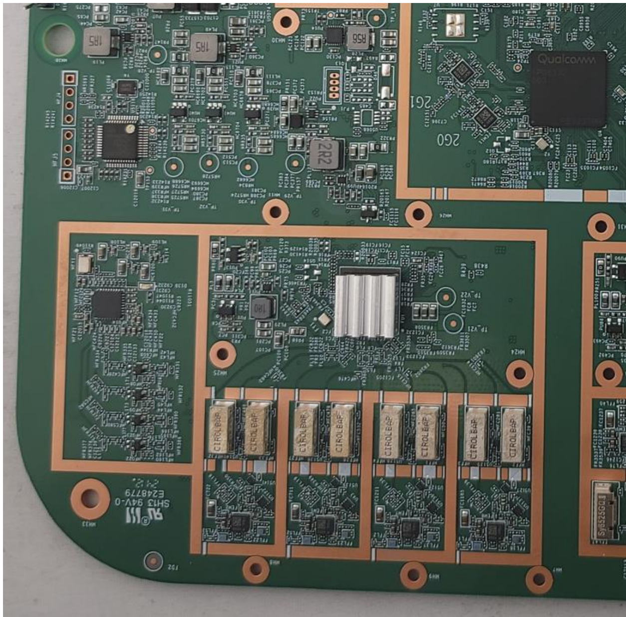
Photograph 1: Top Side Of PCB (Right/Bottom)
