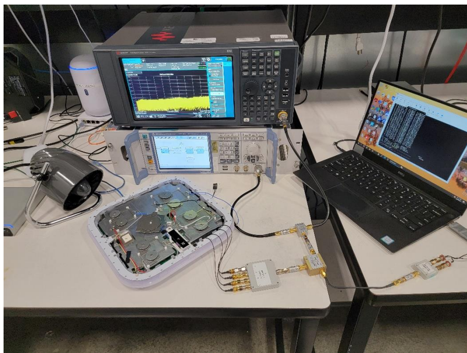
Photograph 6: View Test Setup DFS
