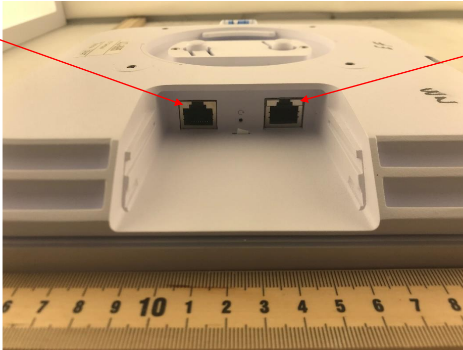
Photograph 7: Bottom Port View of DUT Showing Connectors
